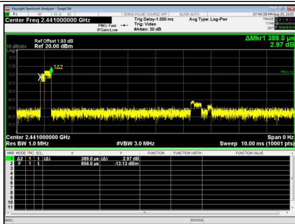
2DH3-2441MHz-One burst
