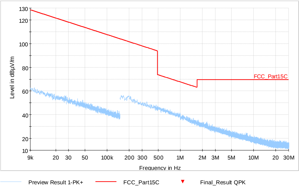
Fig. 3: Ambient level. X axis. Frequency range: 9 kHz – 30 MHz
