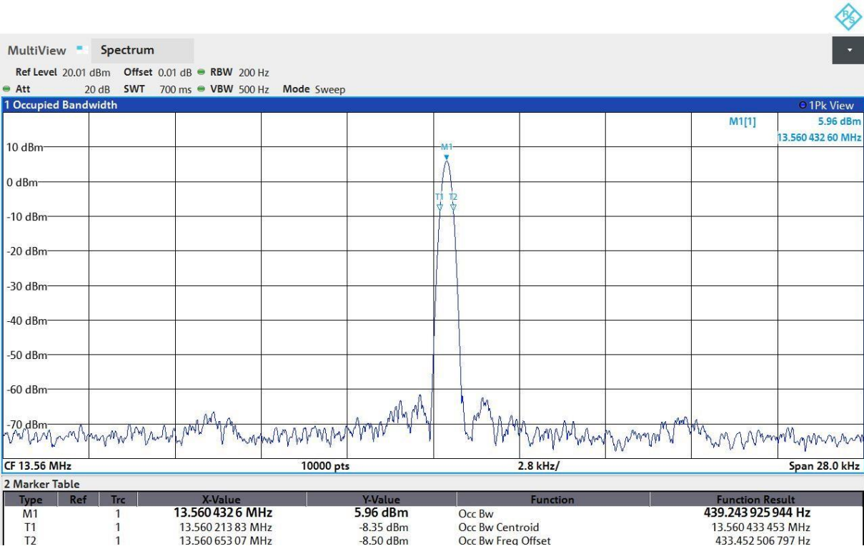
Fig. 15: 99% Bandwidth
