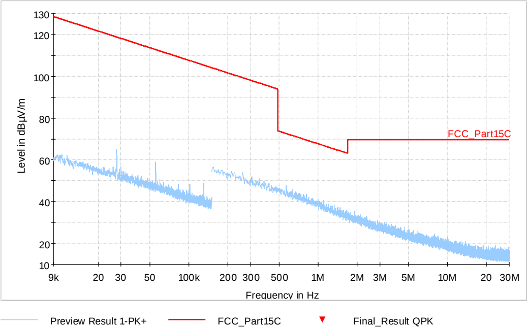
Fig. 5: Ambient level. Z axis. Frequency range: 9 kHz – 30 MHz
