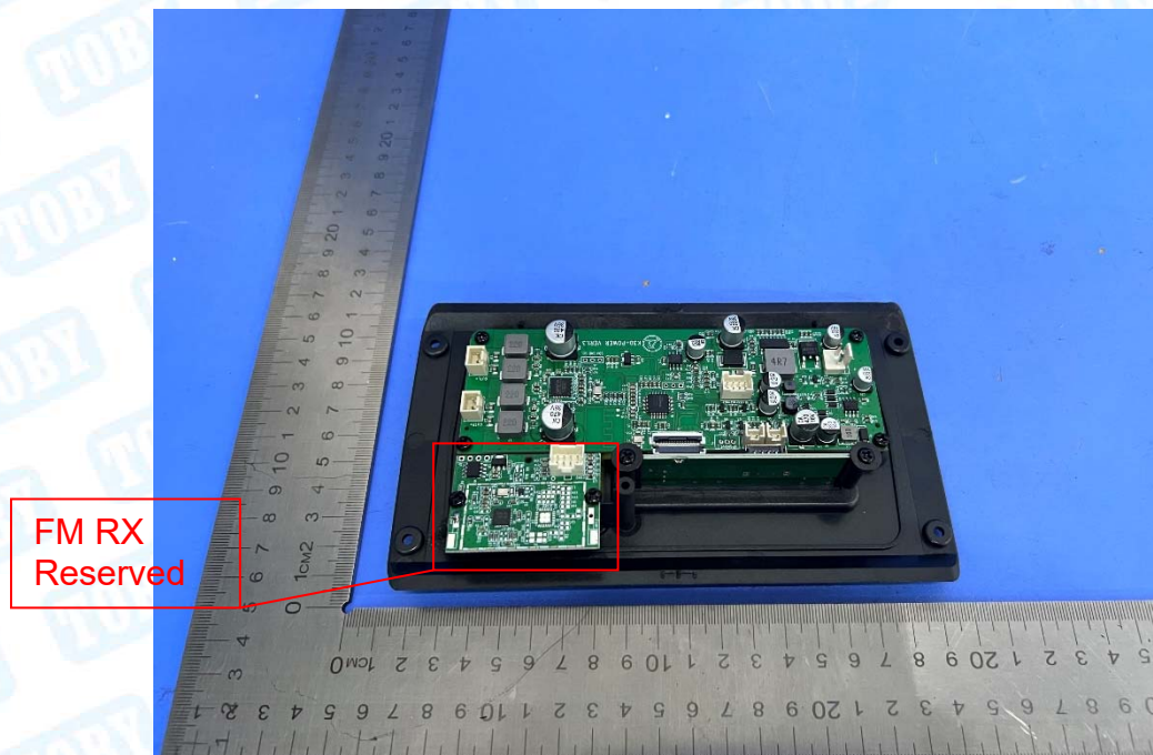
Photo 9 Internal of EUT
