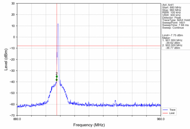
LCH_902.75MHz_Ant1_NTNV
