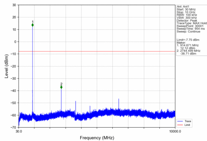
MCH_914.75MHz_Ant1_NTNV
