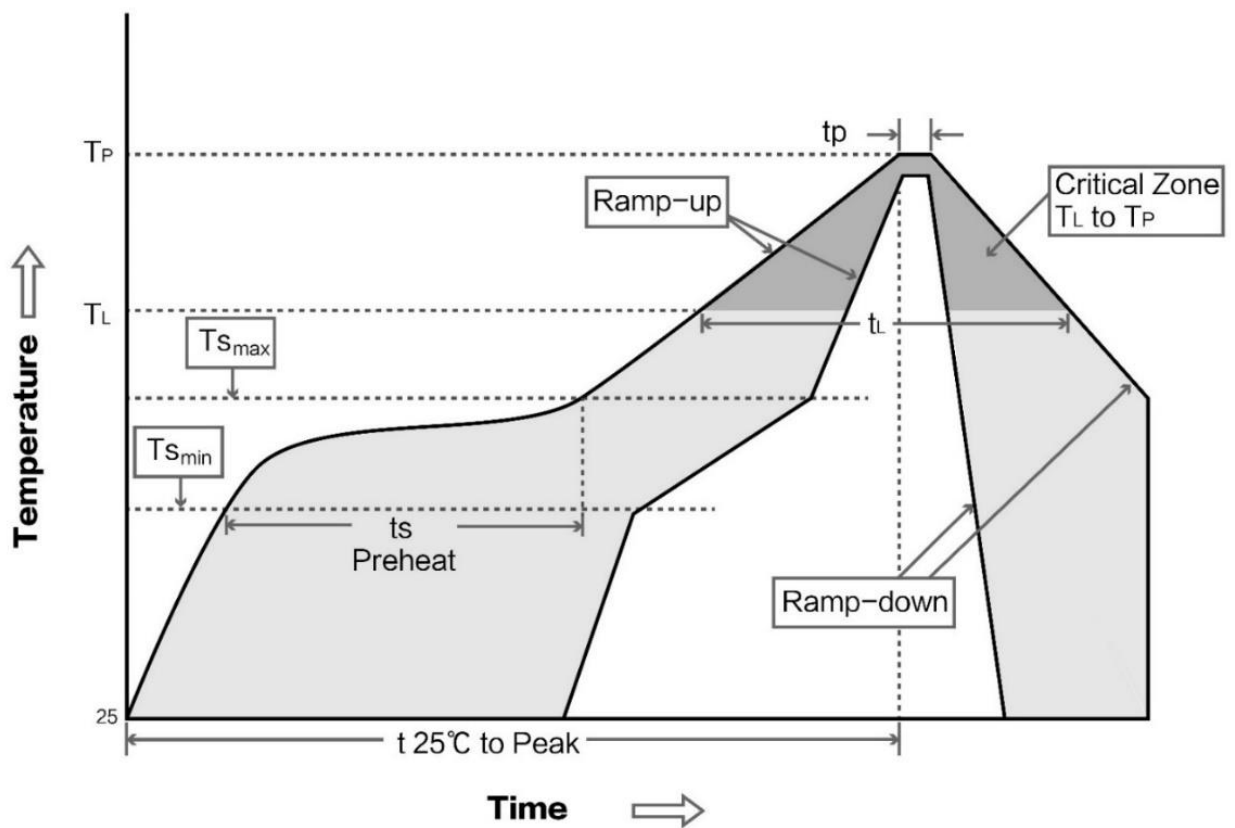
Figure 12 Reflow weld curve diagram
