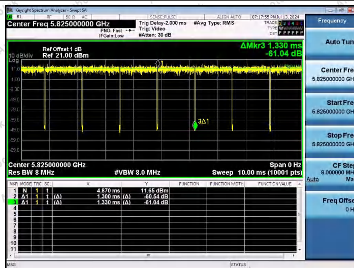
NTVN-11N20SISO-Ant1-5825
