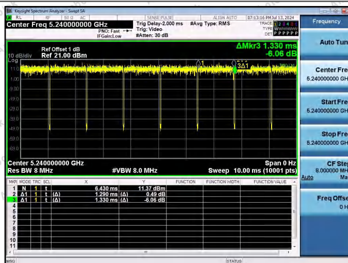
NTNV-11N20SISO-Ant1-5240
