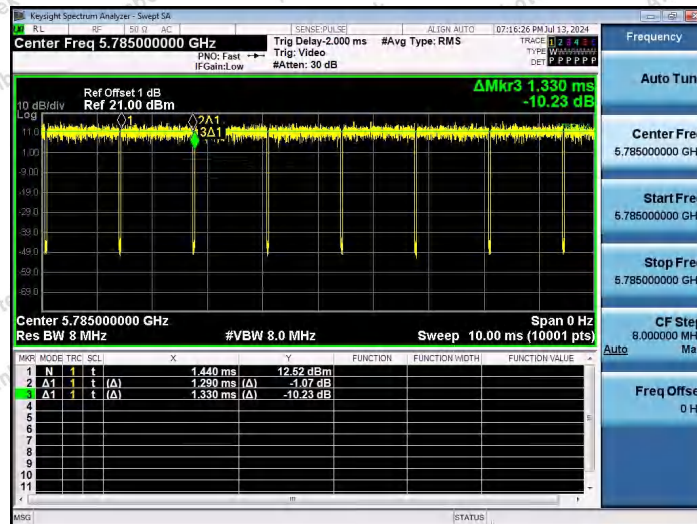
NTVN-11N20SISO-Ant1-5785
