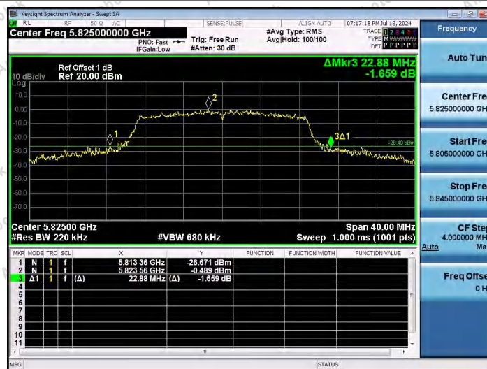
11N20SISO-Ant1-5825
