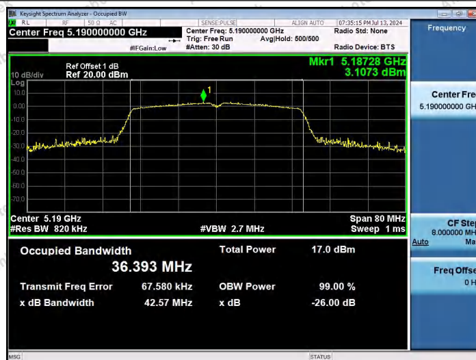
11AC40SISO-Ant1-5190
