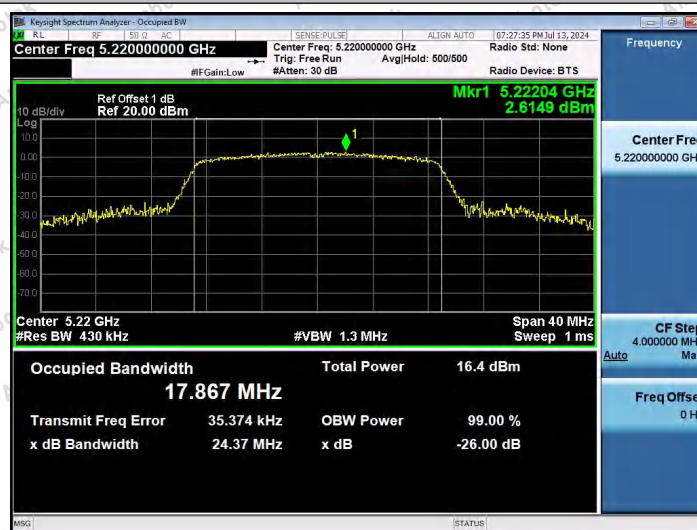
11AC20SISO-Ant1-5220
