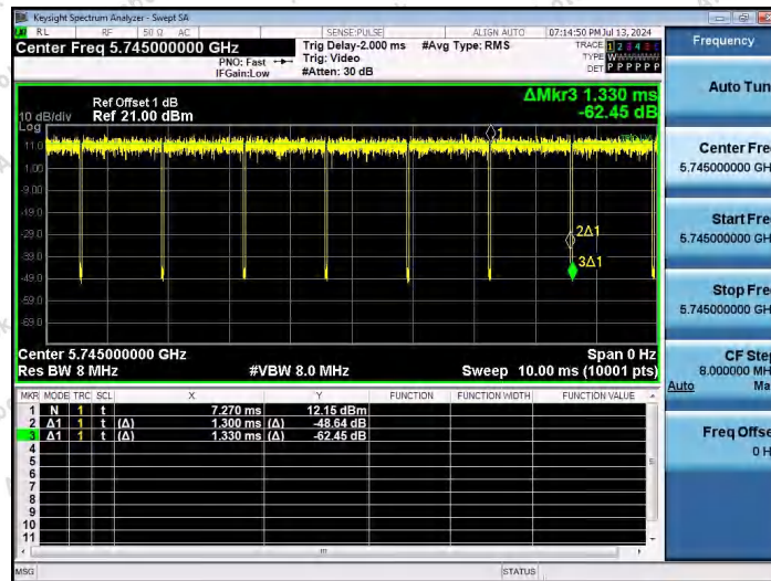
NTVN-11N20SISO-Ant1-5745
