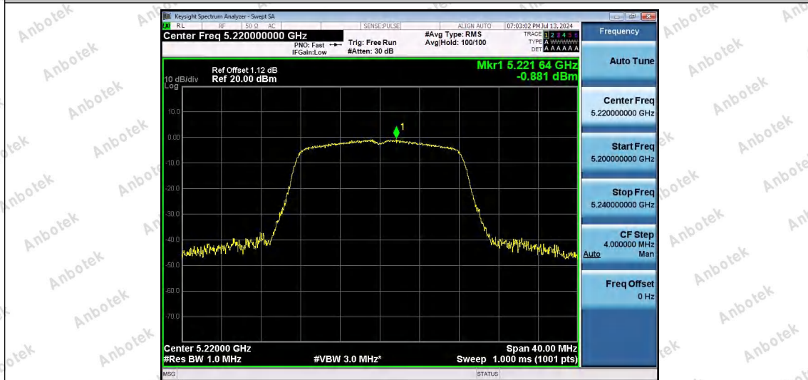
11A-Ant1-5220-PASS
