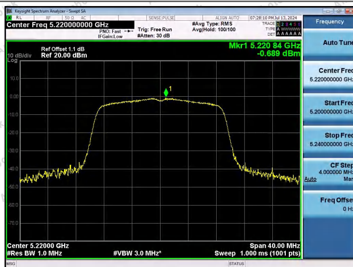
11AC20SISO-Ant1-5220-PASS
