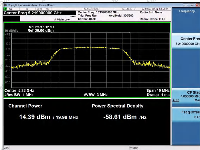
11A-Ant1-5220-PASS
