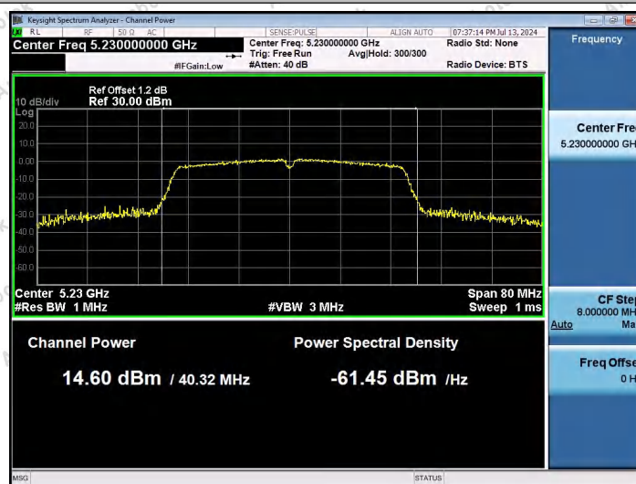
11AC40SISO-Ant1-5230-PASS
