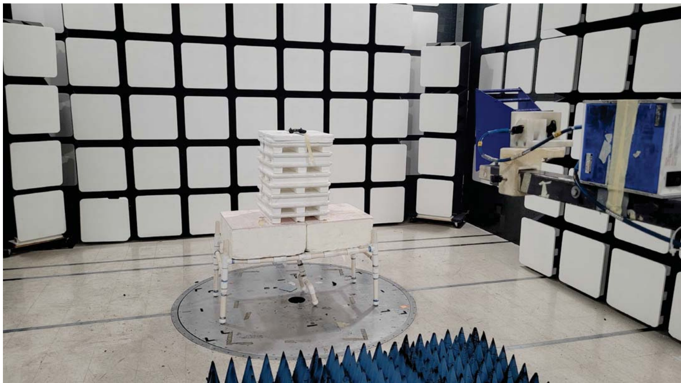
FRONT VIEW
