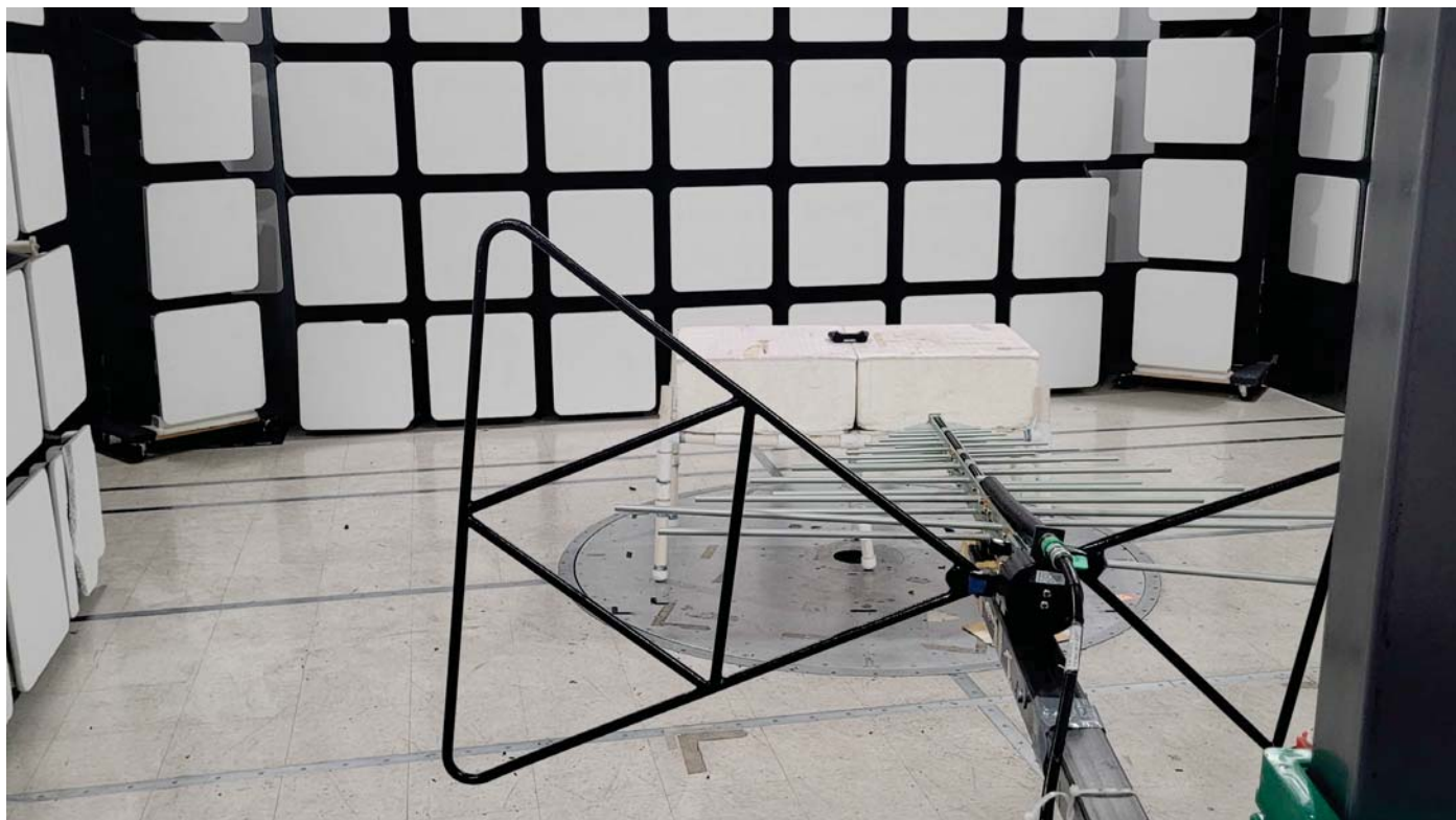
REAR VIEW
