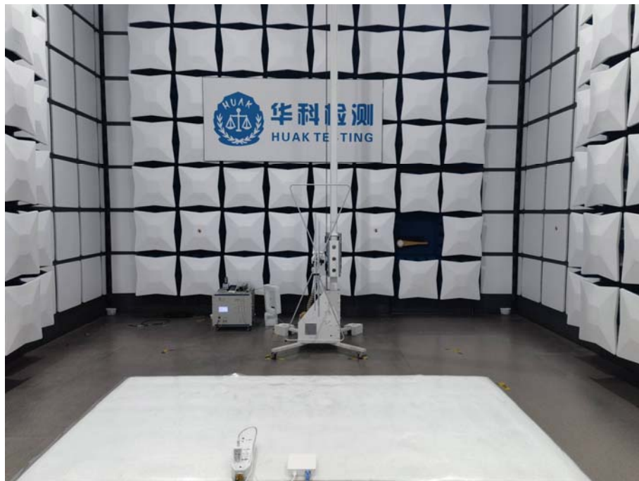
FGS80B0 Radiated Emissions
