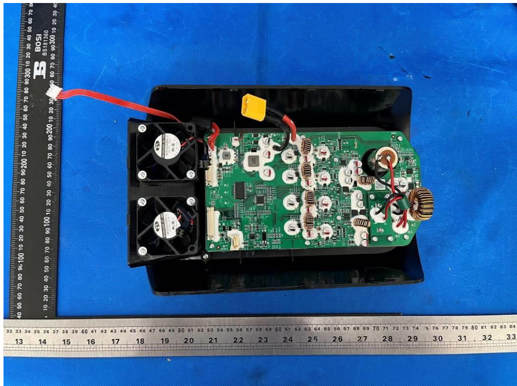
Figure 6 Internal view (DC output side)
