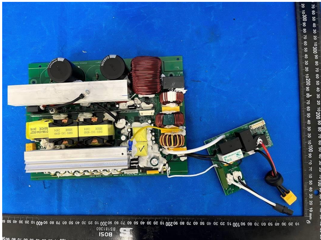
Figure 13 Top view of inverter & relay board
