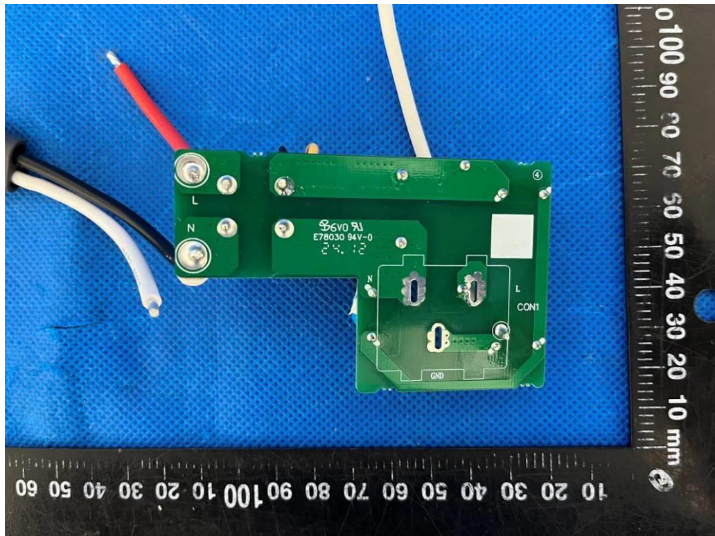
Figure 5 Bottom view of AC input board
