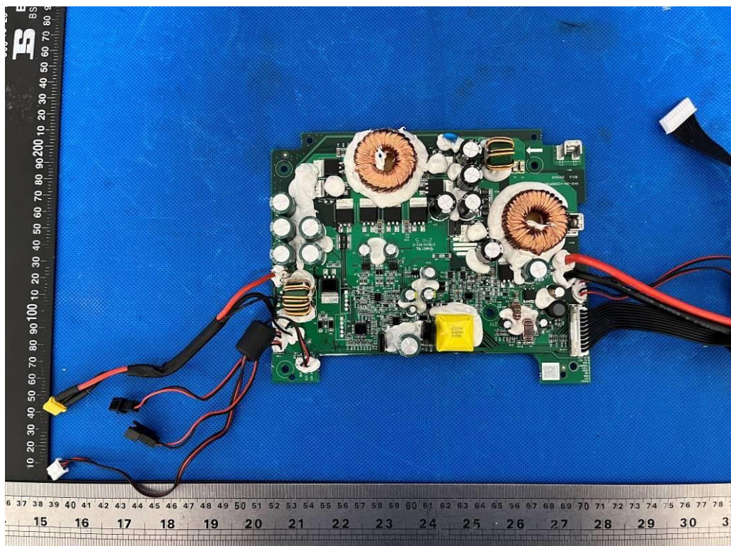
Figure 22 Top view of MPPT board
