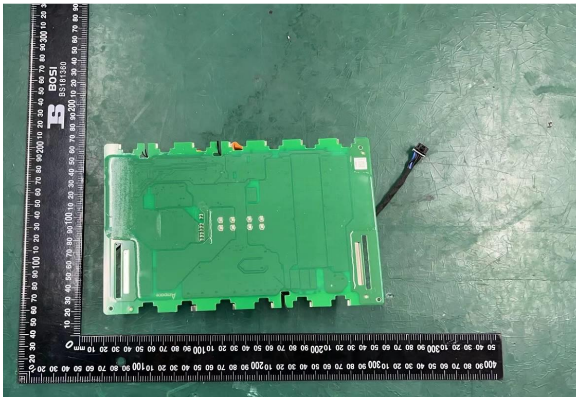
Figure 30 Bottom view of BMS board
