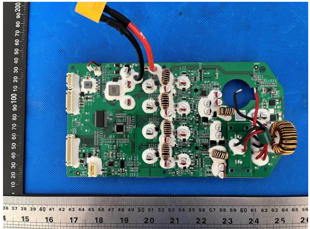
Figure 8 Top view of DC output board
