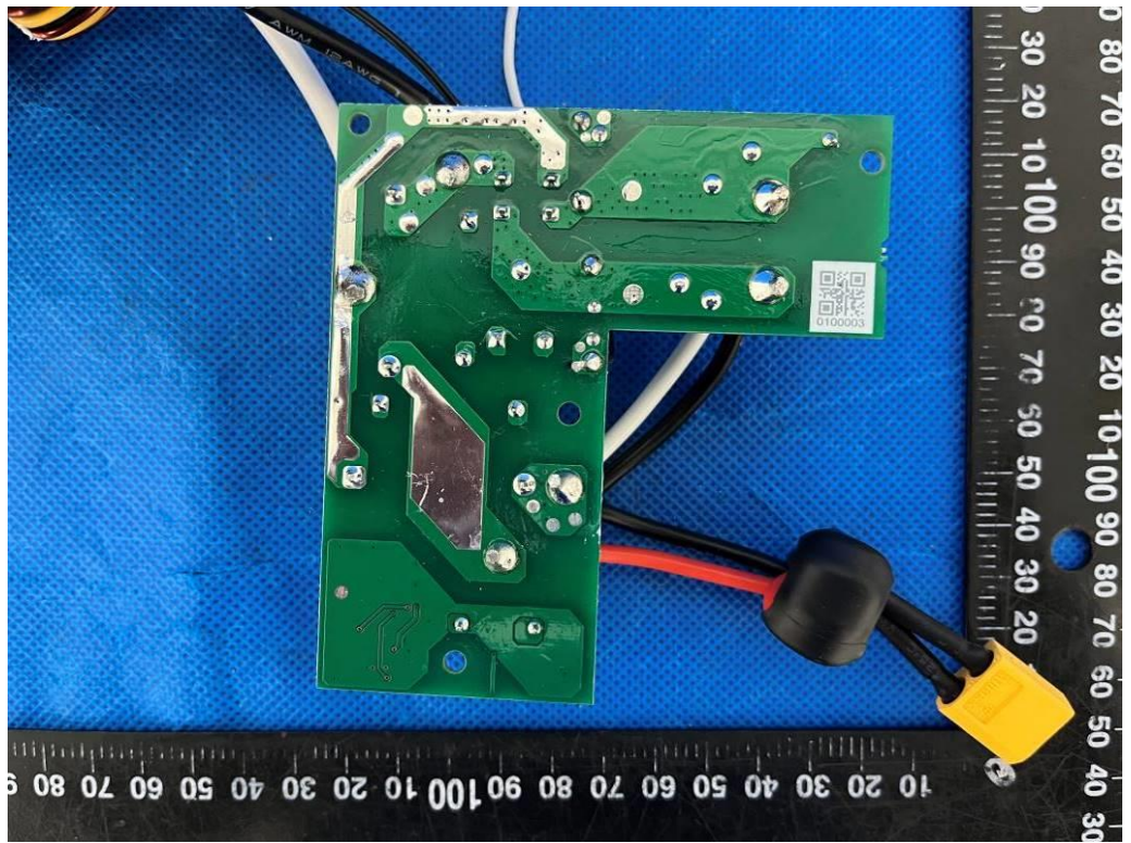
Figure 17 Bottom view of relay board
