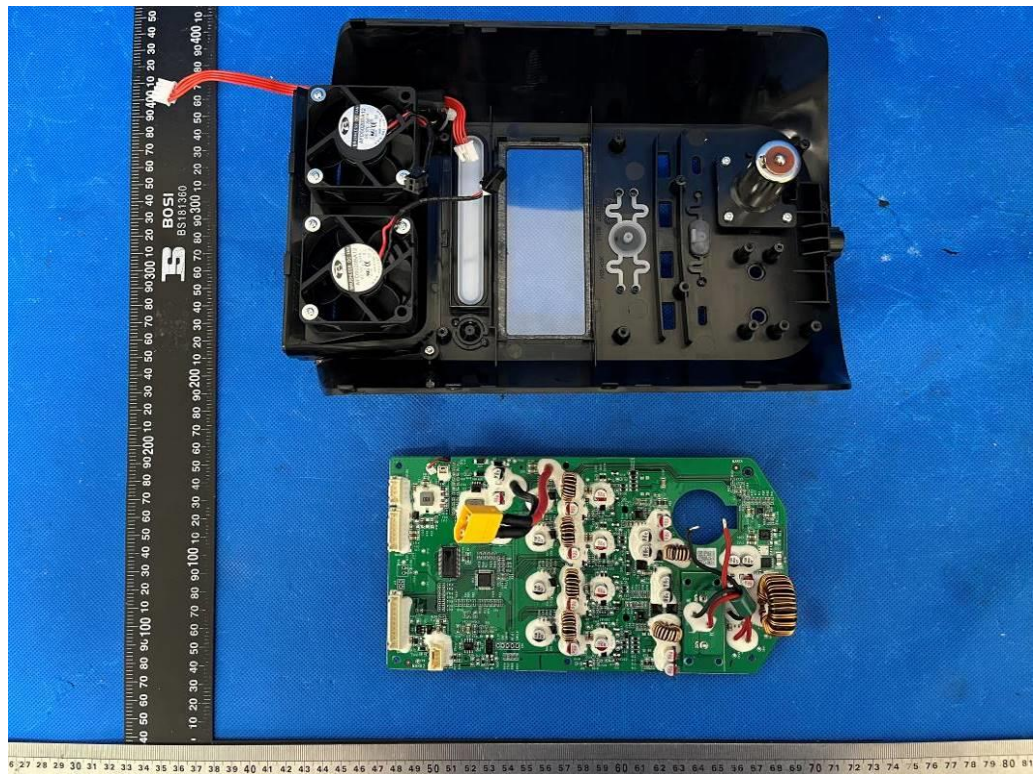
Figure 7 Internal view (DC output side)
