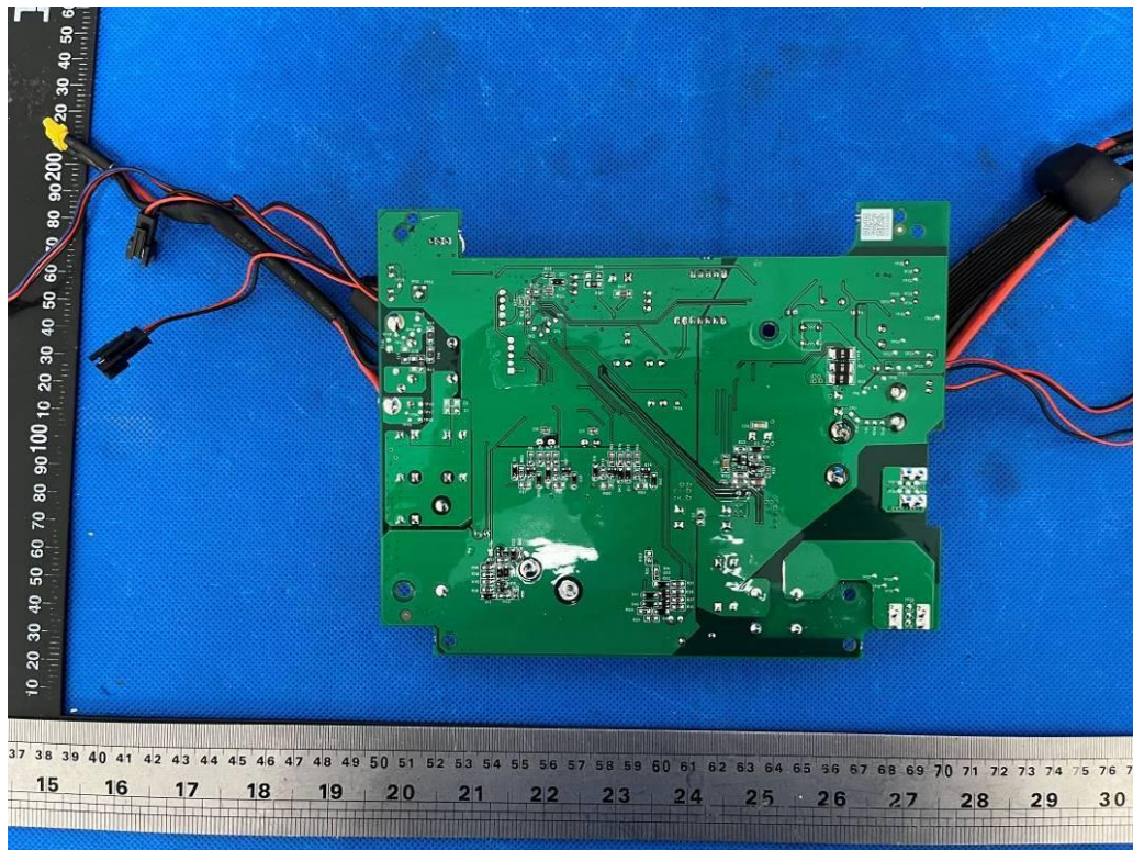
Figure 23 Bottom view of MPPT board
