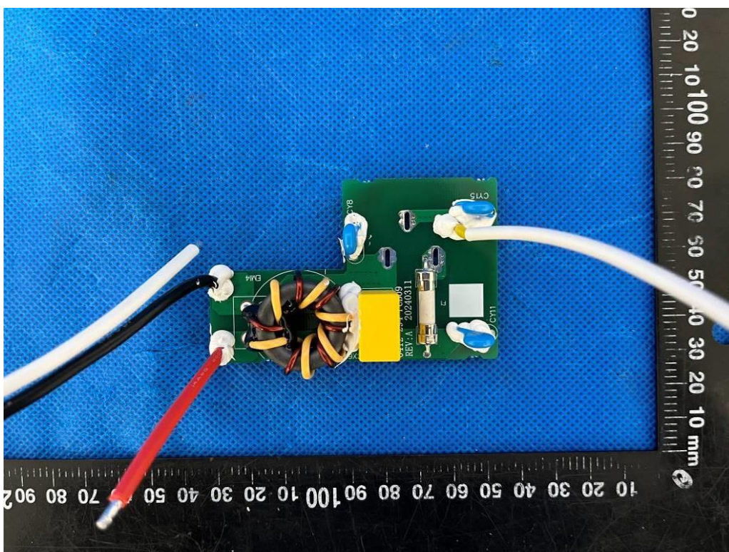
Figure 4 Top view of AC input board
