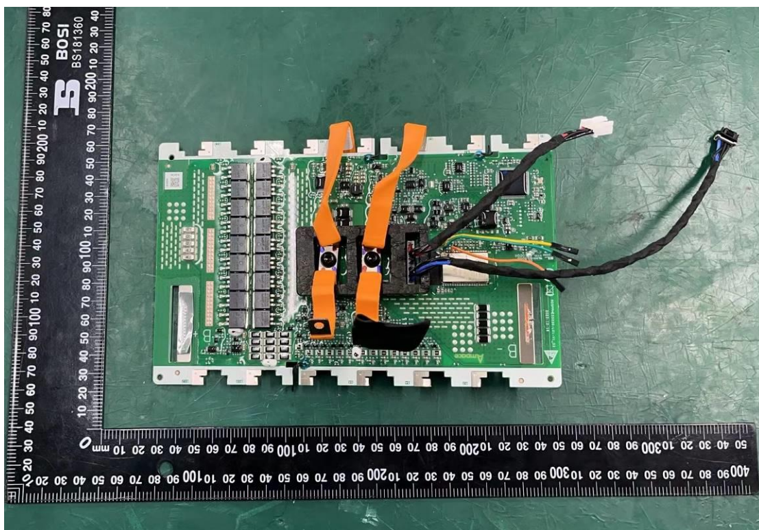
Figure 27 Top view of BMS board
