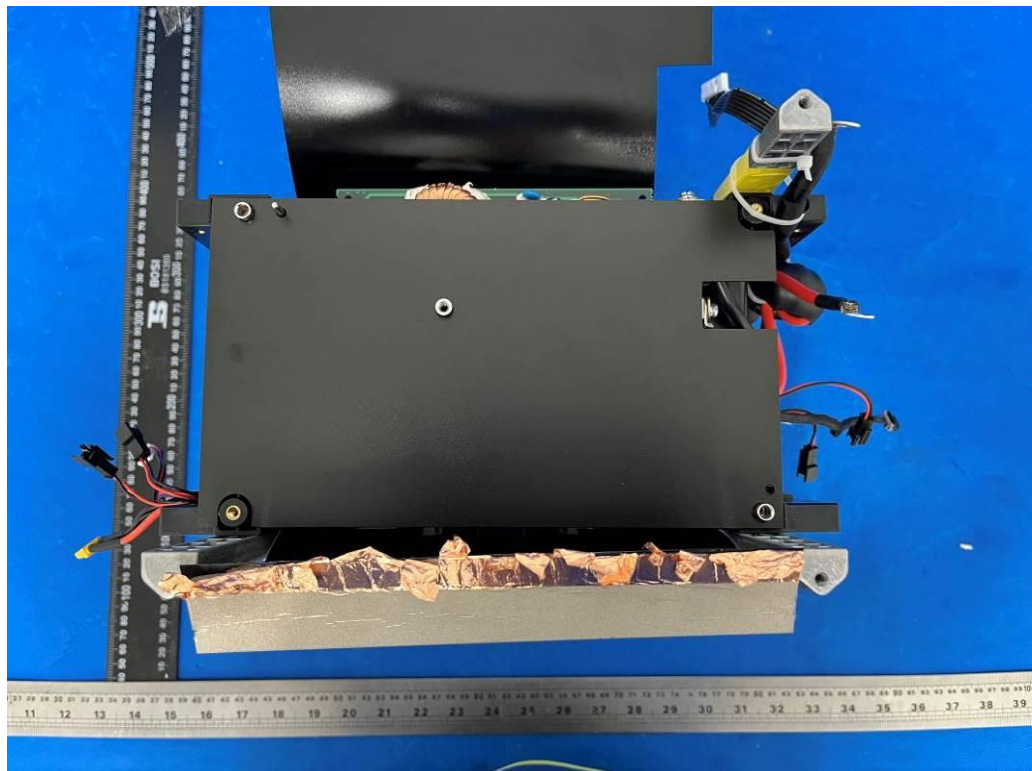
Figure 12 Internal view
