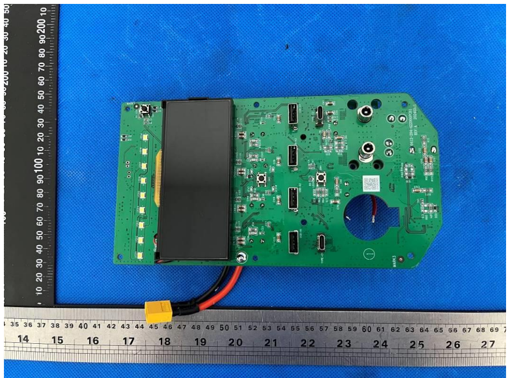
Figure 9 Bottom view of DC output board
