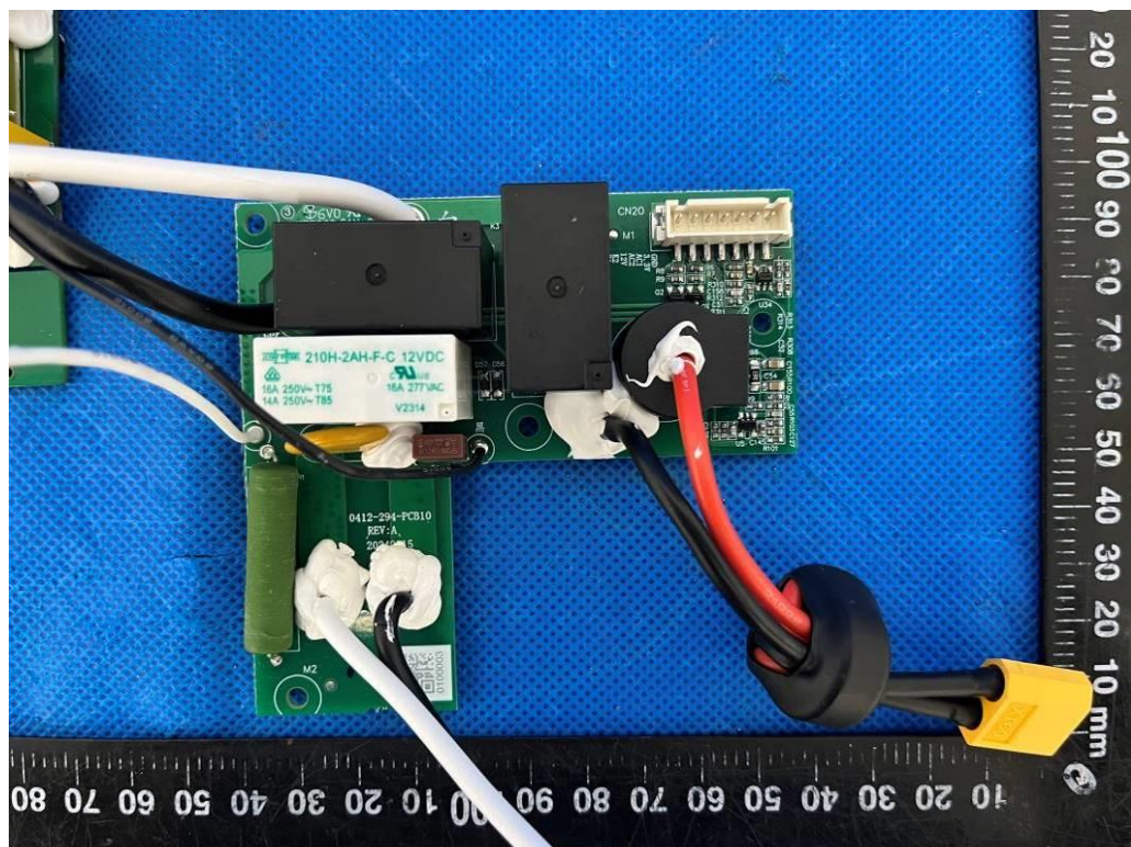
Figure 16 Top view of relay board
