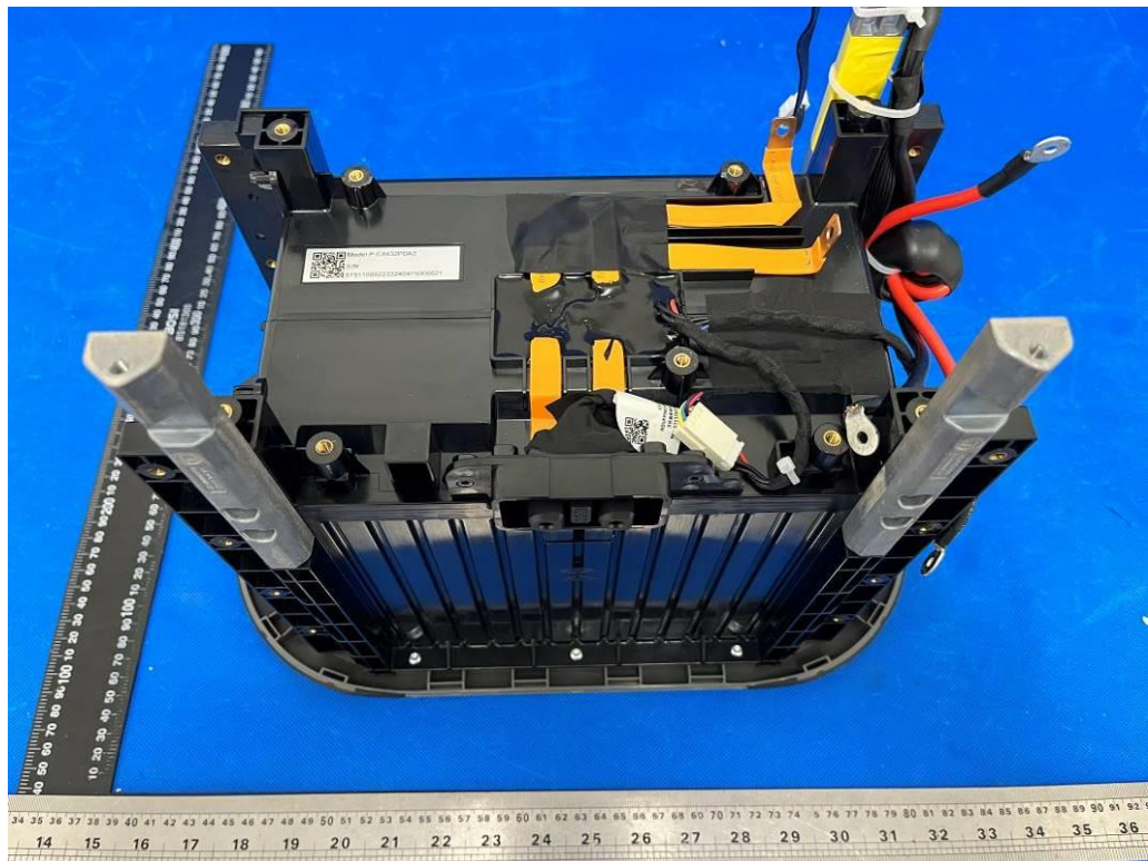
Figure 25 Battery module (include BMS board)
