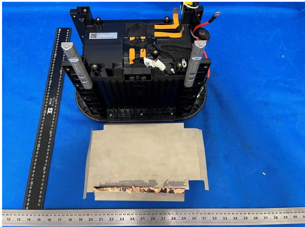
Figure 24 Internal view
