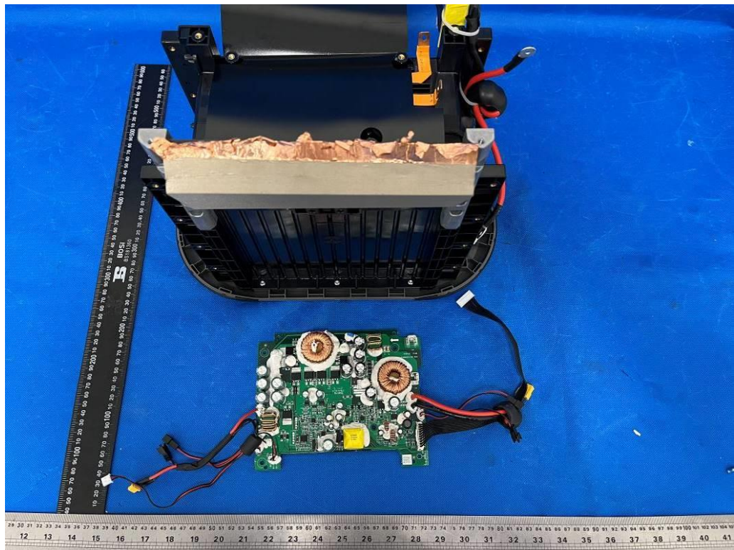
Figure 21 Internal view
