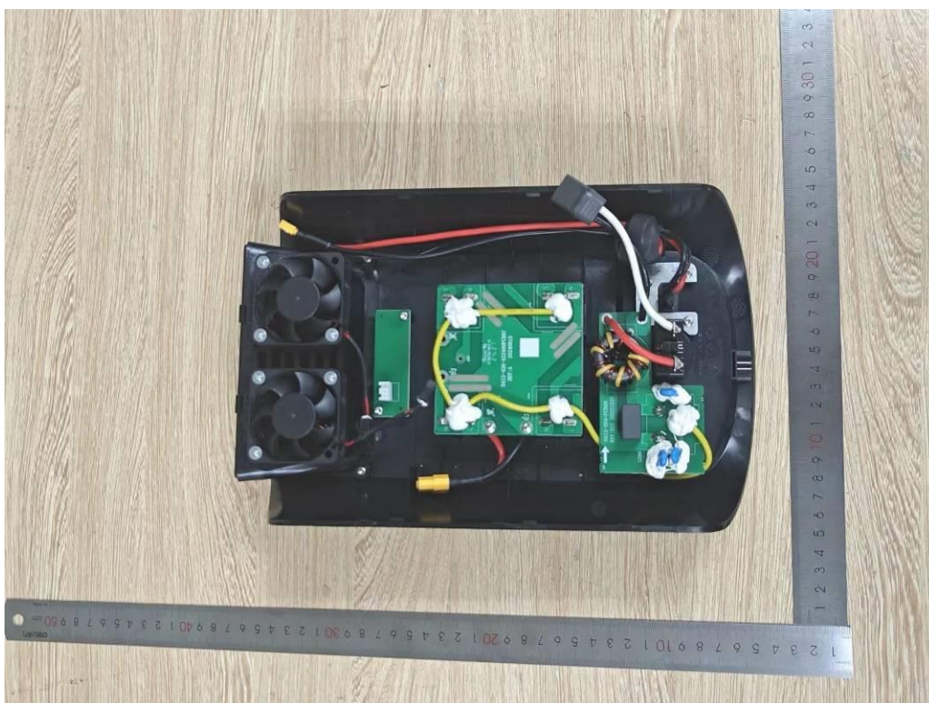
Figure 3 Internal view (Input & AC output side)
