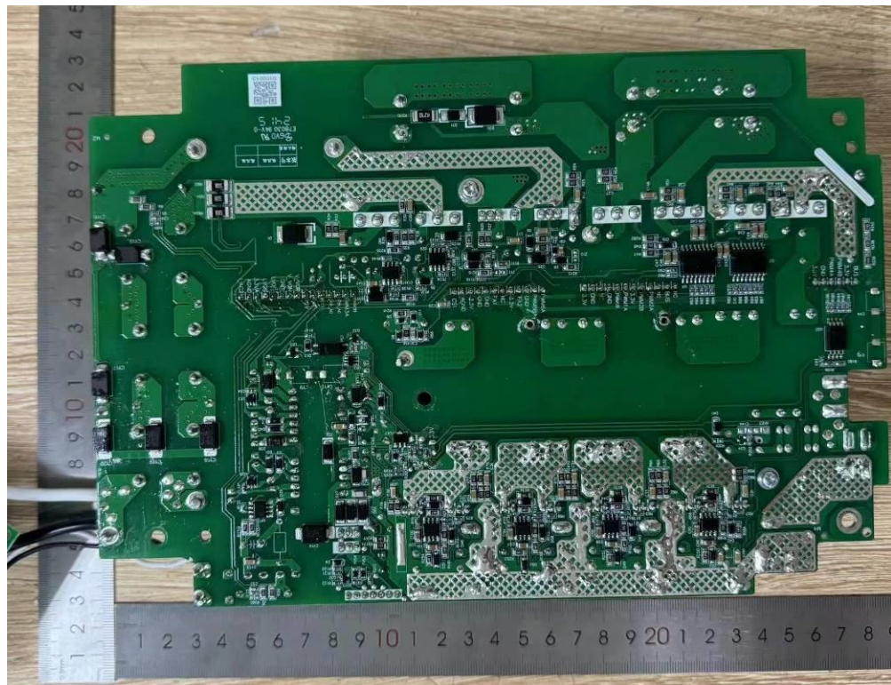
Figure 15 Bottom view of inverter board
