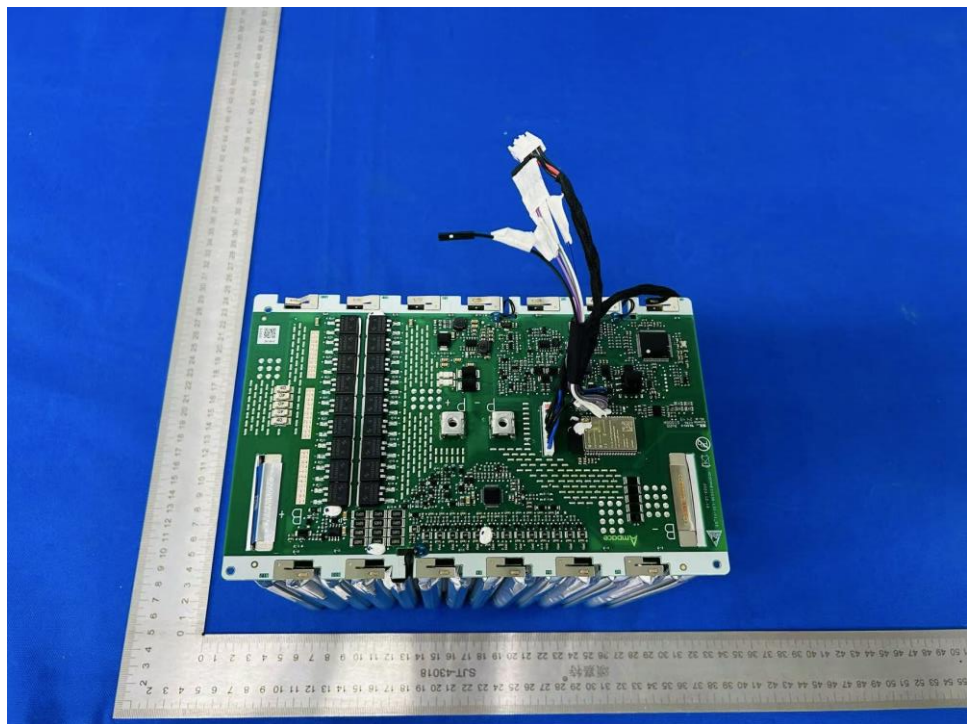
Figure 26 Internal view of battery module
