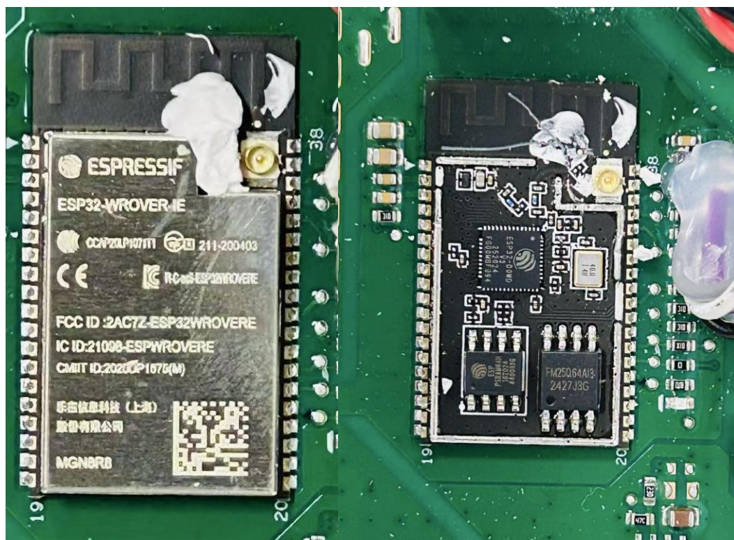
Figure 28 Wireless module
