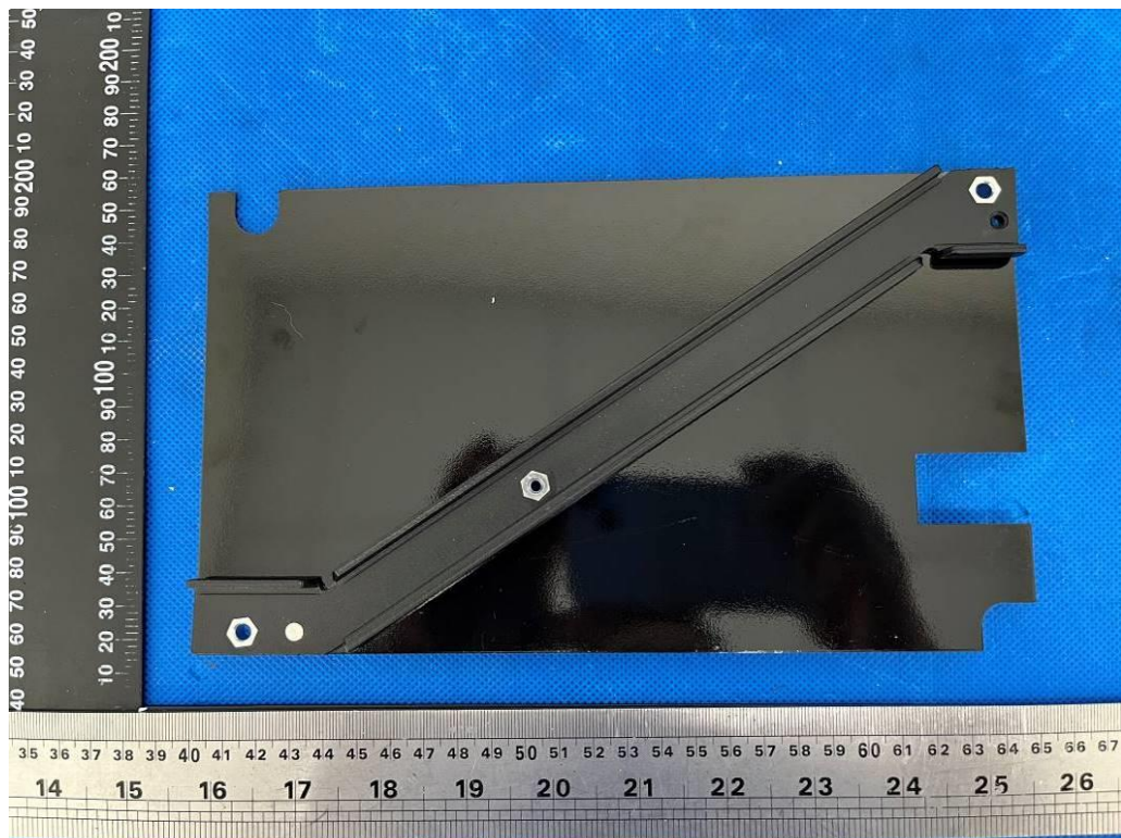
Figure 19 Bottom view of Mylar (Between the inverter & MPPT board)
