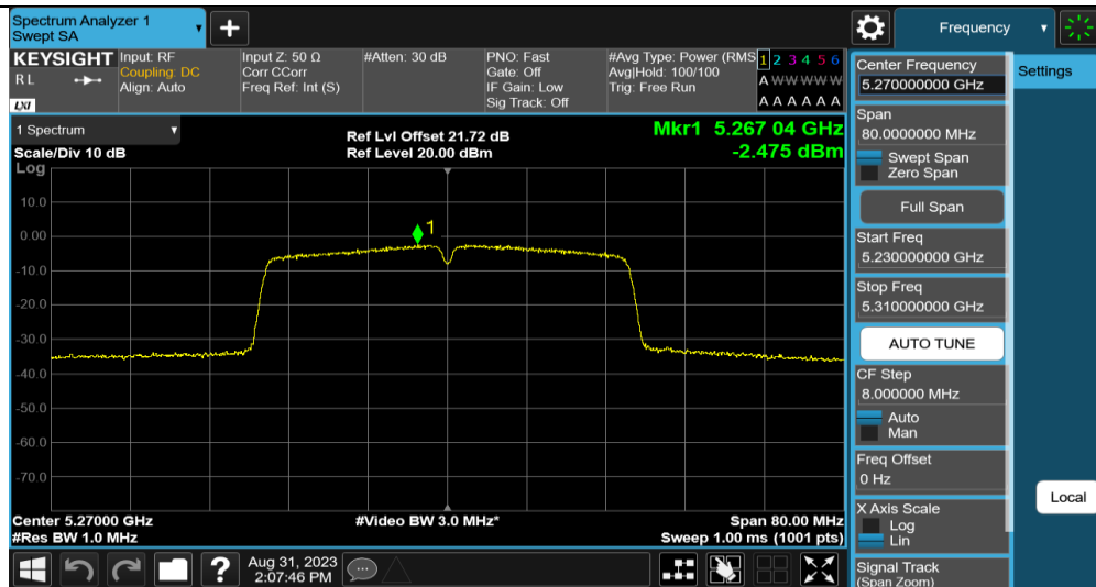
11N40MIMO Ant2 5270
