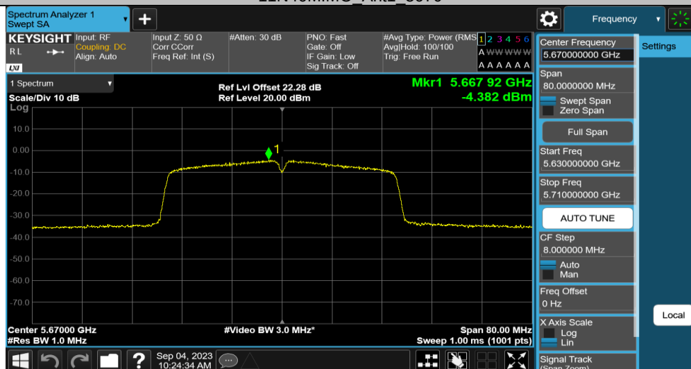
11N40MIMO Ant2 5670
