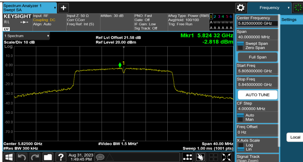
11N20MIMO Ant2 5825
