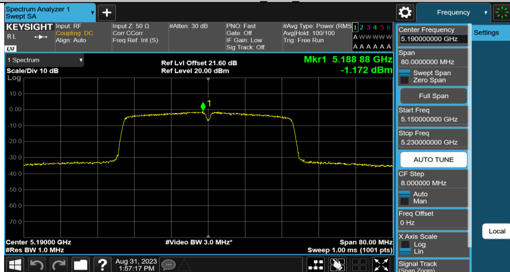
11N40MIMO Ant2 5190
