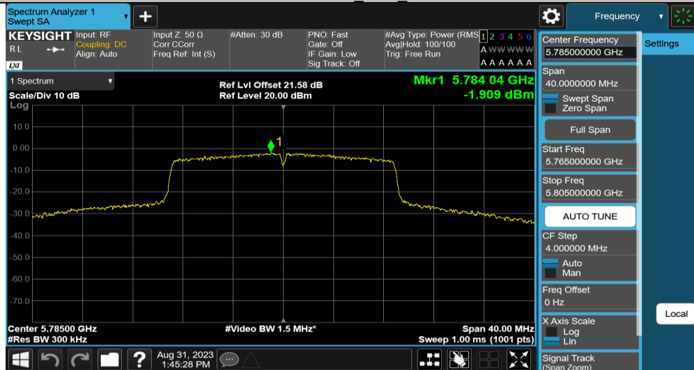
11N20MIMO Ant2 5785
