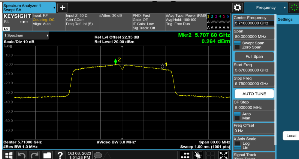
11N40MIMO Ant2 5710
