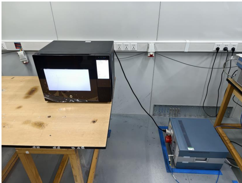
Conducted Disturbance
