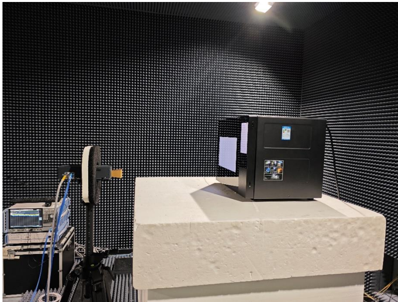
Radiated Emission Above 42GHz
