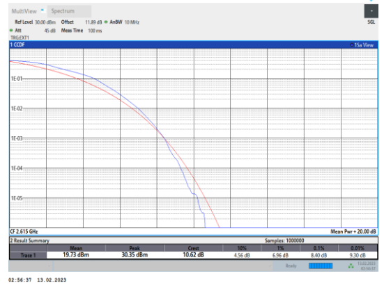
Band38-10MHz-16QAM-38200-50RB#0
