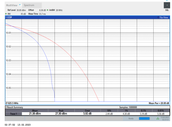
Band5-3MHz-QPSK-20415-15RB#0
