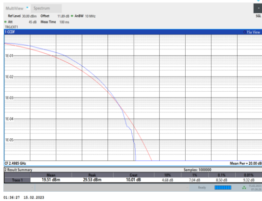
Band41-5MHz-64QAM-39675-25RB#0
