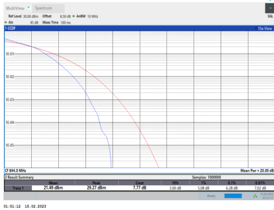
Band5-10MHz-64QAM-20600-50RB#0
