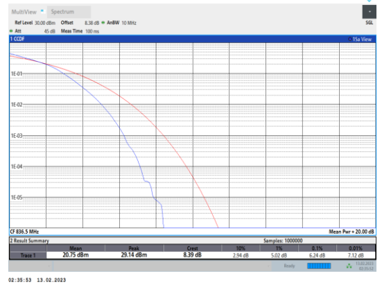
Band5-10MHz-16QAM-20525-50RB#0
