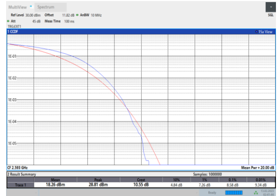
Band41-20MHz-16QAM-40620-100RB#0
