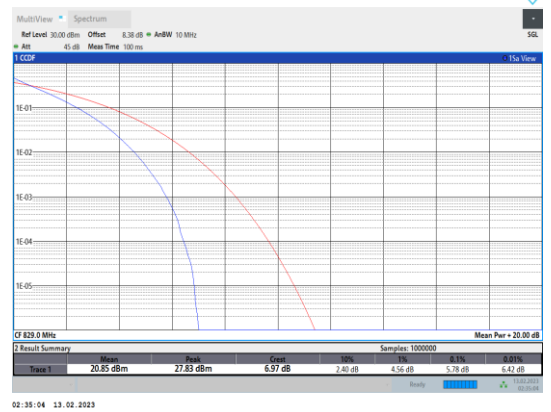
Band5-10MHz-QPSK-20450-50RB#0
