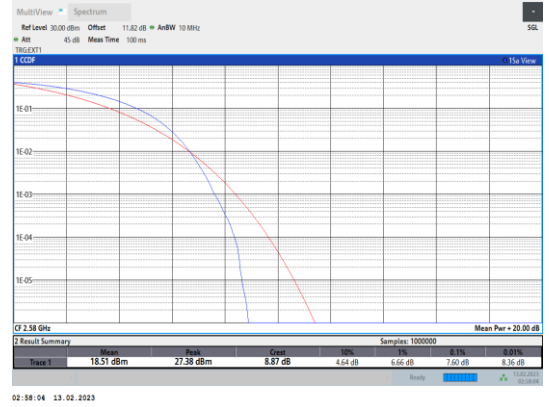
Band38-20MHz-QPSK-37850-100RB#0
