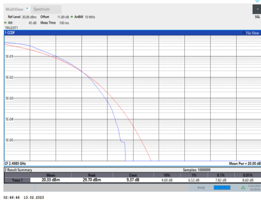
Band41-5MHz-QPSK-39675-25RB#0
