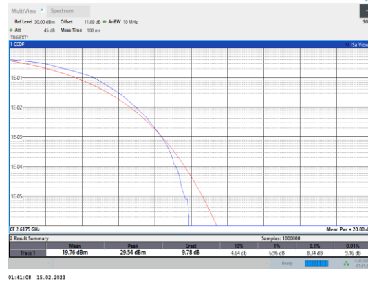
Band38-5MHz-64QAM-38225-25RB#0
