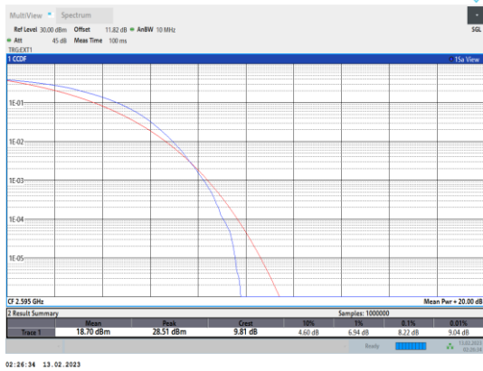
Band38-15MHz-16QAM-38000-75RB#0
