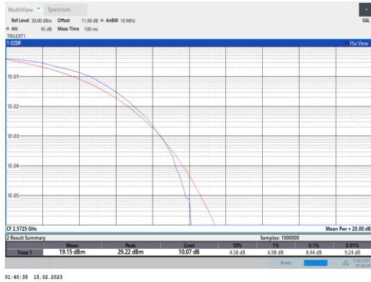
Band38-5MHz-64QAM-37775-25RB#0
