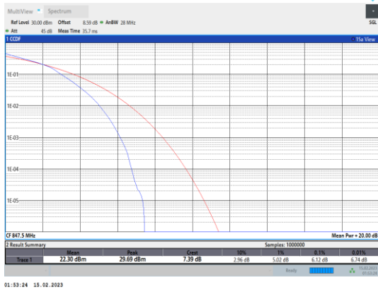
Band5-3MHz-64QAM-20635-15RB#0
