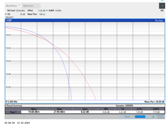
Band41-15MHz-QPSK-40620-75RB#0
