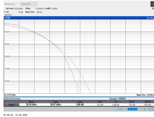
Band38-10MHz-QPSK-37800-50RB#0
