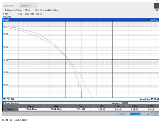
Band41-10MHz-64QAM-40620-50RB#0
