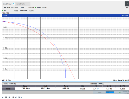
Band38-20MHz-64QAM-38150-100RB#0
