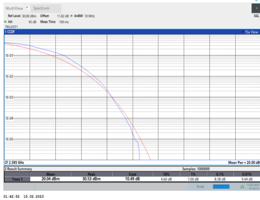
Band38-10MHz-64QAM-38000-50RB#0
