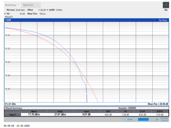
Band38-20MHz-16QAM-38150-100RB#0
