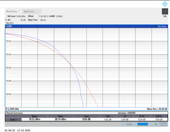
Band41-15MHz-16QAM-39725-75RB#0
