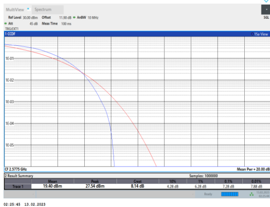
Band38-15MHz-QPSK-37825-75RB#0
