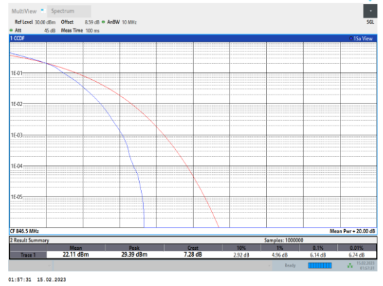
Band5-5MHz-64QAM-20625-25RB#0
