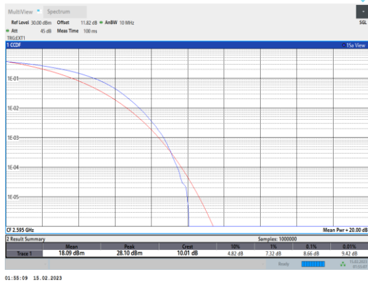
Band38-20MHz-64QAM-38000-100RB#0
