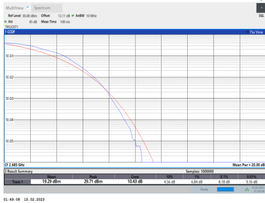
Band41-10MHz-64QAM-41540-50RB#0
