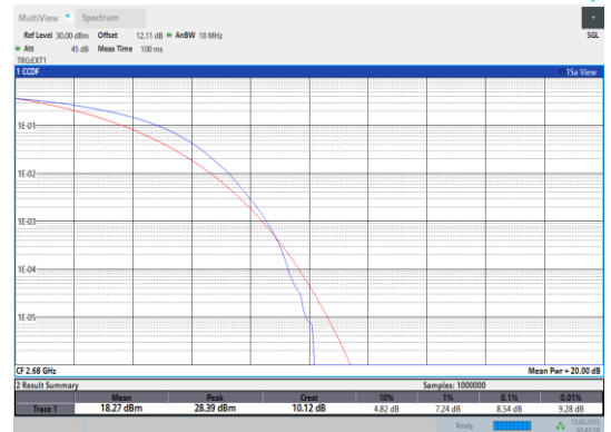
Band41-20MHz-16QAM-41490-100RB#0
