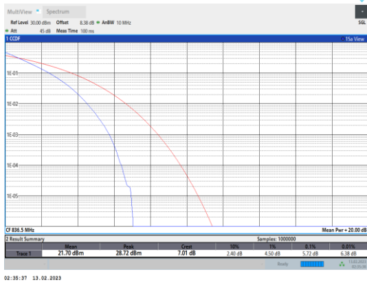
Band5-10MHz-QPSK-20525-50RB#0
