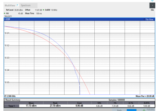
Band41-20MHz-64QAM-39750-100RB#0
