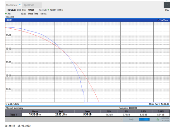
Band41-5MHz-64QAM-41565-25RB#0
