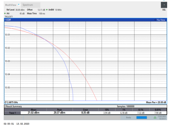
Band41-5MHz-QPSK-41565-25RB#0
