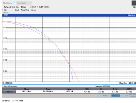
Band38-10MHz-16QAM-37800-50RB#0
