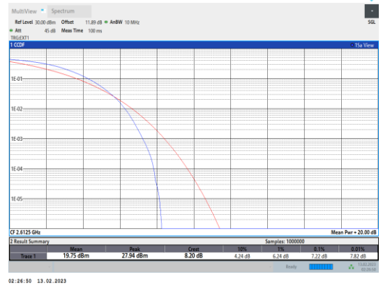
Band38-15MHz-QPSK-38175-75RB#0
