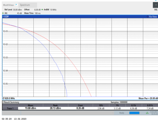
Band5-10MHz-16QAM-20450-50RB#0
