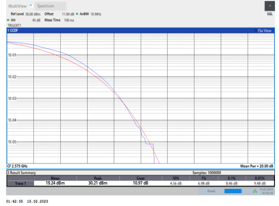
Band38-10MHz-64QAM-37800-50RB#0
