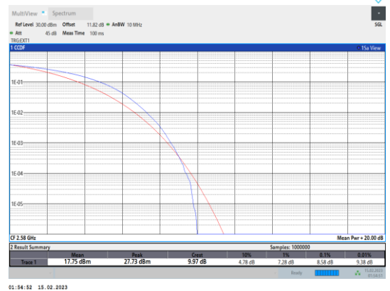
Band38-20MHz-64QAM-37850-100RB#0
