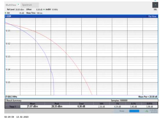
Band5-5MHz-QPSK-20525-25RB#0
