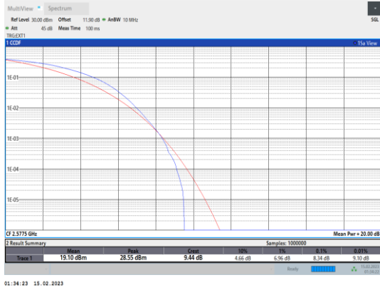
Band38-15MHz-64QAM-37825-75RB#0
