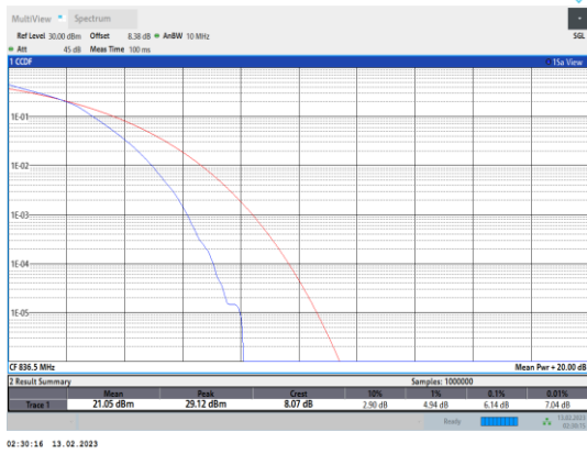
Band5-5MHz-16QAM-20525-25RB#0
