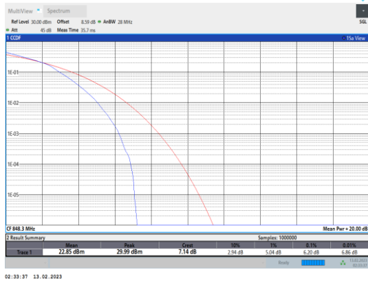
Band5-1.4MHz-16QAM-20643-6RB#0
