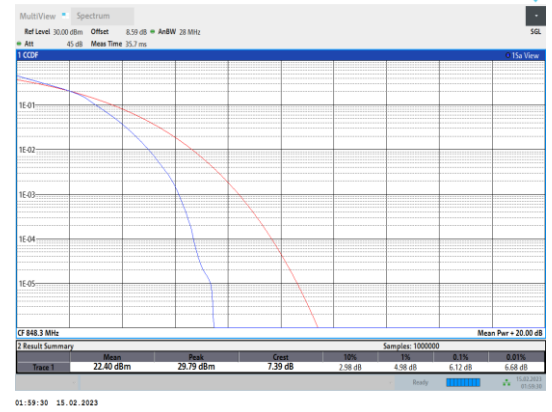
Band5-1.4MHz-64QAM-20643-6RB#0
