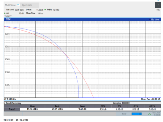
Band38-15MHz-64QAM-38000-75RB#0
