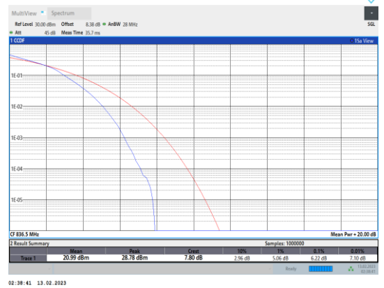
Band5-3MHz-16QAM-20525-15RB#0
