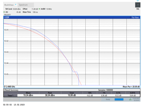
Band41-5MHz-16QAM-39675-25RB#0
