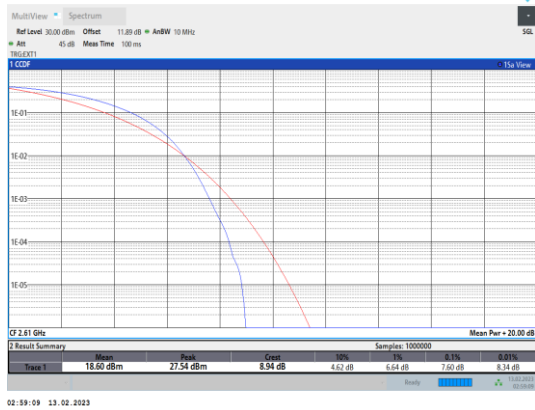
Band38-20MHz-QPSK-38150-100RB#0
