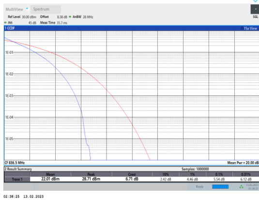
Band5-3MHz-QPSK-20525-15RB#0
