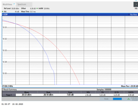
Band5-3MHz-64QAM-20525-15RB#0
