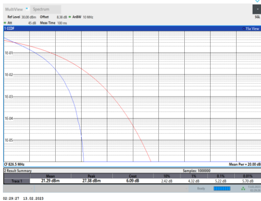
Band5-5MHz-QPSK-20425-25RB#0
