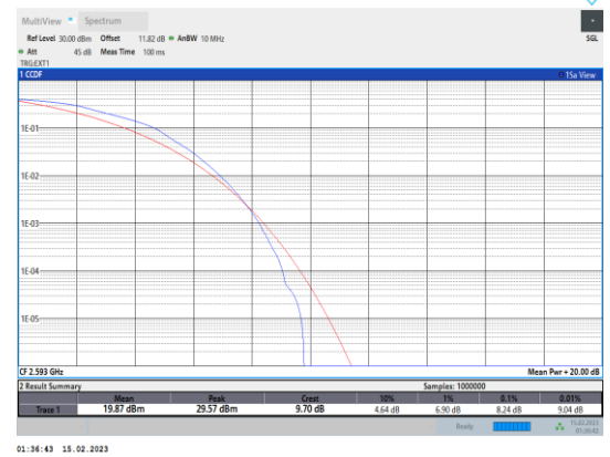
Band41-5MHz-64QAM-40620-25RB#0
