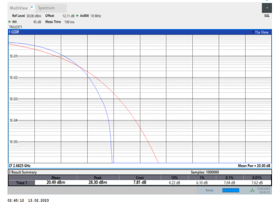
Band41-15MHz-QPSK-41515-75RB#0
