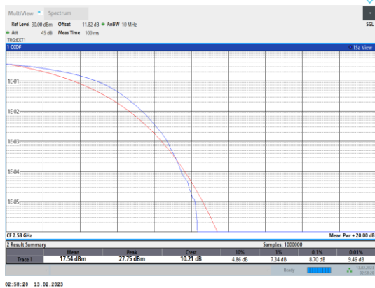
Band38-20MHz-16QAM-37850-100RB#0
