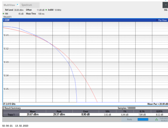
Band38-10MHz-QPSK-38200-50RB#0
