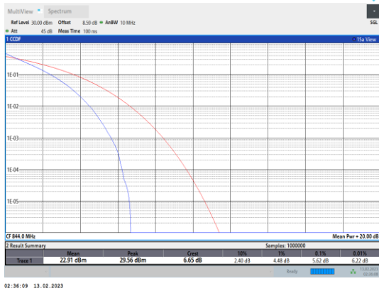
Band5-10MHz-QPSK-20600-50RB#0
