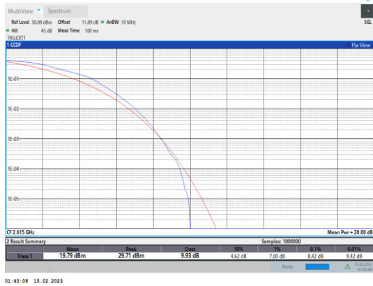
Band38-10MHz-64QAM-38200-50RB#0
