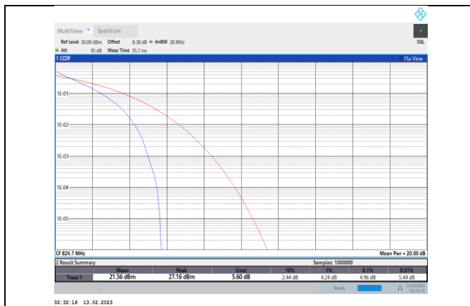
Band5-1.4MHz-QPSK-20407-6RB#0
