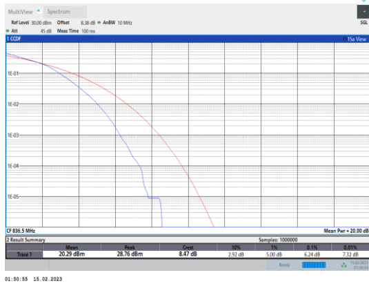
Band5-10MHz-64QAM-20525-50RB#0
