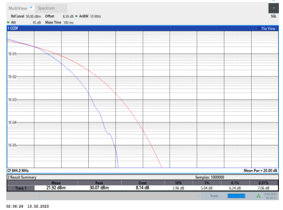
Band5-10MHz-16QAM-20600-50RB#0
