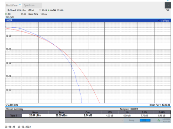
Band38-5MHz-QPSK-38000-25RB#0
