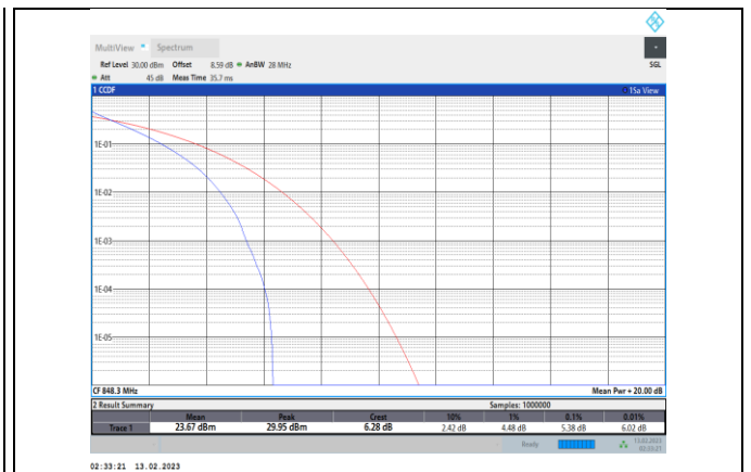
Band5-1.4MHz-QPSK-20643-6RB#0
