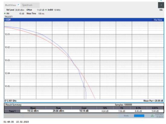
Band41-10MHz-64QAM-39700-50RB#0
