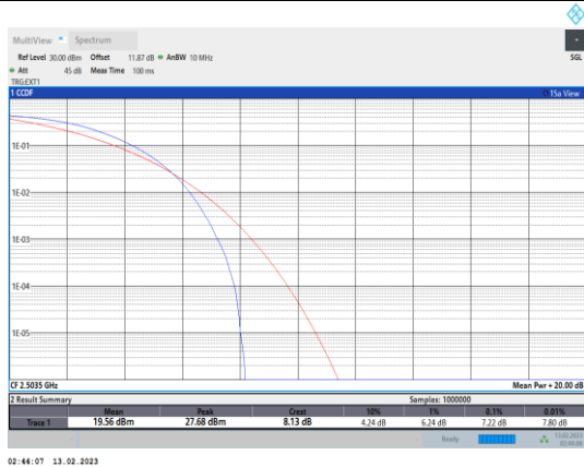
Band41-15MHz-QPSK-39725-75RB#0
