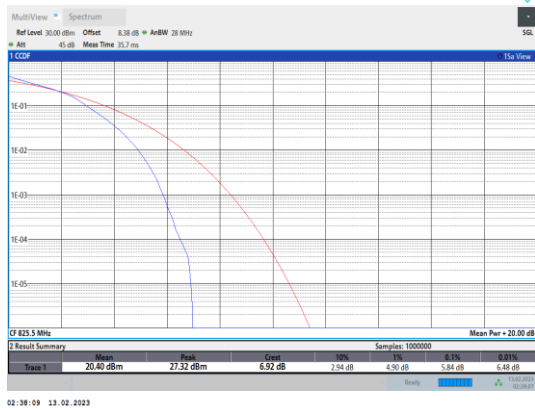
Band5-3MHz-16QAM-20415-15RB#0
