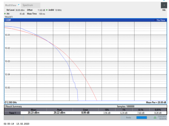
Band41-5MHz-QPSK-40620-25RB#0
