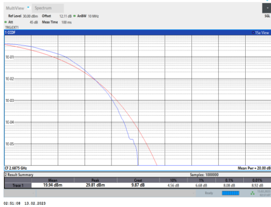
Band41-5MHz-16QAM-41565-25RB#0
