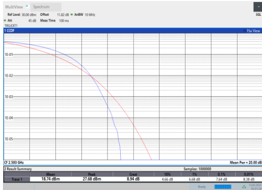
Band41-20MHz-QPSK-40620-100RB#0
