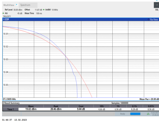
Band41-15MHz-64QAM-39725-75RB#0
