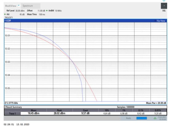
Band38-15MHz-16QAM-37825-75RB#0
