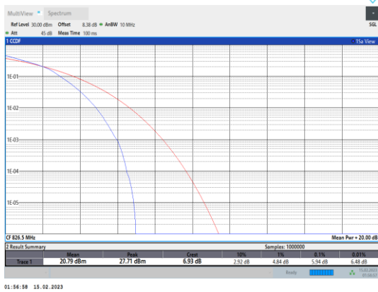
Band5-5MHz-64QAM-20425-25RB#0
