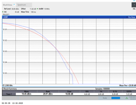
Band41-5MHz-16QAM-40620-25RB#0
