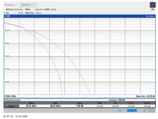
Band5-5MHz-64QAM-20525-25RB#0
