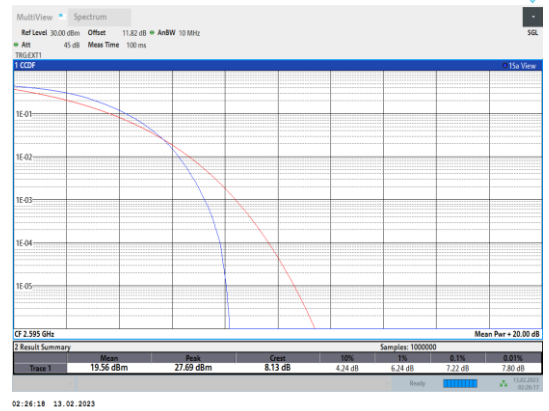
Band38-15MHz-QPSK-38000-75RB#0
