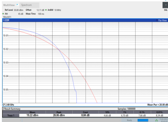
Band41-20MHz-QPSK-41490-100RB#0
