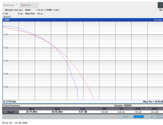
Band38-5MHz-QPSK-37775-25RB#0
