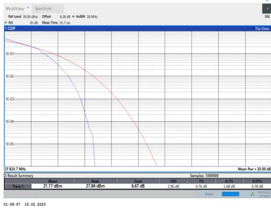
Band5-1.4MHz-64QAM-20407-6RB#0
