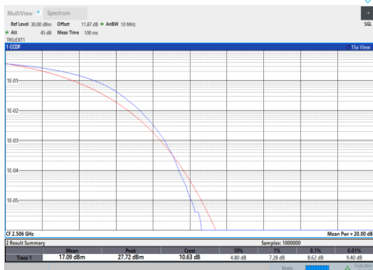
Band41-20MHz-16QAM-39750-100RB#0
