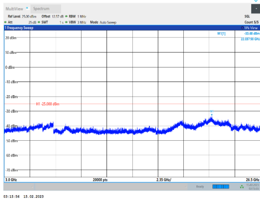
Band38-5MHz-64QAM-38225-1RB#0-Range3:3000~26500MHz
