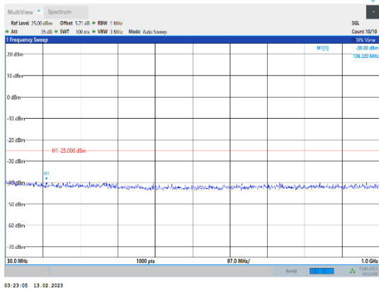
Band38-15MHz-16QAM-38000-1RB#0-Range1:30~1000MHz
