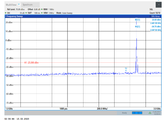
Band41-10MHz-64QAM-41540-1RB#0-Range2:1000~3000MHz
