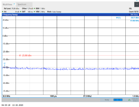
Band41-5MHz-16QAM-40620-1RB#0-Range1:30~1000MHz
