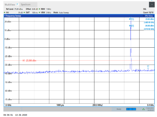
Band41-5MHz-16QAM-41565-1RB#0-Range2:1000~3000MHz
