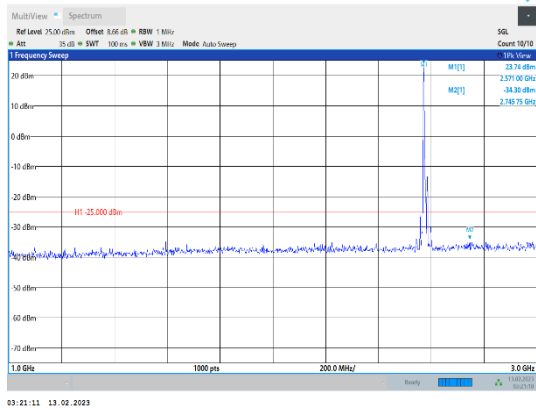
Band38-15MHz-QPSK-37825-1RB#0-Range2:1000~3000MHz
