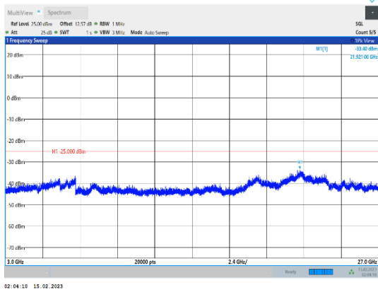
Band41-5MHz-64QAM-41565-1RB#0-Range3:3000~27000MHz
