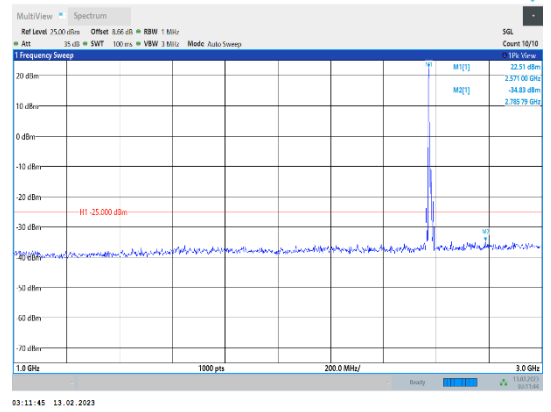
Band38-10MHz-QPSK-37800-1RB#0-Range2:1000~3000MHz
