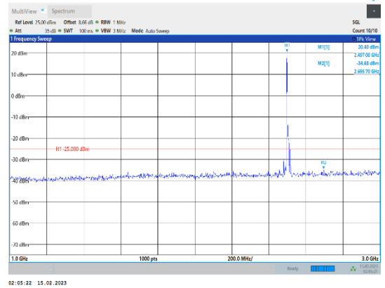
Band41-10MHz-64QAM-39700-1RB#0-Range2:1000~3000MHz
