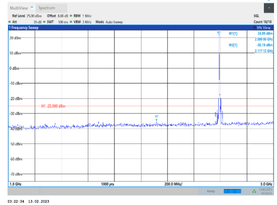
Band38-15MHz-QPSK-38000-1RB#0-Range2:1000~3000MHz
