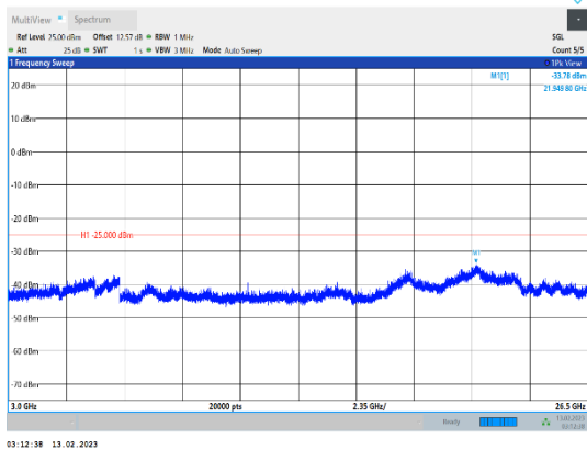
Band38-10MHz-16QAM-37800-1RB#0-Range3:3000~26500MHz
