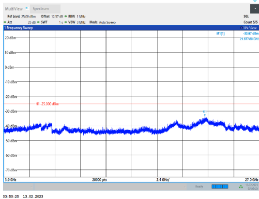
Band41-10MHz-16QAM-39700-1RB#0-Range3:3000~27000MHz
