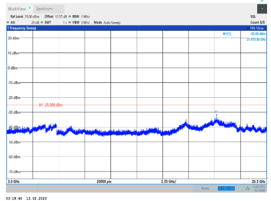
Band38-20MHz-16QAM-38000-1RB#0-Range3:3000~26500MHz
