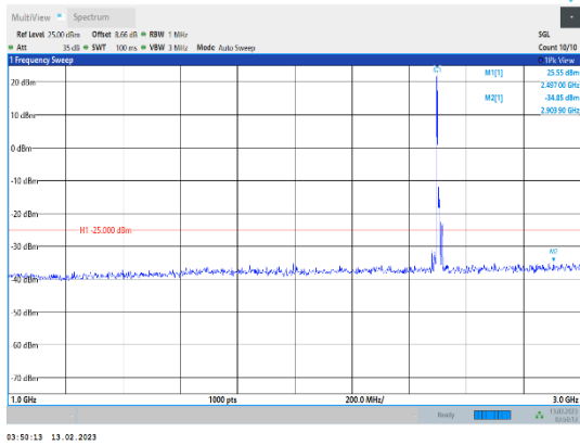
Band41-10MHz-16QAM-39700-1RB#0-Range2:1000~3000MHz
