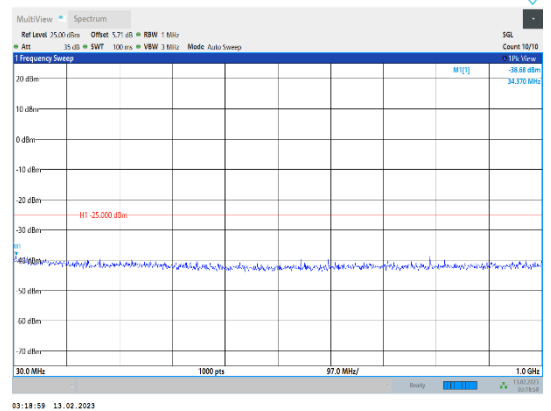
Band38-20MHz-QPSK-38150-1RB#0-Range1:30~1000MHz
