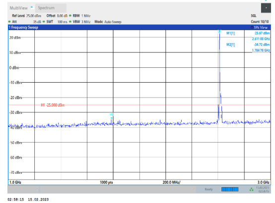
Band38-10MHz-64QAM-38200-1RB#0-Range2:1000~3000MHz
