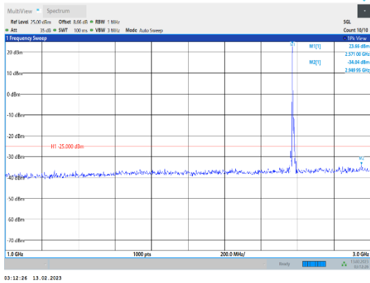
Band38-10MHz-16QAM-37800-1RB#0-Range2:1000~3000MHz
