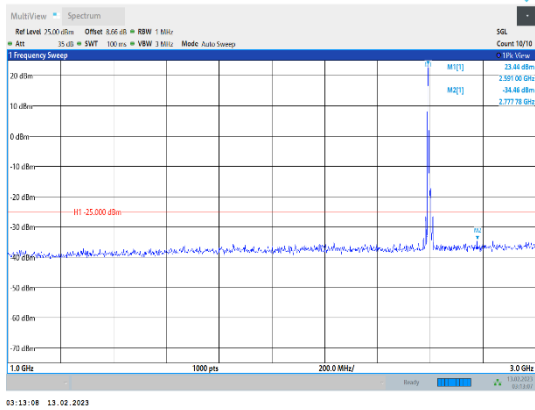
Band38-10MHz-QPSK-38000-1RB#0-Range2:1000~3000MHz
