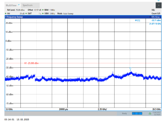
Band38-10MHz-16QAM-38000-1RB#0-Range3:3000~26500MHz
