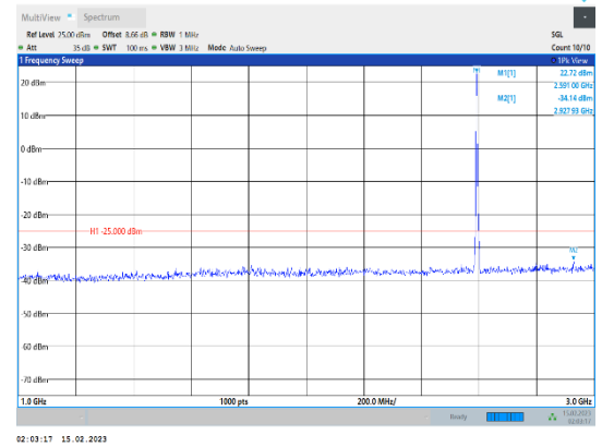
Band41-5MHz-64QAM-40620-1RB#0-Range2:1000~3000MHz
