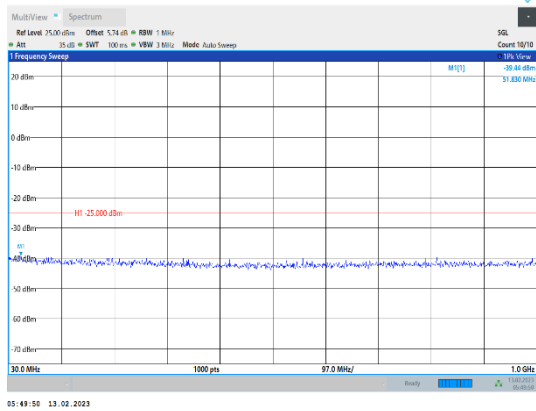
Band41-15MHz-QPSK-41515-1RB#0-Range1:30~1000MHz
