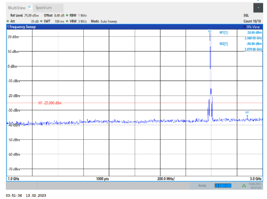
Band41-10MHz-16QAM-40620-1RB#0-Range2:1000~3000MHz
