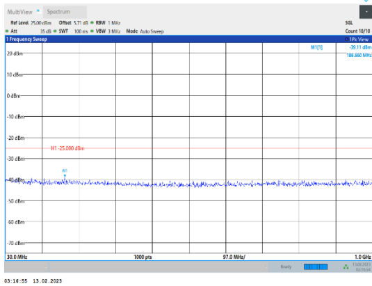
Band38-20MHz-16QAM-37850-1RB#0-Range1:30~1000MHz
