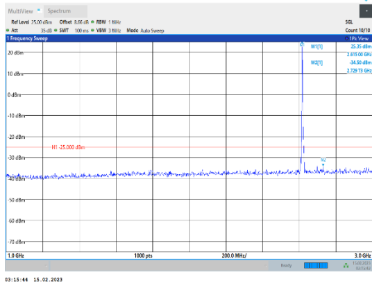
Band38-5MHz-64QAM-38225-1RB#0-Range2:1000~3000MHz
