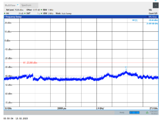
Band41-15MHz-16QAM-41515-1RB#0-Range3:3000~27000MHz
