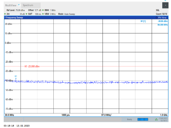
Band38-20MHz-16QAM-38000-1RB#0-Range1:30~1000MHz
