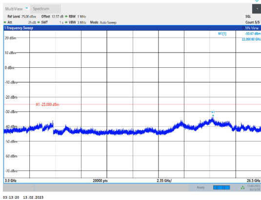
Band38-10MHz-QPSK-38000-1RB#0-Range3:3000~26500MHz
