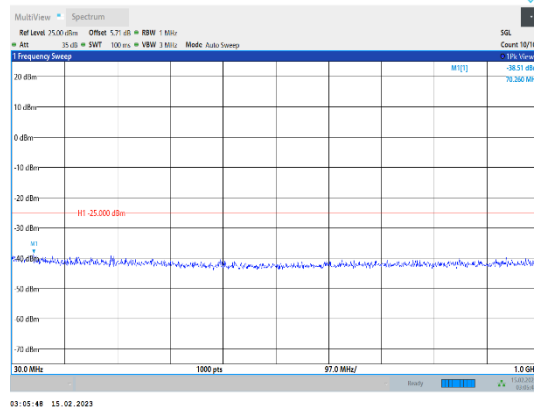
Band38-20MHz-64QAM-38150-1RB#0-Range1:30~1000MHz
