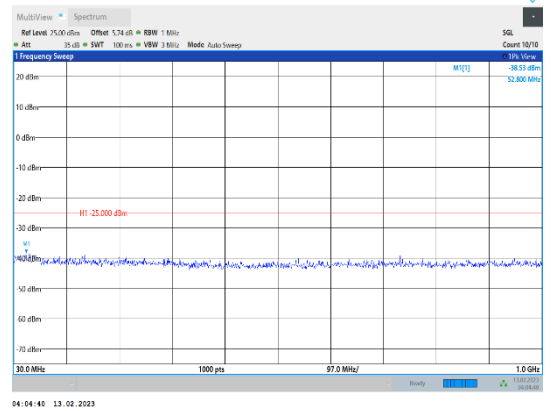
Band41-5MHz-16QAM-41565-1RB#0-Range1:30~1000MHz
