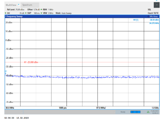
Band41-10MHz-64QAM-41540-1RB#0-Range1:30~1000MHz
