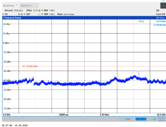
Band38-10MHz-64QAM-38000-1RB#0-Range3:3000~26500MHz
