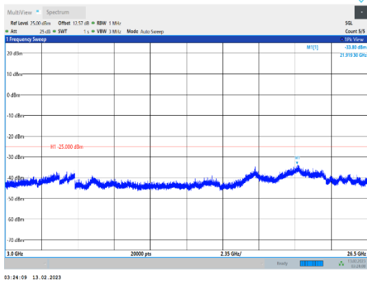
Band38-15MHz-QPSK-38175-1RB#0-Range3:3000~26500MHz
