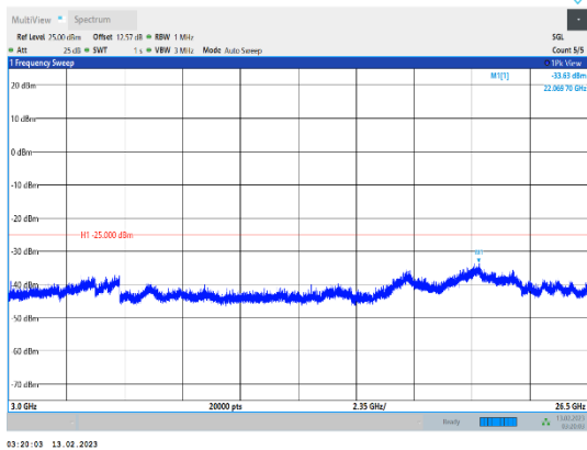
Band38-20MHz-16QAM-38150-1RB#0-Range3:3000~26500MHz
