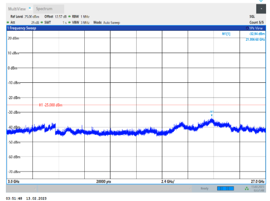
Band41-10MHz-16QAM-40620-1RB#0-Range3:3000~27000MHz
