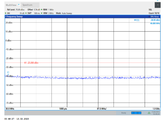
Band41-15MHz-QPSK-40620-1RB#0-Range1:30~1000MHz
