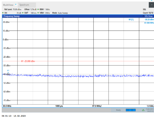
Band41-5MHz-QPSK-39675-1RB#0-Range1:30~1000MHz
