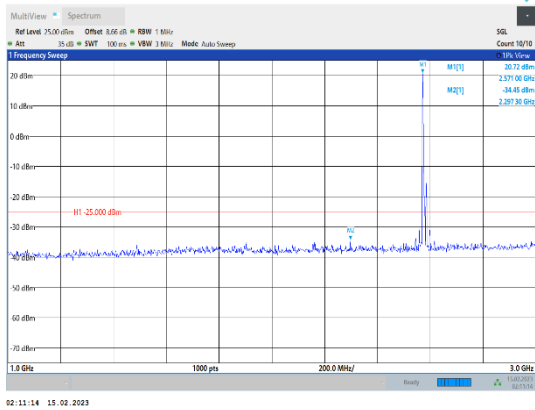
Band38-15MHz-64QAM-37825-1RB#0-Range2:1000~3000MHz
