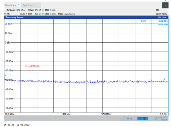
Band41-5MHz-QPSK-40620-1RB#0-Range1:30~1000MHz
