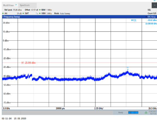
Band38-15MHz-64QAM-37825-1RB#0-Range3:3000~26500MHz
