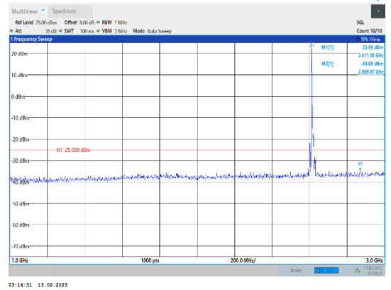
Band38-10MHz-QPSK-38200-1RB#0-Range2:1000~3000MHz
