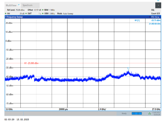
Band41-5MHz-64QAM-40620-1RB#0-Range3:3000~27000MHz
