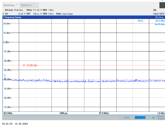
Band38-15MHz-QPSK-37825-1RB#0-Range1:30~1000MHz
