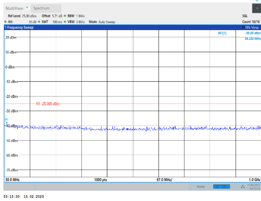
Band38-5MHz-64QAM-38225-1RB#0-Range1:30~1000MHz
