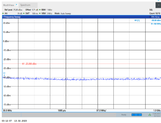
Band38-10MHz-QPSK-38000-1RB#0-Range1:30~1000MHz
