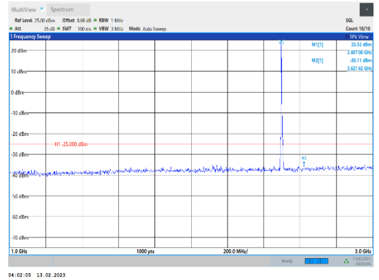
Band41-5MHz-16QAM-39675-1RB#0-Range2:1000~3000MHz
