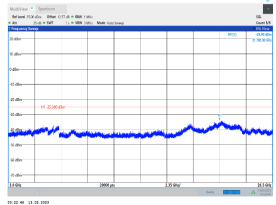
Band38-15MHz-QPSK-38000-1RB#0-Range3:3000~26500MHz
