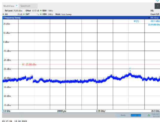
Band38-20MHz-QPSK-38000-1RB#0-Range3:3000~26500MHz
