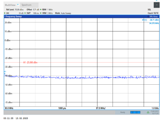
Band38-10MHz-QPSK-37800-1RB#0-Range1:30~1000MHz
