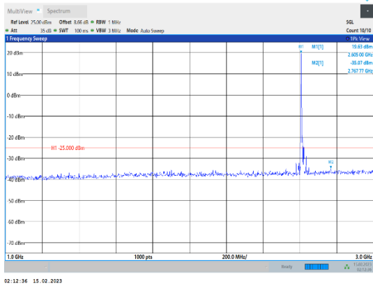
Band38-15MHz-64QAM-38175-1RB#0-Range2:1000~3000MHz
