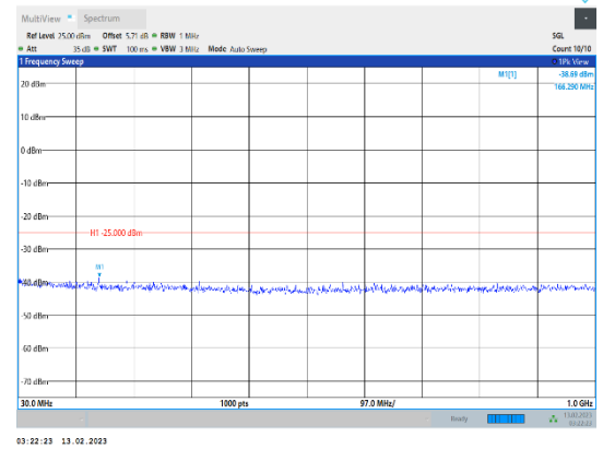
Band38-15MHz-QPSK-38000-1RB#0-Range1:30~1000MHz
