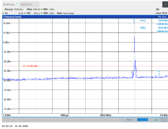
Band38-15MHz-16QAM-38000-1RB#0-Range2:1000~3000MHz
