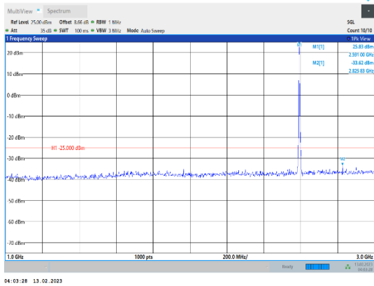
Band41-5MHz-16QAM-40620-1RB#0-Range2:1000~3000MHz
