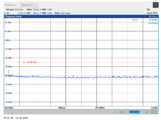
Band41-5MHz-16QAM-39675-1RB#0-Range1:30~1000MHz
