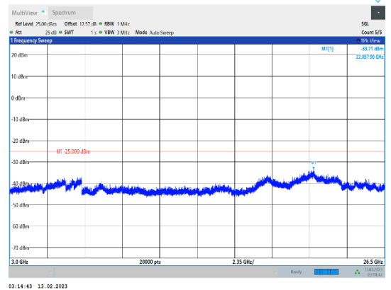
Band38-10MHz-QPSK-38200-1RB#0-Range3:3000~26500MHz
