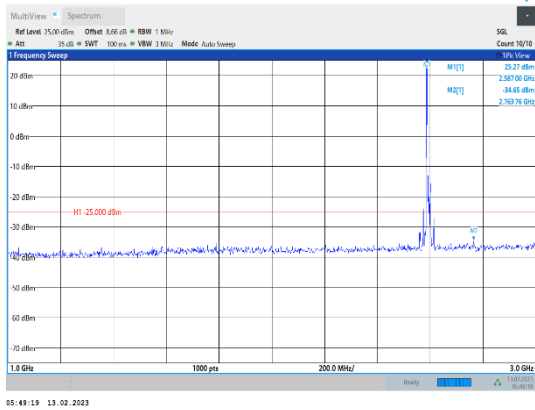
Band41-15MHz-16QAM-40620-1RB#0-Range2:1000~3000MHz
