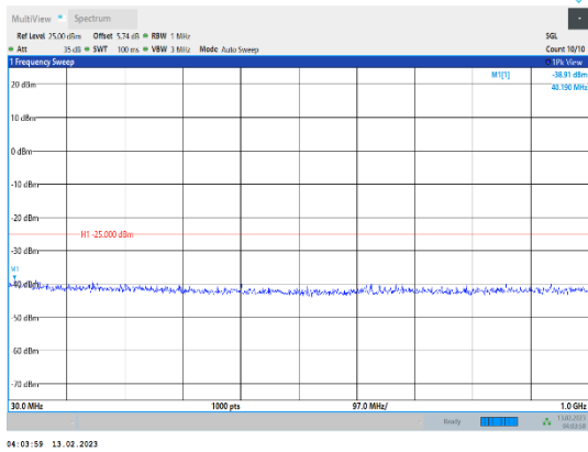
Band41-5MHz-QPSK-41565-1RB#0-Range1:30~1000MHz
