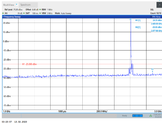
Band38-15MHz-QPSK-38175-1RB#0-Range2:1000~3000MHz
