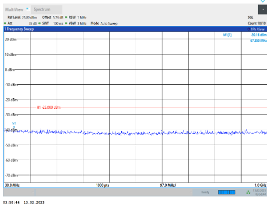
Band41-10MHz-QPSK-40620-1RB#0-Range1:30~1000MHz
