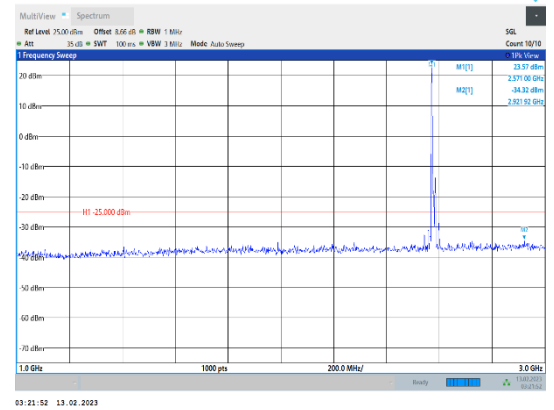
Band38-15MHz-16QAM-37825-1RB#0-Range2:1000~3000MHz
