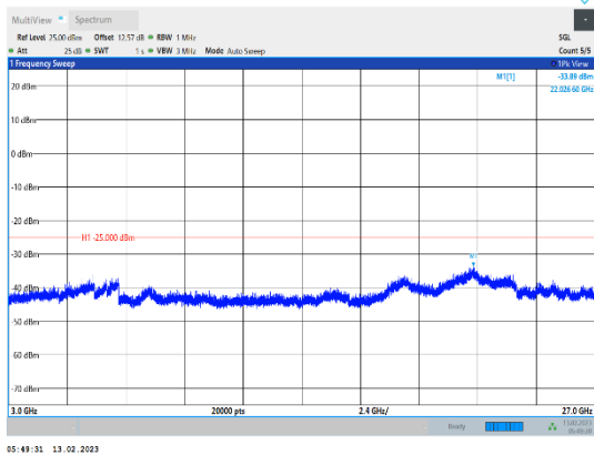
Band41-15MHz-16QAM-40620-1RB#0-Range3:3000~27000MHz
