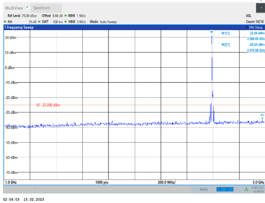
Band41-10MHz-64QAM-40620-1RB#0-Range2:1000~3000MHz
