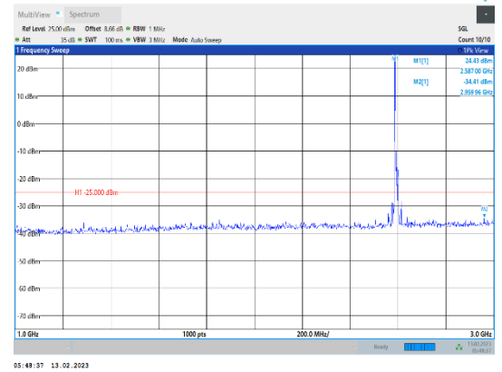
Band41-15MHz-QPSK-40620-1RB#0-Range2:1000~3000MHz
