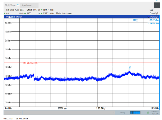
Band38-15MHz-64QAM-38000-1RB#0-Range3:3000~26500MHz
