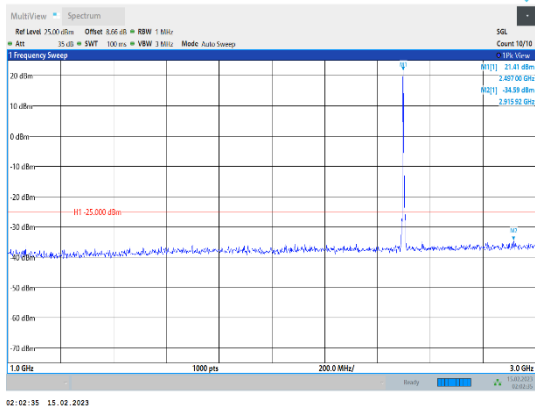
Band41-5MHz-64QAM-39675-1RB#0-Range2:1000~3000MHz
