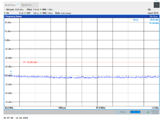
Band41-15MHz-16QAM-39725-1RB#0-Range1:30~1000MHz
