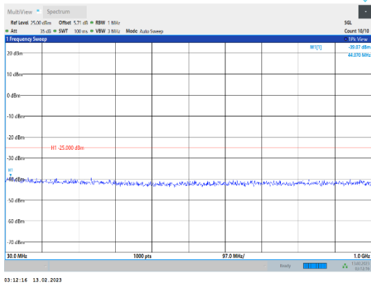
Band38-10MHz-16QAM-37800-1RB#0-Range1:30~1000MHz
