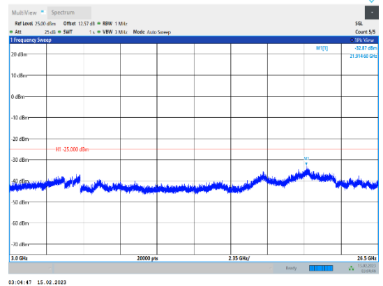
Band38-20MHz-64QAM-37850-1RB#0-Range3:3000~26500MHz
