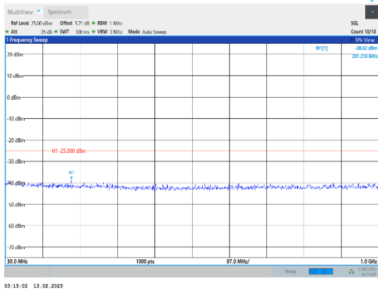
Band38-10MHz-16QAM-38200-1RB#0-Range1:30~1000MHz
