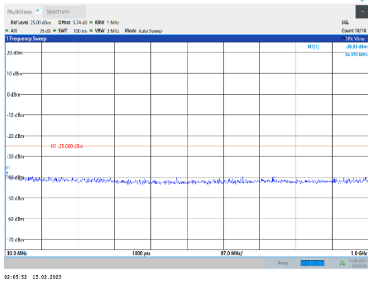
Band41-10MHz-64QAM-40620-1RB#0-Range1:30~1000MHz
