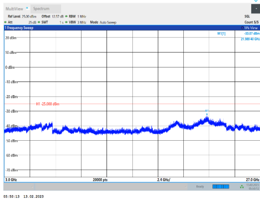
Band41-15MHz-QPSK-41515-1RB#0-Range3:3000~27000MHz
