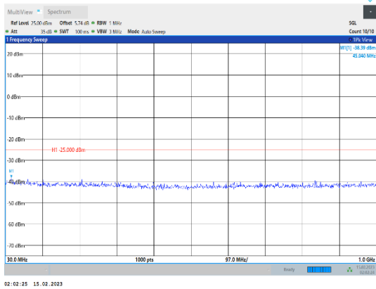
Band41-5MHz-64QAM-39675-1RB#0-Range1:30~1000MHz
