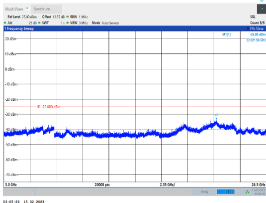
Band38-20MHz-64QAM-38000-1RB#0-Range3:3000~26500MHz
