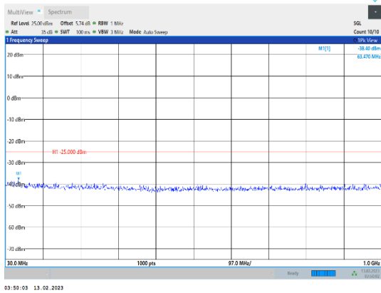
Band41-10MHz-16QAM-39700-1RB#0-Range1:30~1000MHz
