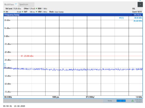
Band41-15MHz-16QAM-41515-1RB#0-Range1:30~1000MHz
