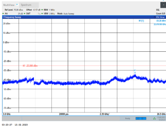
Band38-15MHz-16QAM-38000-1RB#0-Range3:3000~26500MHz
