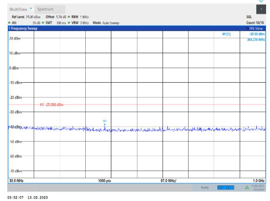
Band41-10MHz-QPSK-41540-1RB#0-Range1:30~1000MHz
