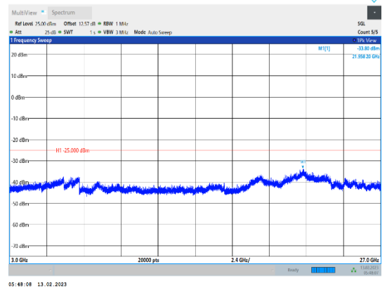
Band41-15MHz-16QAM-39725-1RB#0-Range3:3000~27000MHz
