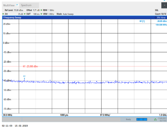
Band38-15MHz-64QAM-37825-1RB#0-Range1:30~1000MHz
