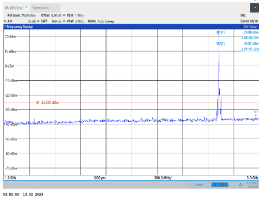
Band41-10MHz-16QAM-41540-1RB#0-Range2:1000~3000MHz
