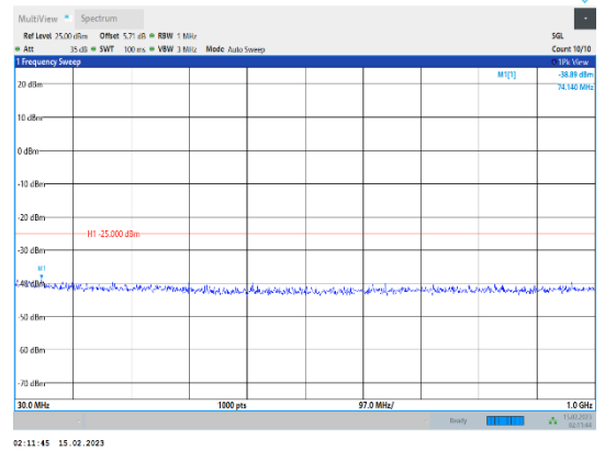
Band38-15MHz-64QAM-38000-1RB#0-Range1:30~1000MHz
