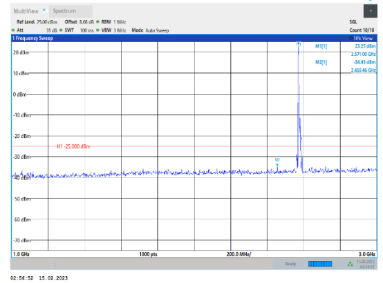
Band38-10MHz-64QAM-37800-1RB#0-Range2:1000~3000MHz
