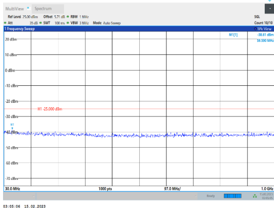
Band38-20MHz-64QAM-38000-1RB#0-Range1:30~1000MHz
