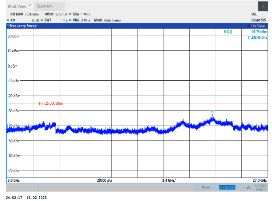
Band41-5MHz-16QAM-39675-1RB#0-Range3:3000~27000MHz
