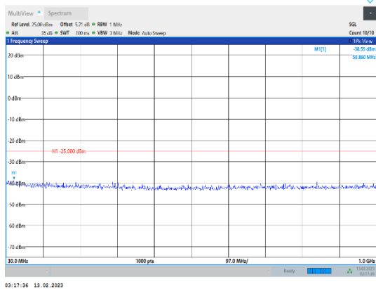
Band38-20MHz-QPSK-38000-1RB#0-Range1:30~1000MHz
