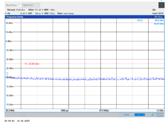
Band38-10MHz-64QAM-37800-1RB#0-Range1:30~1000MHz
