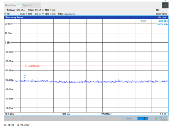
Band41-10MHz-16QAM-40620-1RB#0-Range1:30~1000MHz
