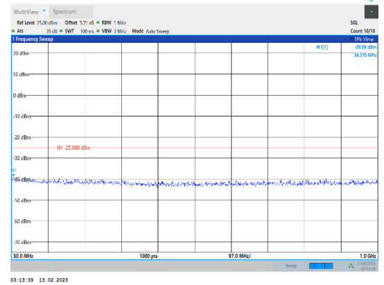
Band38-10MHz-16QAM-38000-1RB#0-Range1:30~1000MHz
