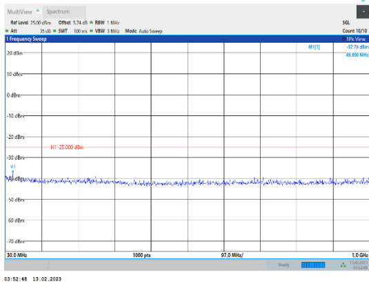
Band41-10MHz-16QAM-41540-1RB#0-Range1:30~1000MHz
