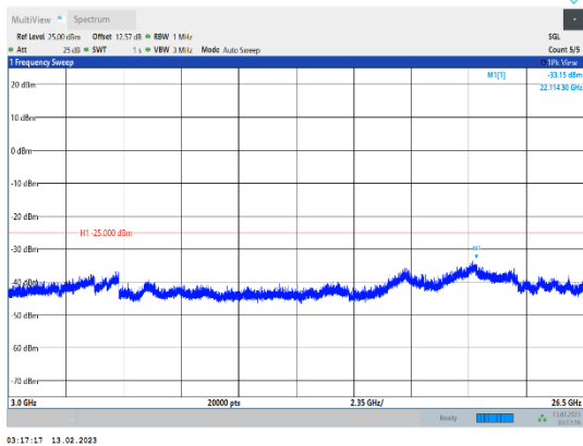
Band38-20MHz-16QAM-37850-1RB#0-Range3:3000~26500MHz
