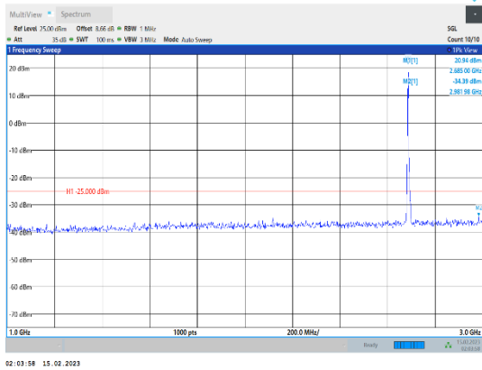
Band41-5MHz-64QAM-41565-1RB#0-Range2:1000~3000MHz
