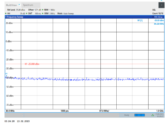
Band38-15MHz-16QAM-38175-1RB#0-Range1:30~1000MHz
