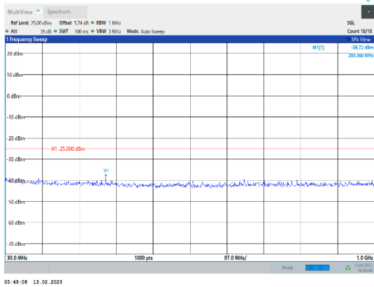
Band41-15MHz-16QAM-40620-1RB#0-Range1:30~1000MHz
