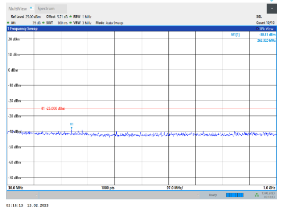
Band38-20MHz-QPSK-37850-1RB#0-Range1:30~1000MHz
