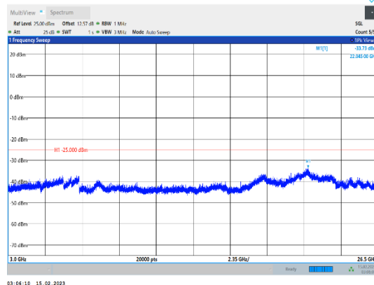
Band38-20MHz-64QAM-38150-1RB#0-Range3:3000~26500MHz
