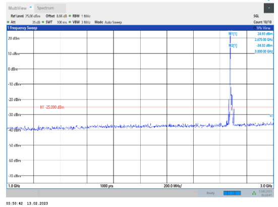
Band41-15MHz-16QAM-41515-1RB#0-Range2:1000~3000MHz
