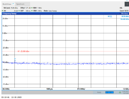
Band38-20MHz-16QAM-38150-1RB#0-Range1:30~1000MHz
