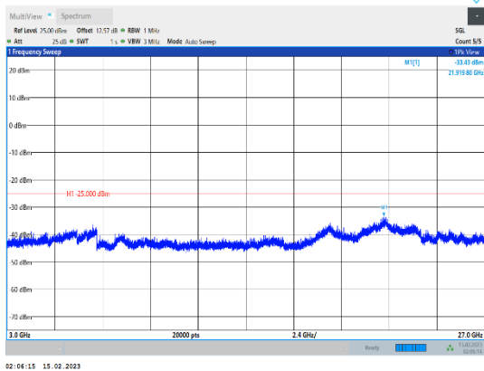
Band41-10MHz-64QAM-40620-1RB#0-Range3:3000~27000MHz
