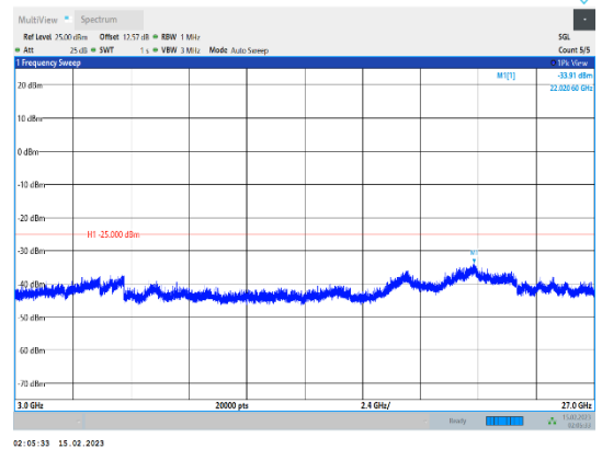
Band41-10MHz-64QAM-39700-1RB#0-Range3:3000~27000MHz
