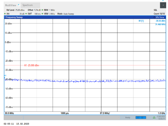
Band41-10MHz-64QAM-39700-1RB#0-Range1:30~1000MHz
