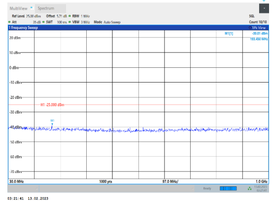
Band38-15MHz-16QAM-37825-1RB#0-Range1:30~1000MHz
