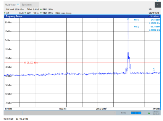
Band38-20MHz-16QAM-38000-1RB#0-Range2:1000~3000MHz
