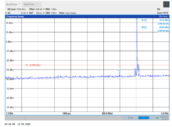
Band38-15MHz-16QAM-38175-1RB#0-Range2:1000~3000MHz
