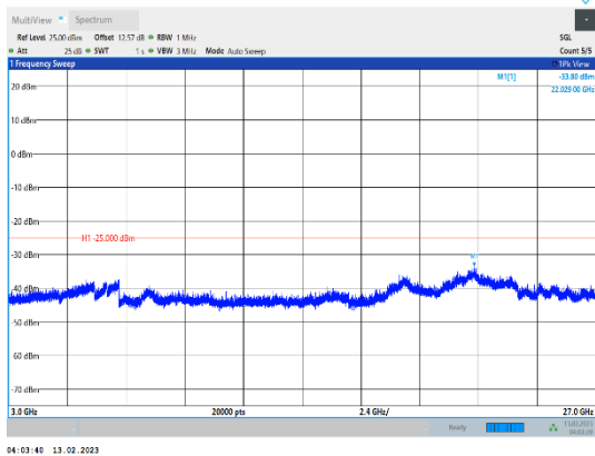
Band41-5MHz-16QAM-40620-1RB#0-Range3:3000~27000MHz
