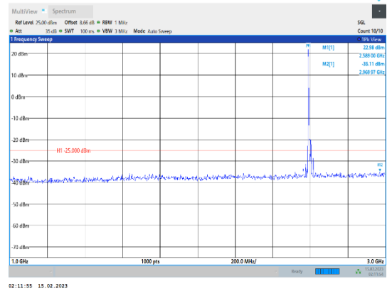
Band38-15MHz-64QAM-38000-1RB#0-Range2:1000~3000MHz
