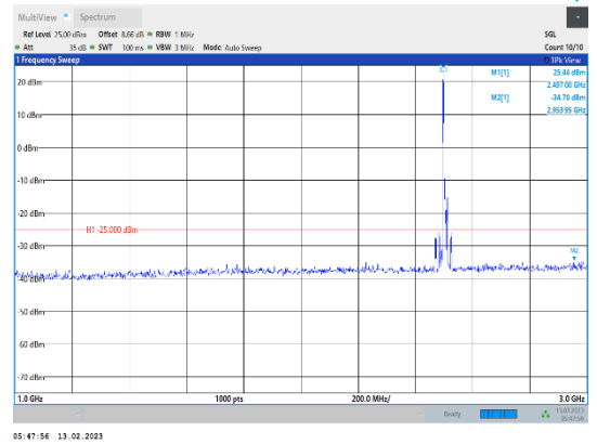
Band41-15MHz-16QAM-39725-1RB#0-Range2:1000~3000MHz
