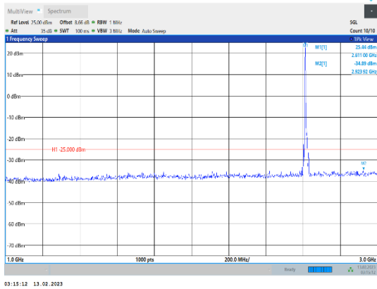
Band38-10MHz-16QAM-38200-1RB#0-Range2:1000~3000MHz
