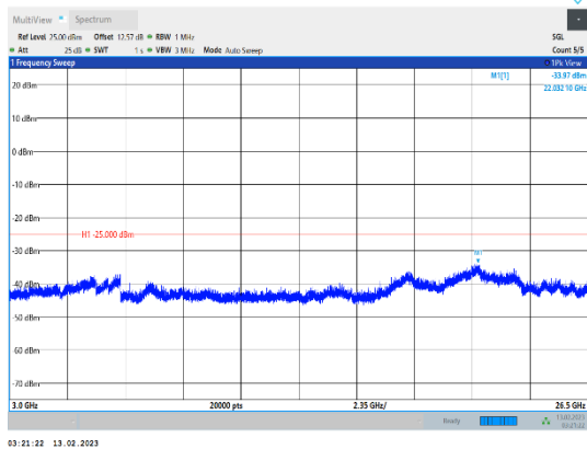
Band38-15MHz-QPSK-37825-1RB#0-Range3:3000~26500MHz
