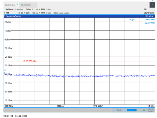
Band38-20MHz-64QAM-37850-1RB#0-Range1:30~1000MHz
