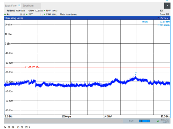
Band41-5MHz-QPSK-40620-1RB#0-Range3:3000~27000MHz
