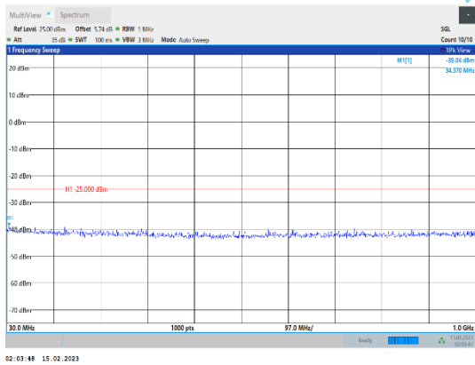
Band41-5MHz-64QAM-41565-1RB#0-Range1:30~1000MHz
