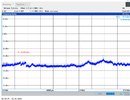
Band41-5MHz-64QAM-39675-1RB#0-Range3:3000~27000MHz
