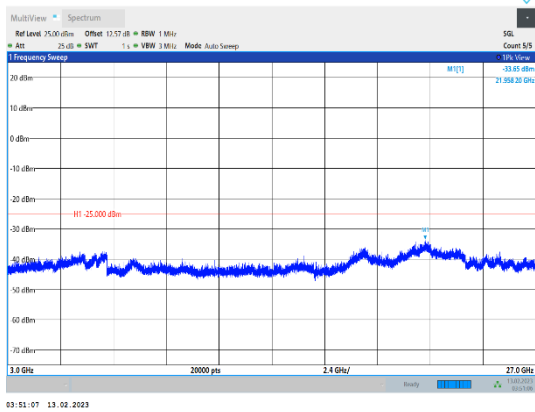
Band41-10MHz-QPSK-40620-1RB#0-Range3:3000~27000MHz
