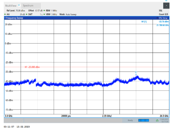
Band38-10MHz-QPSK-37800-1RB#0-Range3:3000~26500MHz
