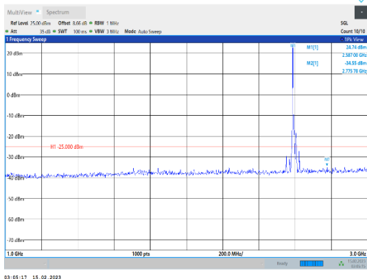
Band38-20MHz-64QAM-38000-1RB#0-Range2:1000~3000MHz
