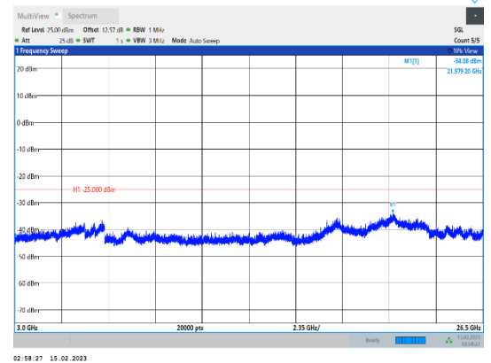
Band38-10MHz-64QAM-38200-1RB#0-Range3:3000~26500MHz
