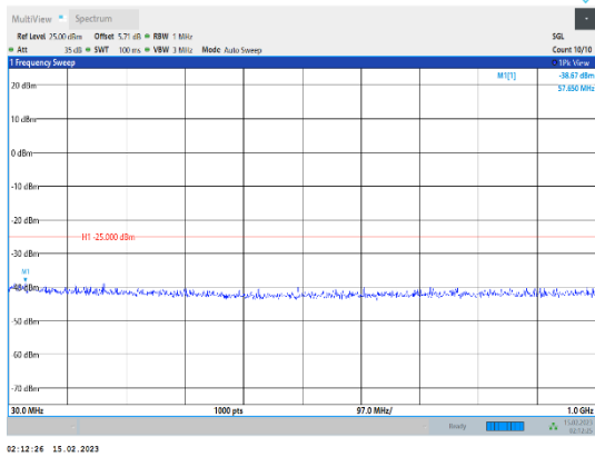
Band38-15MHz-64QAM-38175-1RB#0-Range1:30~1000MHz
