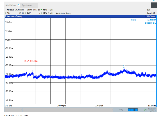
Band41-10MHz-64QAM-41540-1RB#0-Range3:3000~27000MHz
