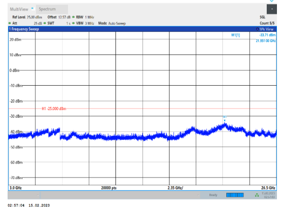
Band38-10MHz-64QAM-37800-1RB#0-Range3:3000~26500MHz
