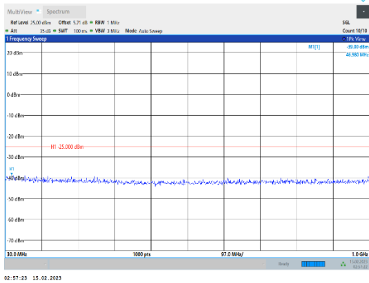
Band38-10MHz-64QAM-38000-1RB#0-Range1:30~1000MHz
