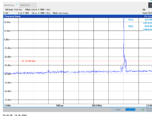
Band38-20MHz-64QAM-38150-1RB#0-Range2:1000~3000MHz
