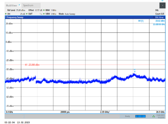
Band38-15MHz-16QAM-37825-1RB#0-Range3:3000~26500MHz
