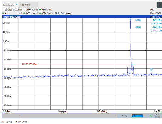
Band38-20MHz-16QAM-38150-1RB#0-Range2:1000~3000MHz
