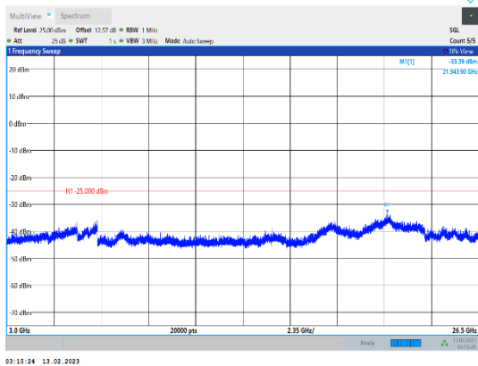
Band38-10MHz-16QAM-38200-1RB#0-Range3:3000~26500MHz
