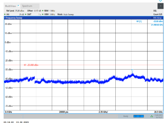
Band38-20MHz-QPSK-38150-1RB#0-Range3:3000~26500MHz
