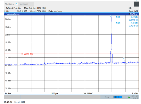
Band38-10MHz-16QAM-38000-1RB#0-Range2:1000~3000MHz
