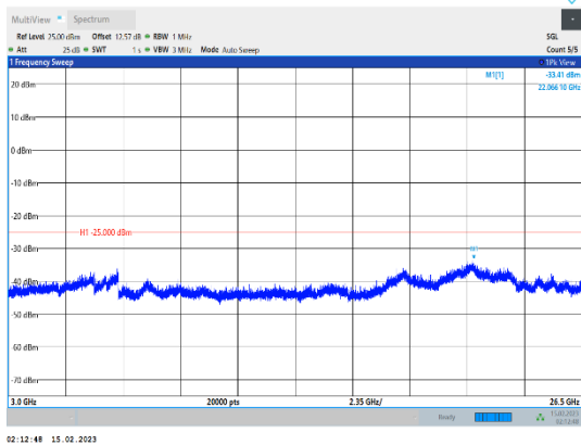
Band38-15MHz-64QAM-38175-1RB#0-Range3:3000~26500MHz
