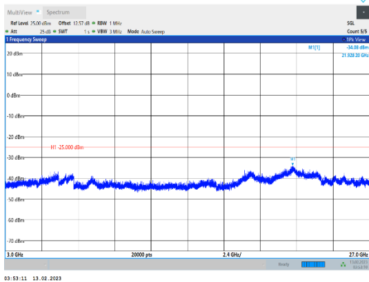
Band41-10MHz-16QAM-41540-1RB#0-Range3:3000~27000MHz
