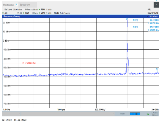
Band38-10MHz-64QAM-38000-1RB#0-Range2:1000~3000MHz
