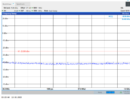
Band38-15MHz-QPSK-38175-1RB#0-Range1:30~1000MHz
