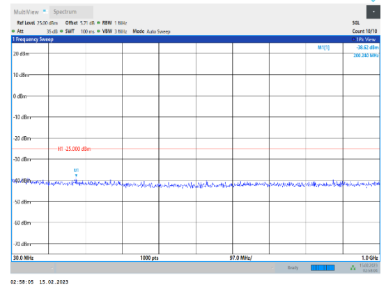
Band38-10MHz-64QAM-38200-1RB#0-Range1:30~1000MHz
