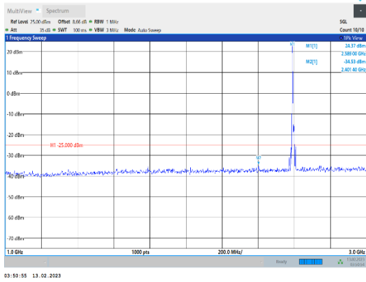
Band41-10MHz-QPSK-40620-1RB#0-Range2:1000~3000MHz
