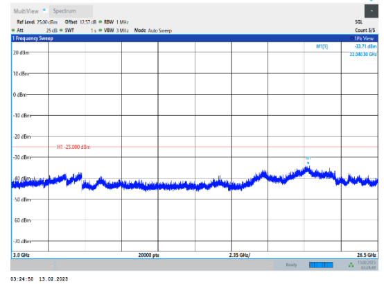
Band38-15MHz-16QAM-38175-1RB#0-Range3:3000~26500MHz
