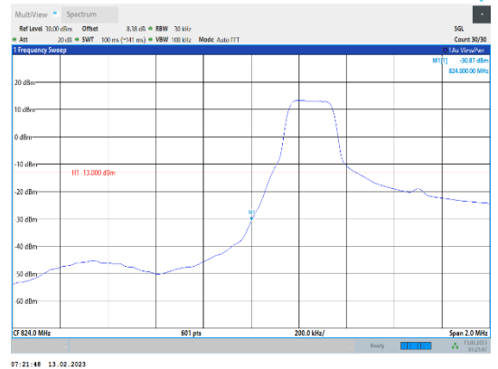
Band5-1.4MHz-16QAM-20407-1RB#0
