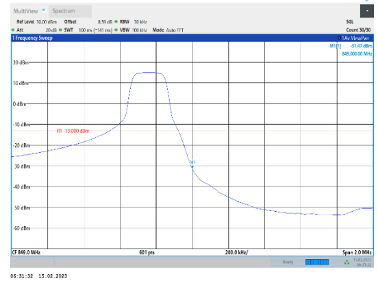
Band5-3MHz-64QAM-20635-1RB#14
