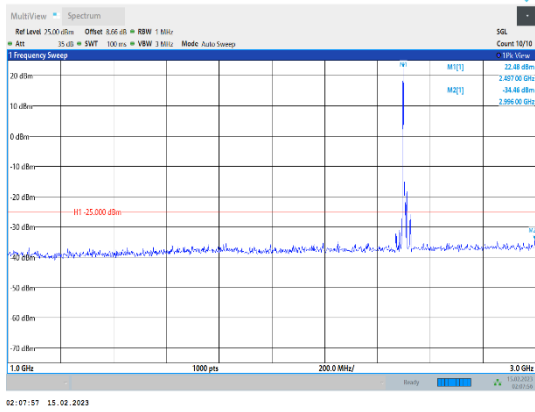
Band41-15MHz-64QAM-39725-1RB#0-Range2:1000~3000MHz
