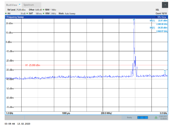
Band41-20MHz-16QAM-40620-1RB#0-Range2:1000~3000MHz
