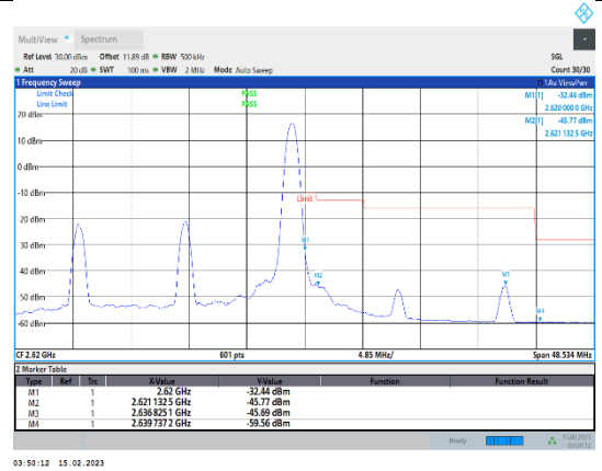
Band38-20MHz-64QAM-38150-1RB#99
