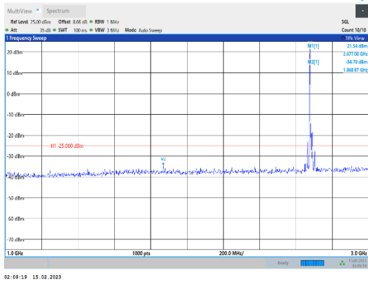
Band41-15MHz-64QAM-41515-1RB#0-Range2:1000~3000MHz
