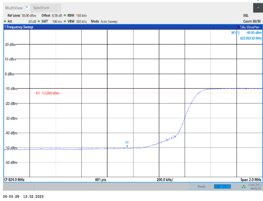
Band5-10MHz-QPSK-20450-50RB#0
