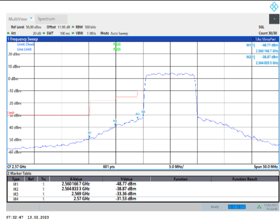
Band38-10MHz-16QAM-37800-50RB#0
