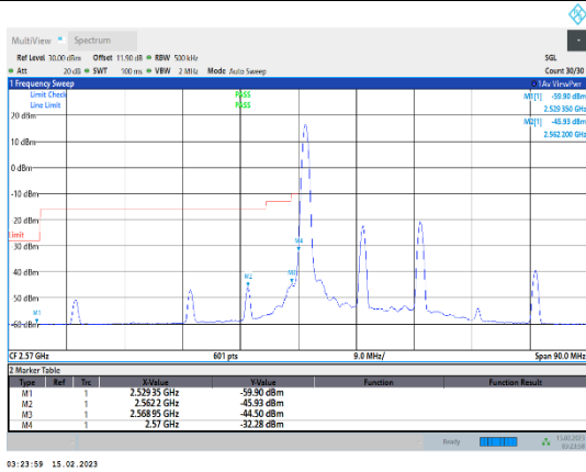
Band38-20MHz-64QAM-37850-1RB#0
