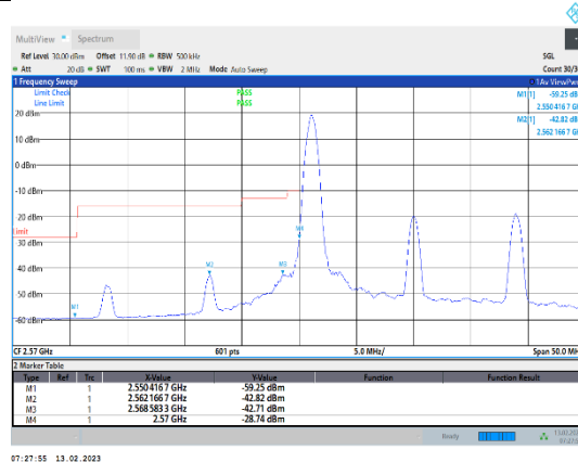
Band38-20MHz-16QAM-37850-1RB#0
