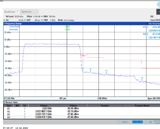
Band38-15MHz-QPSK-38175-75RB#0
