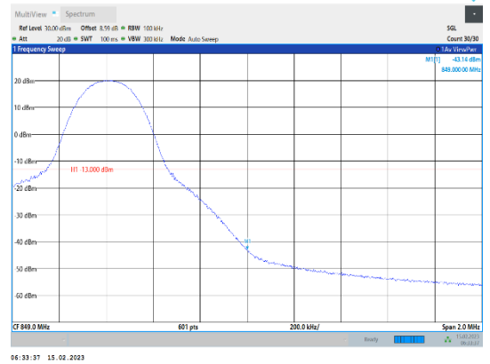
Band5-10MHz-64QAM-20600-1RB#49
