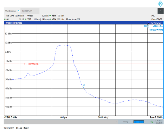
Band5-1.4MHz-64QAM-20643-1RB#5
