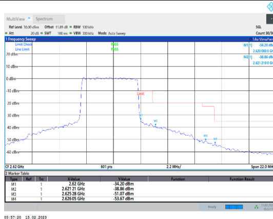
Band38-5MHz-64QAM-38225-25RB#0
