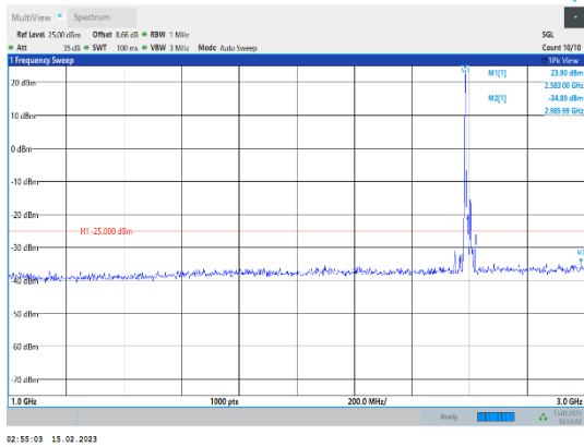
Band41-20MHz-64QAM-40620-1RB#0-Range2:1000~3000MHz
