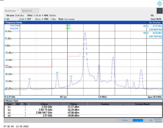
Band38-10MHz-16QAM-37800-1RB#0
