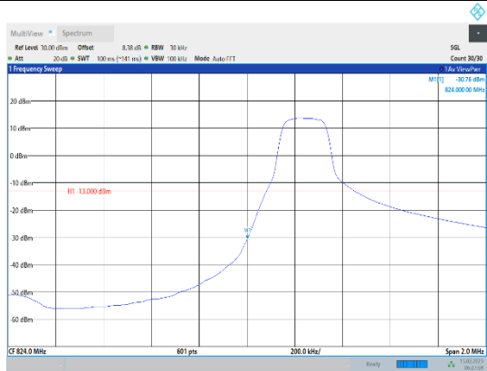
Band5-3MHz-64QAM-20415-1RB#0
