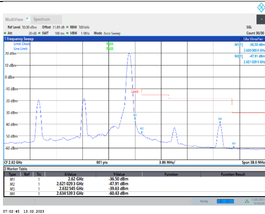
Band38-15MHz-16QAM-38175-1RB#74
