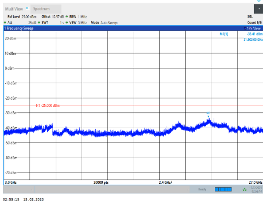
Band41-20MHz-64QAM-40620-1RB#0-Range3:3000~27000MHz
