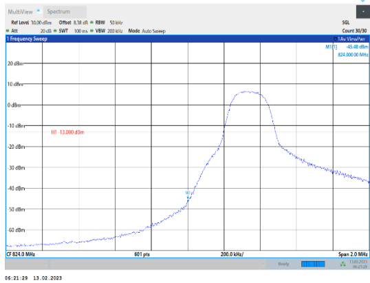
Band5-5MHz-QPSK-20425-1RB#0
