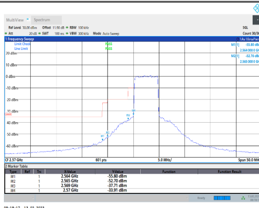
Band38-5MHz-16QAM-37775-25RB#0
