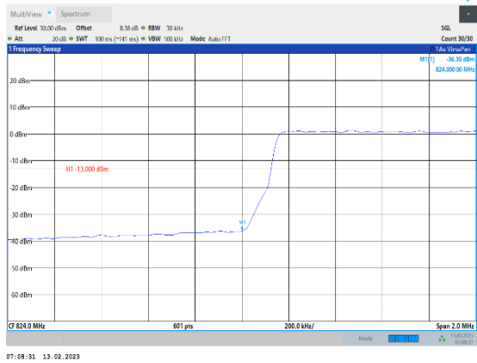
Band5-3MHz-QPSK-20415-15RB#0
