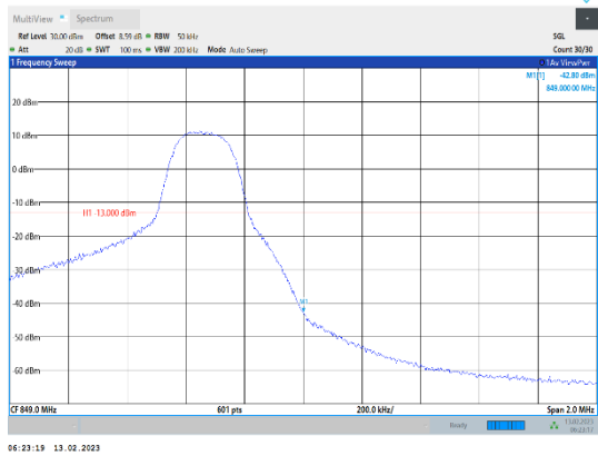
Band5-5MHz-QPSK-20625-1RB#24
