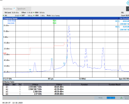
Band38-15MHz-16QAM-37825-1RB#0
