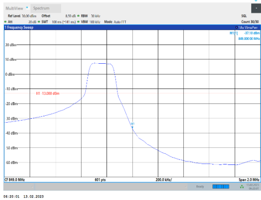
Band5-3MHz-16QAM-20635-1RB#14
