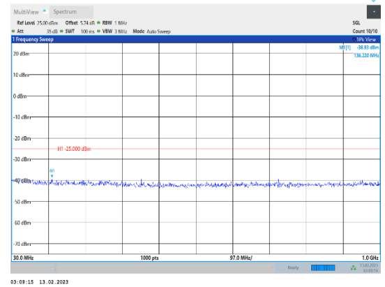
Band41-20MHz-QPSK-41490-1RB#0-Range1:30~1000MHz
