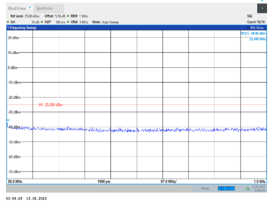
Band41-20MHz-QPSK-39750-1RB#0-Range1:30~1000MHz
