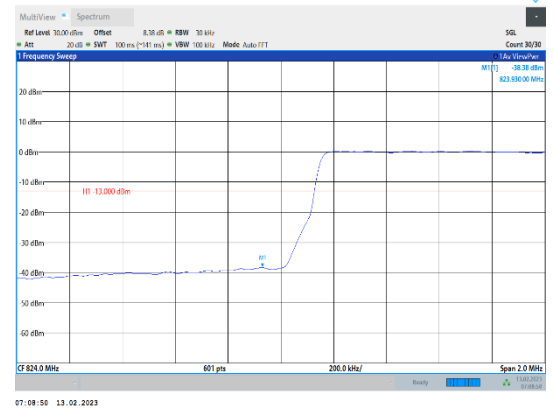
Band5-3MHz-16QAM-20415-15RB#0
