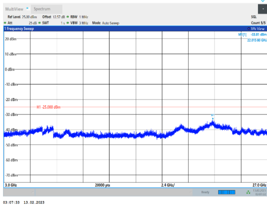
Band41-20MHz-16QAM-39750-1RB#0-Range3:3000~27000MHz
