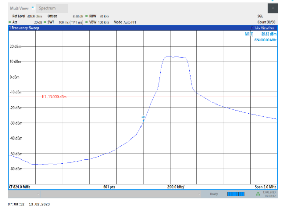
Band5-3MHz-16QAM-20415-1RB#0
