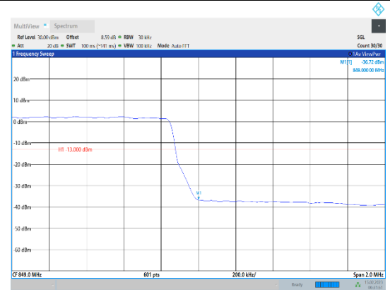
Band5-3MHz-64QAM-20635-15RB#0
