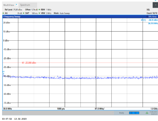
Band41-20MHz-QPSK-40620-1RB#0-Range1:30~1000MHz
