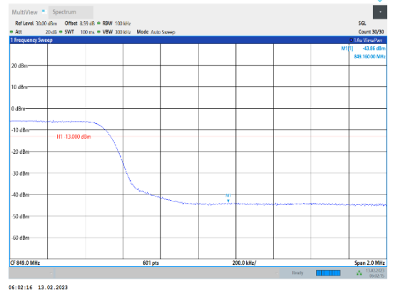
Band5-10MHz-QPSK-20600-50RB#0
