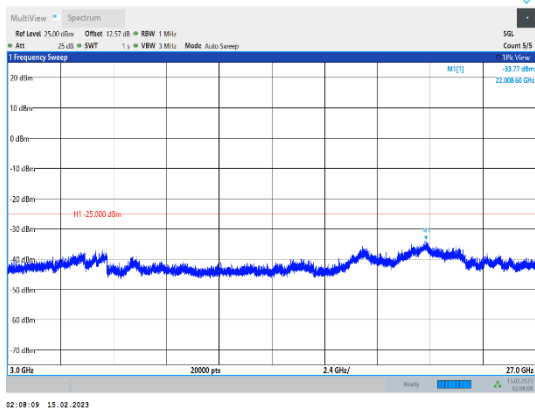
Band41-15MHz-64QAM-39725-1RB#0-Range3:3000~27000MHz
