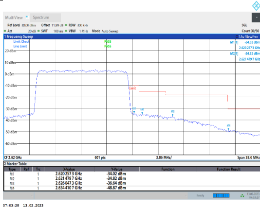
Band38-15MHz-16QAM-38175-75RB#0
