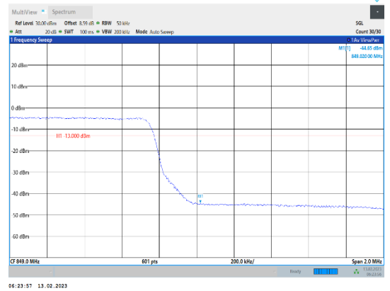
Band5-5MHz-QPSK-20625-25RB#0
