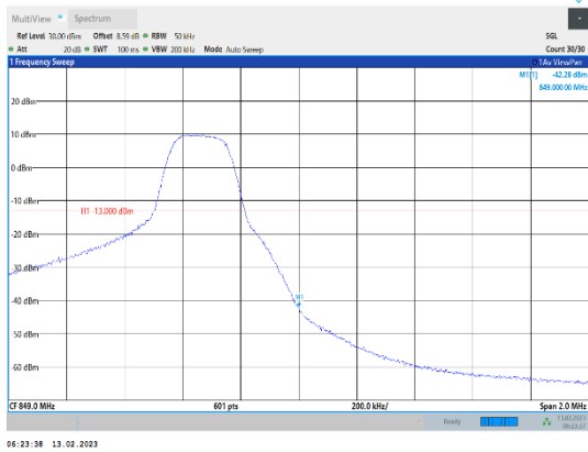
Band5-5MHz-16QAM-20625-1RB#24
