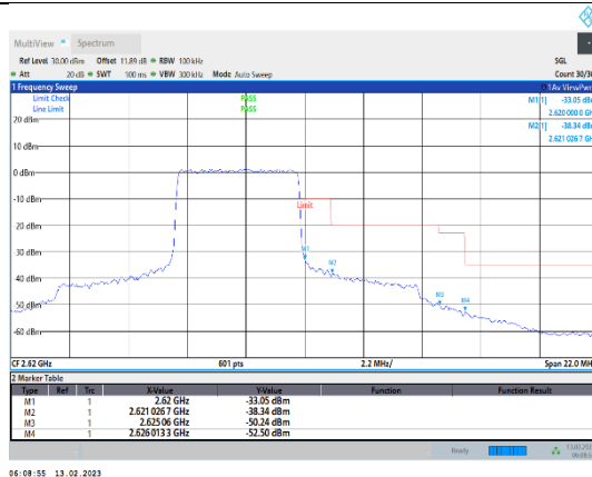
Band38-5MHz-QPSK-38225-25RB#0
