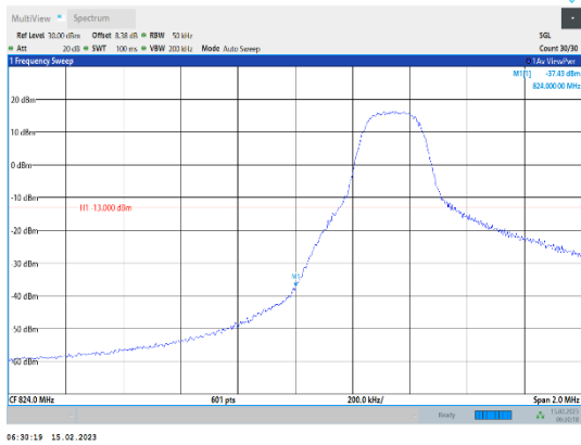
Band5-5MHz-64QAM-20425-1RB#0
