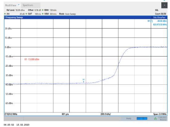
Band5-10MHz-64QAM-20450-50RB#0
