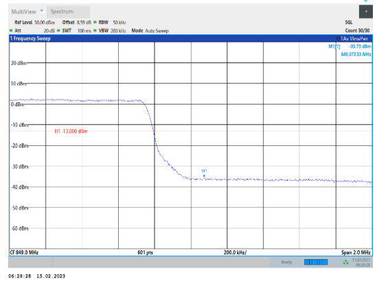
Band5-5MHz-64QAM-20625-25RB#0
