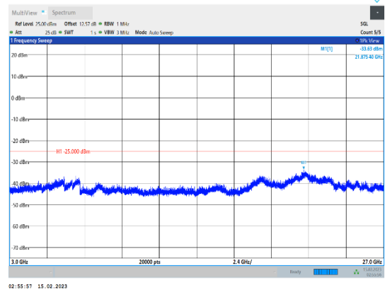
Band41-20MHz-64QAM-41490-1RB#0-Range3:3000~27000MHz
