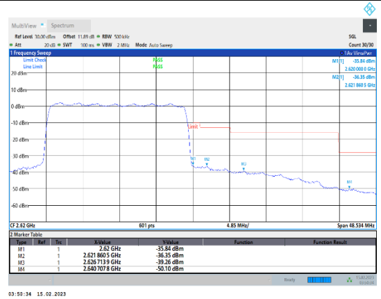
Band38-20MHz-64QAM-38150-100RB#0
