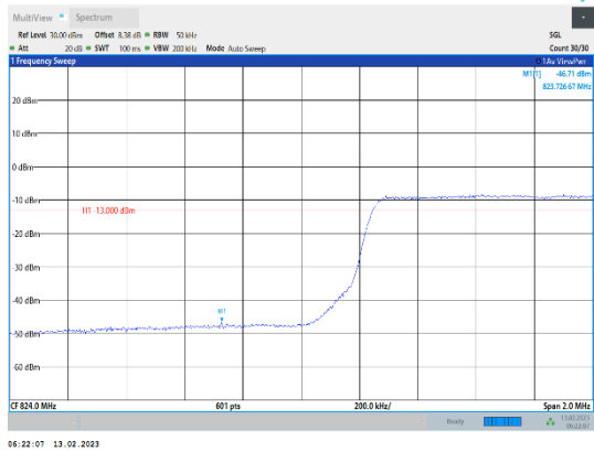
Band5-5MHz-QPSK-20425-25RB#0
