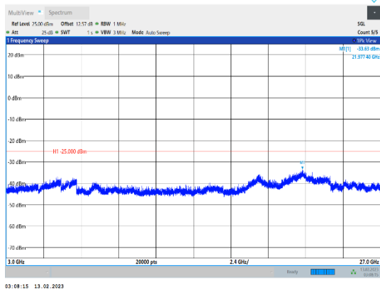
Band41-20MHz-QPSK-40620-1RB#0-Range3:3000~27000MHz
