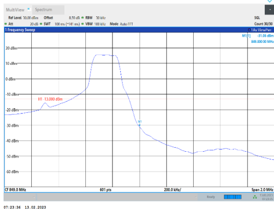
Band5-1.4MHz-16QAM-20643-1RB#5
