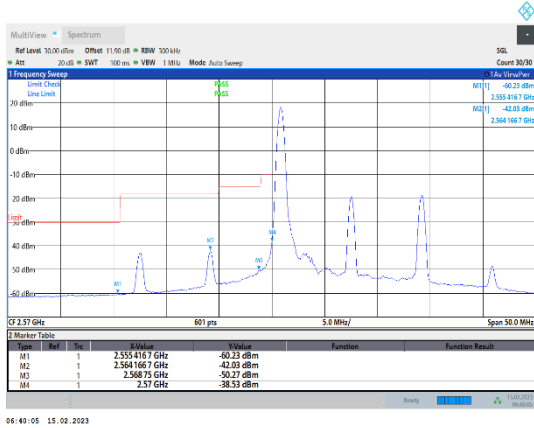
Band38-15MHz-64QAM-37825-1RB#0
