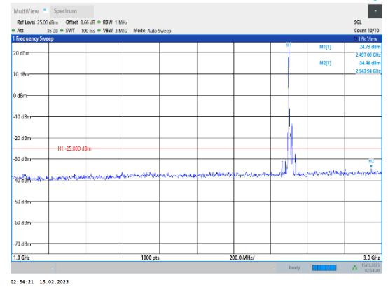
Band41-20MHz-64QAM-39750-1RB#0-Range2:1000~3000MHz
