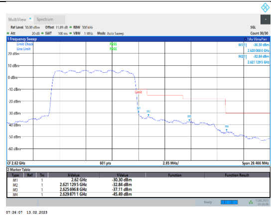
Band38-10MHz-QPSK-38200-50RB#0
