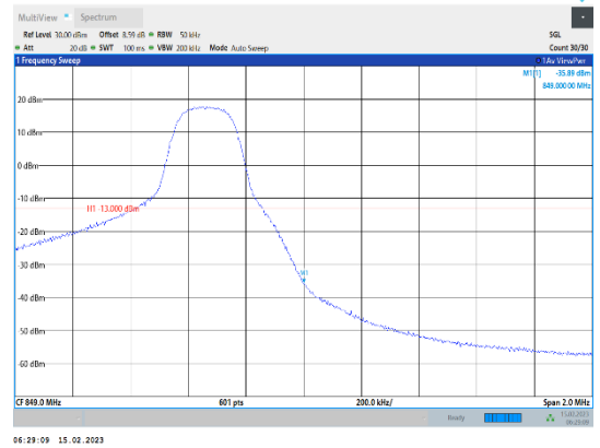
Band5-5MHz-64QAM-20625-1RB#24
