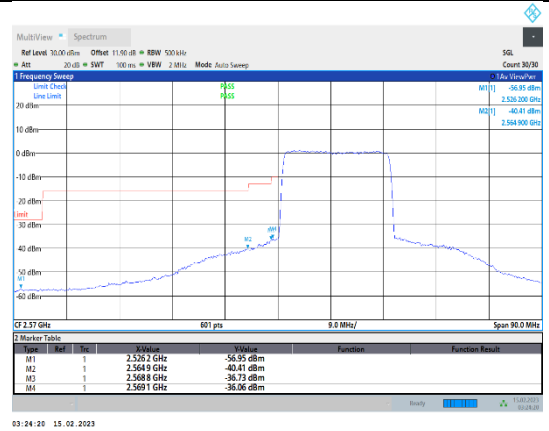
Band38-20MHz-64QAM-37850-100RB#0
