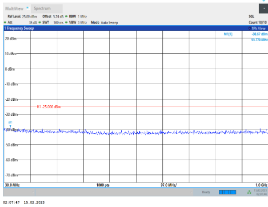
Band41-15MHz-64QAM-39725-1RB#0-Range1:30~1000MHz
