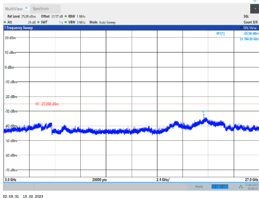
Band41-15MHz-64QAM-41515-1RB#0-Range3:3000~27000MHz
