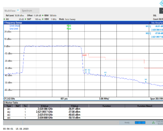
Band38-15MHz-64QAM-38175-75RB#0
