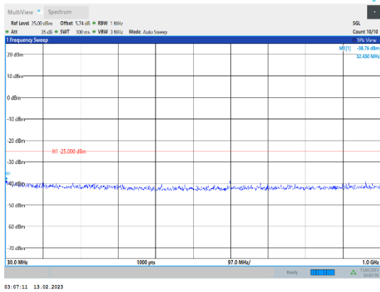
Band41-20MHz-16QAM-39750-1RB#0-Range1:30~1000MHz
