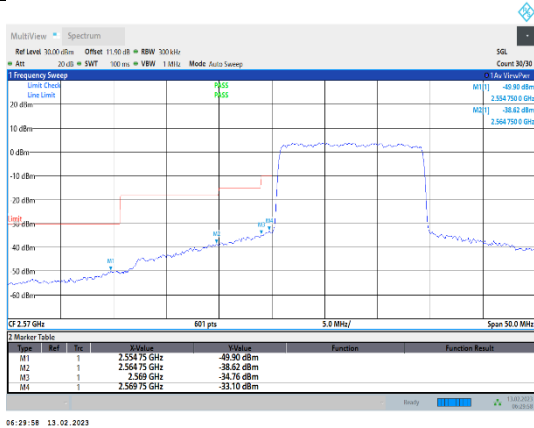
Band38-15MHz-QPSK-37825-75RB#0
