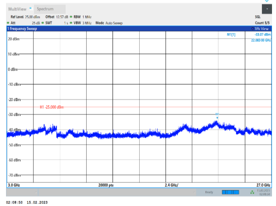
Band41-15MHz-64QAM-40620-1RB#0-Range3:3000~27000MHz
