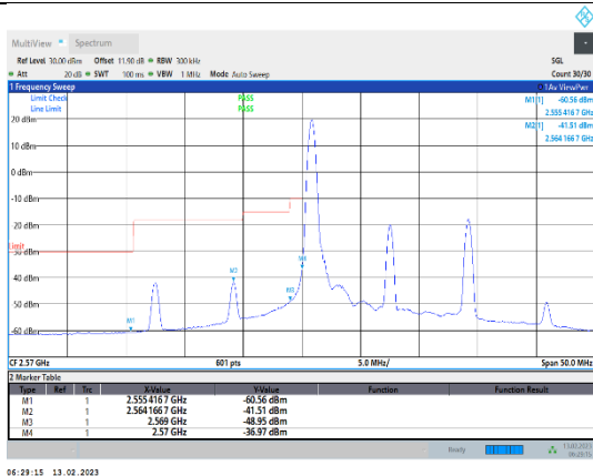
Band38-15MHz-QPSK-37825-1RB#0
