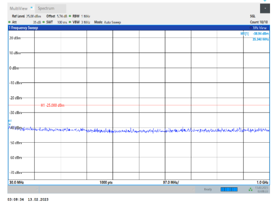
Band41-20MHz-16QAM-40620-1RB#0-Range1:30~1000MHz
