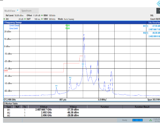
Band41-5MHz-16QAM-39675-1RB#0
