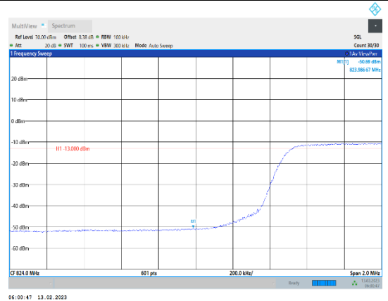
Band5-10MHz-16QAM-20450-50RB#0
