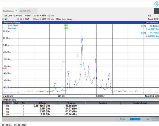
Band38-5MHz-64QAM-37775-1RB#0
