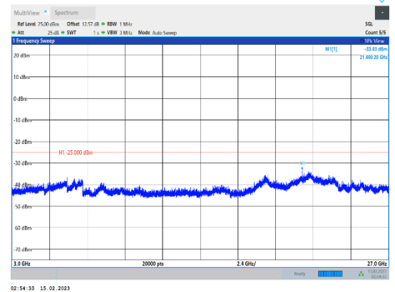
Band41-20MHz-64QAM-39750-1RB#0-Range3:3000~27000MHz
