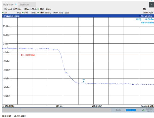
Band5-5MHz-16QAM-20625-25RB#0
