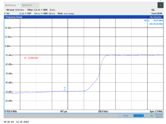
Band5-5MHz-16QAM-20425-25RB#0
