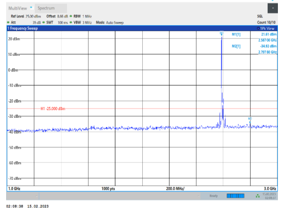
Band41-15MHz-64QAM-40620-1RB#0-Range2:1000~3000MHz
