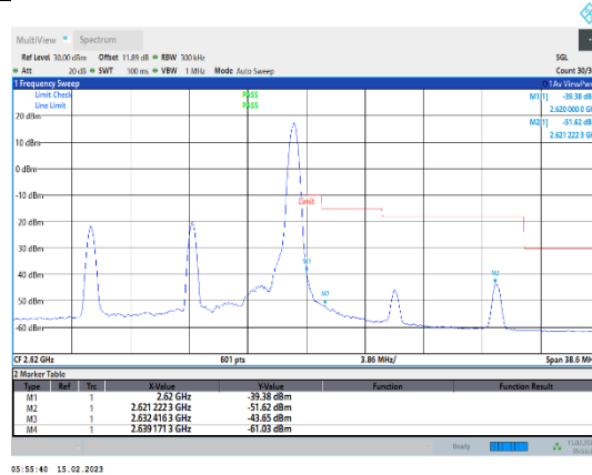
Band38-15MHz-64QAM-38175-1RB#74
