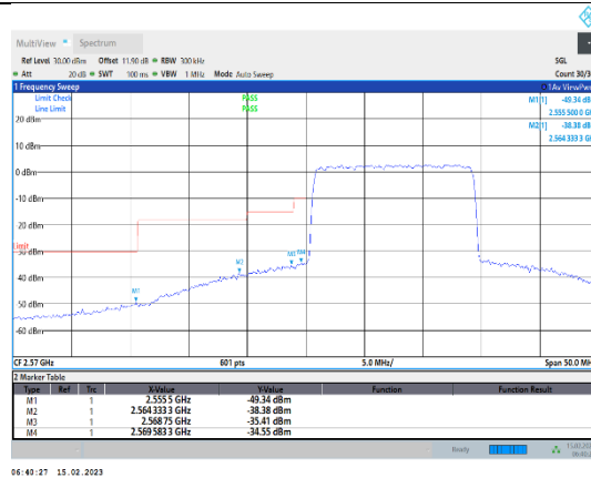
Band38-15MHz-64QAM-37825-75RB#0
