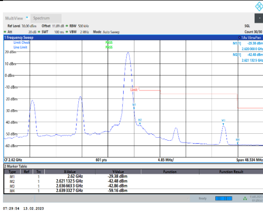
Band38-20MHz-16QAM-38150-1RB#99
