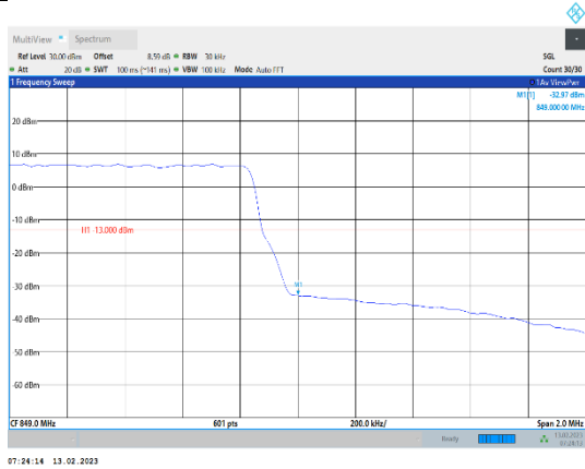
Band5-1.4MHz-16QAM-20643-6RB#0
