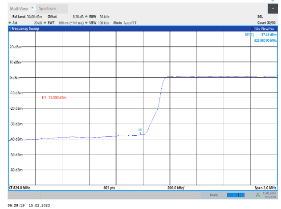
Band5-3MHz-64QAM-20415-15RB#0
