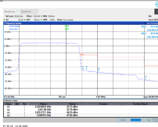
Band38-20MHz-QPSK-38150-100RB#0
