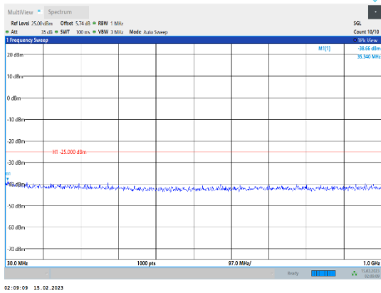
Band41-15MHz-64QAM-41515-1RB#0-Range1:30~1000MHz
