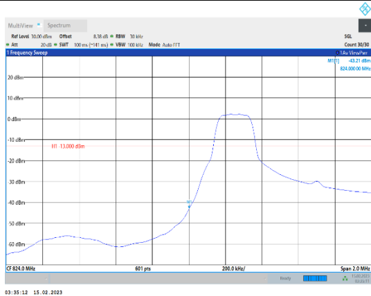
Band5-1.4MHz-64QAM-20407-1RB#0
