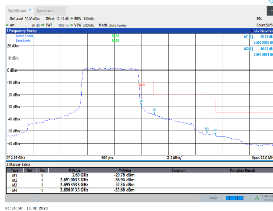
Band41-5MHz-QPSK-41565-25RB#0
