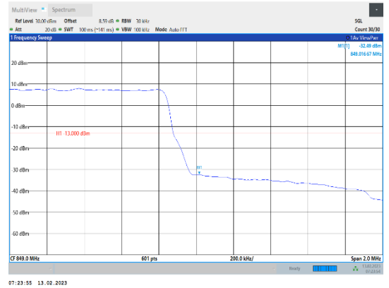
Band5-1.4MHz-QPSK-20643-6RB#0
