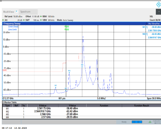
Band38-5MHz-QPSK-37775-1RB#0
