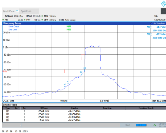
Band38-5MHz-QPSK-37775-25RB#0
