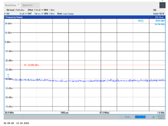
Band41-15MHz-64QAM-40620-1RB#0-Range1:30~1000MHz
