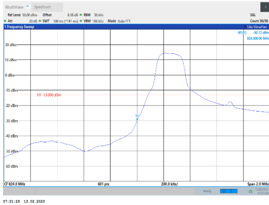
Band5-1.4MHz-QPSK-20407-1RB#0
