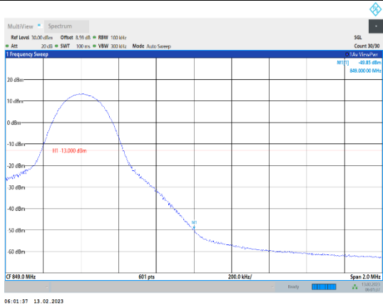
Band5-10MHz-QPSK-20600-1RB#49
