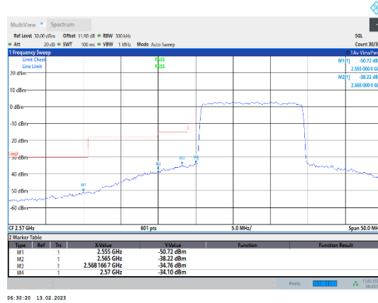
Band38-15MHz-16QAM-37825-75RB#0
