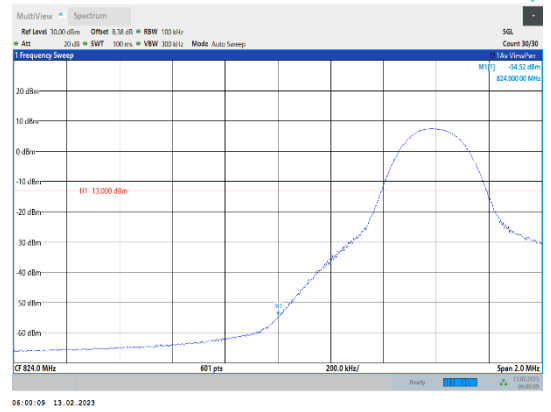
Band5-10MHz-16QAM-20450-1RB#0
