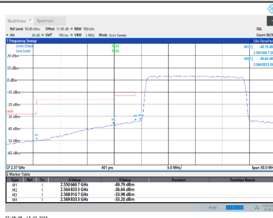
Band38-20MHz-16QAM-37850-100RB#0
