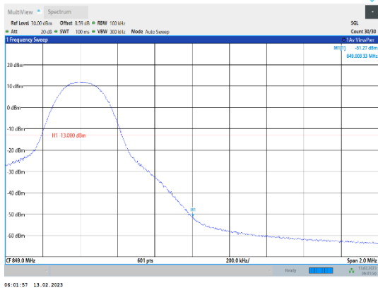
Band5-10MHz-16QAM-20600-1RB#49
