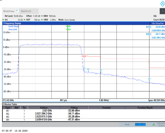
Band38-20MHz-16QAM-38150-100RB#0
