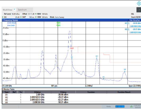
Band41-5MHz-QPSK-41565-1RB#24
