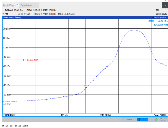
Band5-10MHz-64QAM-20450-1RB#0
