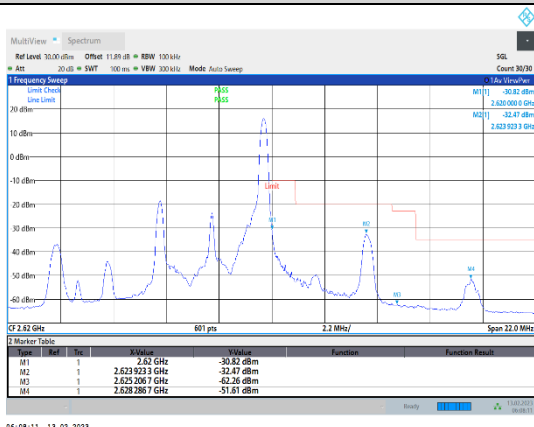
Band38-5MHz-QPSK-38225-1RB#24
