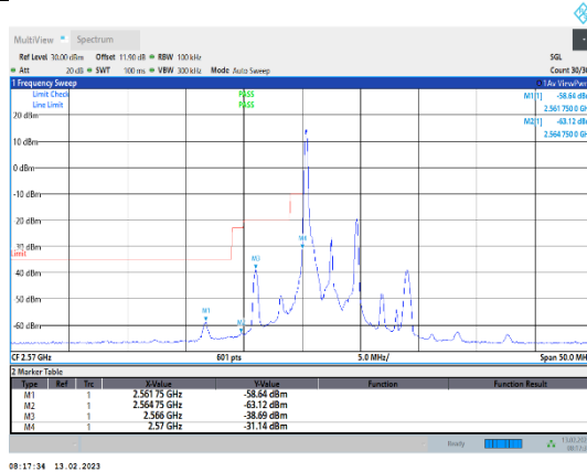
Band38-5MHz-16QAM-37775-1RB#0
