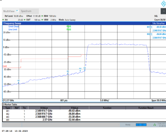
Band38-20MHz-QPSK-37850-100RB#0
