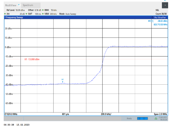
Band5-5MHz-64QAM-20425-25RB#0
