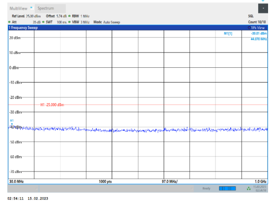
Band41-20MHz-64QAM-39750-1RB#0-Range1:30~1000MHz
