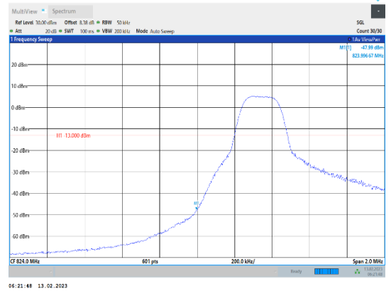
Band5-5MHz-16QAM-20425-1RB#0
