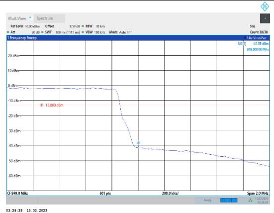
Band5-1.4MHz-64QAM-20643-6RB#0
