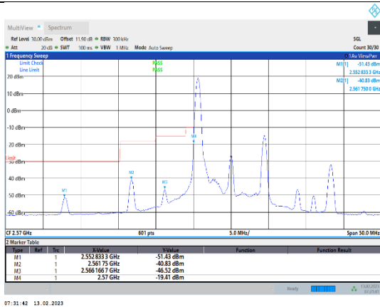
Band38-10MHz-QPSK-37800-1RB#0
