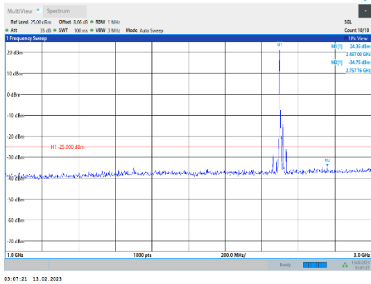
Band41-20MHz-16QAM-39750-1RB#0-Range2:1000~3000MHz
