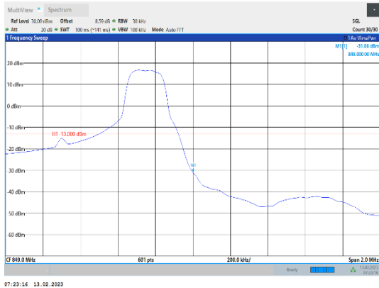
Band5-1.4MHz-QPSK-20643-1RB#5
