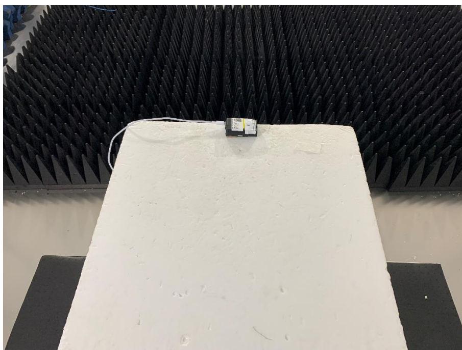
Above 1GHz-LoRa
