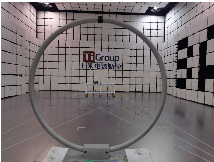
Below 30MHz-LoRa
