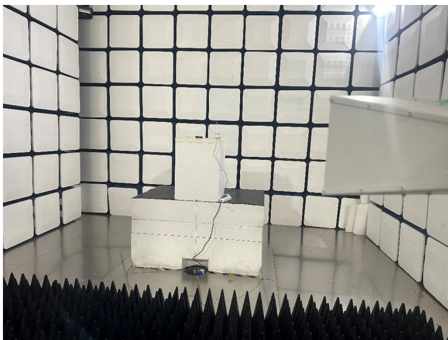
Above 1GHz-BLE
