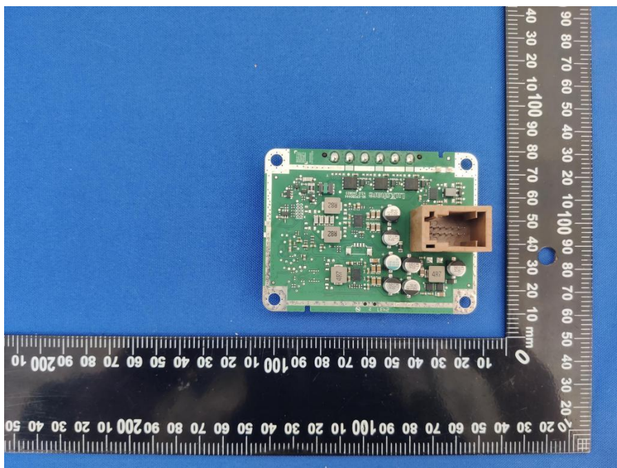
MAIN BOARD TOP VIEW_WCM(fanless)
