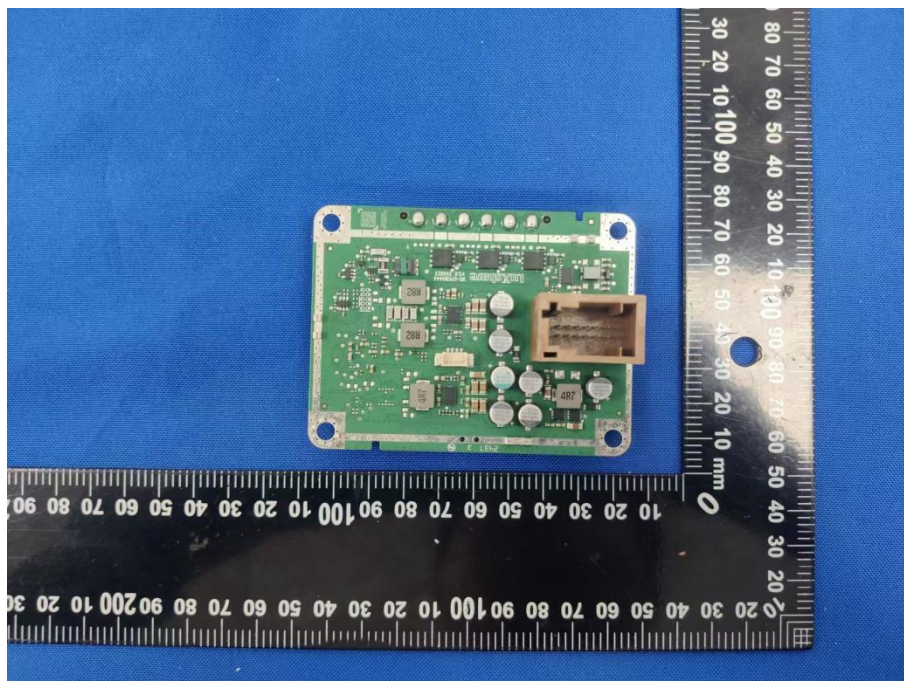
MAIN BOARD TOP VIEW_WCM(Have a fan)
