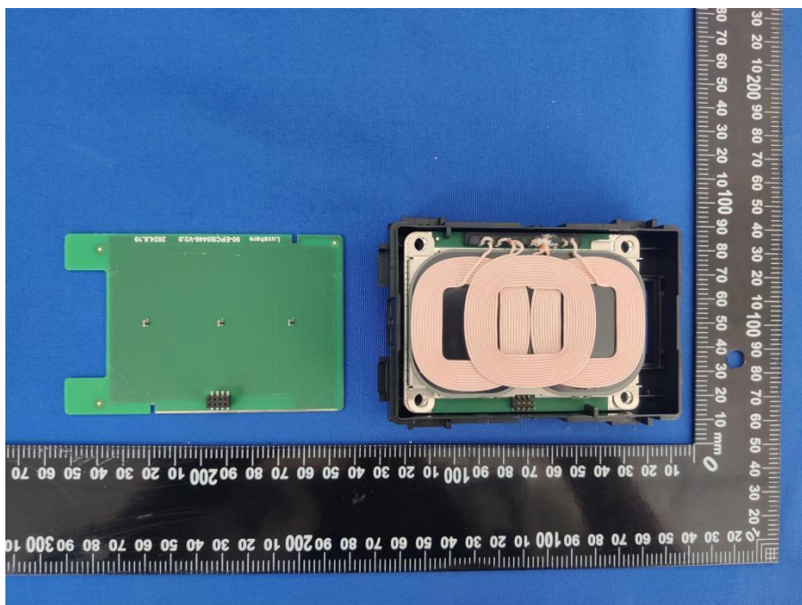
EUT UNCOVER VIEW 2_WCM(fanless)
