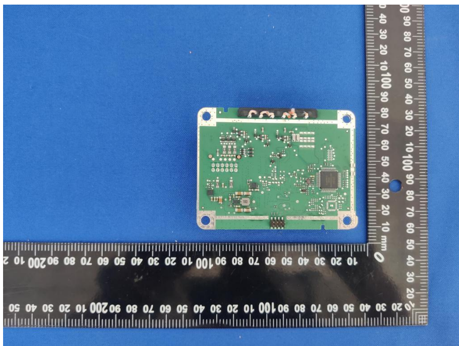
MAIN BOARD REAR VIEW_WCM(fanless)
