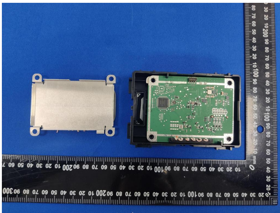
EUT UNCOVER VIEW 3_WCM(Have a fan)
