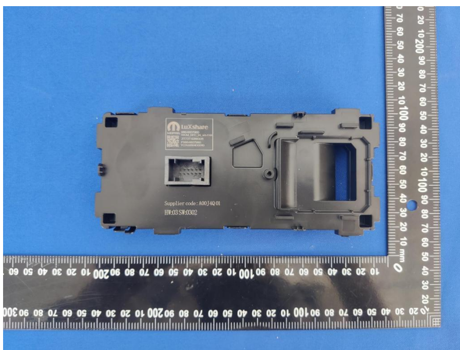
REAR VIEW OF EUT_WCM_NFC_Int(fanless)
