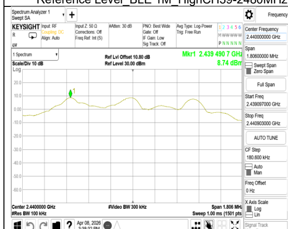
Reference Level_BLE 2M_MidCH19-2440MHz
