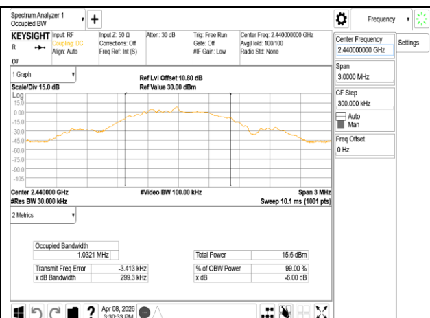
IC OBW_BLE 1M_MidCH19-2440MHz
