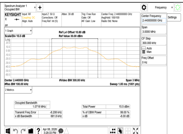
OBW_BLE 1M_MidCH19-2440MHz
