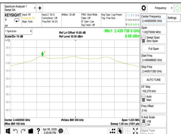
Reference Level_BLE 1M_MidCH19-2440MHz
