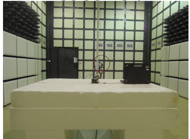
FCC_15_247_BT_Radiated_Setup
