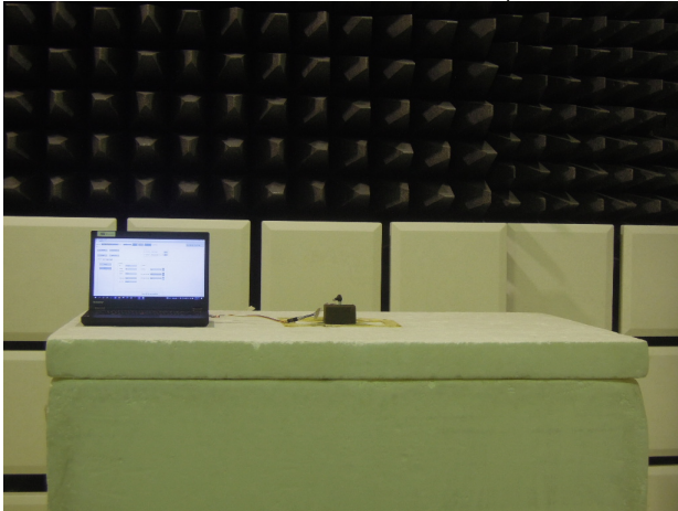
FCC_15_247_BLE_Radiated_Setup
