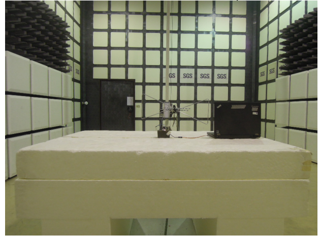
FCC_15_247_BLE_Radiated_Setup
