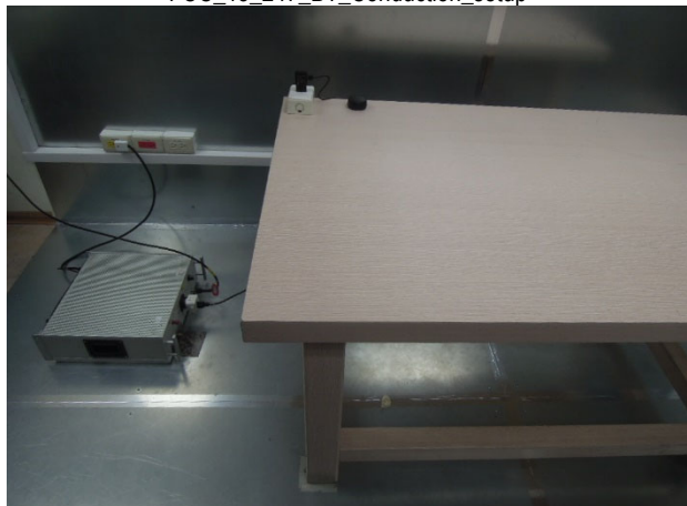
FCC_15_247_BT_Conduction_setup
