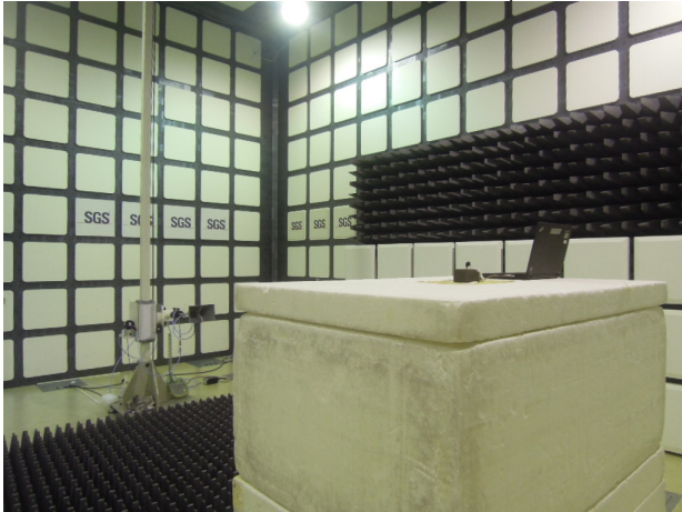
FCC_15_247_BLE_Radiated_Setup
