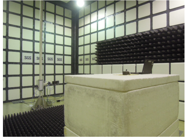
FCC_15_247_BT_Radiated_Setup
