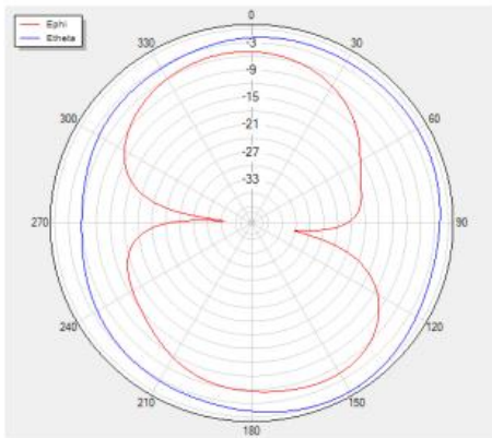
Phi=90 freq=750MHz
