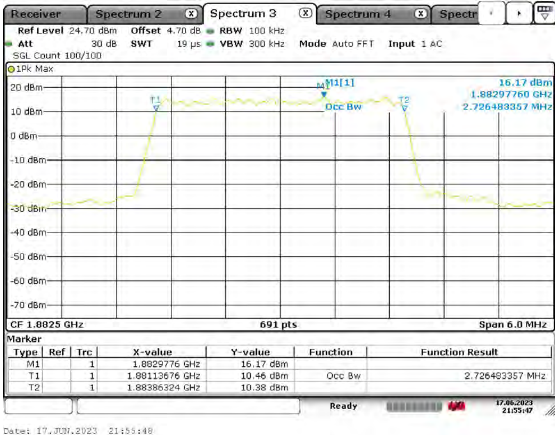
Band25-3MHz-16QAM-26365-15RB#0
