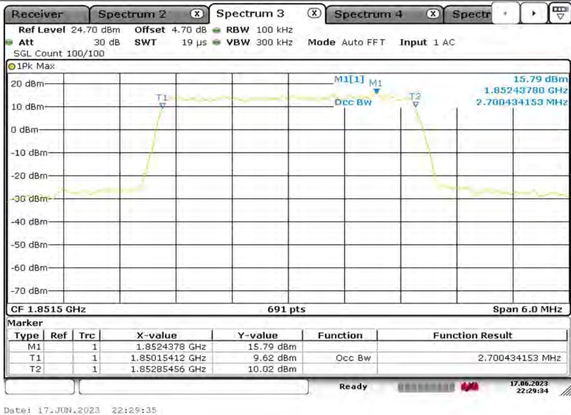
Band25-3MHz-16QAM-26055-15RB#0
