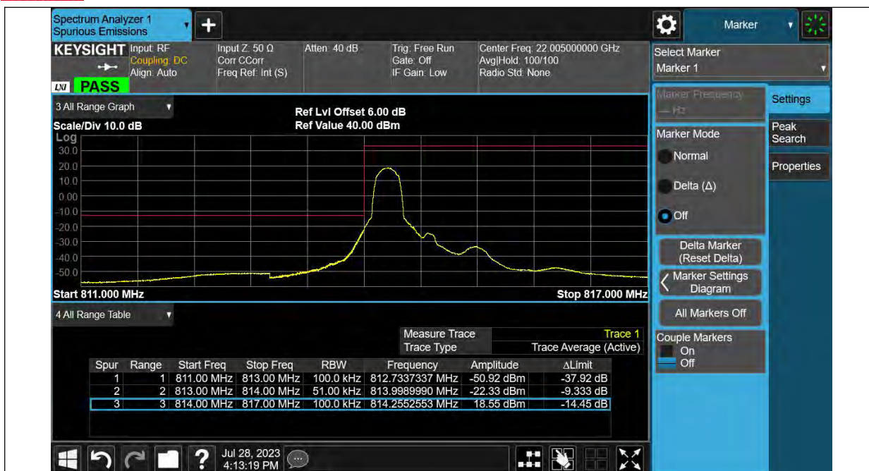
Band26-1.4MHz-64QAM-26697-6RB#0
