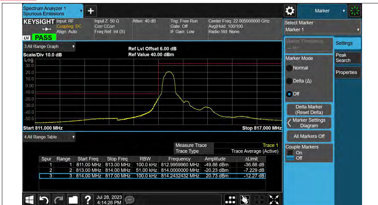
Band26-1.4MHz-16QAM-26697-6RB#0
