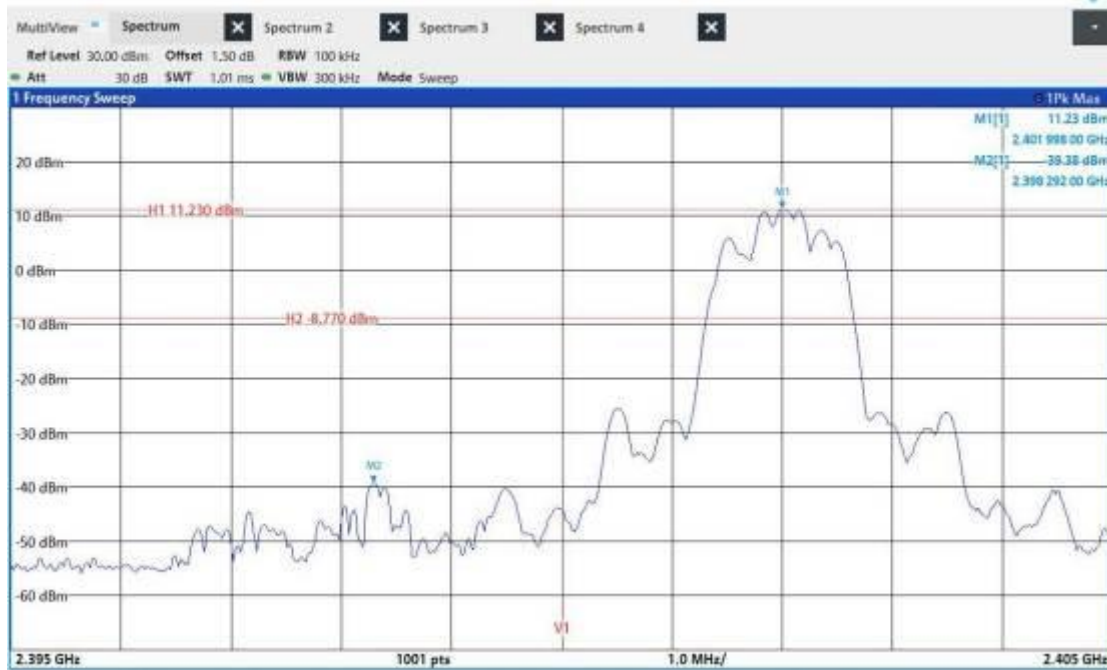
3DH5_Ant1_Low_2402
