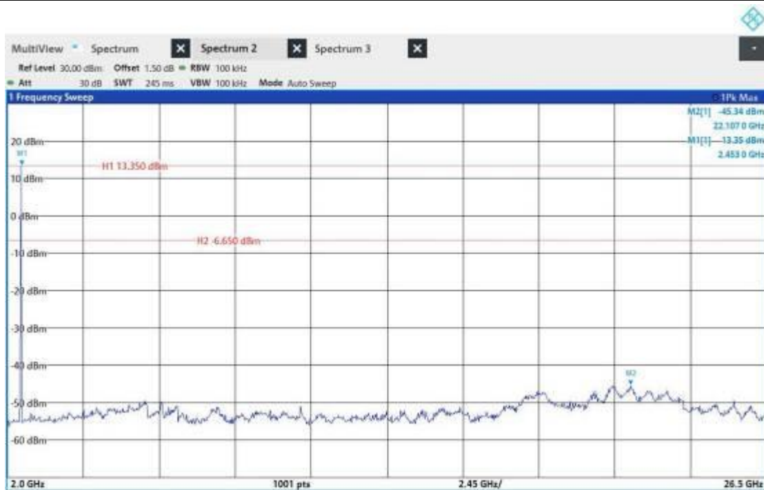
DH5_Ant1_2441_2000~26500
