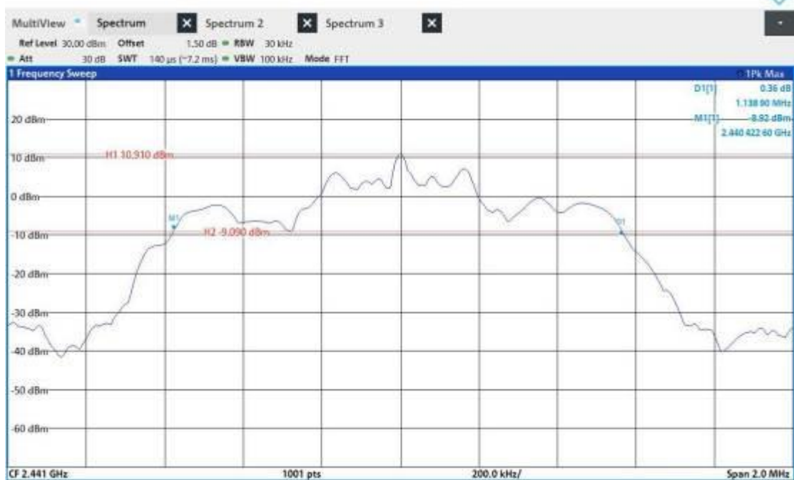
3DH5_Ant1_2441
