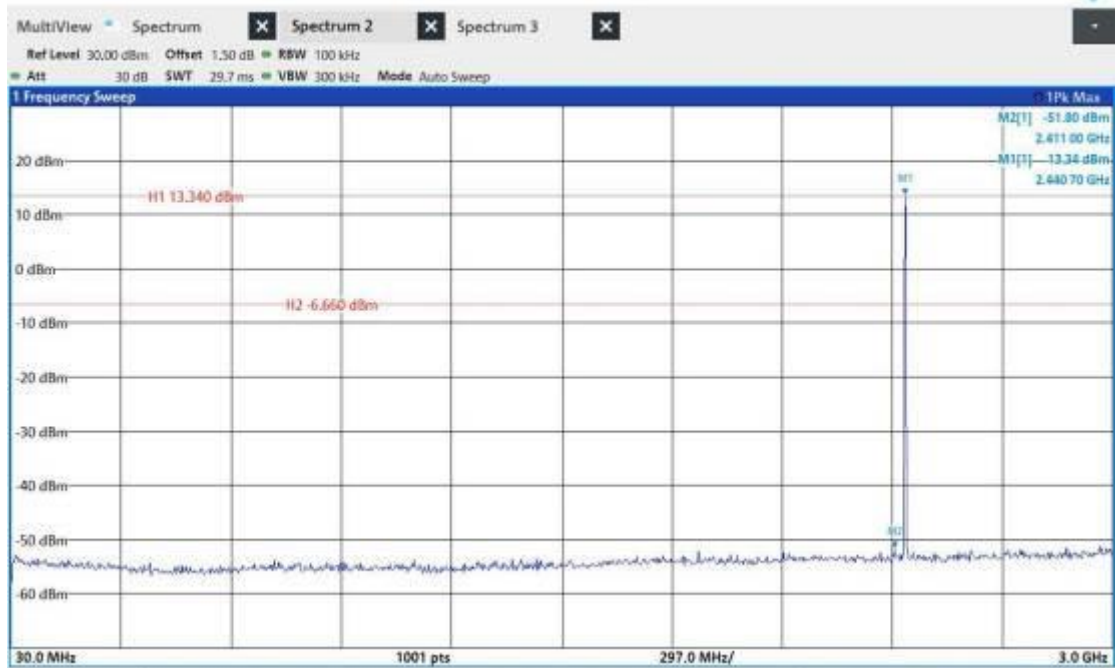
DH5_Ant1_2441_30~3000
