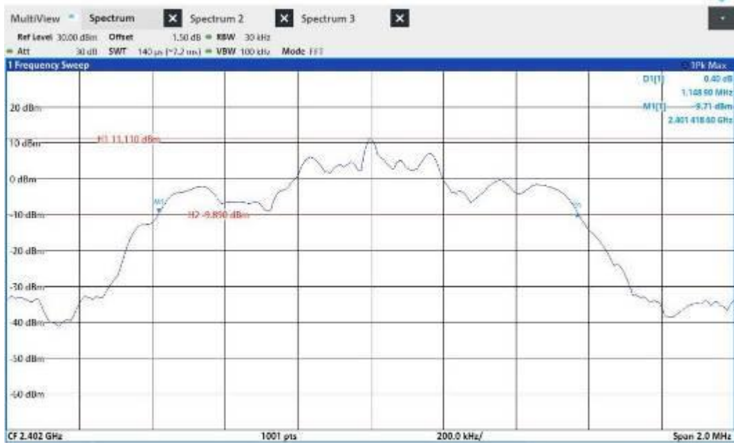
3DH5_Ant1_2402
