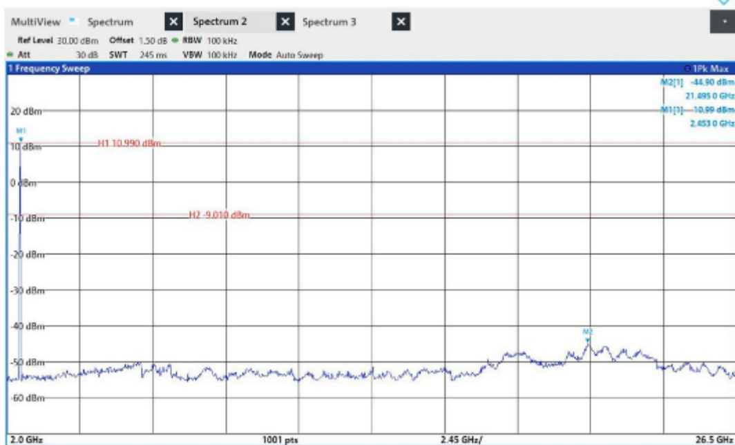
2DH5_Ant1_2441_2000~26500
