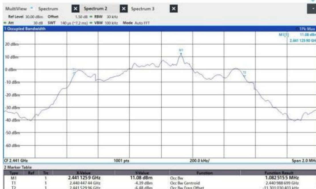
2DH5_Ant1_2441
