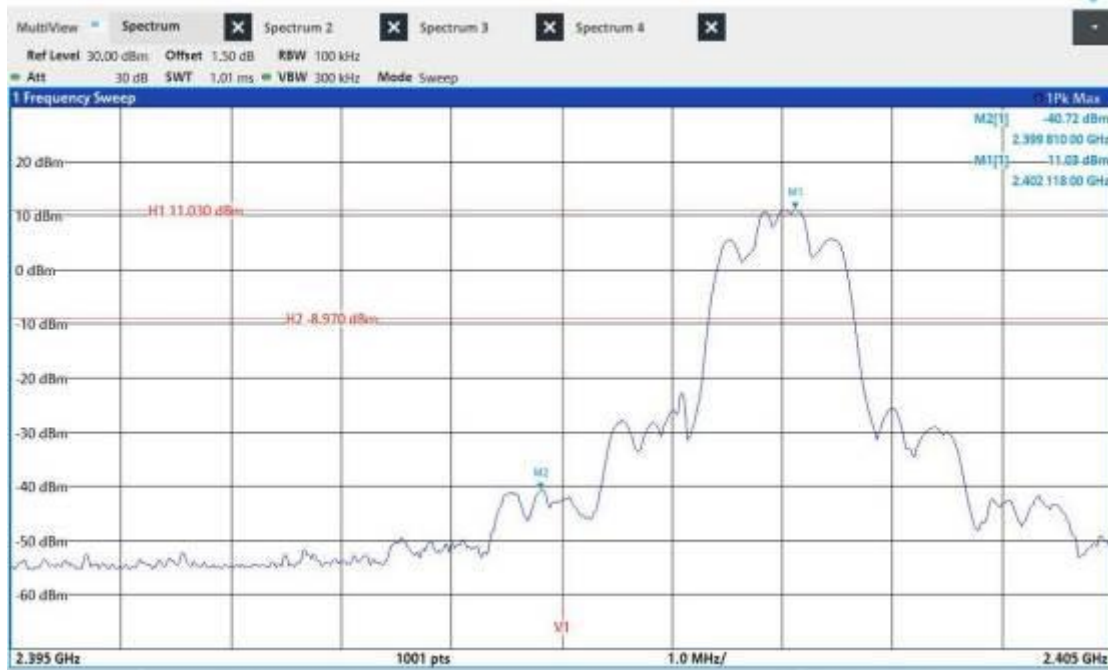
2DH5_Ant1_Low_2402
