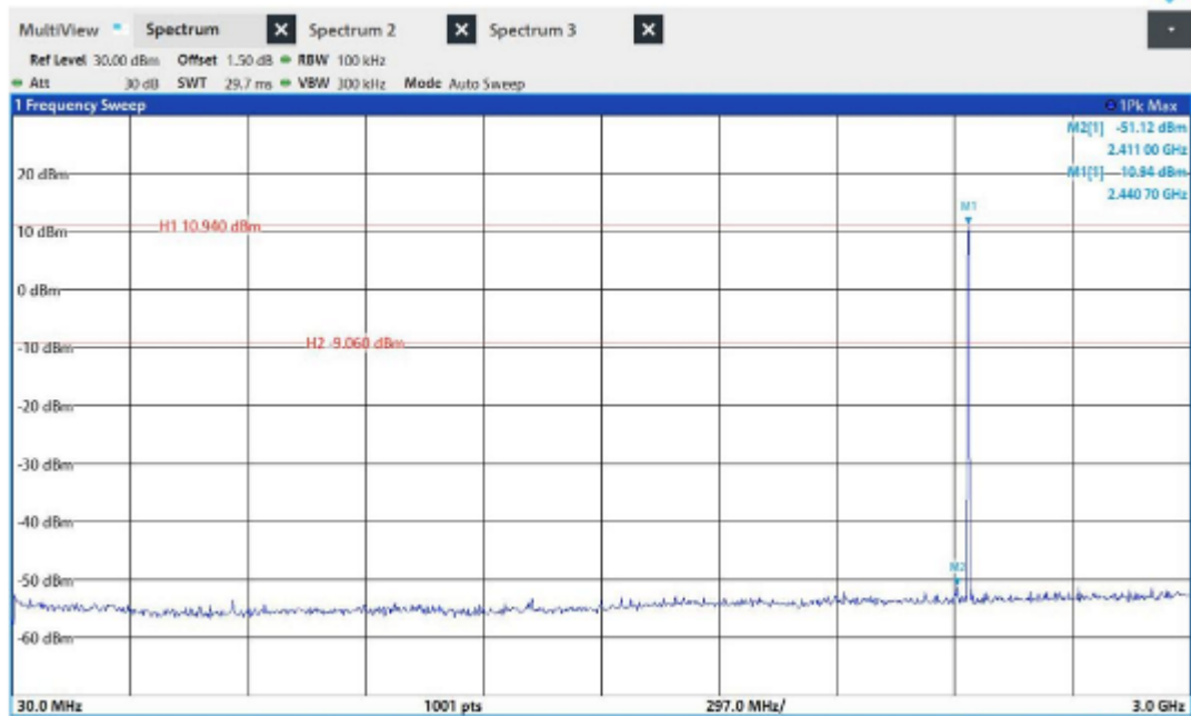
2DH5_Ant1_2441_30~3000
