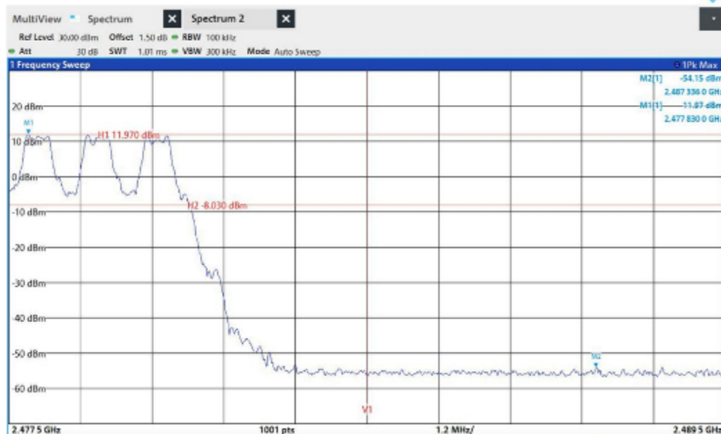
DH5_Ant1_High_Hop_2480
