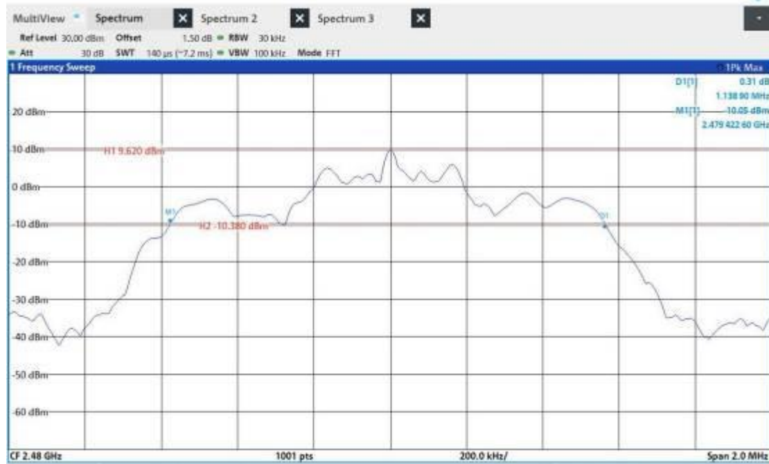
3DH5_Ant1_2480
