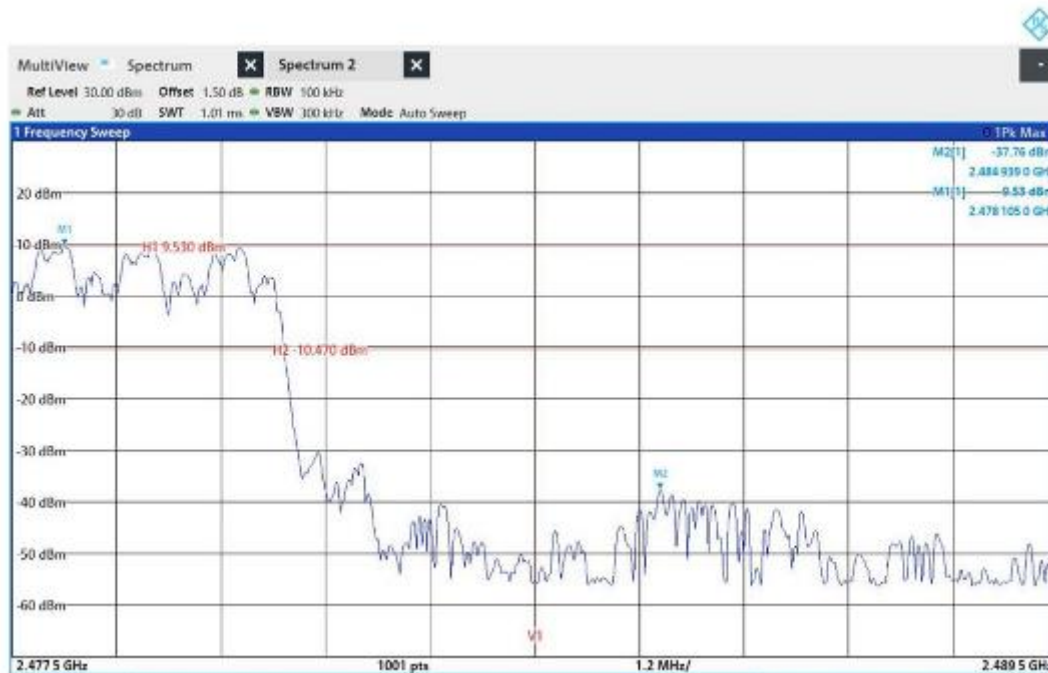
2DH5_Ant1_High_Hop_2480
