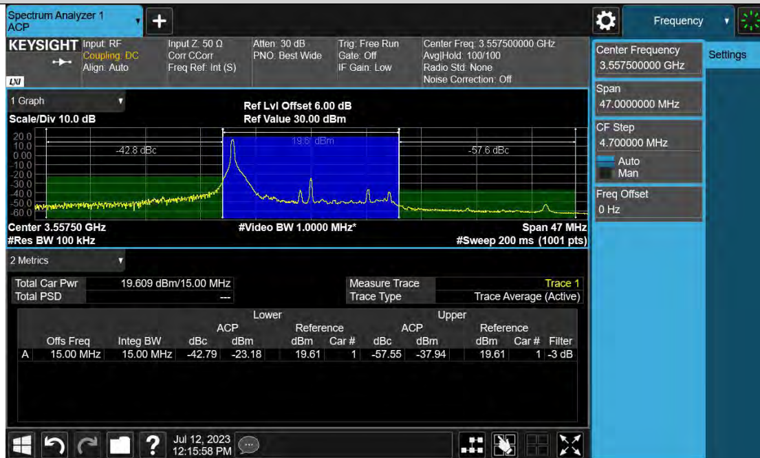
Band48-15MHz-QPSK-55315-75RB#0
