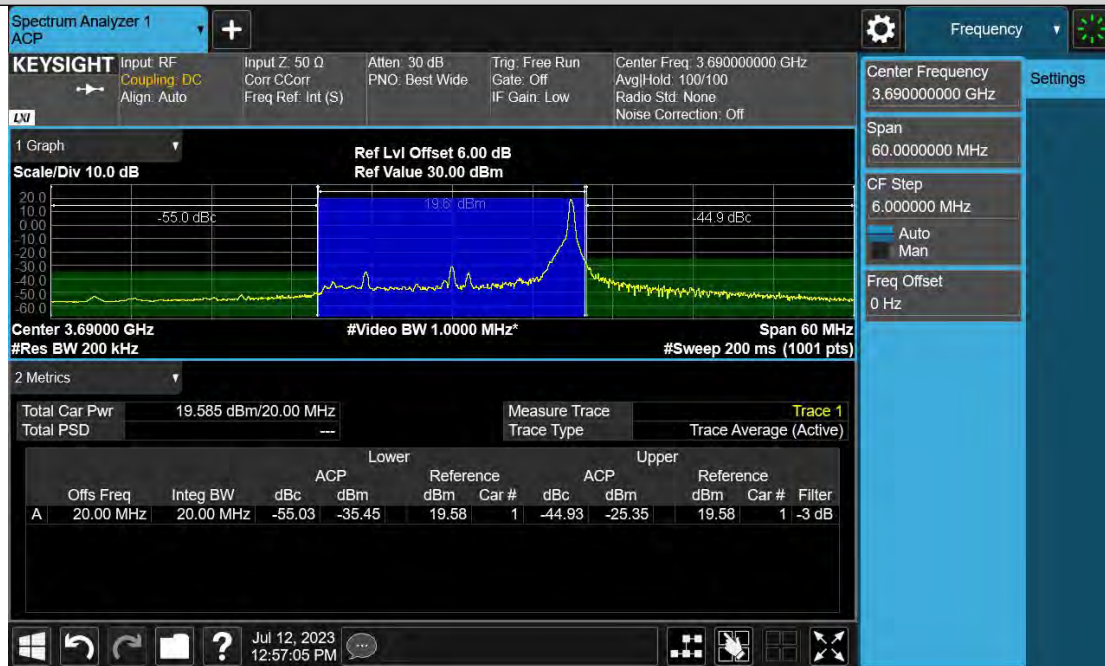
Band48-20MHz-QPSK-56640-100RB#0
