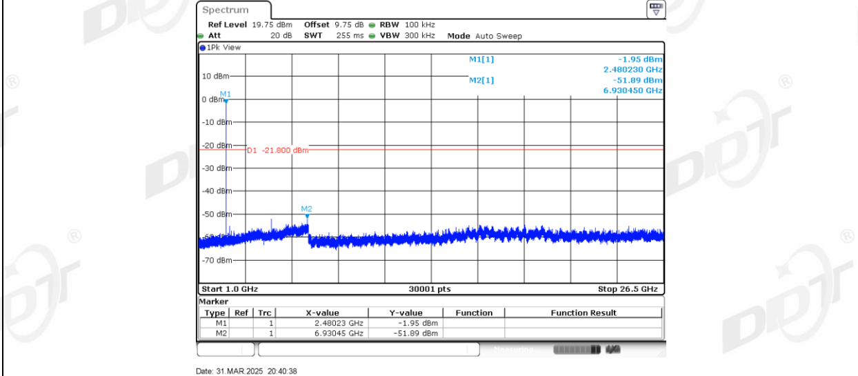
3DH5 Right side 2480 0~Reference
