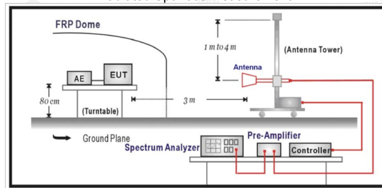
Radiated Spurious Measurement:
