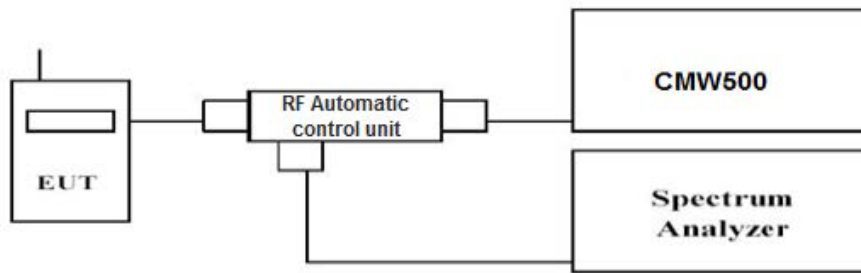
Conducted Spurious Measurement:
