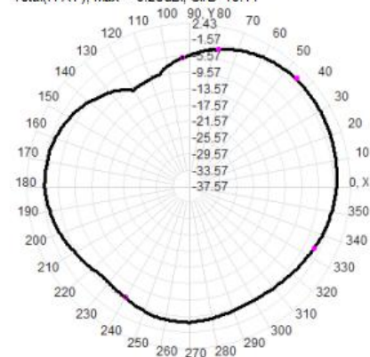
Total(H-XY), Max= -0.23dBi, CirD=10.11
