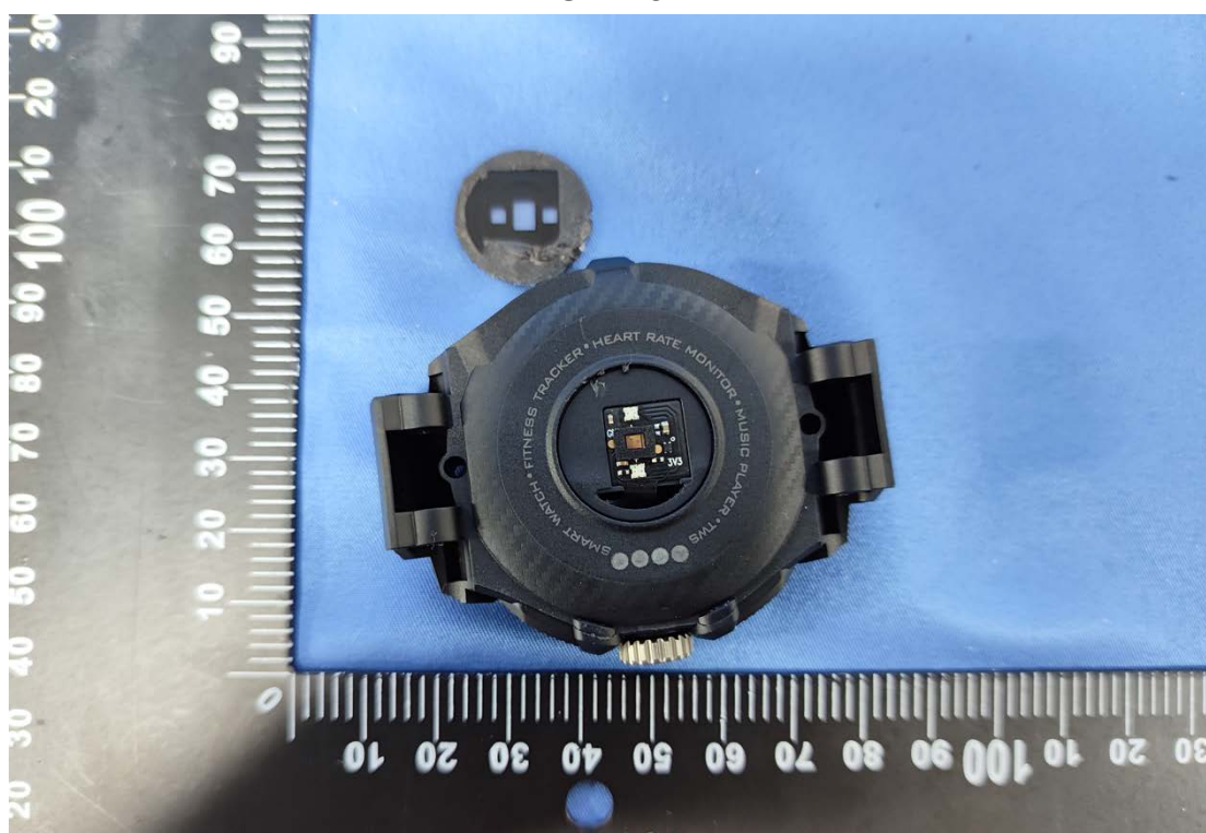
EUT View
