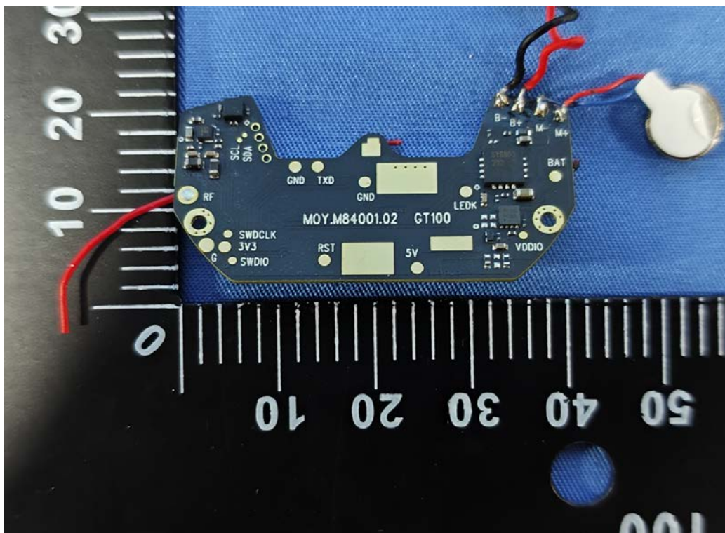
EUT View
