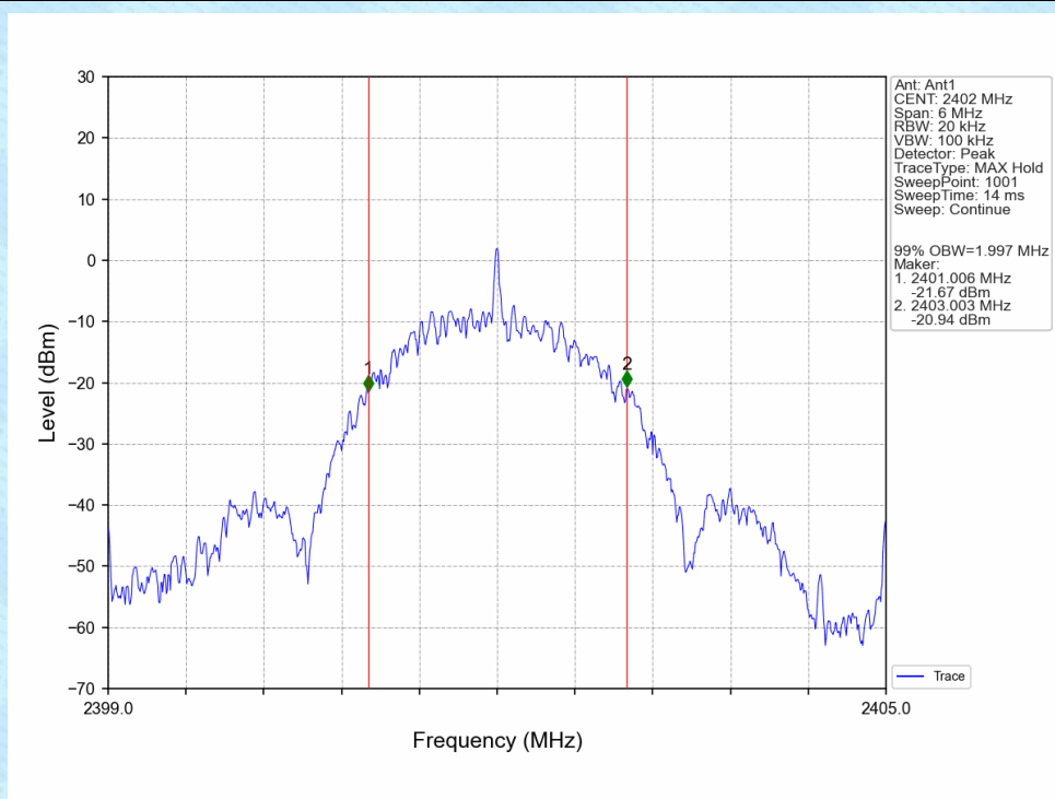
2M_LCH_2402MHz_Ant1_NTNV
