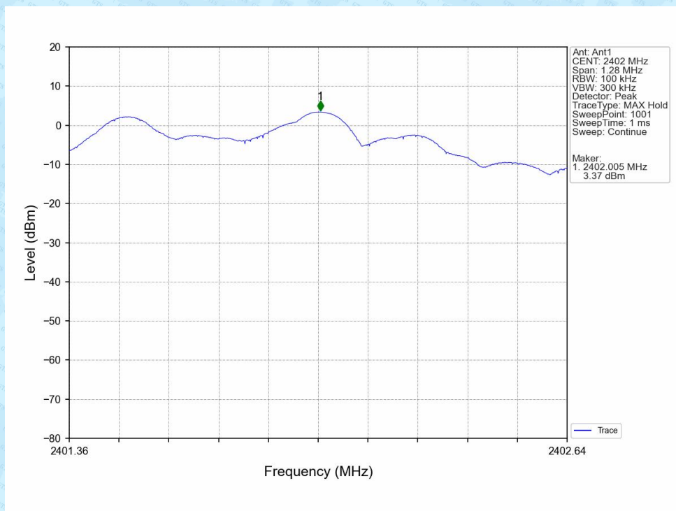
2M_LCH_2402MHz_Ant1_NTNV
