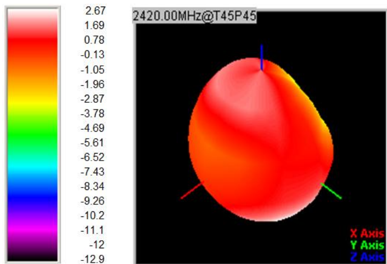
© 3D Gain Pattern (2420 MHz)
