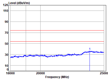
2.4G SRD_TX_CH_M_Horizontal
