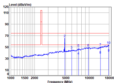
2.4G SRD_TX_CH_M_Horizontal
