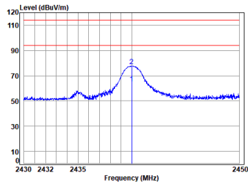
2.4G SRD_TX_CH_M_Horizontal
