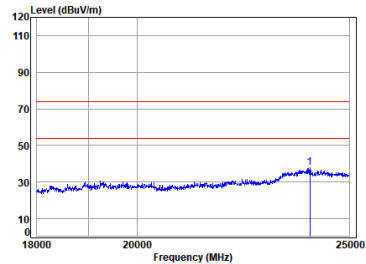
2.4G SRD_TX_CH_M_Vertical
