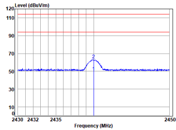
2.4G SRD_TX_CH_M_Vertical
