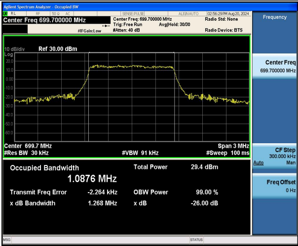
Band12-1.4MHz-16QAM-23017-6RB#0-PASS
