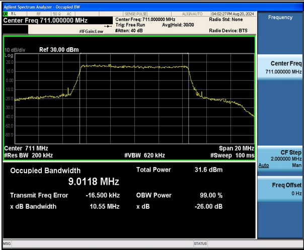
Band12-10MHz-QPSK-23130-50RB#0-PASS
