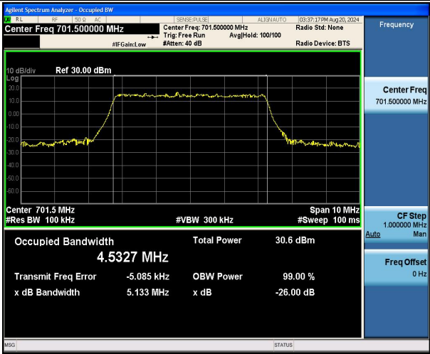
Band12-5MHz-16QAM-23035-25RB#0-PASS
