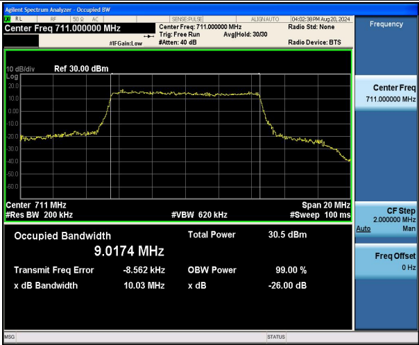
Band12-10MHz-16QAM-23130-50RB#0-PASS
