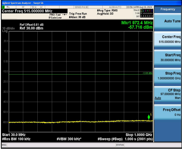
Band2_20MHz_16QAM_18700_1RB#0_30~1000_30~1000
