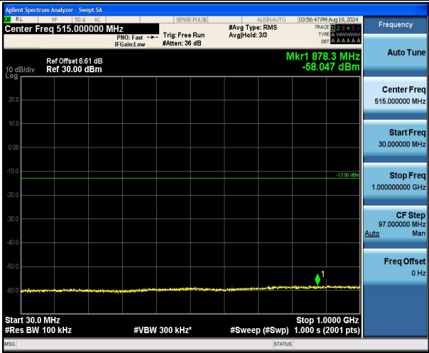
Band2_20MHz_QPSK_18900_1RB#0_30~1000_30~1000
