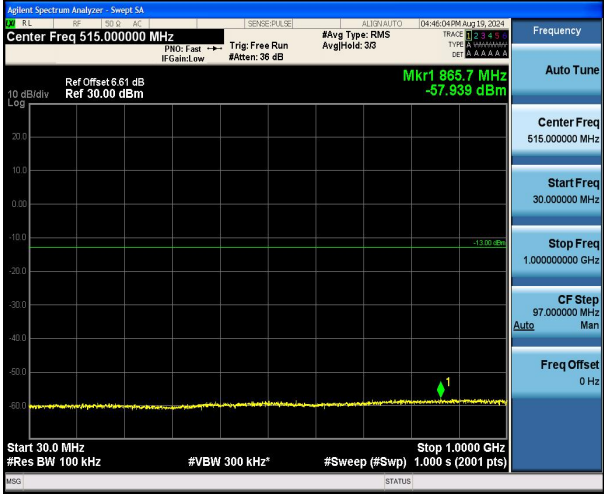
Band4_5MHz_16QAM_19975_1RB#0_30~1000_30~1000
