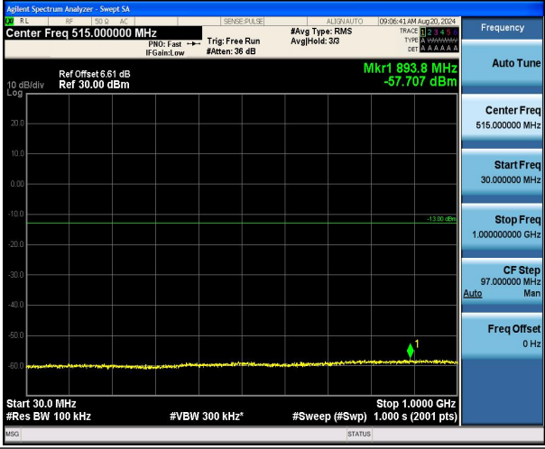
Band4_15MHz_QPSK_20325_1RB#0_30~1000_30~1000
