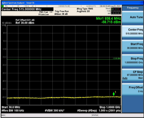
Band4_10MHz_QPSK_20350_1RB#0_30~1000_30~1000
