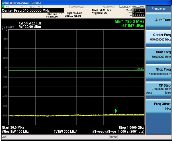
Band4_15MHz_16QAM_2025_1RB#0_30~1000_30~1000
