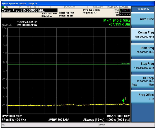
Band4_3MHz_16QAM_20385_1RB#0_30~1000_30~1000
