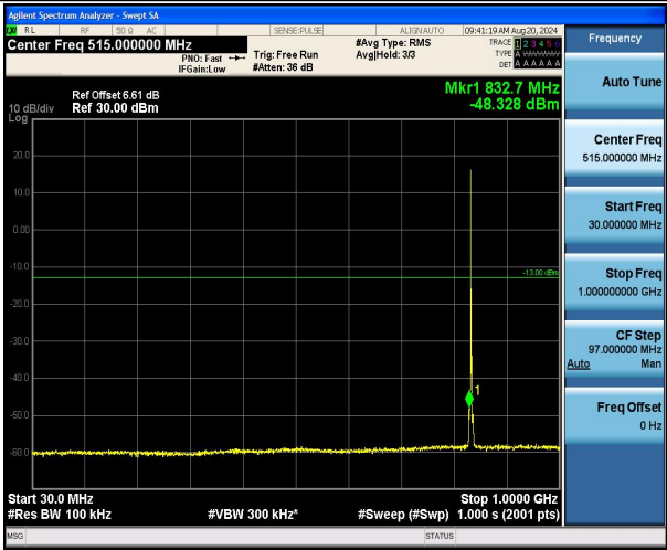
Band5_1.4MHz_QPSK_20525_1RB#0_30~1000_30~1000
