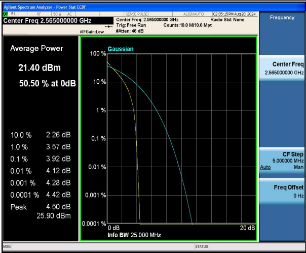
Band7-10MHz-QPSK-21400-50RB#0-PASS
