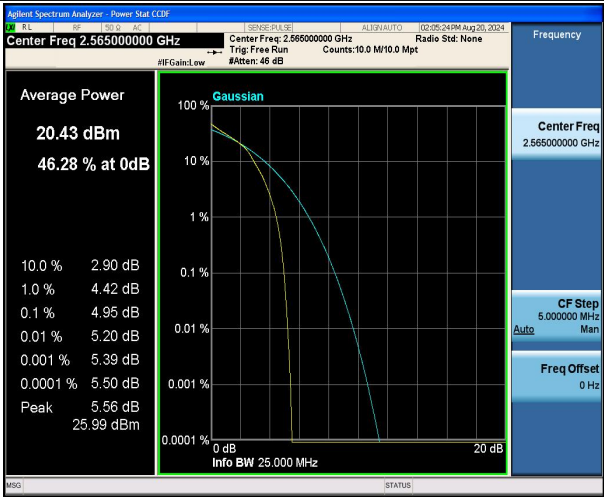
Band7-10MHz-16QAM-21400-50RB#0-PASS
