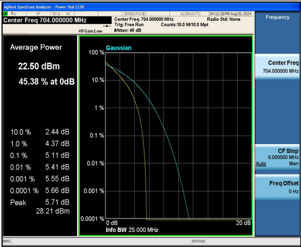
Band12-10MHz-QPSK-23060-50RB#0-PASS
