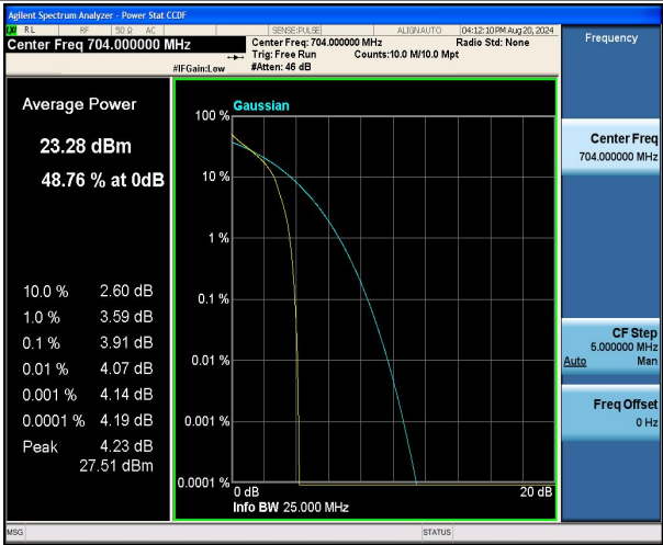
Band12-10MHz-QPSK-23060-1RB#0-PASS
