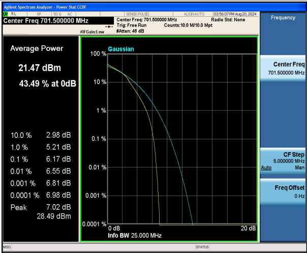
Band12-5MHz-16QAM-23035-25RB#0-PASS
