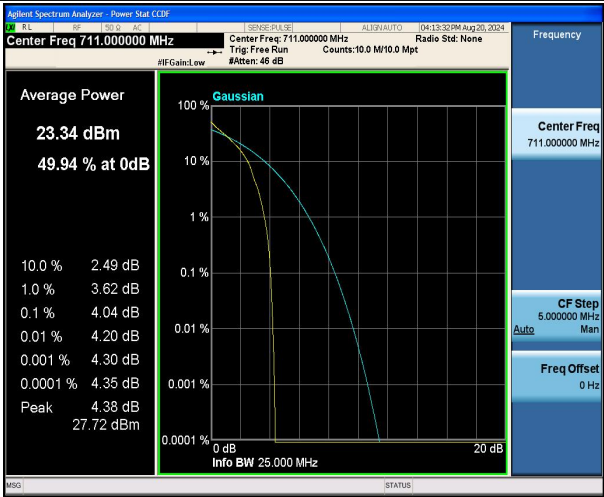
Band12-10MHz-QPSK-23130-1RB#0-PASS
