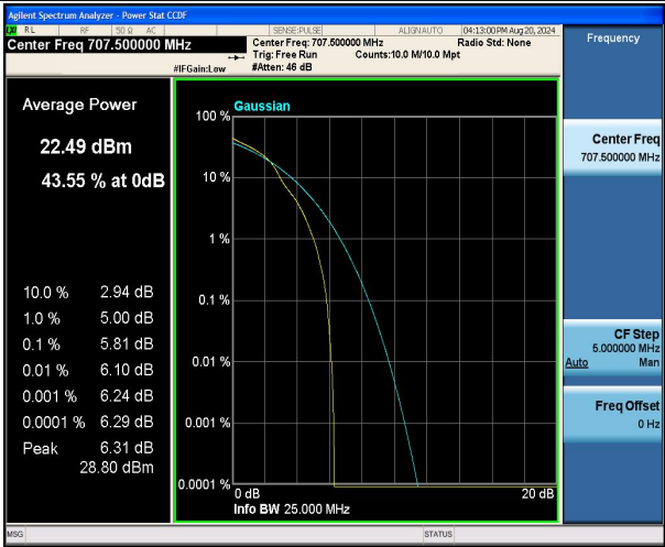
Band12-10MHz-16QAM-23095-1RB#0-PASS
