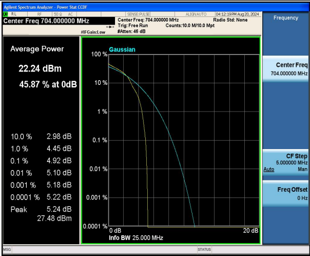
Band12-10MHz-16QAM-23060-1RB#0-PASS
