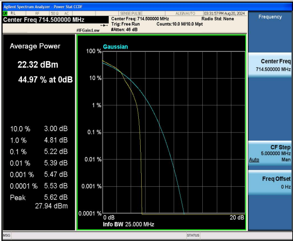
Band12-3MHz-16QAM-23165-1RB#0-PASS
