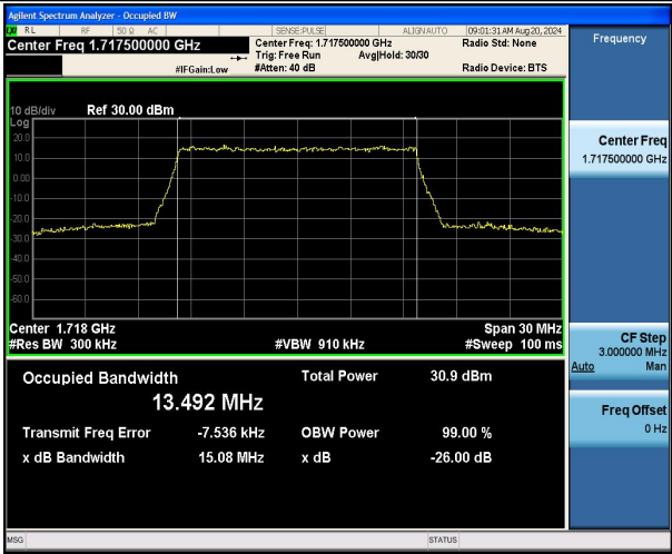
Band4-15MHz-16QAM-20025-75RB#0-PASS
