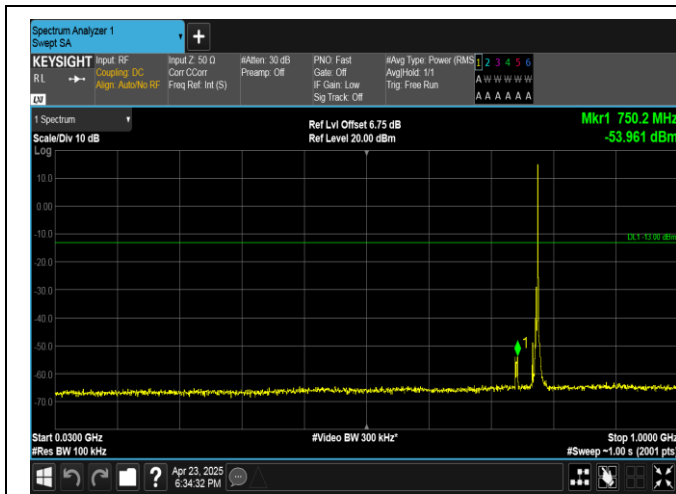
Band13-5MHz-16QAM-23205-1RB#24-30~1000-PASS
