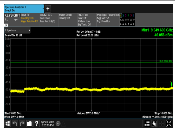
Band13-5MHz-16QAM-23255-25RB#0-3000~10000-PASS
