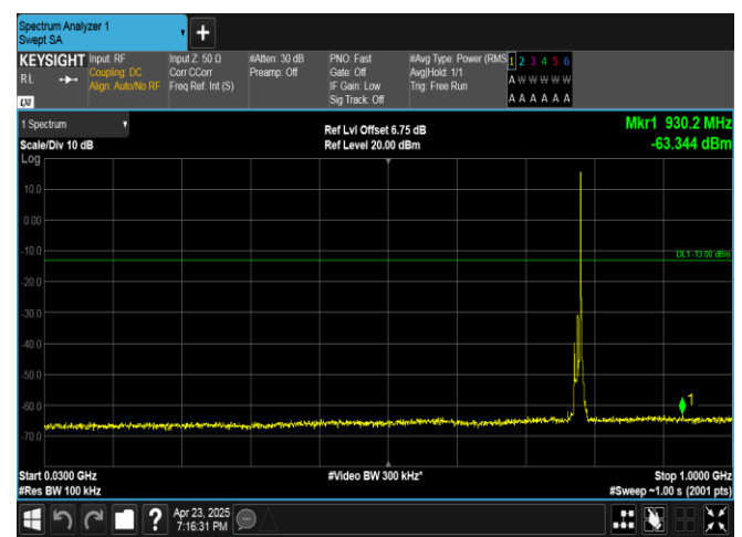
Band13-10MHz-QPSK-23230-1RB#49-30~1000-PASS
