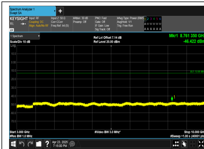
Band13-10MHz-QPSK-23230-1RB#0-3000~10000-PASS
