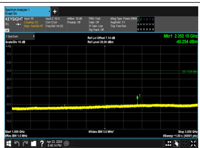
Band13-5MHz-QPSK-23230-1RB#24-1000~3000-PASS
