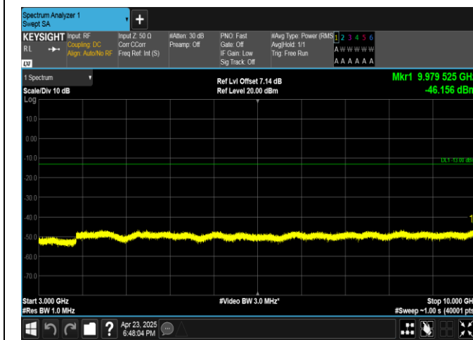
Band13-5MHz-16QAM-23255-1RB#24-3000~10000-PASS
