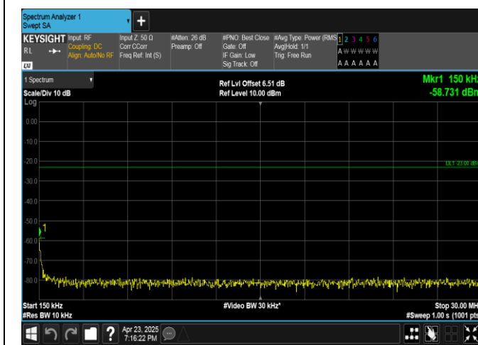
Band13-10MHz-QPSK-23230-1RB#49-0.15~30-PASS
