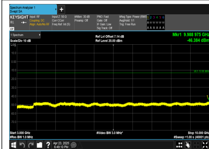
Band13-5MHz-QPSK-23255-25RB#0-3000~10000-PASS
