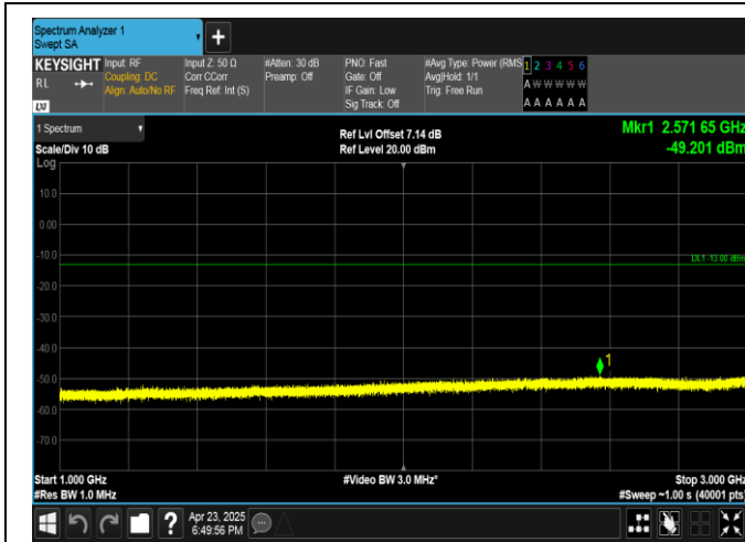
Band13-5MHz-16QAM-23255-25RB#0-1000~3000-PASS
