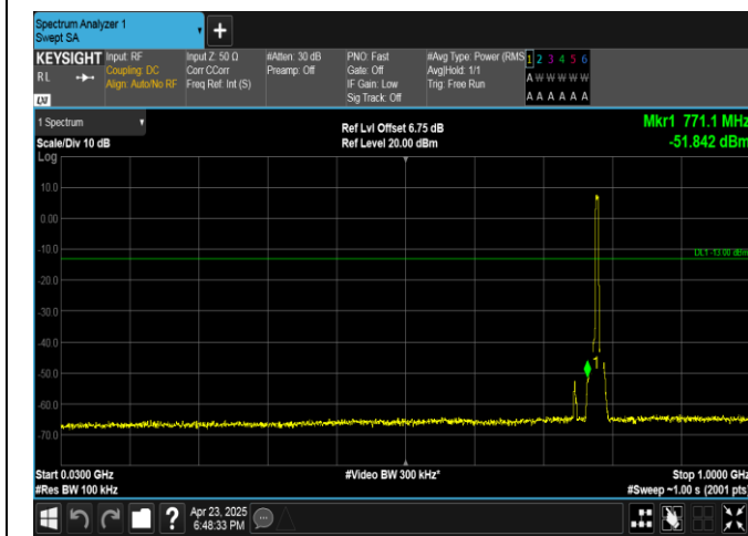
Band13-5MHz-QPSK-23255-25RB#0-30~1000-PASS
