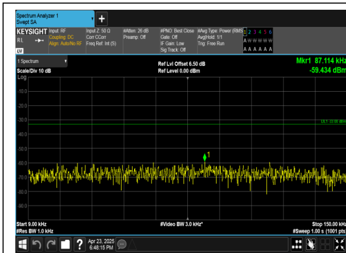
Band13-5MHz-QPSK-23255-25RB#0-0.009~0.15-PASS
