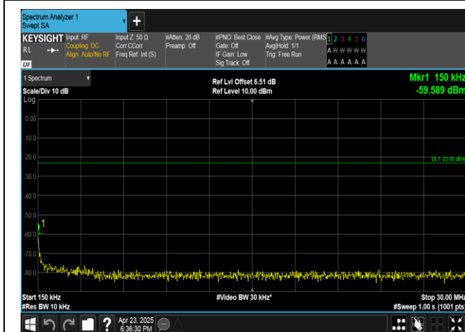
Band13-5MHz-16QAM-23205-25RB#0-0.15~30-PASS
