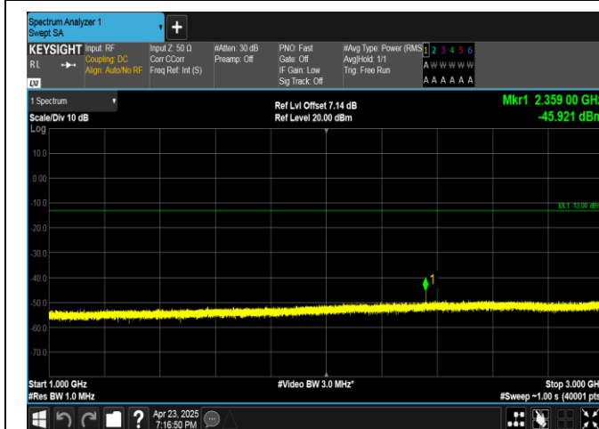
Band13-10MHz-QPSK-23230-1RB#49-1000~3000-PASS
