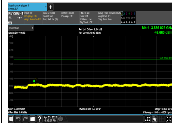
Band13-5MHz-16QAM-23205-1RB#24-3000~10000-PASS
