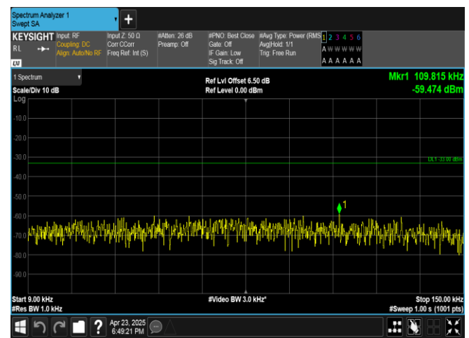
Band13-5MHz-16QAM-23255-25RB#0-0.009~0.15-PASS
