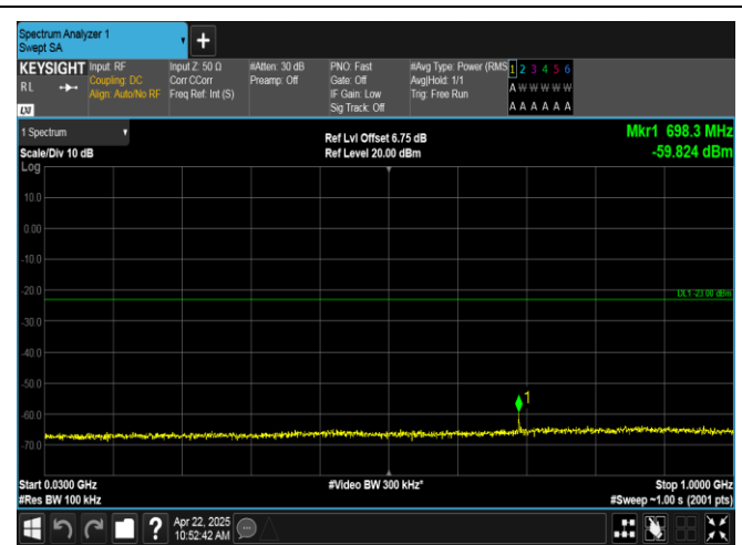
Band2-1.4MHz-16QAM-18900-1RB#5-30~1000-PASS
