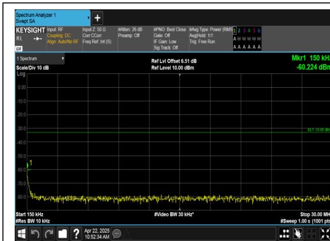
Band2-1.4MHz-16QAM-18900-1RB#5-0.15~30-PASS
