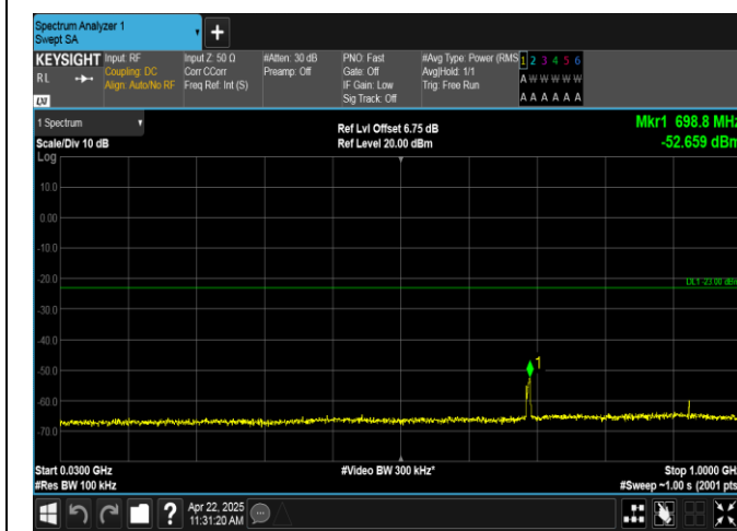
Band2-3MHz-QPSK-18615-1RB#0-30~1000-PASS
