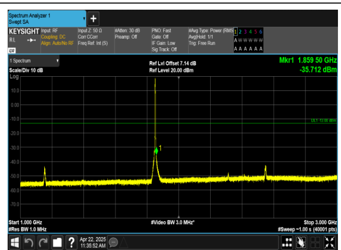
Band2-3MHz-QPSK-18615-15RB#0-1000~3000-PASS
