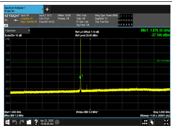
Band2-1.4MHz-16QAM-18900-6RB#0-1000~3000-PASS
