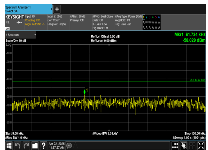
Band2-3MHz-QPSK-18900-1RB#0-0.009~0.15-PASS
