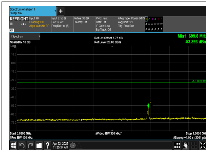
Band2-3MHz-QPSK-18615-15RB#0-30~1000-PASS
