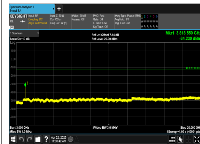
Band2-1.4MHz-QPSK-19193-6RB#0-3000~20000-PASS
