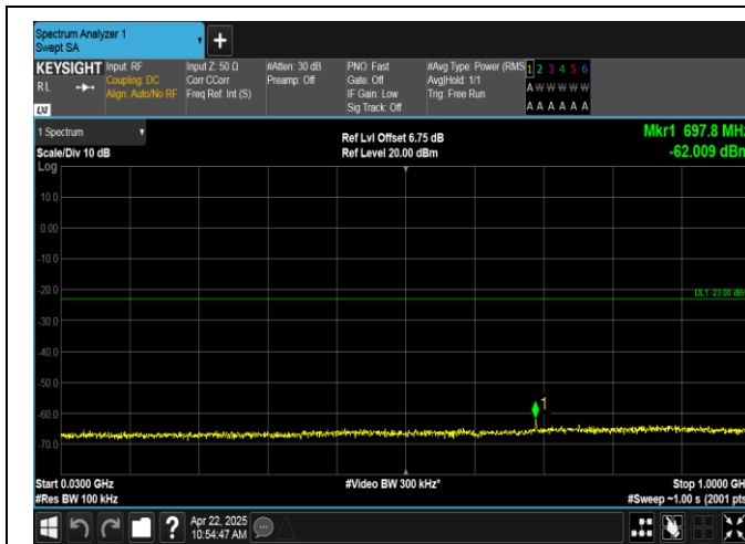
Band2-1.4MHz-16QAM-18900-6RB#0-30~1000-PASS
