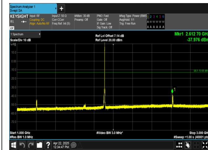
Band2-5MHz-QPSK-19175-1RB#24-1000~3000-PASS
