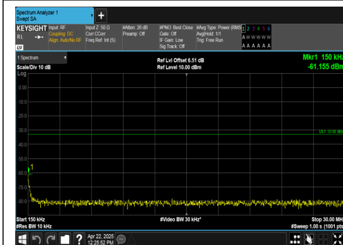
Band2-5MHz-QPSK-18900-1RB#0-0.15~30-PASS
