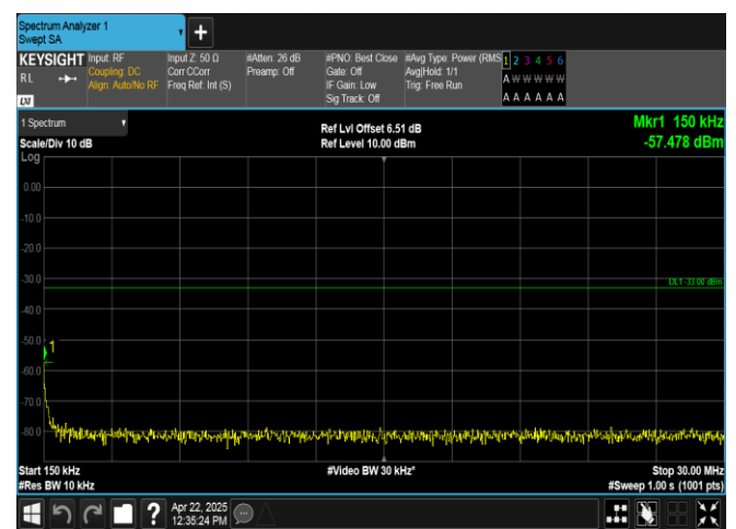
Band2-5MHz-16QAM-19175-1RB#24-0.15~30-PASS
