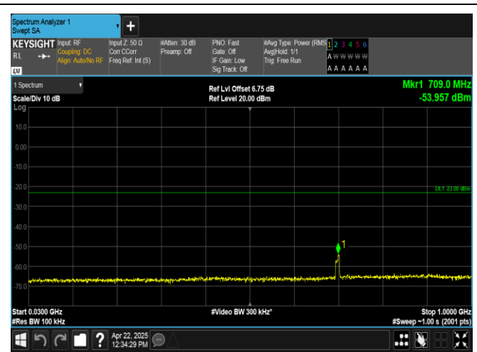
Band2-5MHz-QPSK-19175-1RB#24-30~1000-PASS
