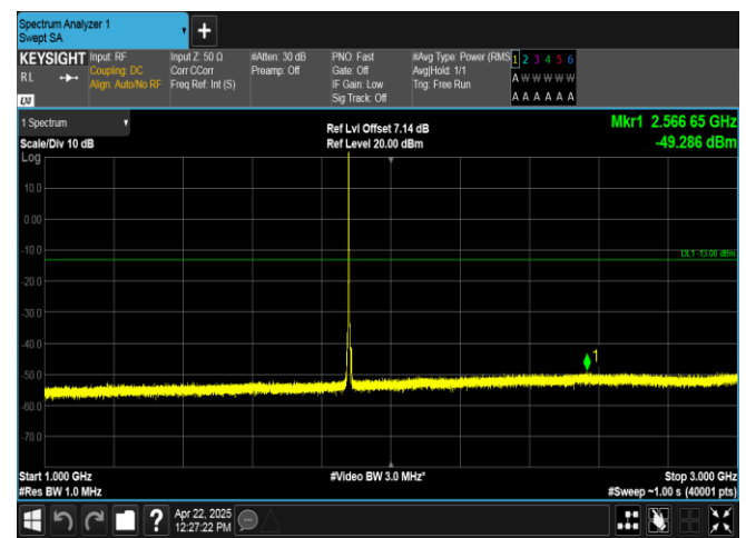
Band2-5MHz-16QAM-18900-1RB#0-1000~3000-PASS
