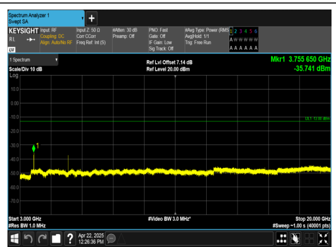
Band2-5MHz-QPSK-18900-1RB#0-3000~20000-PASS
