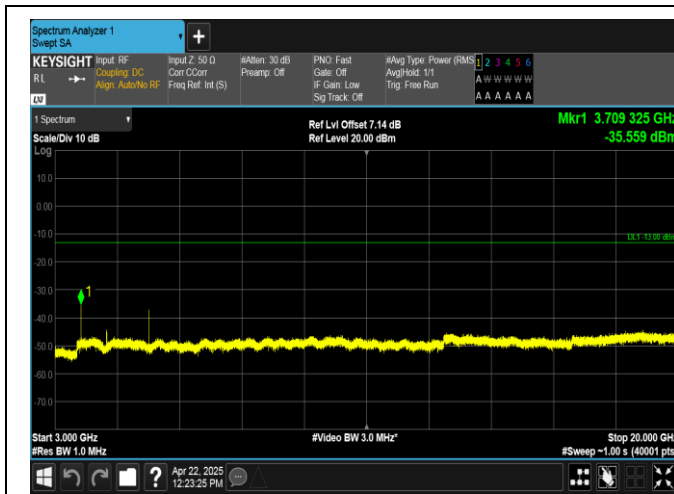
Band2-5MHz-16QAM-18625-1RB#24-3000~20000-PASS
