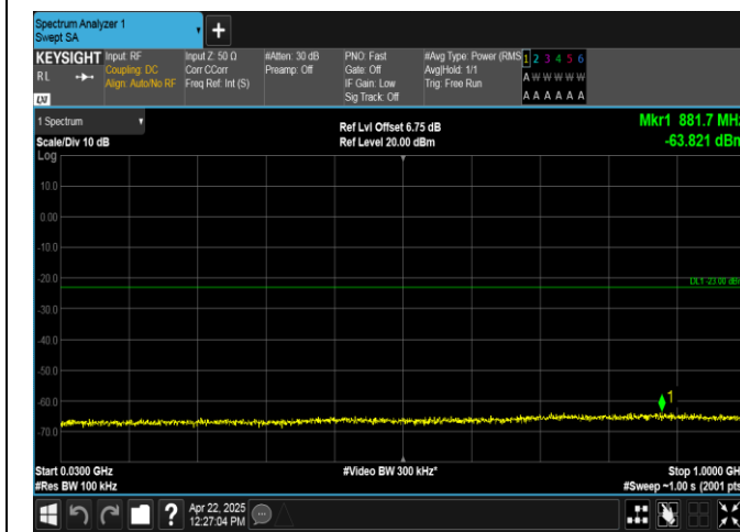
Band2-5MHz-16QAM-18900-1RB#0-30~1000-PASS
