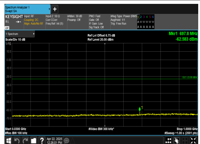
Band2-5MHz-QPSK-18900-1RB#0-30~1000-PASS
