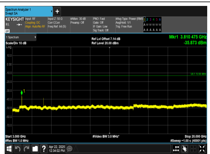
Band2-5MHz-16QAM-19175-1RB#0-3000~20000-PASS
