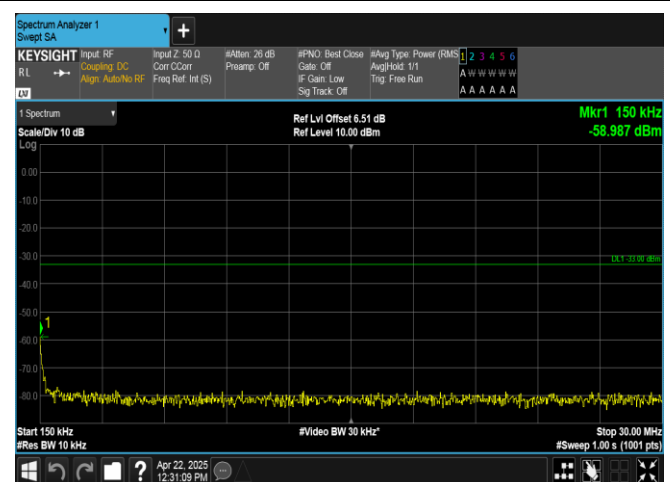
Band2-5MHz-16QAM-18900-25RB#0-0.15~30-PASS
