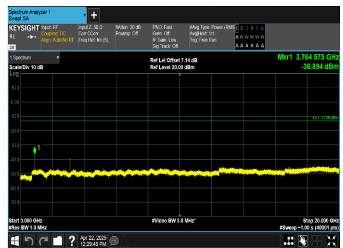
Band2-5MHz-16QAM-18900-1RB#24-3000~20000-PASS
