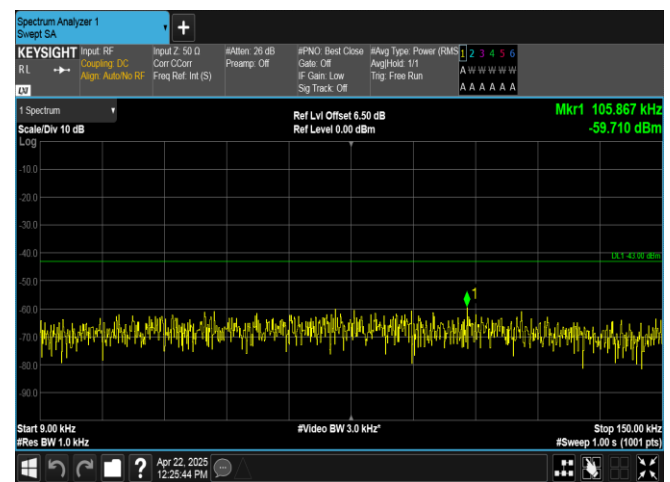
Band2-5MHz-QPSK-18900-1RB#0-0.009~0.15-PASS
