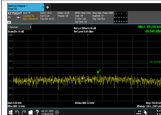
Band2-5MHz-QPSK-19175-25RB#0-0.009~0.15-PASS
