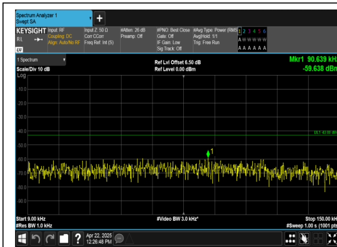
Band2-5MHz-16QAM-18900-1RB#0-0.009~0.15-PASS
