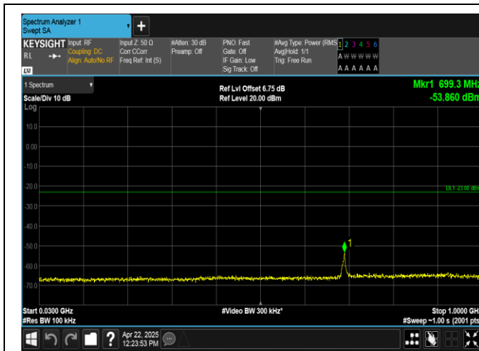
Band2-5MHz-QPSK-18625-25RB#0-30~1000-PASS
