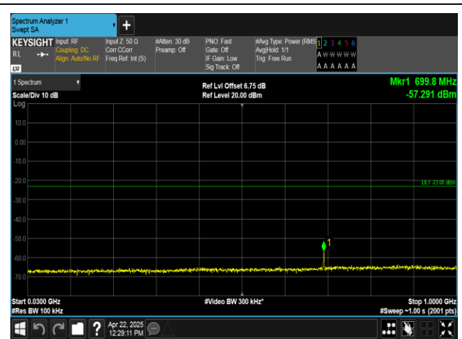
Band2-5MHz-16QAM-18900-1RB#24-30~1000-PASS
