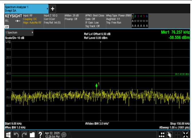
Band2-5MHz-16QAM-18900-1RB#24-0.009~0.15-PASS
