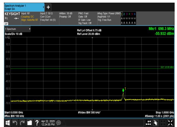
Band2-5MHz-16QAM-18625-25RB#0-30~1000-PASS
