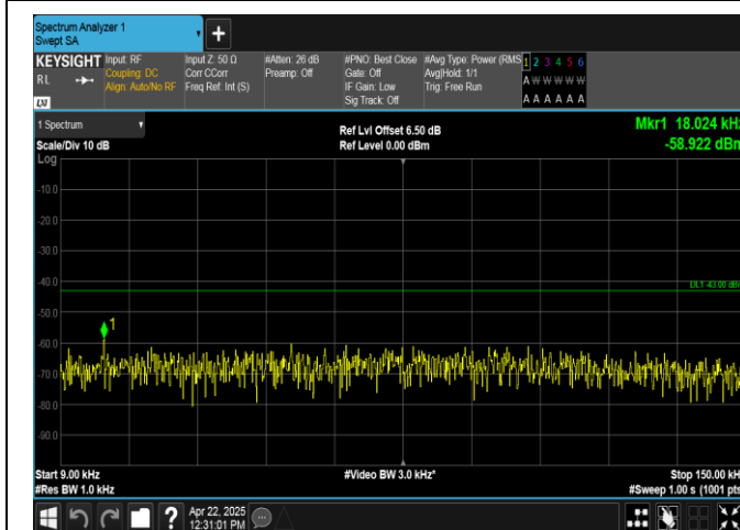
Band2-5MHz-16QAM-18900-25RB#0-0.009~0.15-PASS
