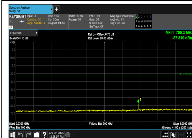
Band2-5MHz-QPSK-18900-1RB#24-30~1000-PASS
