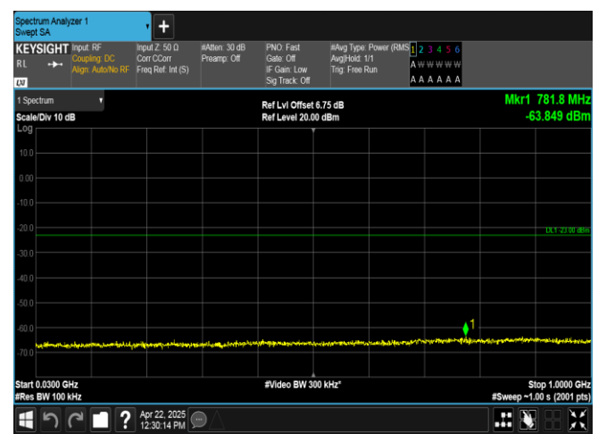
Band2-5MHz-QPSK-18900-25RB#0-30~1000-PASS
