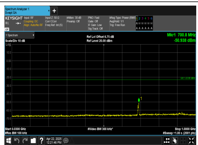
Band2-5MHz-QPSK-18625-1RB#24-30~1000-PASS
