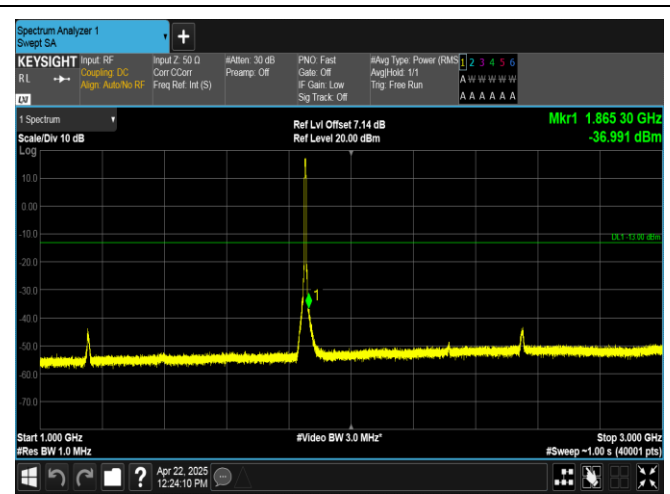
Band2-5MHz-QPSK-18625-25RB#0-1000~3000-PASS
