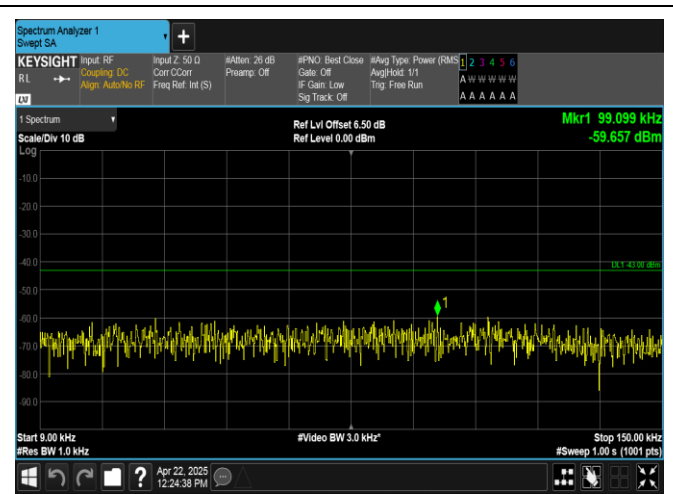
Band2-5MHz-16QAM-18625-25RB#0-0.009~0.15-PASS
