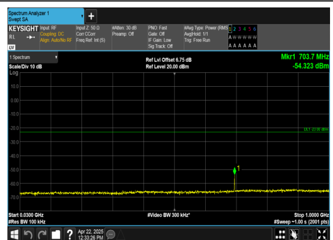
Band2-5MHz-16QAM-19175-1RB#0-30~1000-PASS
