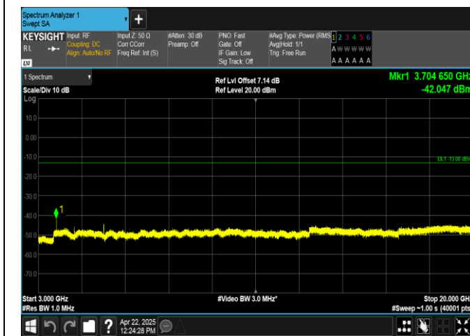
Band2-5MHz-QPSK-18625-25RB#0-3000~20000-PASS
