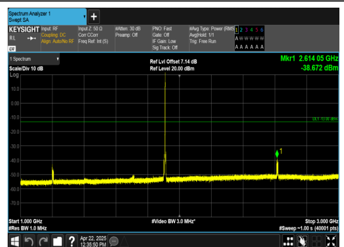
Band2-5MHz-16QAM-19175-1RB#24-1000~3000-PASS
