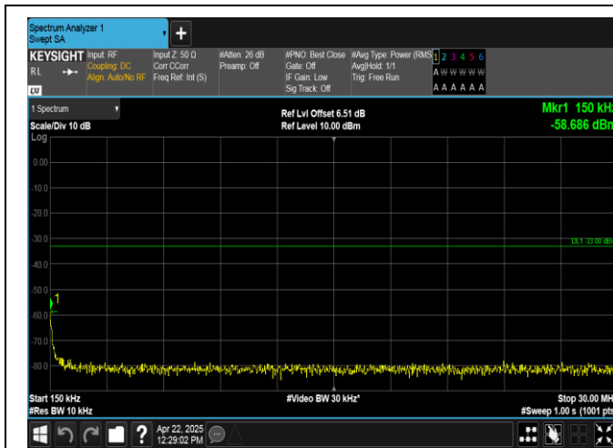
Band2-5MHz-16QAM-18900-1RB#24-0.15~30-PASS
