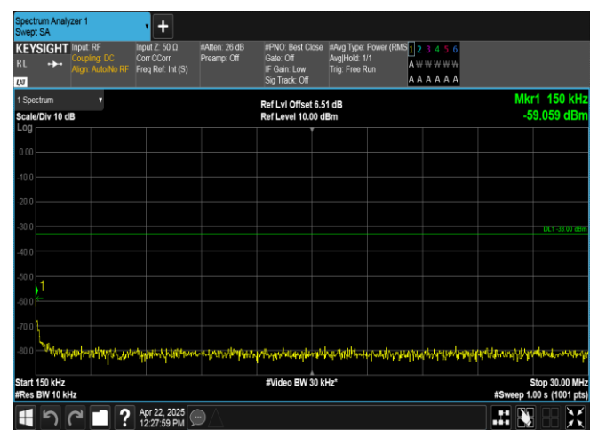
Band2-5MHz-QPSK-18900-1RB#24-0.15~30-PASS
