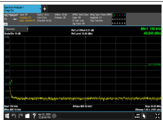
Band2-5MHz-16QAM-18900-1RB#0-0.15~30-PASS
