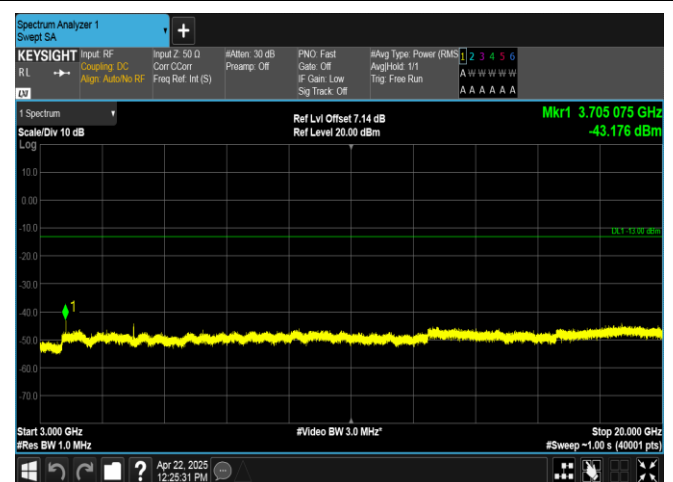
Band2-5MHz-16QAM-18625-25RB#0-3000~20000-PASS
