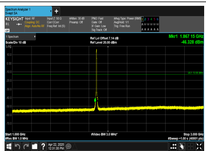
Band2-5MHz-16QAM-18900-25RB#0-1000~3000-PASS
