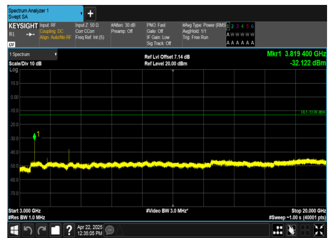
Band2-5MHz-QPSK-19175-1RB#24-3000~20000-PASS
