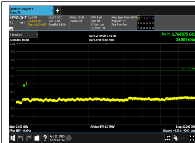
Band2-5MHz-QPSK-18900-1RB#24-3000~20000-PASS
