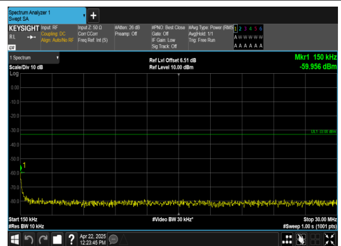
Band2-5MHz-QPSK-18625-25RB#0-0.15~30-PASS
