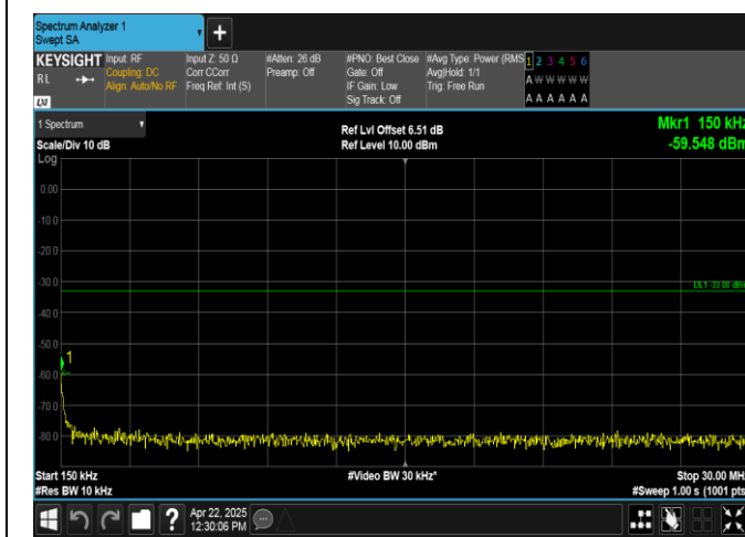
Band2-5MHz-QPSK-18900-25RB#0-0.15~30-PASS
