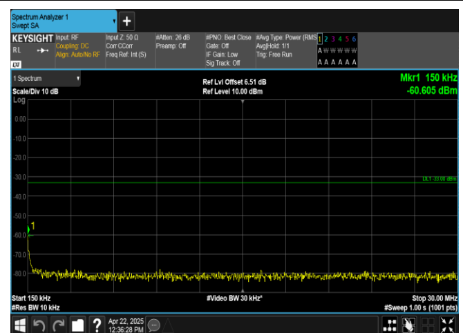
Band2-5MHz-QPSK-19175-25RB#0-0.15~30-PASS
