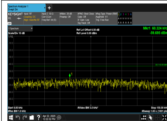
Band2-5MHz-16QAM-18625-1RB#24-0.009~0.15-PASS
