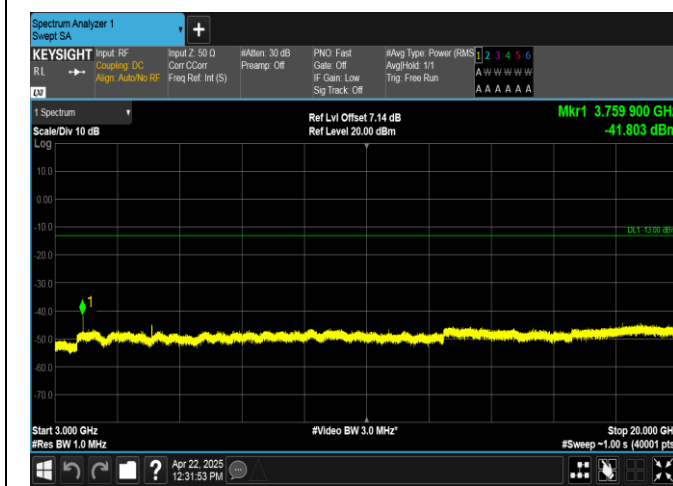
Band2-5MHz-16QAM-18900-25RB#0-3000~20000-PASS
