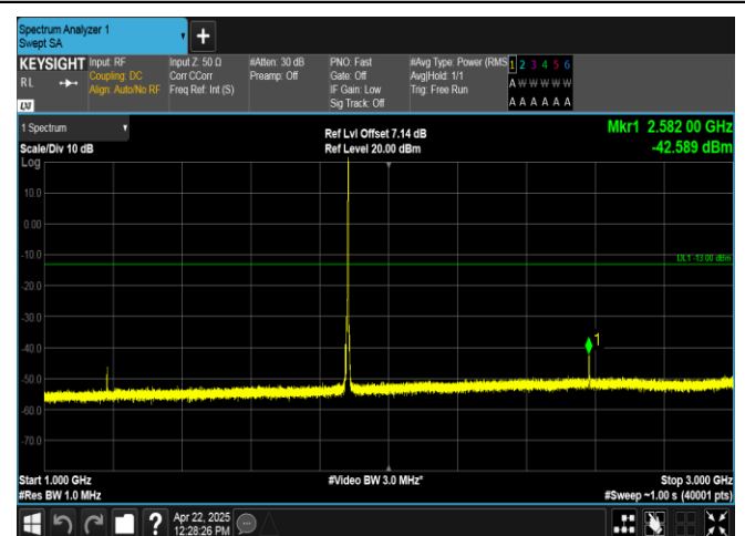
Band2-5MHz-QPSK-18900-1RB#24-1000~3000-PASS
