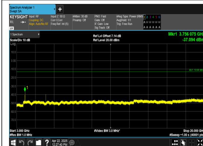
Band2-5MHz-16QAM-18900-1RB#0-3000~20000-PASS
