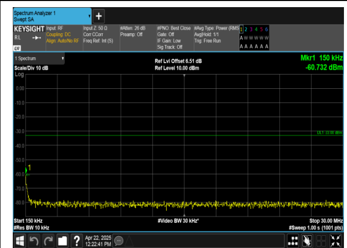
Band2-5MHz-16QAM-18625-1RB#24-0.15~30-PASS
