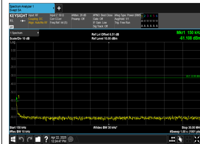
Band2-5MHz-16QAM-18625-25RB#0-0.15~30-PASS
