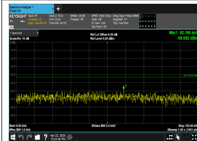
Band2-5MHz-QPSK-18625-25RB#0-0.009~0.15-PASS
