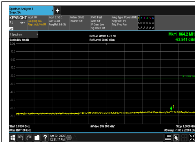
Band2-5MHz-16QAM-18900-25RB#0-30~1000-PASS
