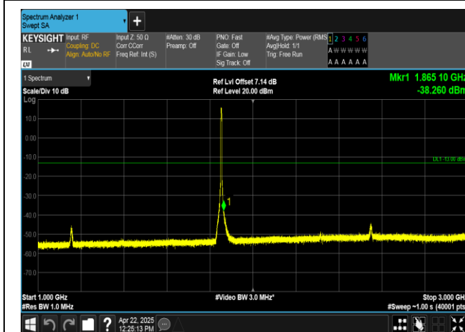
Band2-5MHz-16QAM-18625-25RB#0-1000~3000-PASS
