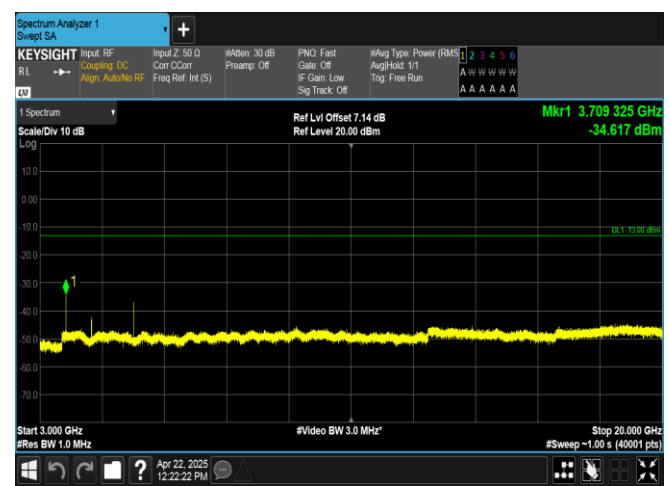
Band2-5MHz-QPSK-18625-1RB#24-3000~20000-PASS
