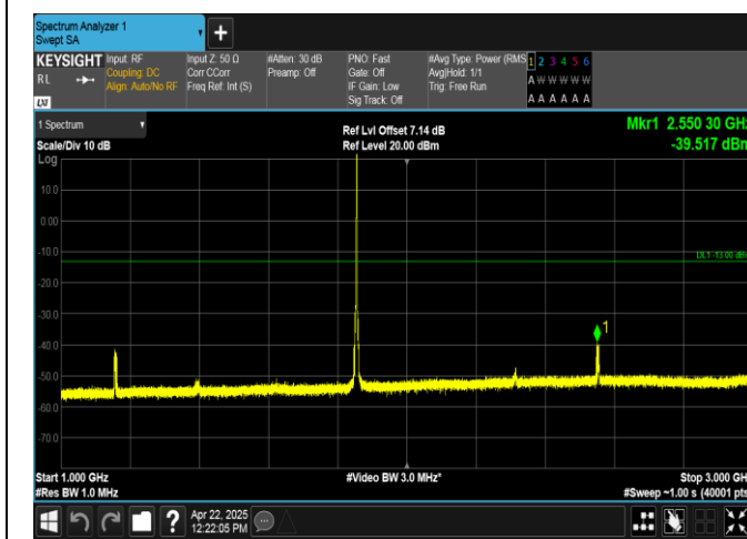
Band2-5MHz-QPSK-18625-1RB#24-1000~3000-PASS
