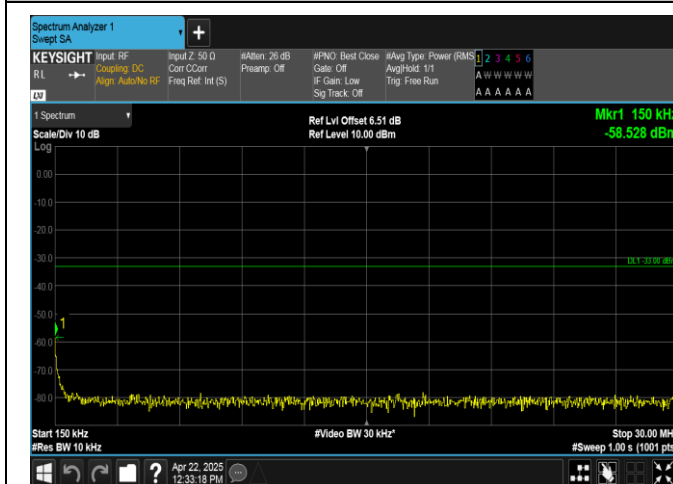
Band2-5MHz-16QAM-19175-1RB#0-0.15~30-PASS
