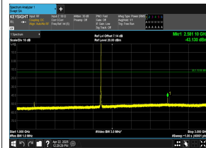
Band2-5MHz-16QAM-18900-1RB#24-1000~3000-PASS
