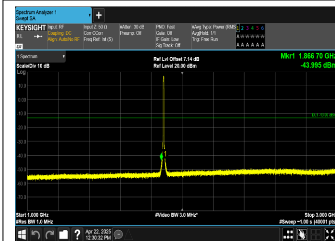
Band2-5MHz-QPSK-18900-25RB#0-1000~3000-PASS
