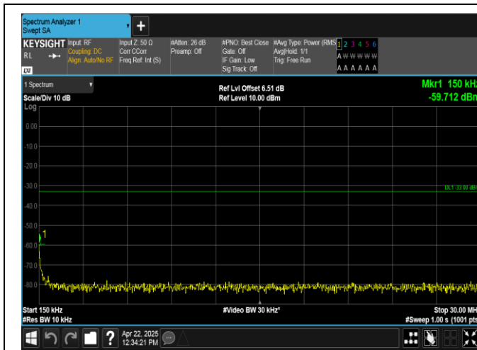
Band2-5MHz-QPSK-19175-1RB#24-0.15~30-PASS
