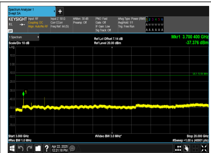
Band2-5MHz-16QAM-18625-1RB#0-3000~20000-PASS
