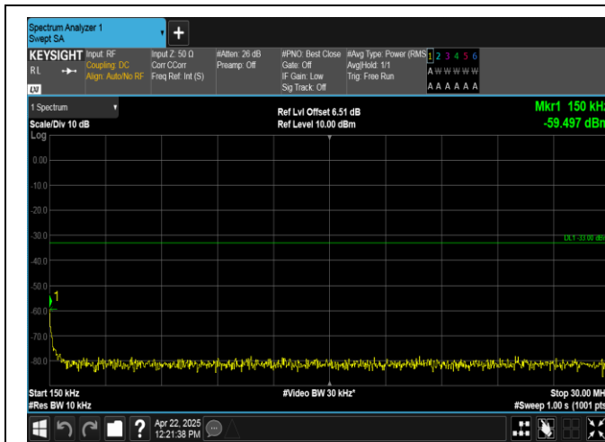
Band2-5MHz-QPSK-18625-1RB#24-0.15~30-PASS
