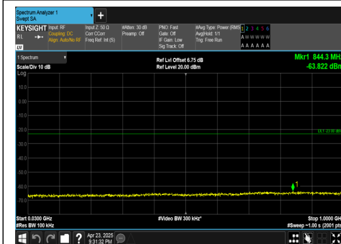
Band25-3MHz-16QAM-26675-1RB#14-30~1000-PASS
