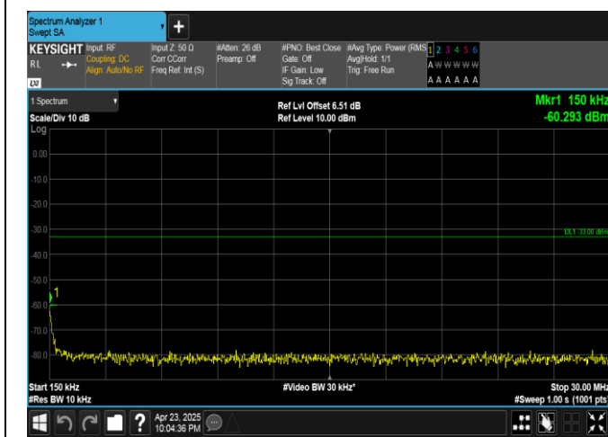
Band25-5MHz-16QAM-26065-25RB#0-0.15~30-PASS
