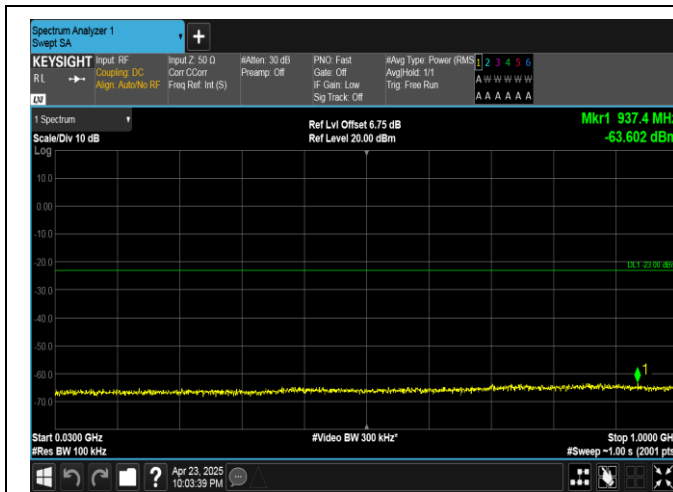
Band25-5MHz-QPSK-26065-25RB#0-30~1000-PASS
