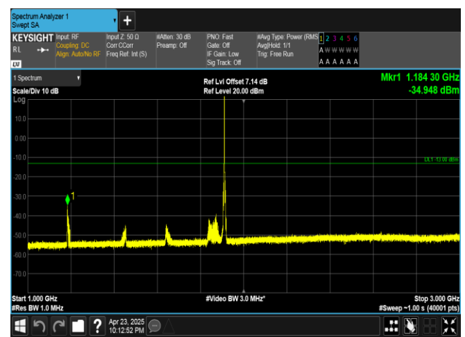
Band25-5MHz-QPSK-26665-1RB#0-1000~3000-PASS
