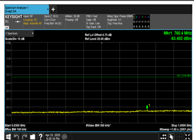
Band25-3MHz-16QAM-26675-1RB#0-30~1000-PASS
