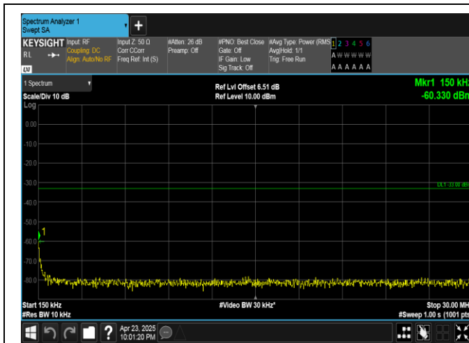
Band25-5MHz-QPSK-26065-1RB#24-0.15~30-PASS
