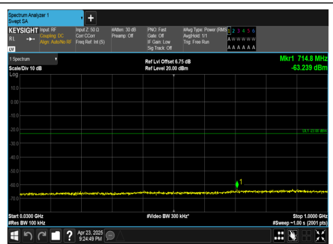
Band25-3MHz-16QAM-26365-1RB#14-30~1000-PASS
