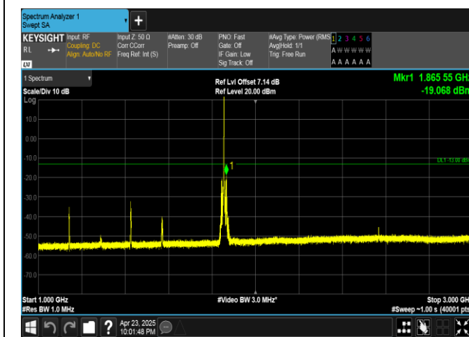
Band25-5MHz-QPSK-26065-1RB#24-1000~3000-PASS
