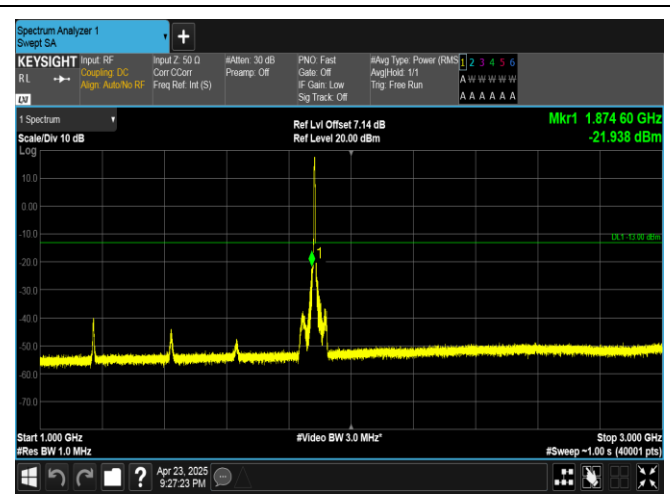
Band25-3MHz-16QAM-26365-15RB#0-1000~3000-PASS
