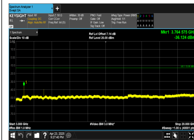
Band25-3MHz-16QAM-26365-15RB#0-3000~20000-PASS
