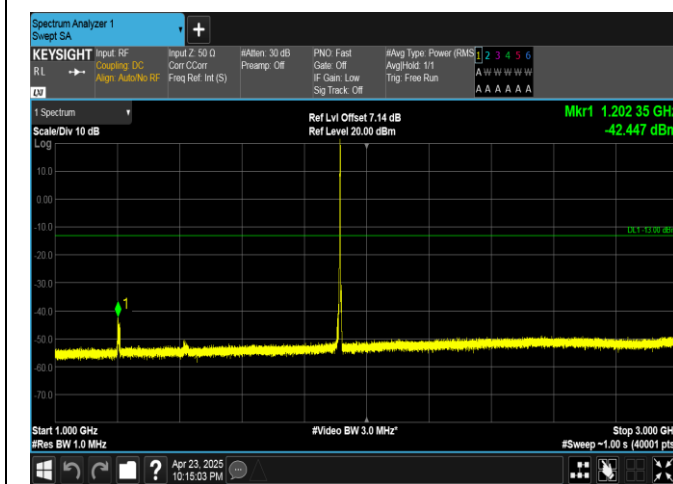
Band25-5MHz-QPSK-26665-1RB#24-1000~3000-PASS
