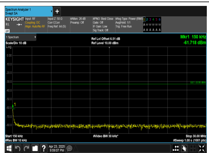
Band25-5MHz-QPSK-26065-1RB#0-0.15~30-PASS
