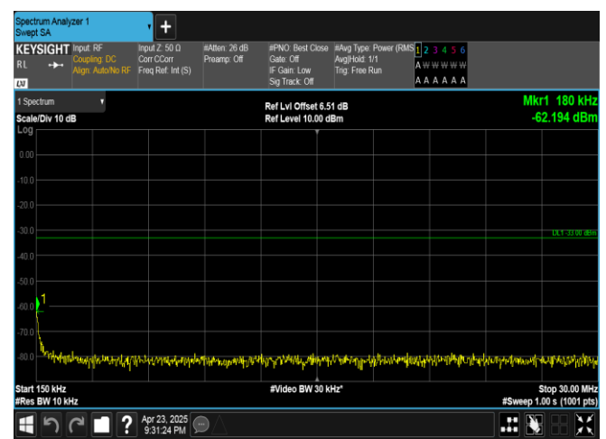
Band25-3MHz-16QAM-26675-1RB#14-0.15~30-PASS
