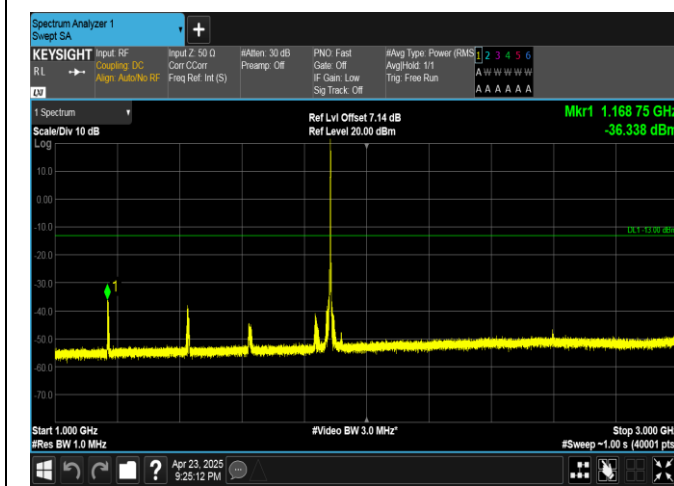
Band25-3MHz-16QAM-26365-1RB#14-1000~3000-PASS
