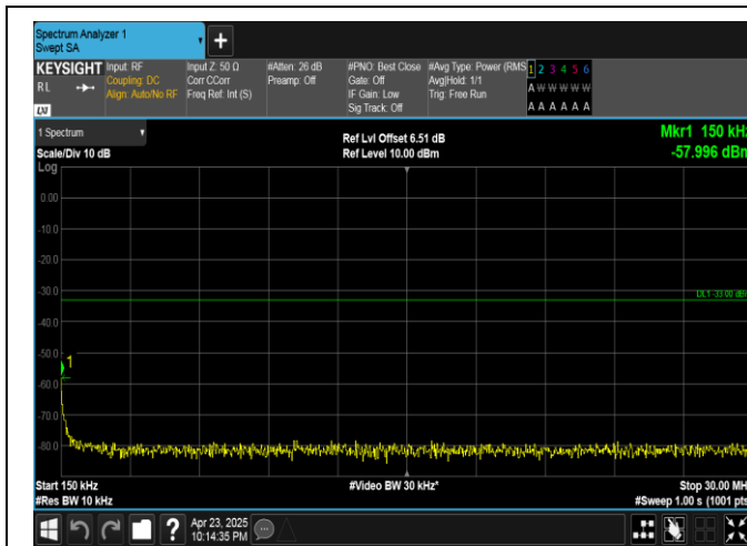
Band25-5MHz-QPSK-26665-1RB#24-0.15~30-PASS
