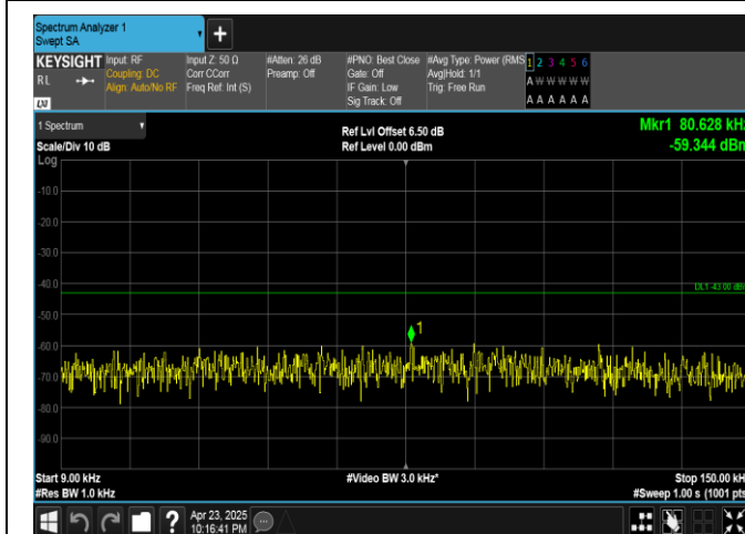
Band25-5MHz-QPSK-26665-25RB#0-0.009~0.15-PASS
