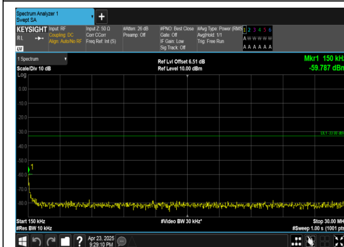
Band25-3MHz-16QAM-26675-1RB#0-0.15~30-PASS
