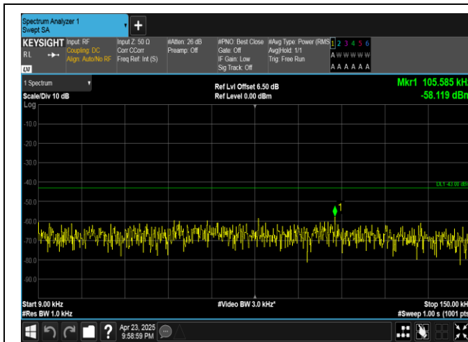
Band25-5MHz-QPSK-26065-1RB#0-0.009~0.15-PASS
