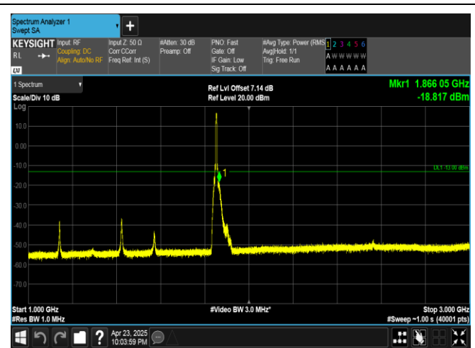
Band25-5MHz-QPSK-26065-25RB#0-1000~3000-PASS
