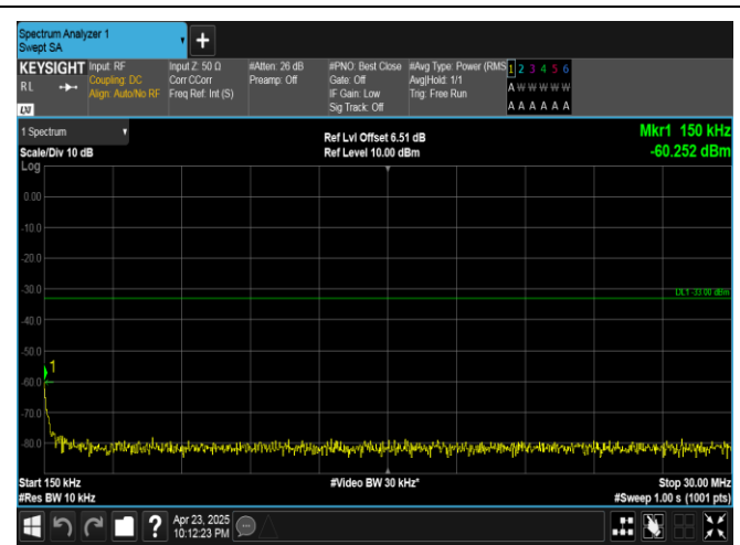
Band25-5MHz-QPSK-26665-1RB#0-0.15~30-PASS
