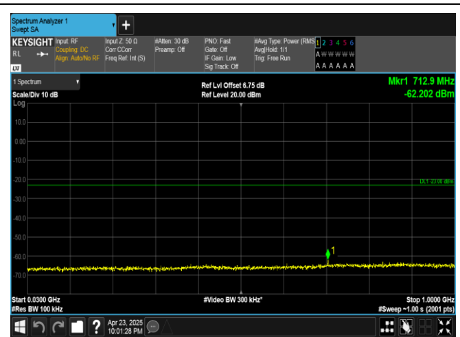
Band25-5MHz-QPSK-26065-1RB#24-30~1000-PASS
