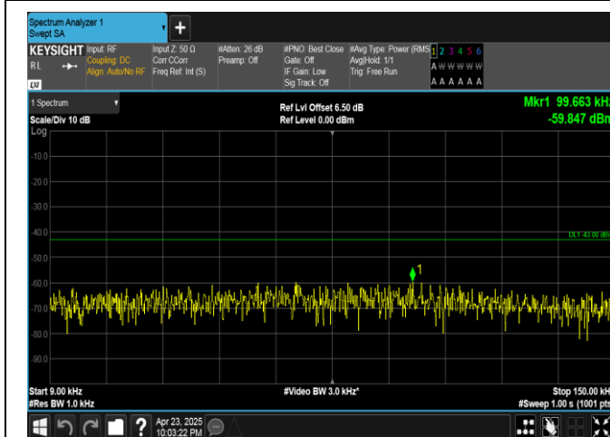
Band25-5MHz-QPSK-26065-25RB#0-0.009~0.15-PASS
