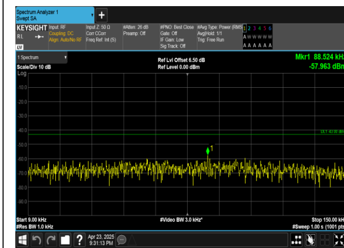
Band25-3MHz-16QAM-26675-1RB#14-0.009~0.15-PASS
