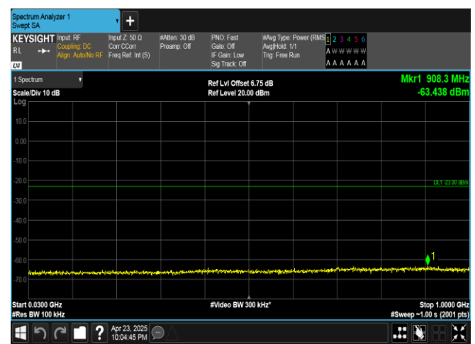
Band25-5MHz-16QAM-26065-25RB#0-30~1000-PASS
