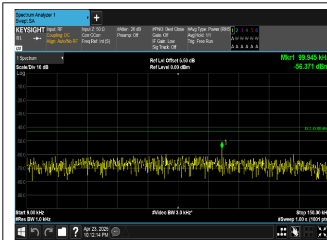
Band25-5MHz-QPSK-26665-1RB#0-0.009~0.15-PASS
