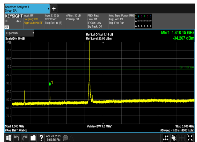
Band25-5MHz-QPSK-26065-1RB#0-1000~3000-PASS
