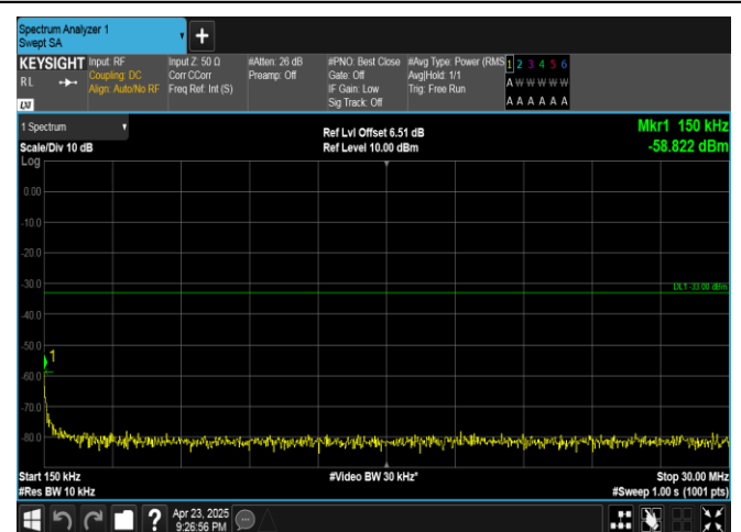
Band25-3MHz-16QAM-26365-15RB#0-0.15~30-PASS
