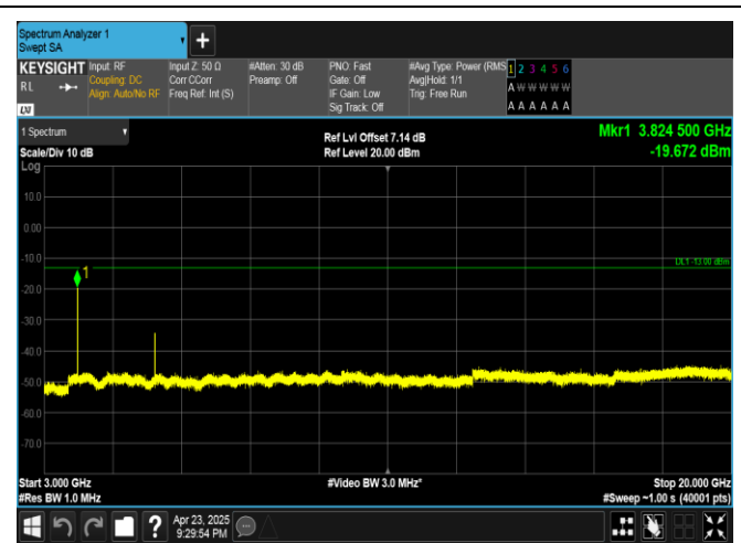
Band25-3MHz-16QAM-26675-1RB#0-3000~20000-PASS
