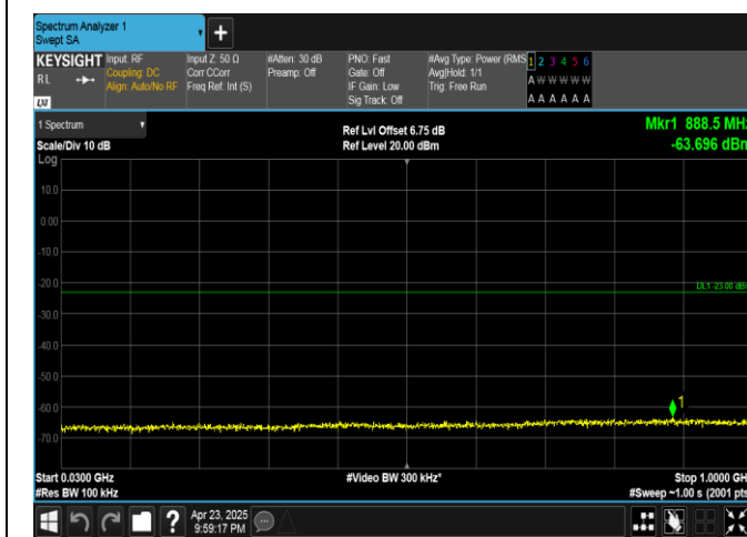
Band25-5MHz-QPSK-26065-1RB#0-30~1000-PASS
