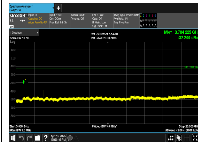
Band25-5MHz-QPSK-26065-25RB#0-3000~20000-PASS
