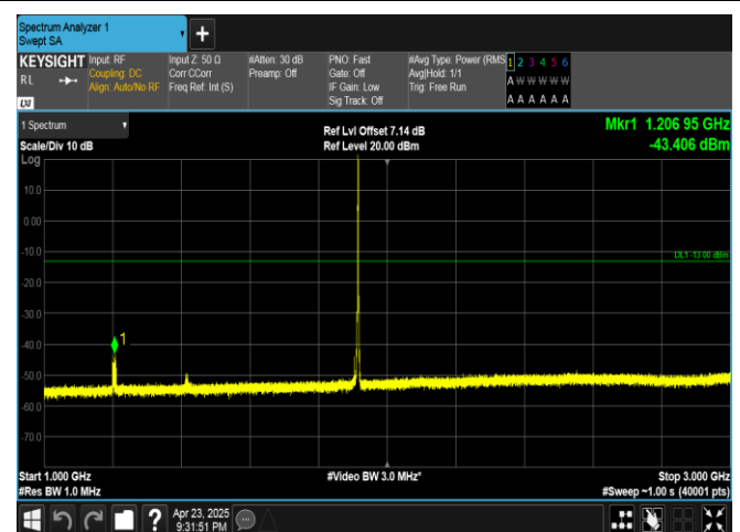
Band25-3MHz-16QAM-26675-1RB#14-1000~3000-PASS
