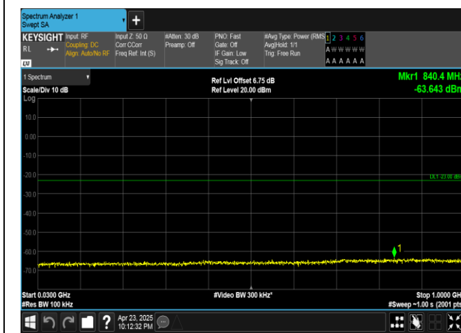
Band25-5MHz-QPSK-26665-1RB#0-30~1000-PASS
