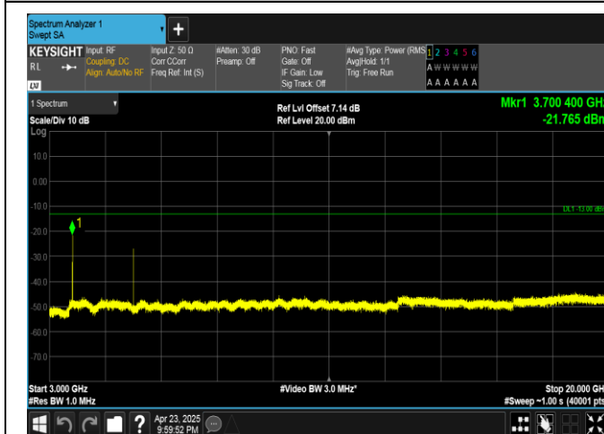
Band25-5MHz-QPSK-26065-1RB#0-3000~20000-PASS
