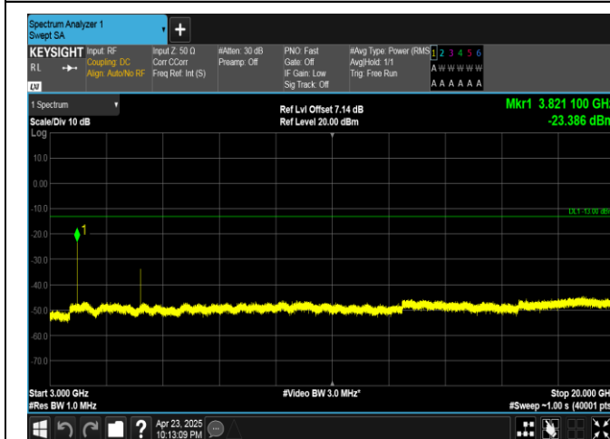
Band25-5MHz-QPSK-26665-1RB#0-3000~20000-PASS
