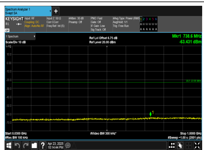
Band25-5MHz-QPSK-26665-1RB#24-30~1000-PASS
