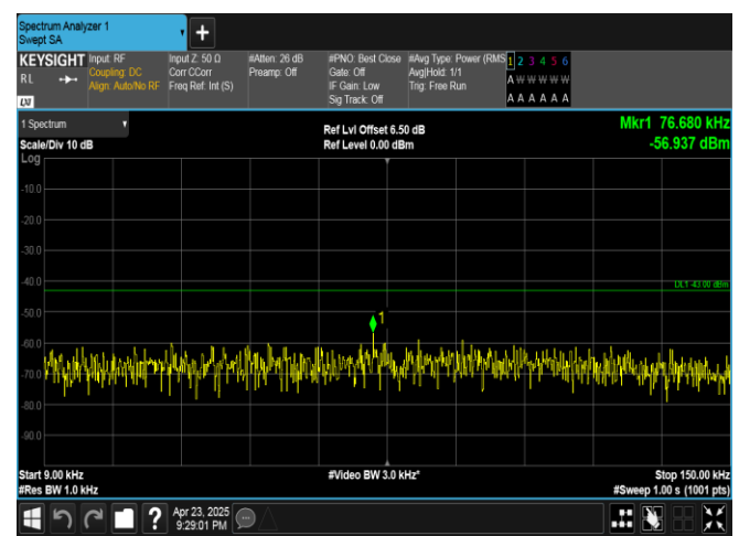
Band25-3MHz-16QAM-26675-1RB#0-0.009~0.15-PASS
