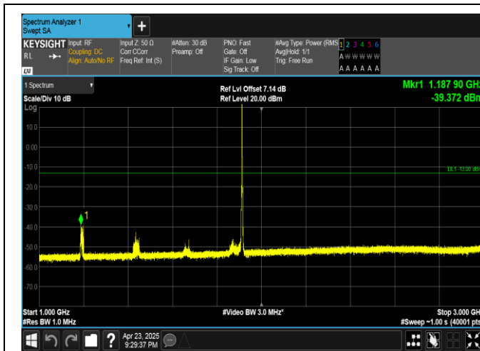
Band25-3MHz-16QAM-26675-1RB#0-1000~3000-PASS
