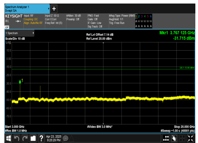
Band25-3MHz-16QAM-26365-1RB#14-3000~20000-PASS
