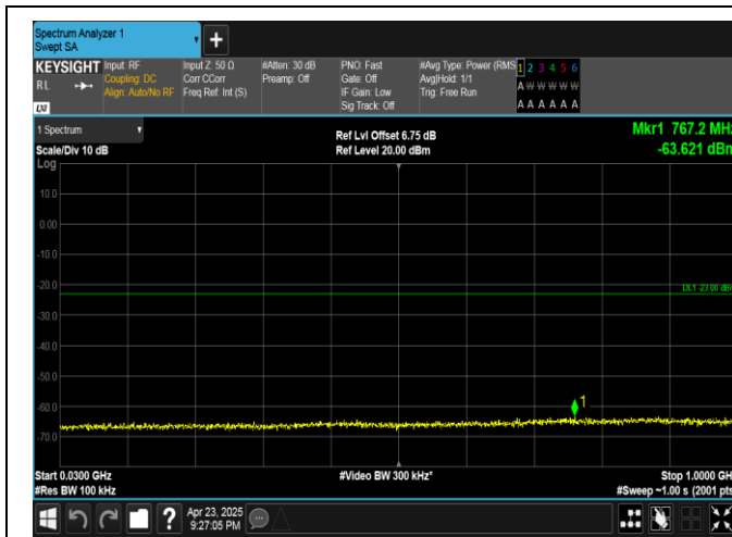
Band25-3MHz-16QAM-26365-15RB#0-30~1000-PASS
