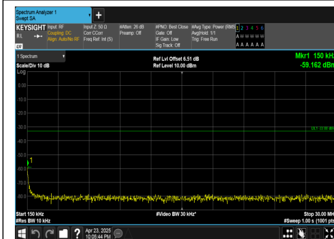
Band25-5MHz-QPSK-26365-1RB#0-0.15~30-PASS
