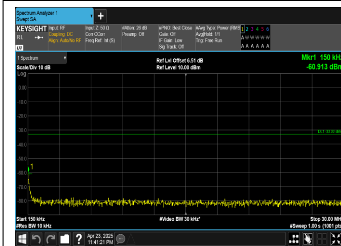
Band25-15MHz-16QAM-26115-75RB#0-0.15~30-PASS
