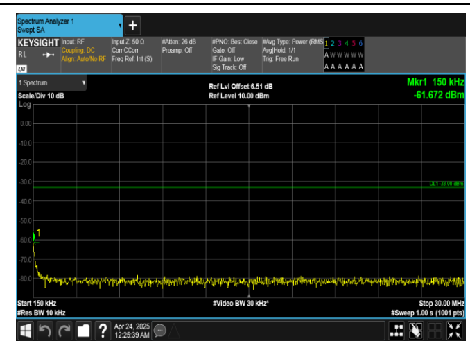
Band25-20MHz-QPSK-26140-1RB#0-0.15~30-PASS
