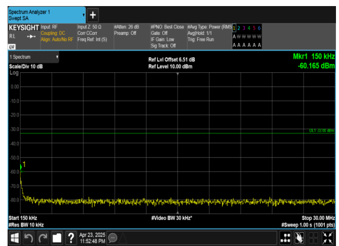
Band25-15MHz-16QAM-26615-1RB#74-0.15~30-PASS
