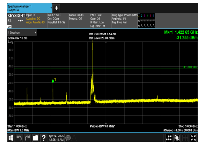
Band25-20MHz-QPSK-26140-1RB#0-1000~3000-PASS
