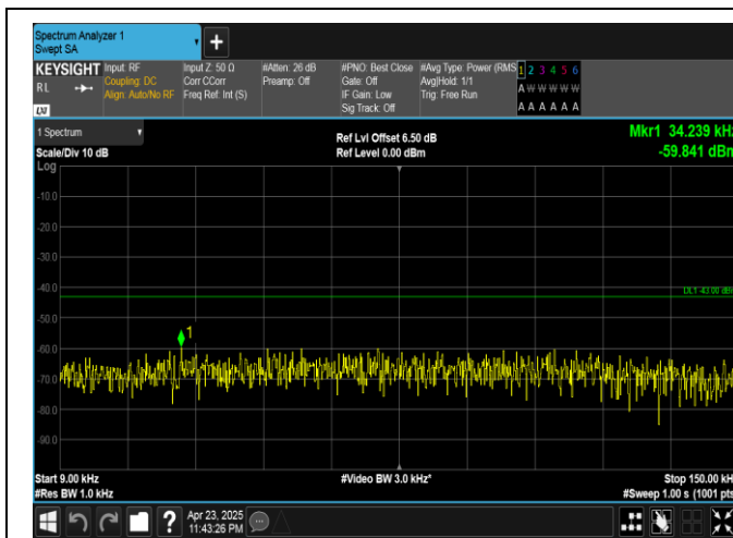
Band25-15MHz-16QAM-26365-1RB#0-0.009~0.15-PASS
