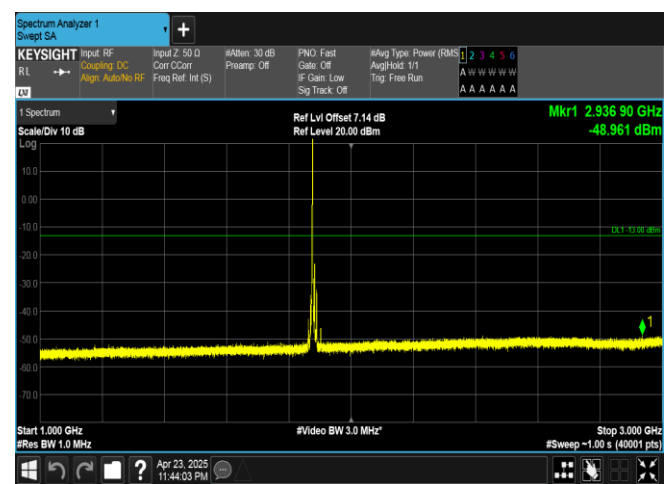
Band25-15MHz-16QAM-26365-1RB#0-1000~3000-PASS
