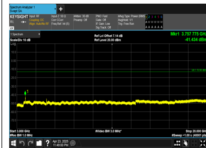
Band25-15MHz-16QAM-26365-75RB#0-3000~20000-PASS
