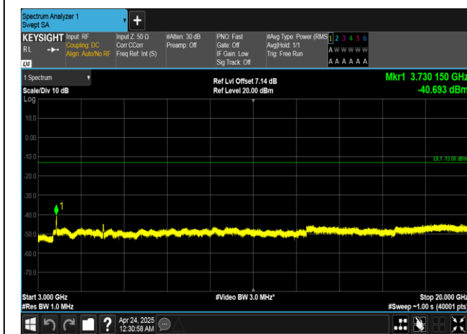
Band25-20MHz-QPSK-26140-100RB#0-3000~20000-PASS
