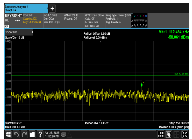
Band25-15MHz-16QAM-26615-1RB#0-0.009~0.15-PASS
