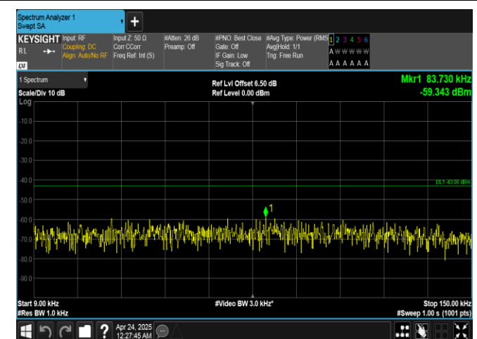
Band25-20MHz-QPSK-26140-1RB#99-0.009~0.15-PASS
