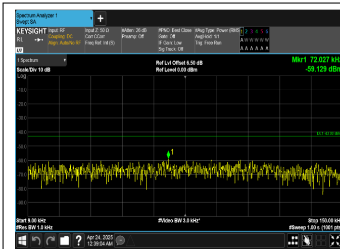
Band25-20MHz-QPSK-26590-1RB#0-0.009~0.15-PASS
