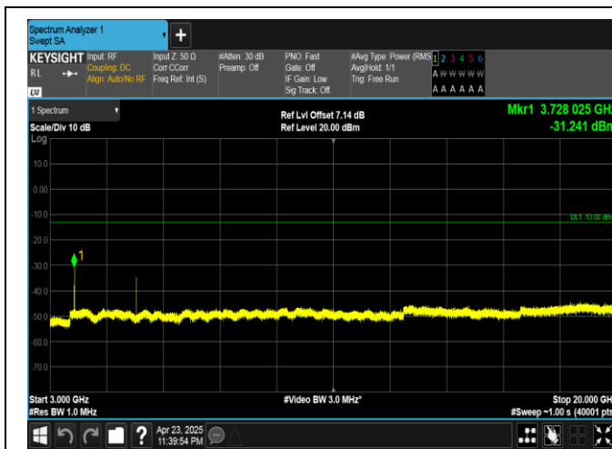
Band25-15MHz-16QAM-26115-1RB#74-3000~20000-PASS
