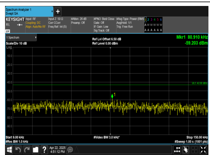
Band4-3MHz-16QAM-20385-1RB#0-0.009~0.15-PASS
