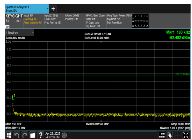
Band4-3MHz-QPSK-20385-1RB#0-0.15~30-PASS
