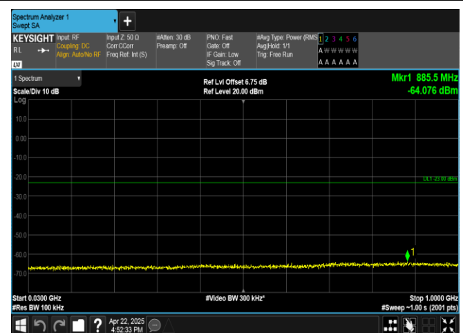
Band4-3MHz-QPSK-20385-1RB#14-30~1000-PASS
