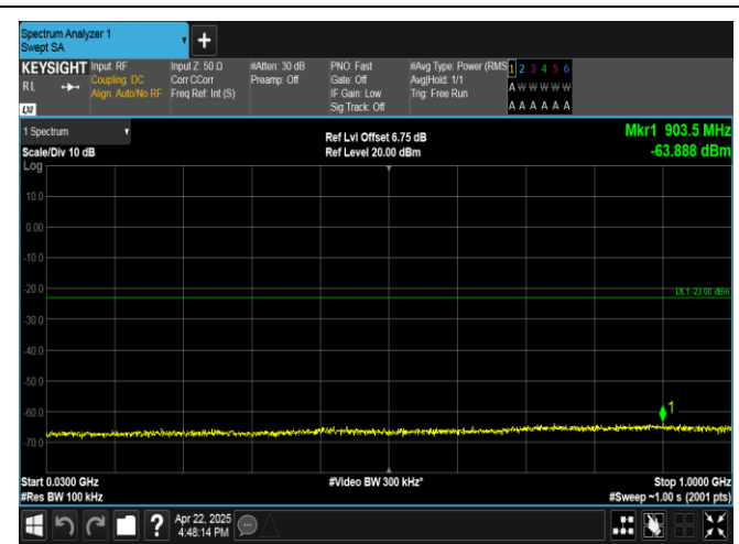
Band4-3MHz-QPSK-20175-15RB#0-30~1000-PASS
