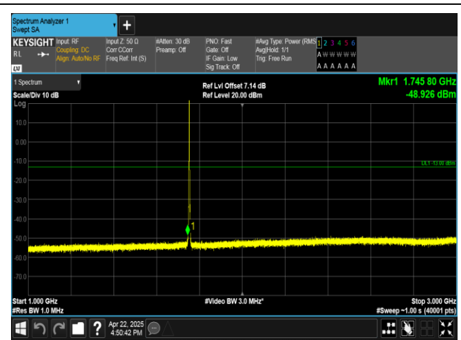
Band4-3MHz-QPSK-20385-1RB#0-1000~3000-PASS
