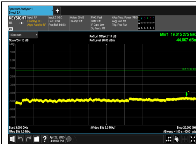
Band4-3MHz-16QAM-20175-15RB#0-3000~20000-PASS
