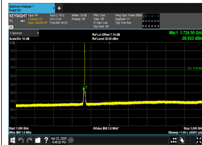
Band4-3MHz-QPSK-20175-15RB#0-1000~3000-PASS
