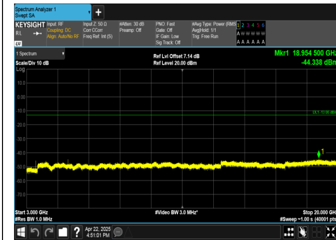
Band4-3MHz-QPSK-20385-1RB#0-3000~20000-PASS
