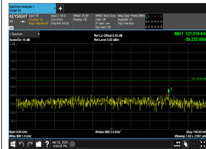
Band4-3MHz-QPSK-20385-15RB#0-0.009~0.15-PASS
