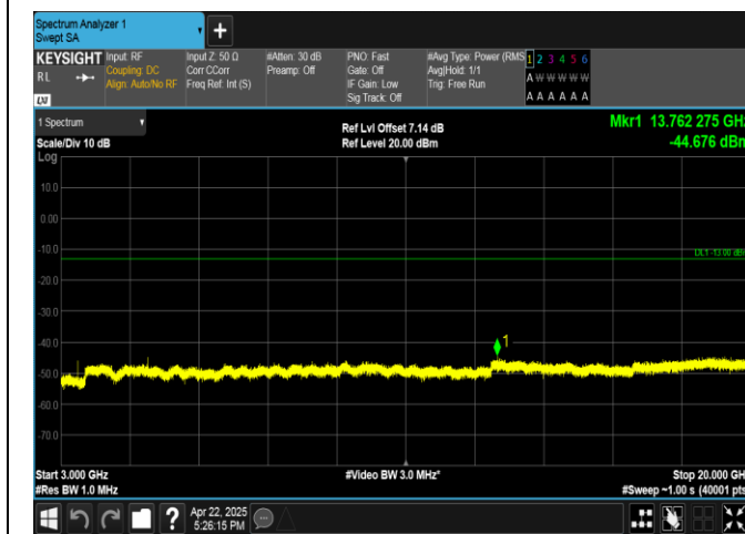
Band4-5MHz-QPSK-19975-1RB#0-3000~20000-PASS
