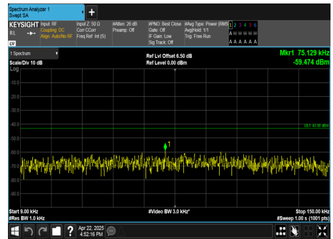
Band4-3MHz-QPSK-20385-1RB#14-0.009~0.15-PASS
