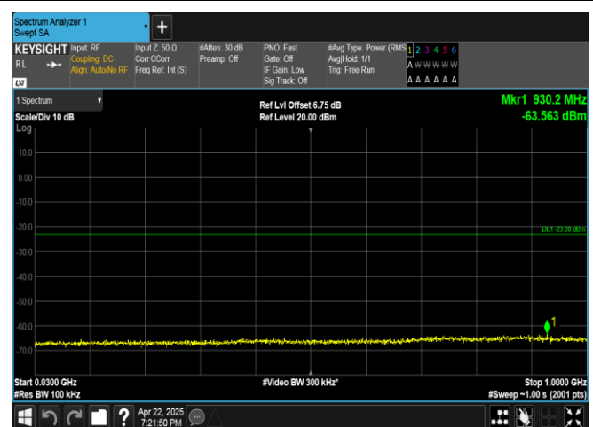
Band4-15MHz-QPSK-20325-1RB#74-30~1000-PASS
