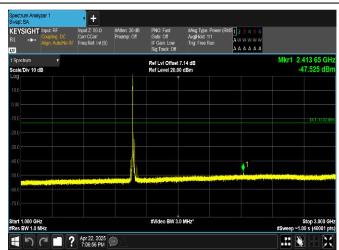
Band4-15MHz-QPSK-20025-1RB#0-1000~3000-PASS
