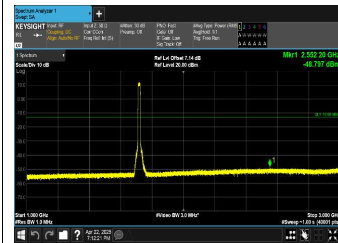
Band4-15MHz-16QAM-20025-75RB#0-1000~3000-PASS
