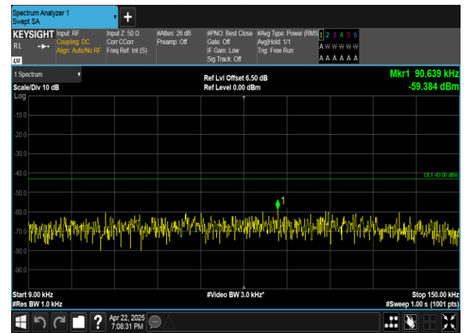
Band4-15MHz-QPSK-20025-1RB#74-0.009~0.15-PASS
