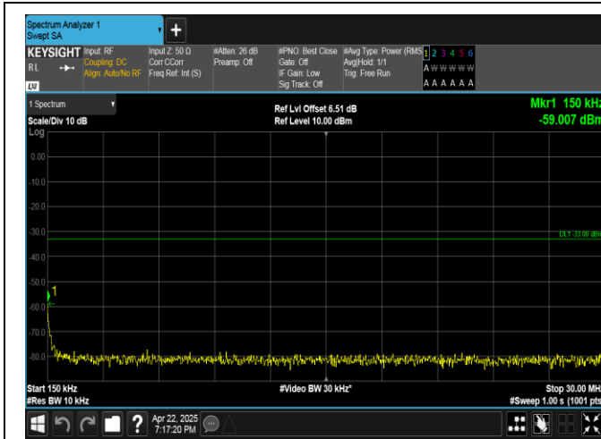
Band4-15MHz-QPSK-20175-75RB#0-0.15~30-PASS
