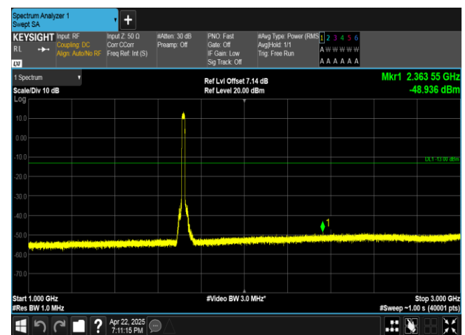
Band4-15MHz-QPSK-2025-75RB#0-1000~3000-PASS
