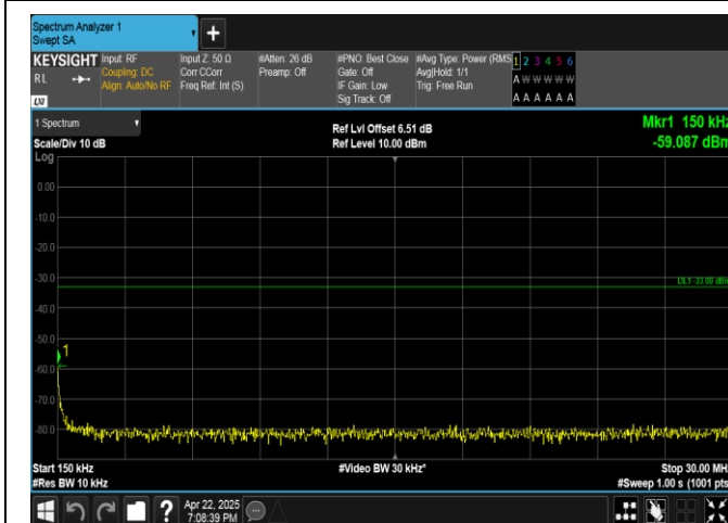
Band4-15MHz-QPSK-20025-1RB#74-0.15~30-PASS
