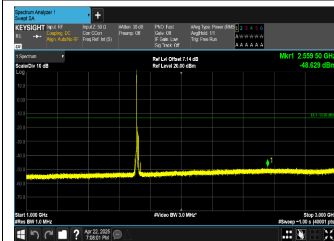
Band4-15MHz-16QAM-20025-1RB#0-1000~3000-PASS
