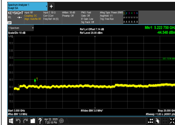
Band4-15MHz-QPSK-20325-1RB#0-3000~20000-PASS
