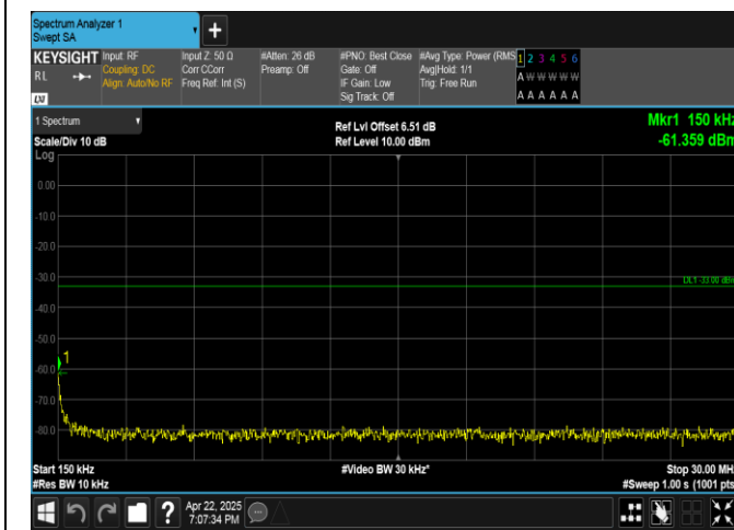
Band4-15MHz-16QAM-20025-1RB#0-0.15~30-PASS
