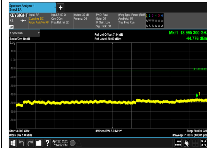
Band4-15MHz-16QAM-20175-1RB#0-3000~20000-PASS
