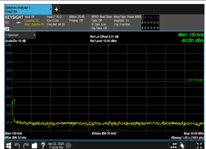
Band4-15MHz-QPSK-20325-1RB#0-0.15~30-PASS
