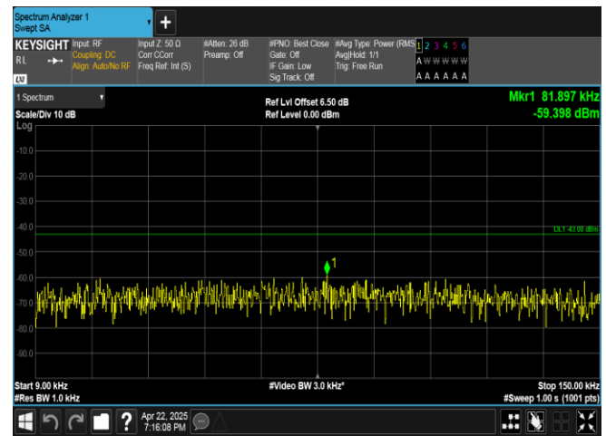
Band4-15MHz-16QAM-20175-1RB#74-0.009~0.15-PASS
