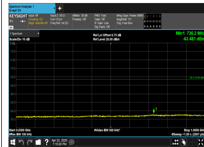
Band4-15MHz-QPSK-20175-1RB#74-30~1000-PASS
