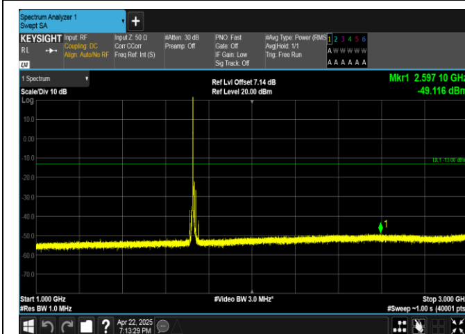
Band4-15MHz-QPSK-20175-1RB#0-1000~3000-PASS
