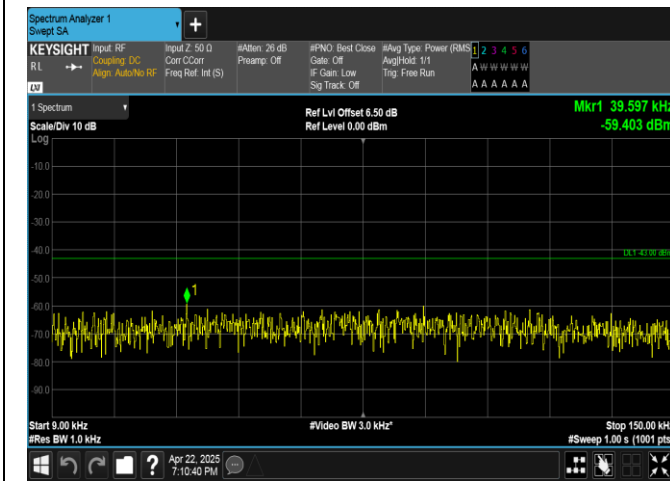
Band4-15MHz-QPSK-2025-75RB#0-0.009~0.15-PASS
