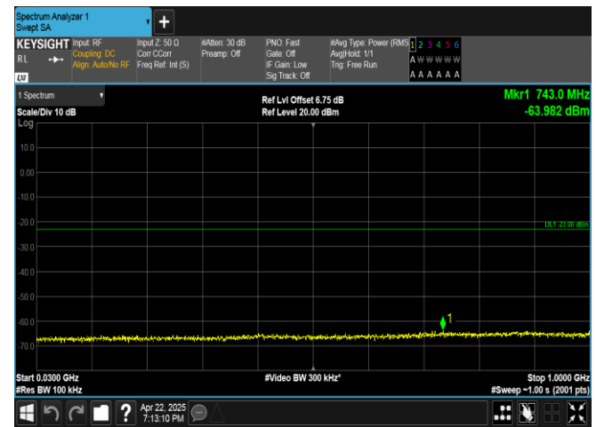
Band4-15MHz-QPSK-20175-1RB#0-30~1000-PASS
