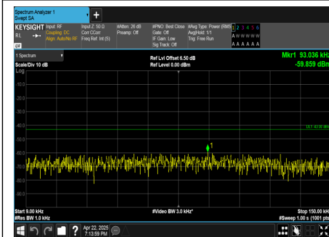
Band4-15MHz-16QAM-20175-1RB#0-0.009~0.15-PASS
