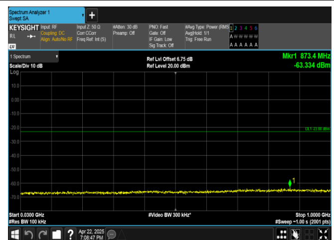
Band4-15MHz-QPSK-20025-1RB#74-30~1000-PASS
