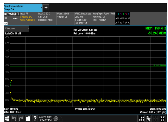
Band4-15MHz-16QAM-20175-1RB#0-0.15~30-PASS
