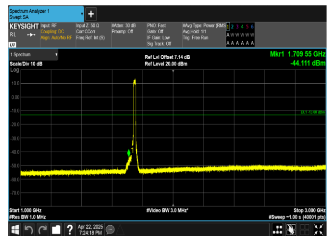
Band4-15MHz-QPSK-20325-75RB#0-1000~3000-PASS
