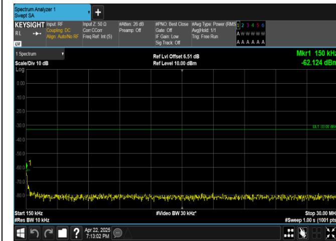
Band4-15MHz-QPSK-20175-1RB#0-0.15~30-PASS
