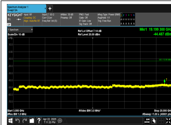
Band4-15MHz-QPSK-20025-75RB#0-3000~20000-PASS
