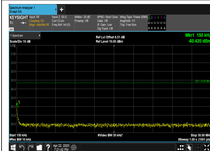
Band4-15MHz-QPSK-20325-1RB#74-0.15~30-PASS
