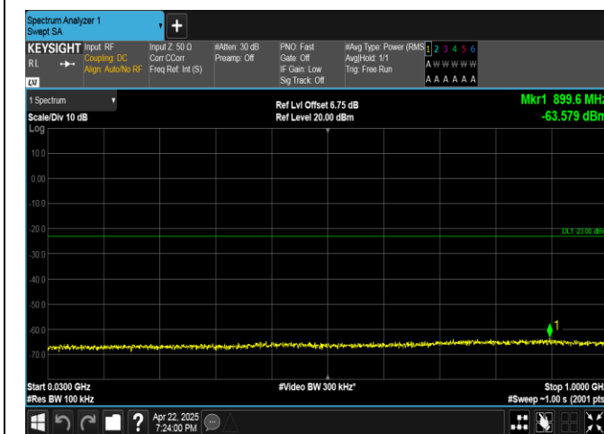
Band4-15MHz-QPSK-20325-75RB#0-30~1000-PASS
