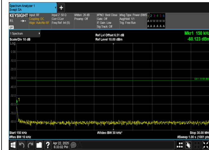
Band4-10MHz-16QAM-20350-1RB#0-0.15~30-PASS
