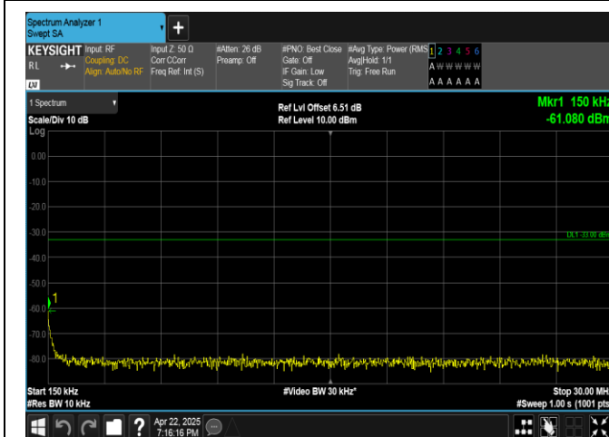
Band4-15MHz-16QAM-20175-1RB#74-0.15~30-PASS
