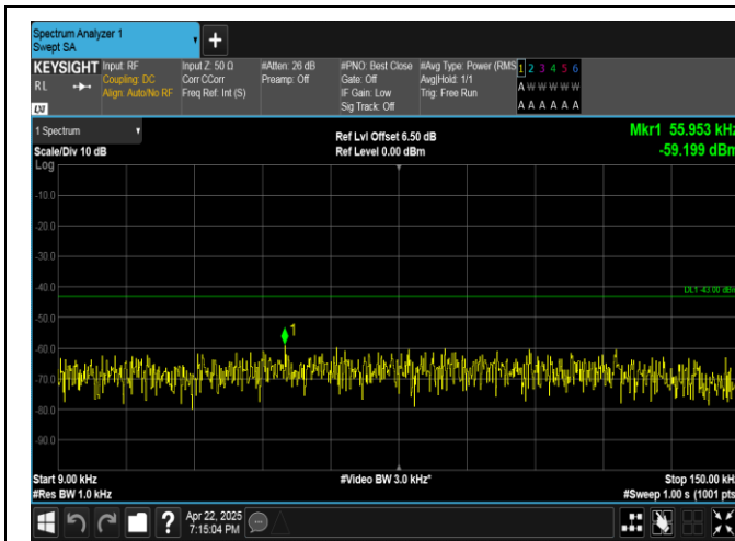
Band4-15MHz-QPSK-20175-1RB#74-0.009~0.15-PASS
