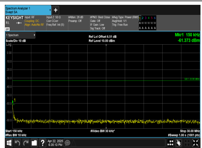
Band4-10MHz-16QAM-20350-1RB#49-0.15~30-PASS
