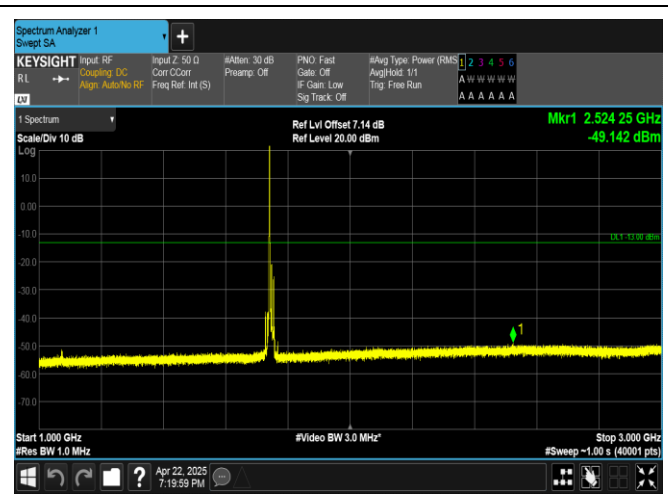
Band4-15MHz-QPSK-20325-1RB#0-1000~3000-PASS
