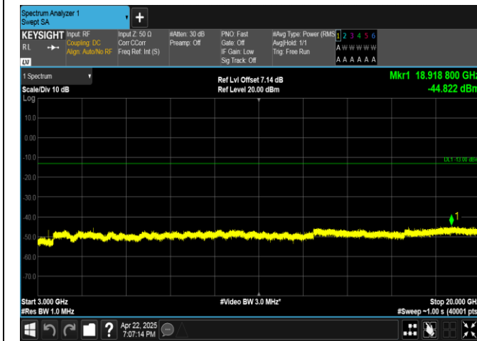
Band4-15MHz-QPSK-20025-1RB#0-3000~20000-PASS
