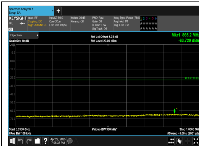
Band4-15MHz-QPSK-20025-1RB#0-30~1000-PASS
