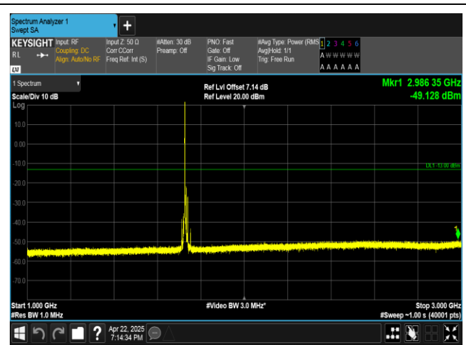
Band4-15MHz-16QAM-20175-1RB#0-1000~3000-PASS
