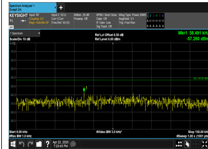
Band4-15MHz-QPSK-20325-75RB#0-0.009~0.15-PASS
