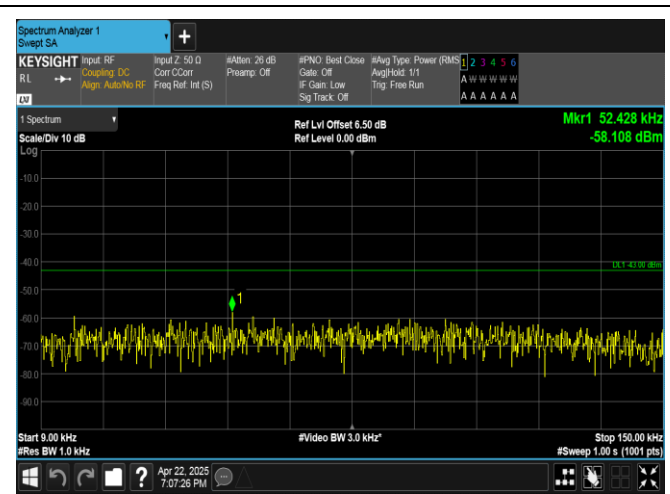
Band4-15MHz-16QAM-20025-1RB#0-0.009~0.15-PASS
