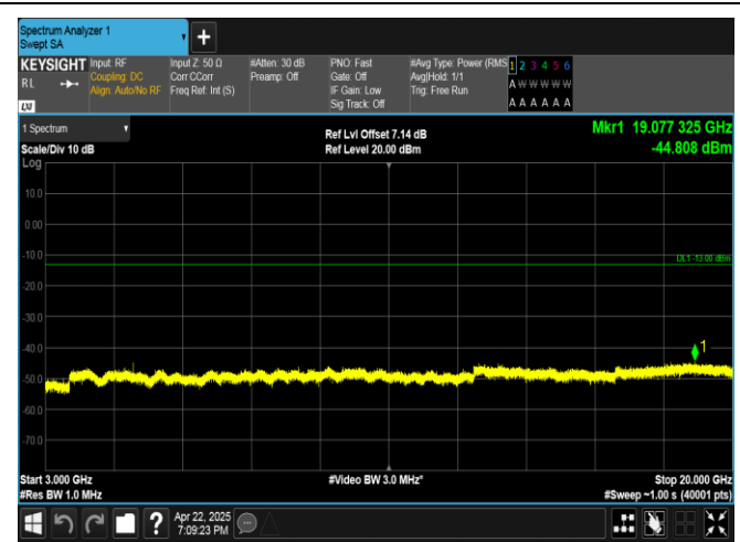
Band4-15MHz-QPSK-2025-1RB#74-3000~20000-PASS
