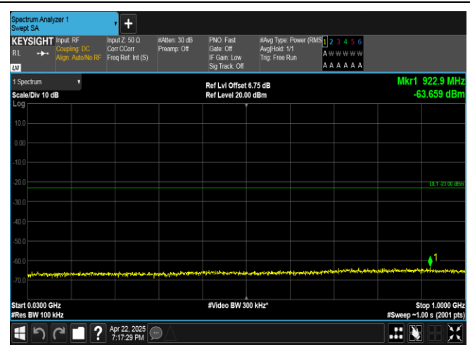
Band4-15MHz-QPSK-20175-75RB#0-30~1000-PASS
