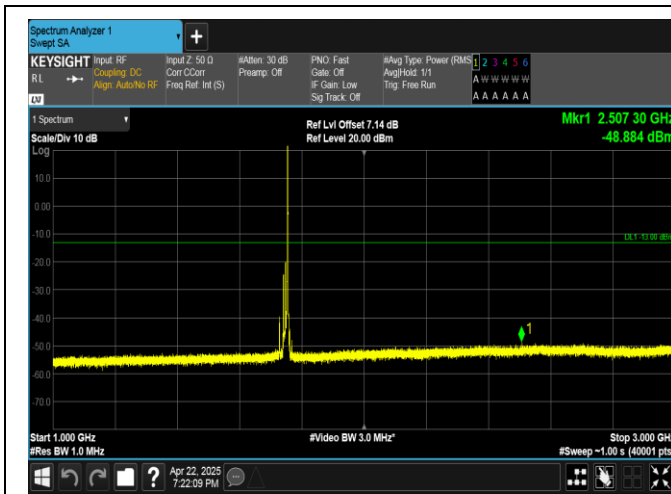
Band4-15MHz-QPSK-20325-1RB#74-1000~3000-PASS
