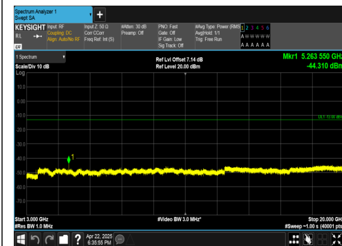
Band4-10MHz-16QAM-20350-1RB#49-3000~20000-PASS
