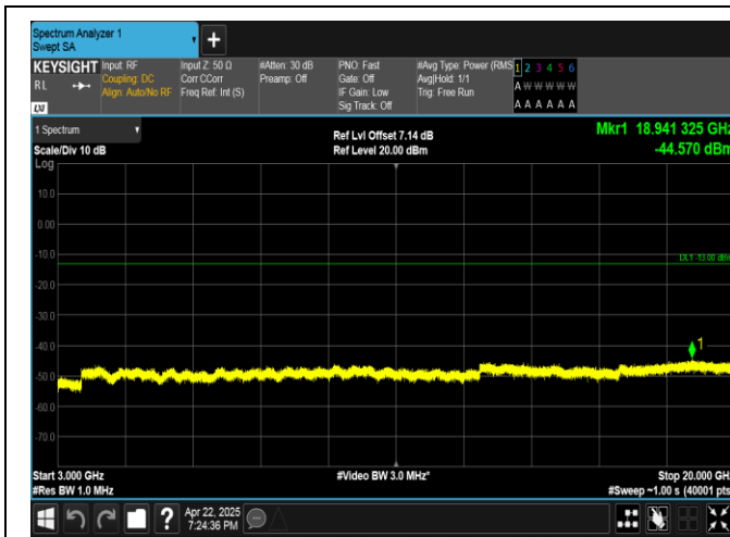
Band4-15MHz-QPSK-20325-75RB#0-3000~20000-PASS
