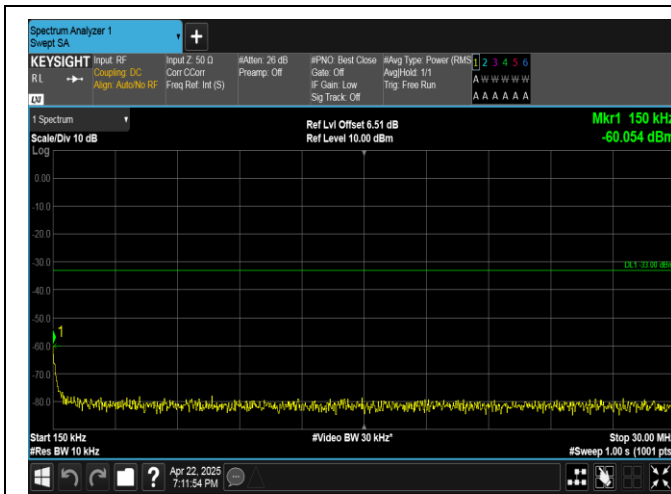
Band4-15MHz-16QAM-20025-75RB#0-0.15~30-PASS
