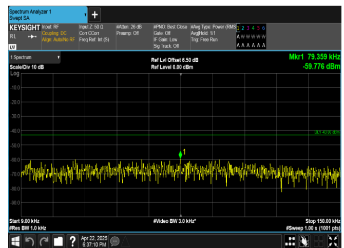
Band4-10MHz-16QAM-20350-50RB#0-0.009~0.15-PASS
