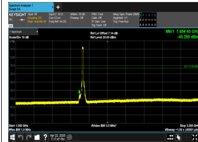
Band4-15MHz-QPSK-20175-75RB#0-1000~3000-PASS
