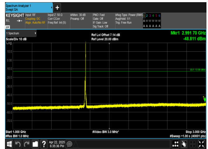
Band4-10MHz-16QAM-20350-1RB#49-1000~3000-PASS
