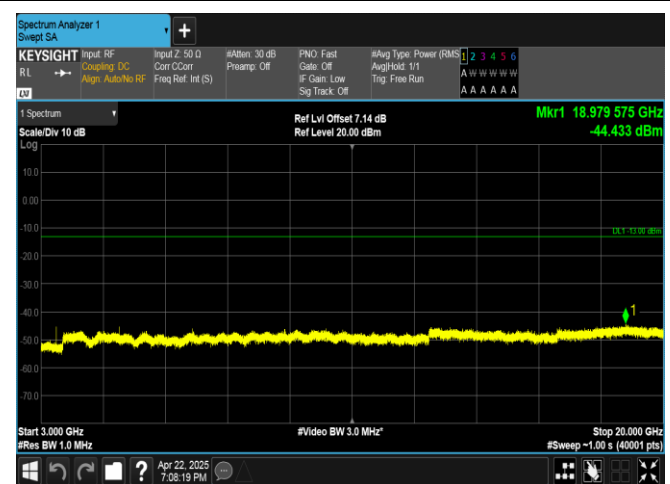
Band4-15MHz-16QAM-20025-1RB#0-3000~20000-PASS
