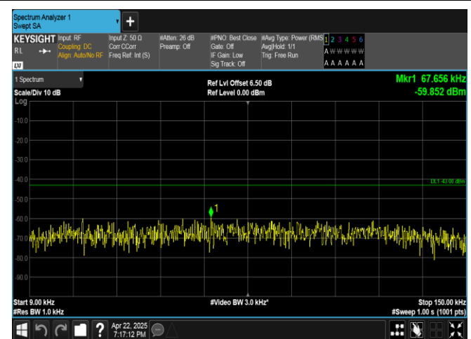
Band4-15MHz-QPSK-20175-75RB#0-0.009~0.15-PASS
