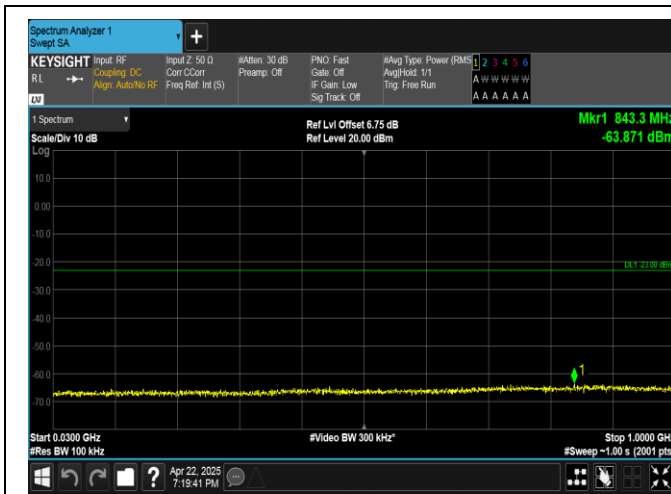
Band4-15MHz-QPSK-20325-1RB#0-30~1000-PASS
