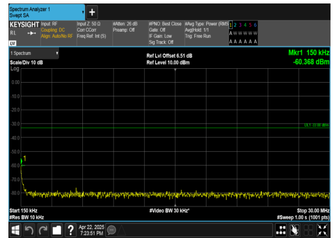
Band4-15MHz-QPSK-20325-75RB#0-0.15~30-PASS
