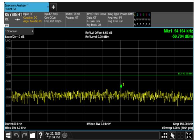
Band4-15MHz-QPSK-20325-1RB#74-0.009~0.15-PASS
