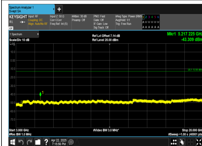
Band4-15MHz-QPSK-20175-1RB#74-3000~20000-PASS
