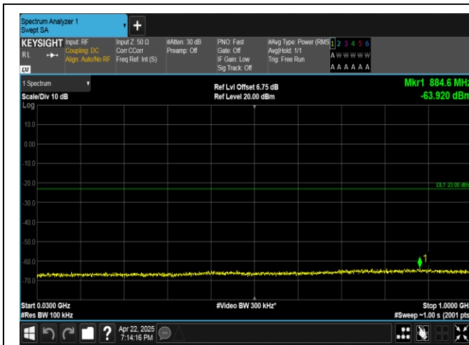
Band4-15MHz-16QAM-20175-1RB#0-30~1000-PASS
