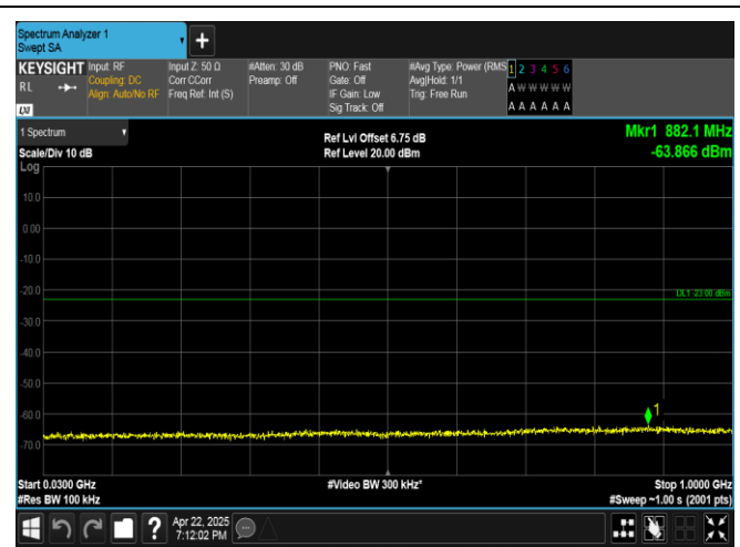
Band4-15MHz-16QAM-20025-75RB#0-30~1000-PASS
