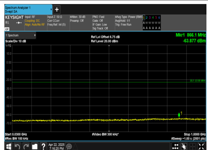
Band4-15MHz-16QAM-20175-1RB#74-30~1000-PASS
