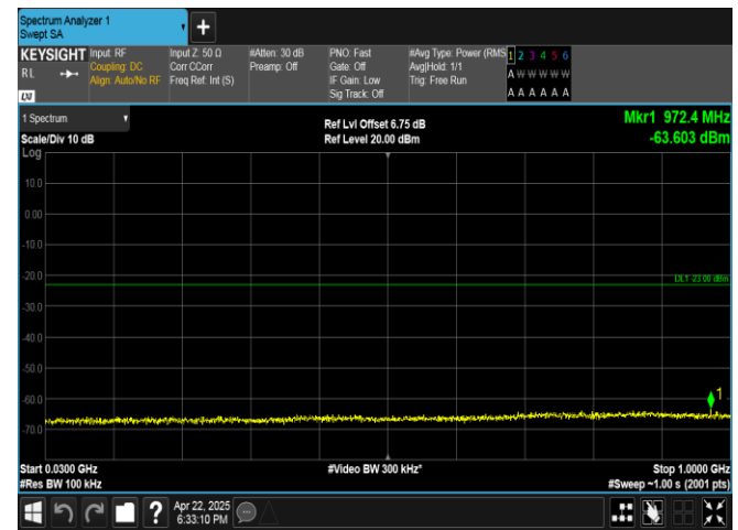
Band4-10MHz-16QAM-20350-1RB#0-30~1000-PASS
