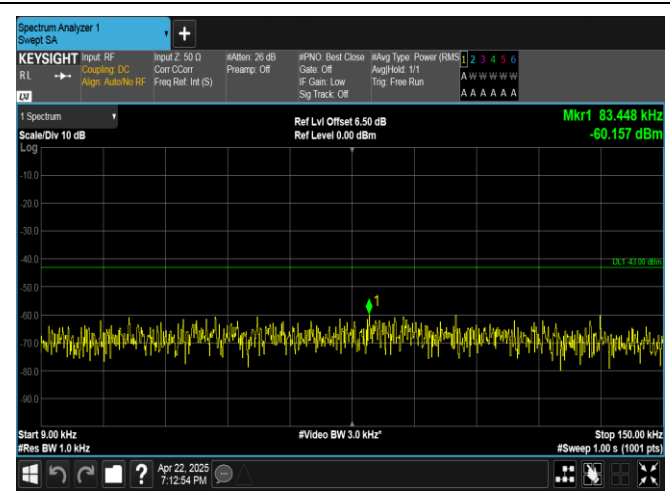
Band4-15MHz-QPSK-20175-1RB#0-0.009~0.15-PASS
