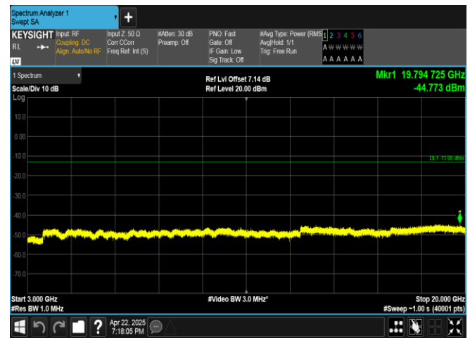
Band4-15MHz-QPSK-20175-75RB#0-3000~20000-PASS
