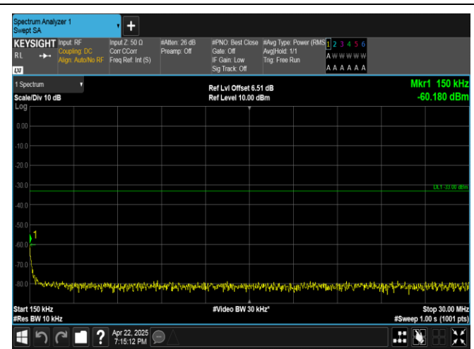
Band4-15MHz-QPSK-20175-1RB#74-0.15~30-PASS
