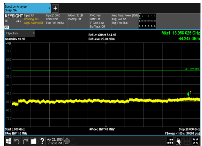
Band4-15MHz-16QAM-20025-75RB#0-3000~20000-PASS
