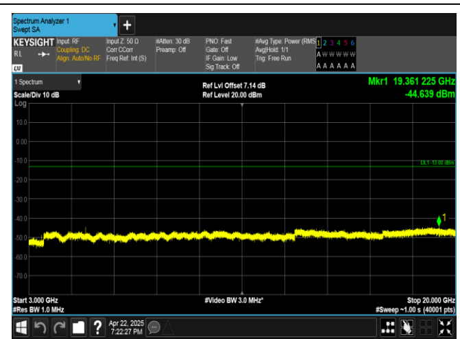
Band4-15MHz-QPSK-20325-1RB#74-3000~20000-PASS
