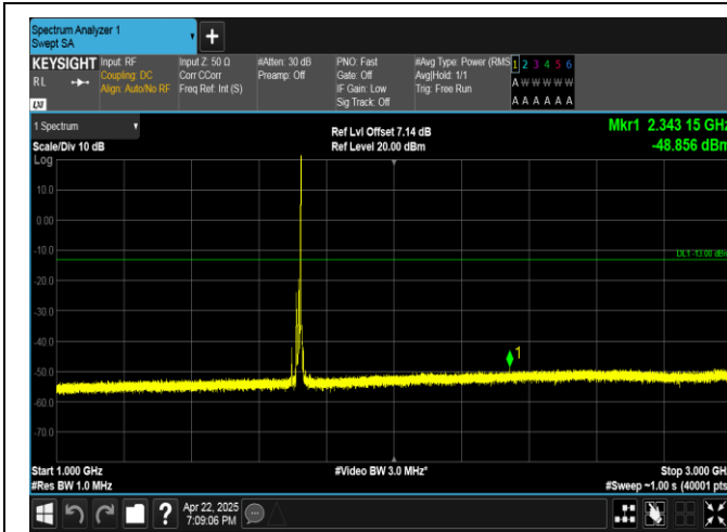
Band4-15MHz-QPSK-2025-1RB#74-1000~3000-PASS
