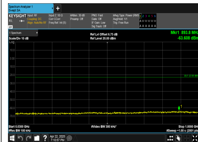
Band4-15MHz-QPSK-2025-75RB#0-30~1000-PASS
