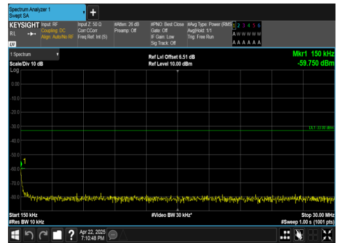
Band4-15MHz-QPSK-2025-75RB#0-0.15~30-PASS
