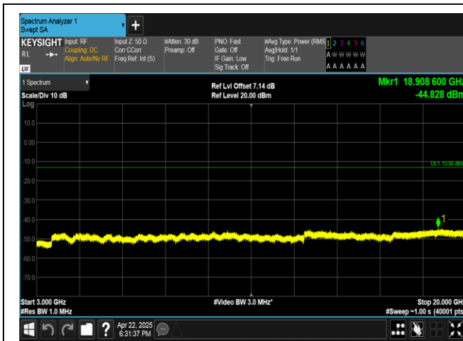
Band4-10MHz-16QAM-20175-50RB#0-3000~20000-PASS
