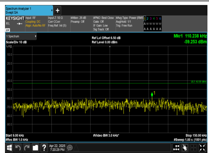
Band4-15MHz-16QAM-20325-1RB#0-0.009~0.15-PASS
