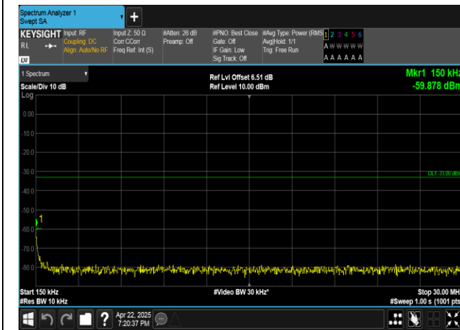
Band4-15MHz-16QAM-20325-1RB#0-0.15~30-PASS
