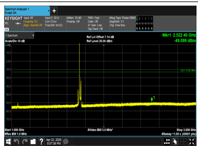
Band4-20MHz-QPSK-20300-1RB#0-1000~3000-PASS
