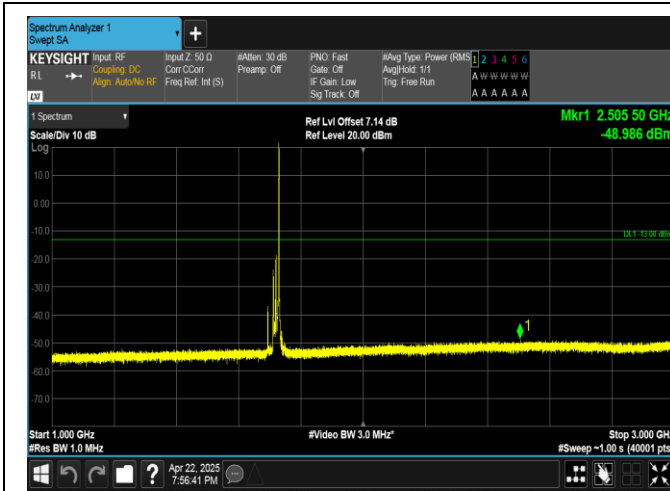
Band4-20MHz-QPSK-20050-1RB#99-1000~3000-PASS
