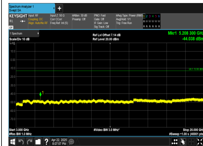
Band4-20MHz-QPSK-20300-1RB#0-3000~20000-PASS
