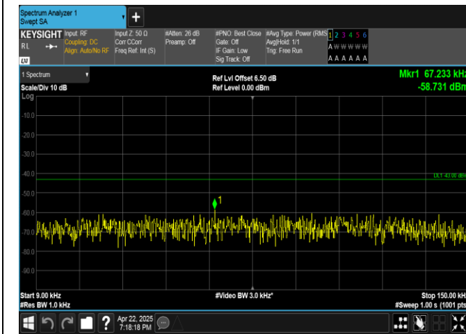
Band4-15MHz-16QAM-20175-75RB#0-0.009~0.15-PASS
