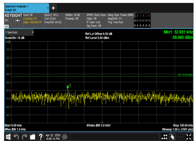
Band4-20MHz-QPSK-20300-1RB#99-0.009~0.15-PASS
