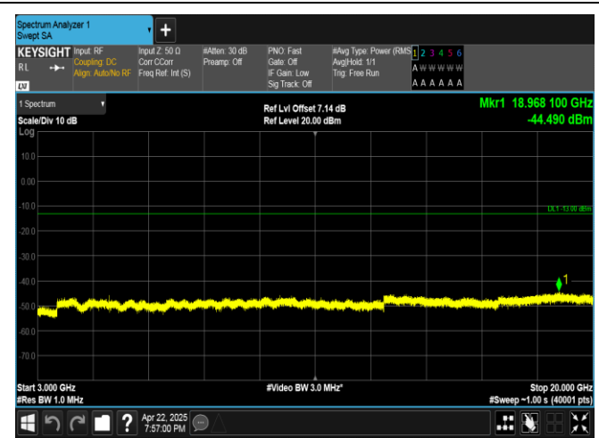
Band4-20MHz-QPSK-20050-1RB#99-3000~20000-PASS
