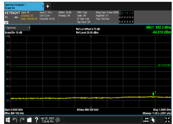
Band4-15MHz-16QAM-20325-1RB#0-30~1000-PASS
