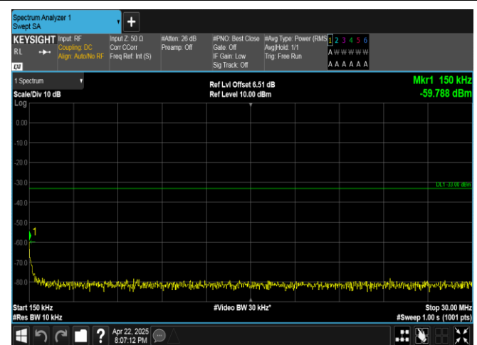
Band4-20MHz-QPSK-20300-1RB#0-0.15~30-PASS
