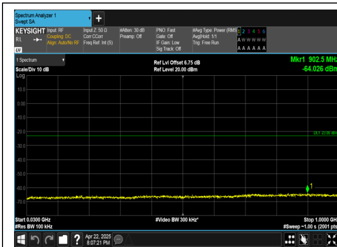
Band4-20MHz-QPSK-20300-1RB#0-30~1000-PASS
