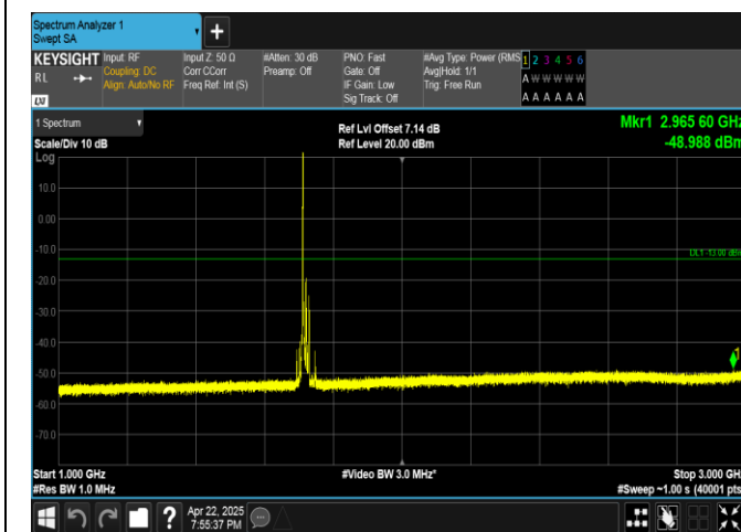
Band4-20MHz-16QAM-20050-1RB#0-1000~3000-PASS
