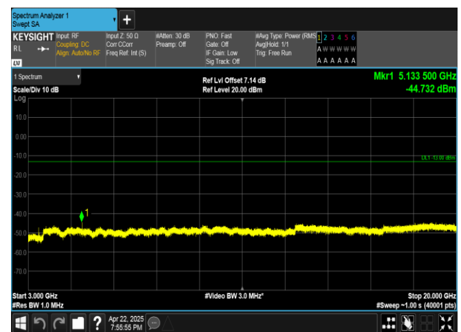
Band4-20MHz-16QAM-20050-1RB#0-3000~20000-PASS
