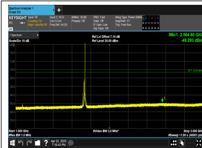
Band4-15MHz-16QAM-20175-1RB#74-1000~3000-PASS
