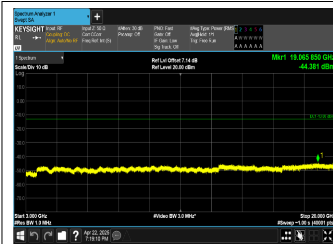
Band4-15MHz-16QAM-20175-75RB#0-3000~20000-PASS
