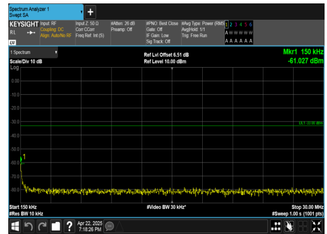
Band4-15MHz-16QAM-20175-75RB#0-0.15~30-PASS
