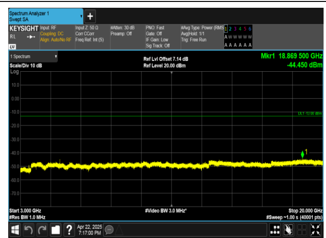
Band4-15MHz-16QAM-20175-1RB#74-3000~20000-PASS
