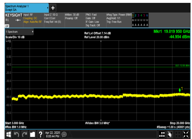
Band4-20MHz-QPSK-20175-100RB#0-3000~20000-PASS
