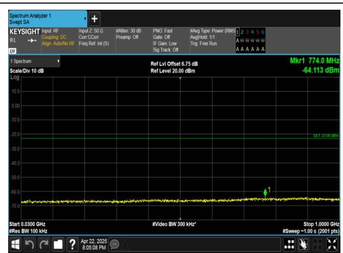
Band4-20MHz-QPSK-20175-100RB#0-30~1000-PASS
