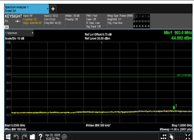
Band4-20MHz-QPSK-20300-1RB#99-30~1000-PASS
