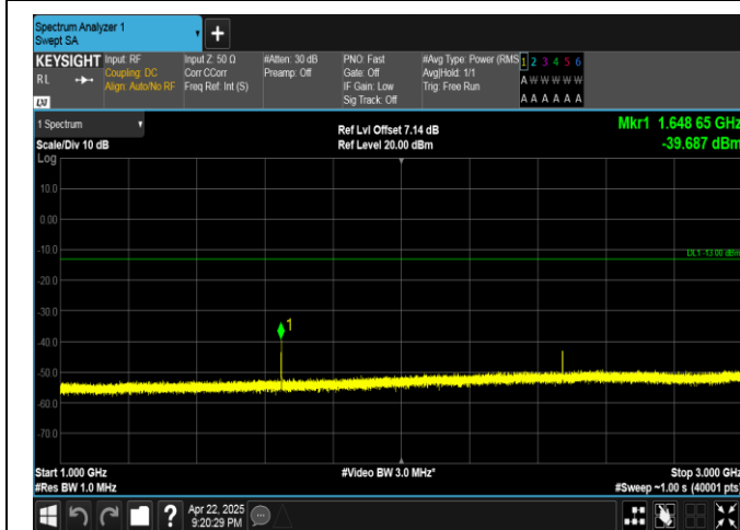
Band5-3MHz-16QAM-20415-1RB#0-1000~3000-PASS
