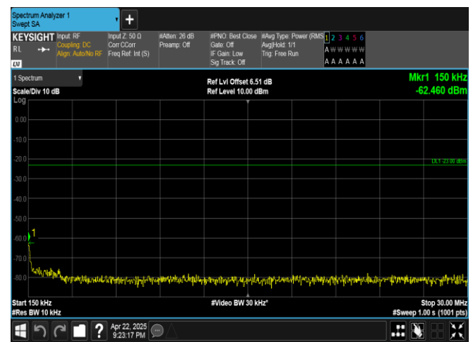
Band5-3MHz-QPSK-20415-15RB#0-0.15~30-PASS
