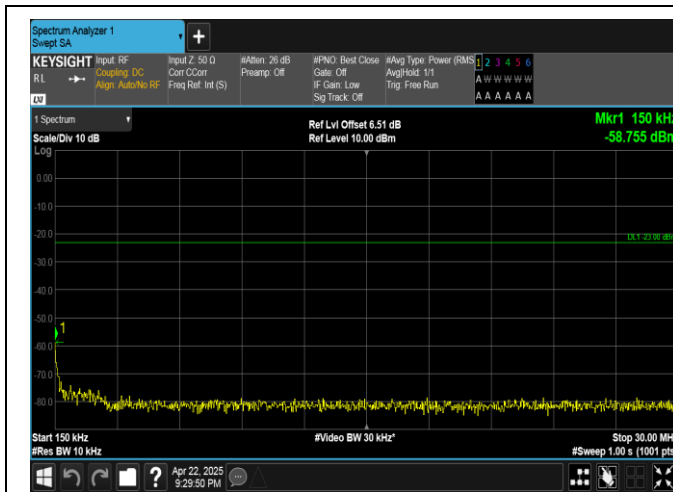
Band5-3MHz-QPSK-20525-15RB#0-0.15~30-PASS
