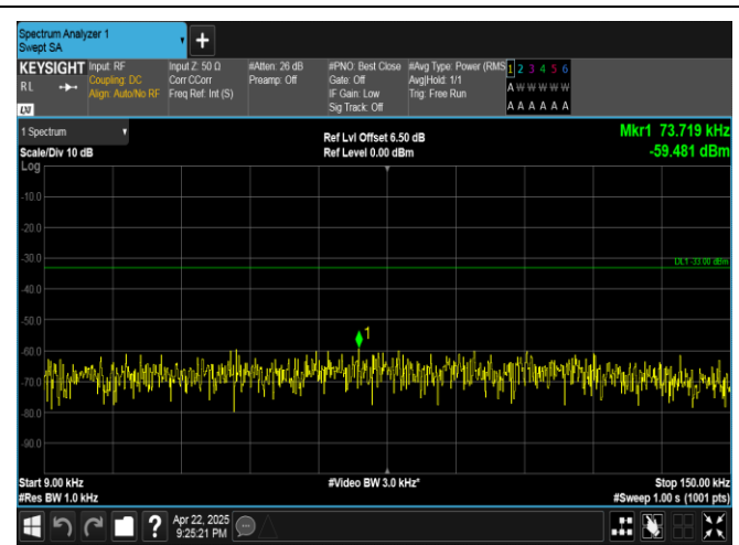
Band5-3MHz-QPSK-20525-1RB#0-0.009~0.15-PASS
