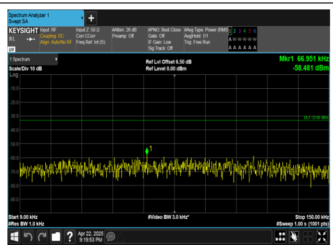
Band5-3MHz-16QAM-20415-1RB#0-0.009~0.15-PASS
