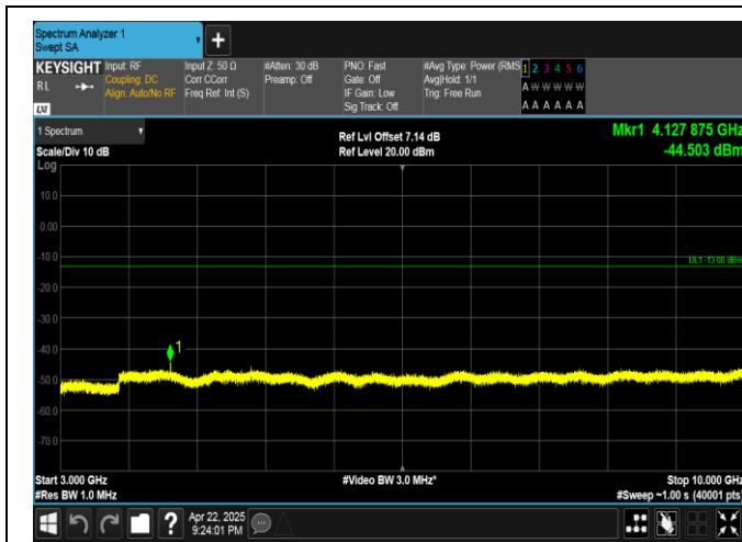
Band5-3MHz-QPSK-20415-15RB#0-3000~10000-PASS
