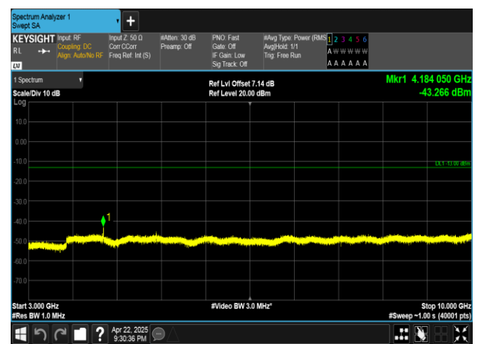
Band5-3MHz-QPSK-20525-15RB#0-3000~10000-PASS
