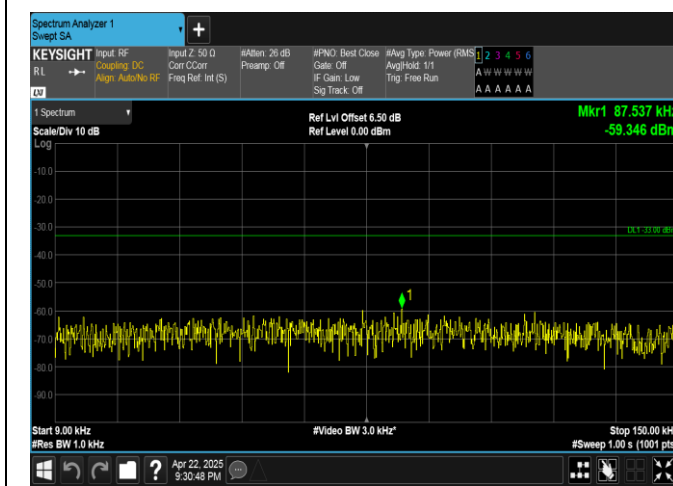
Band5-3MHz-16QAM-20525-15RB#0-0.009~0.15-PASS
