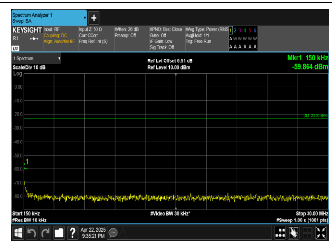
Band5-3MHz-16QAM-20635-1RB#14-0.15~30-PASS
