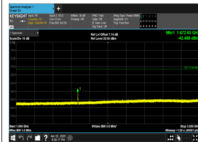
Band5-3MHz-QPSK-20525-15RB#0-1000~3000-PASS
