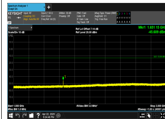
Band5-3MHz-16QAM-20415-15RB#0-1000~3000-PASS
