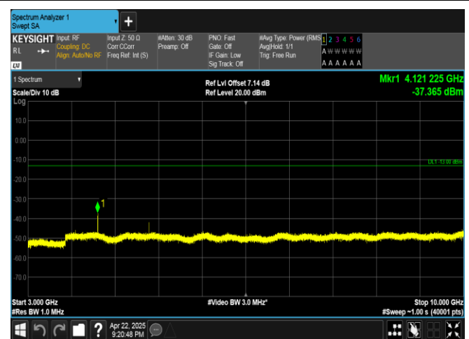
Band5-3MHz-16QAM-20415-1RB#0-3000~10000-PASS
