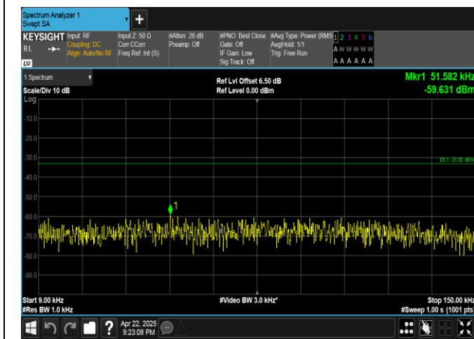
Band5-3MHz-QPSK-20415-15RB#0-0.009~0.15-PASS
