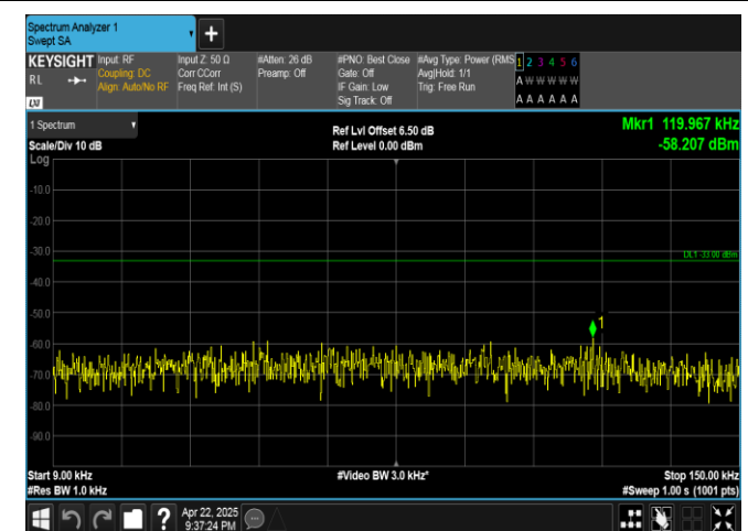
Band5-3MHz-16QAM-20635-15RB#0-0.009~0.15-PASS
