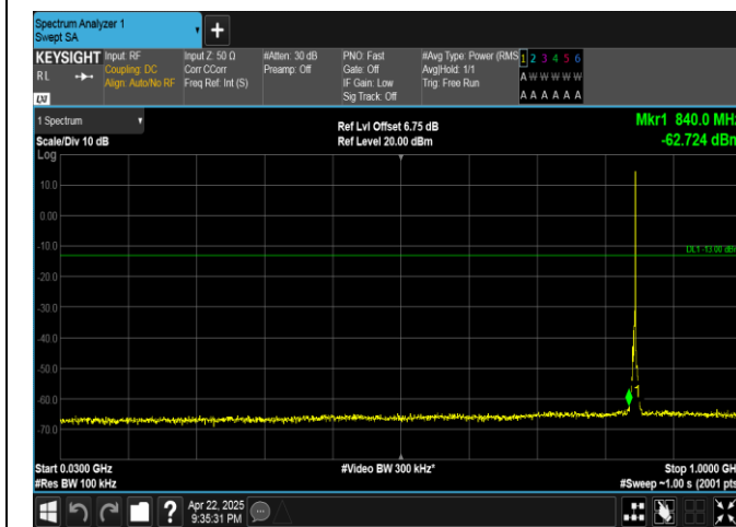
Band5-3MHz-16QAM-20635-1RB#14-30~1000-PASS
