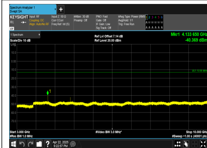
Band5-3MHz-16QAM-20415-1RB#14-3000~10000-PASS
