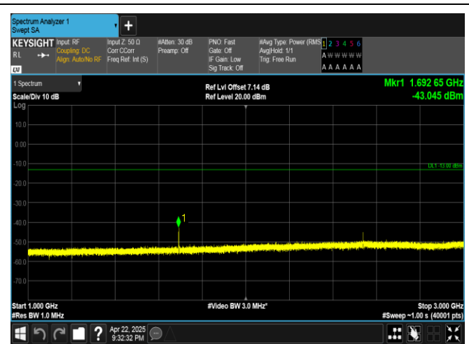
Band5-3MHz-QPSK-20635-1RB#0-1000~3000-PASS
