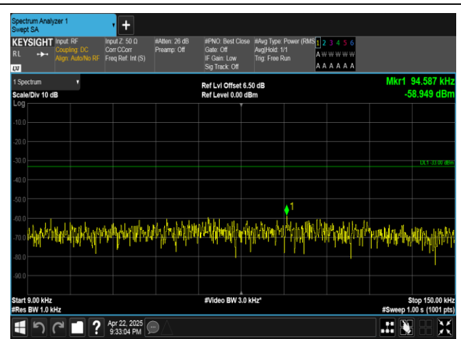
Band5-3MHz-16QAM-20635-1RB#0-0.009~0.15-PASS
