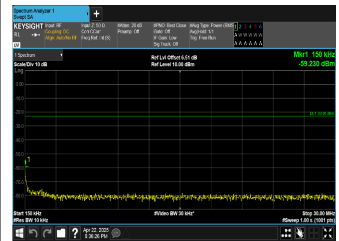
Band5-3MHz-QPSK-20635-15RB#0-0.15~30-PASS
