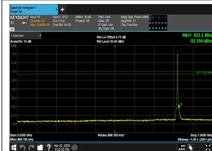
Band5-3MHz-QPSK-20415-15RB#0-30~1000-PASS
