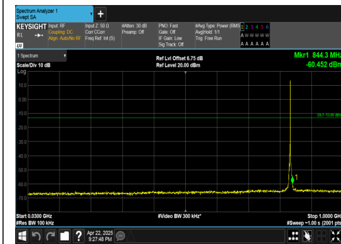
Band5-3MHz-QPSK-20525-1RB#14-30~1000-PASS
