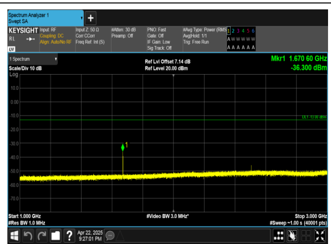
Band5-3MHz-16QAM-20525-1RB#0-1000~3000-PASS
