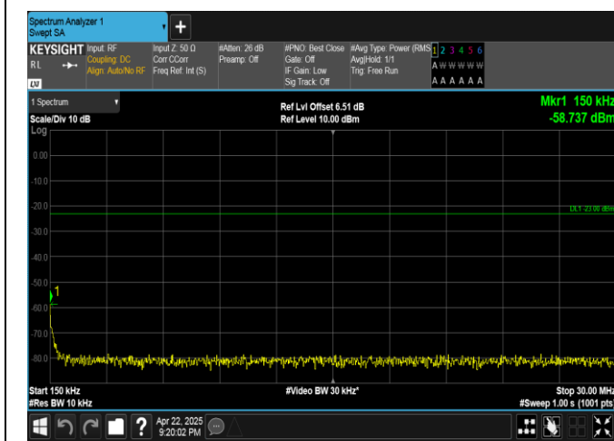
Band5-3MHz-16QAM-20415-1RB#0-0.15~30-PASS
