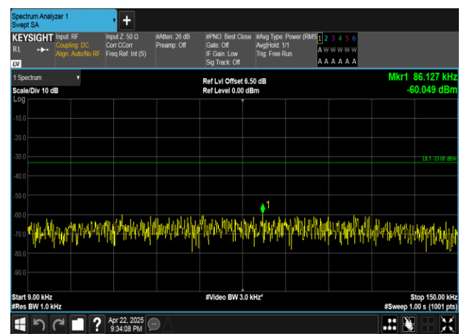
Band5-3MHz-QPSK-20635-1RB#14-0.009~0.15-PASS
