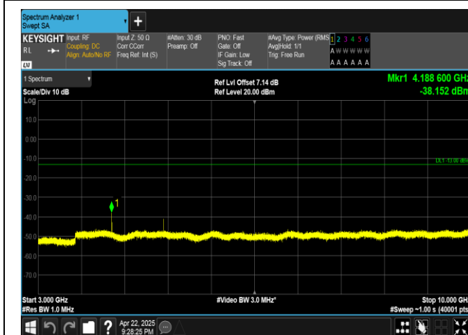
Band5-3MHz-QPSK-20525-1RB#14-3000~10000-PASS
