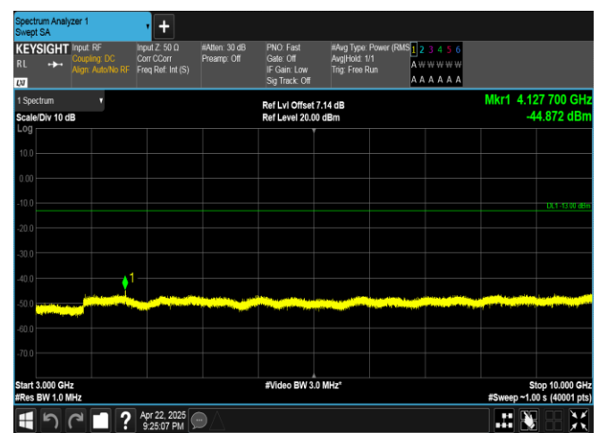
Band5-3MHz-16QAM-20415-15RB#0-3000~10000-PASS
