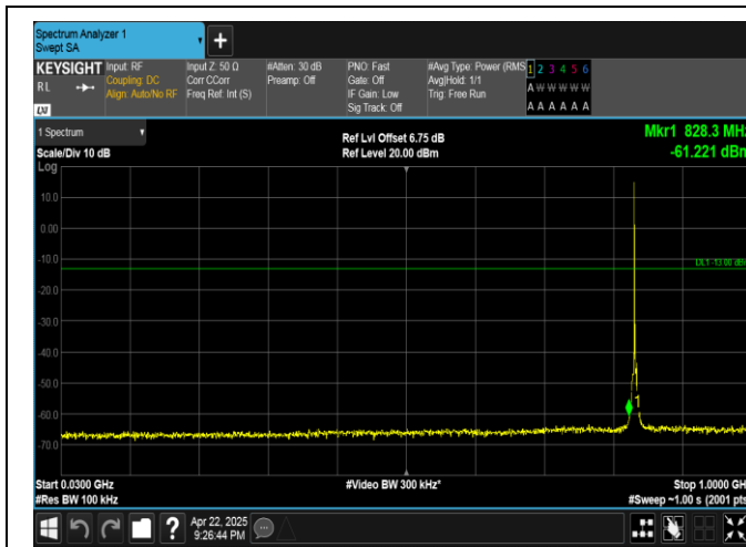
Band5-3MHz-16QAM-20525-1RB#0-30~1000-PASS
