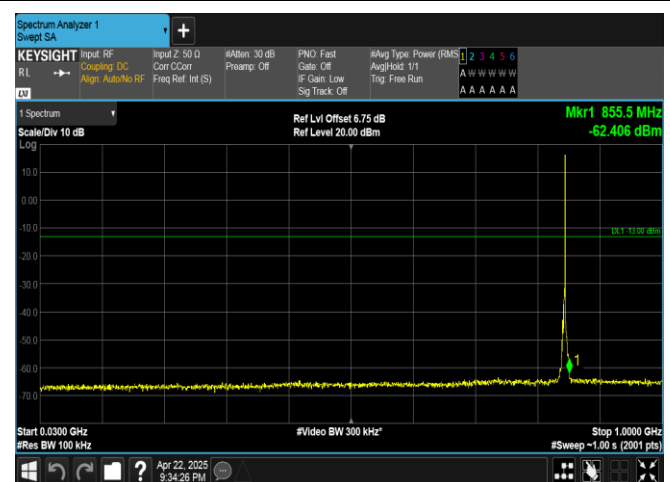
Band5-3MHz-QPSK-20635-1RB#14-30~1000-PASS
