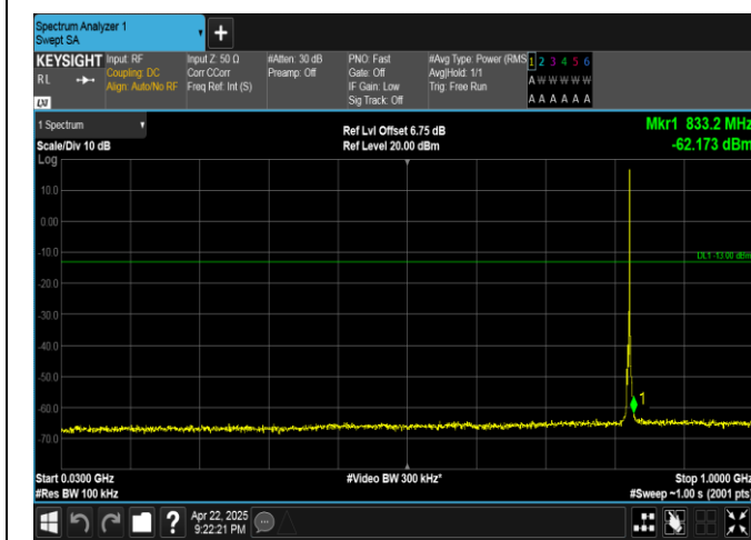
Band5-3MHz-16QAM-20415-1RB#14-30~1000-PASS
