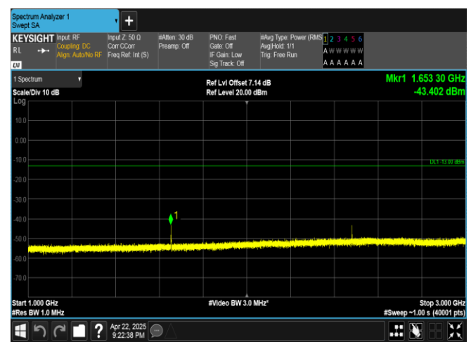
Band5-3MHz-16QAM-20415-1RB#14-1000~3000-PASS
