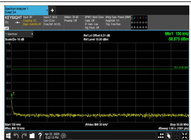
Band5-3MHz-16QAM-20415-1RB#14-0.15~30-PASS
