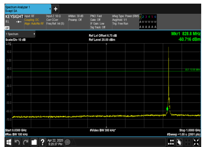
Band5-3MHz-QPSK-20525-1RB#0-30~1000-PASS
