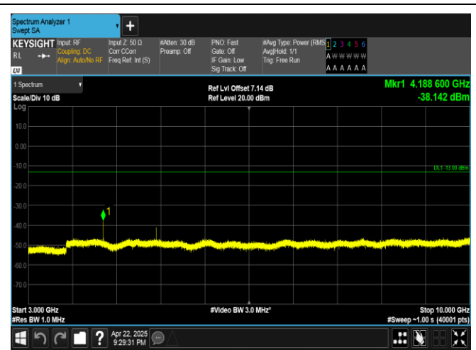
Band5-3MHz-16QAM-20525-1RB#14-3000~10000-PASS
