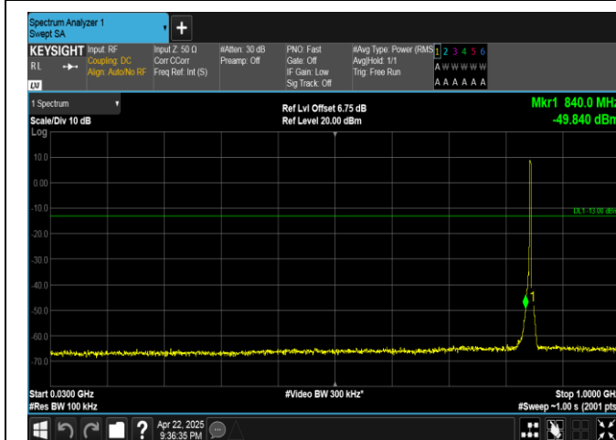
Band5-3MHz-QPSK-20635-15RB#0-30~1000-PASS
