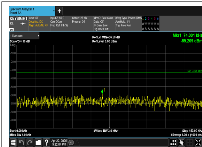
Band5-3MHz-16QAM-20415-1RB#14-0.009~0.15-PASS
