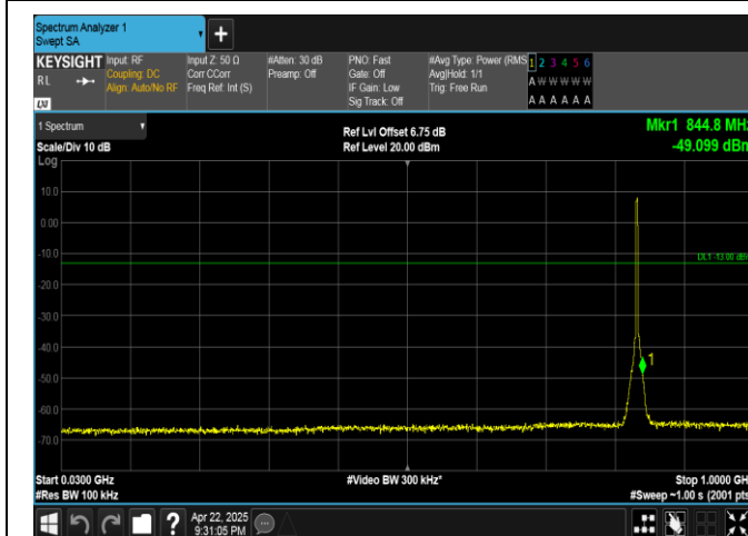
Band5-3MHz-16QAM-20525-15RB#0-30~1000-PASS
