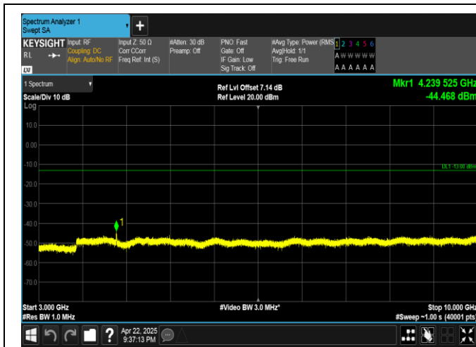
Band5-3MHz-QPSK-20635-15RB#0-3000~10000-PASS
