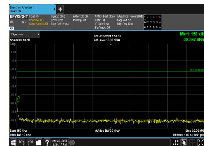
Band5-3MHz-QPSK-20635-1RB#14-0.15~30-PASS
