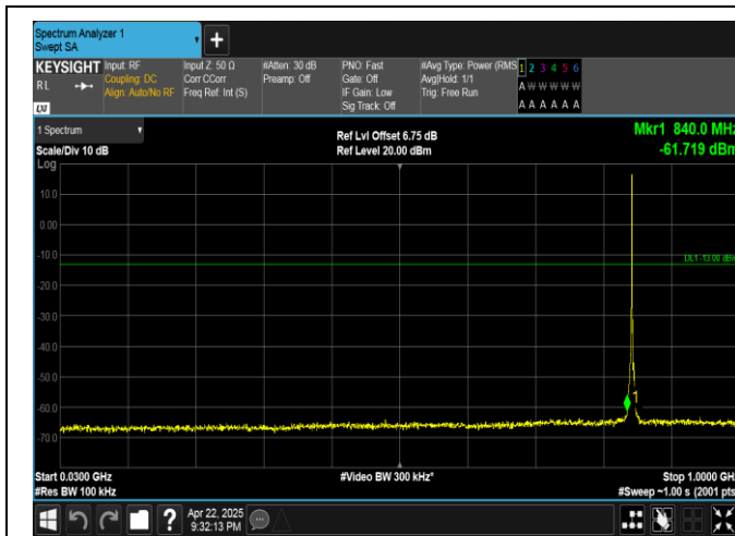
Band5-3MHz-QPSK-20635-1RB#0-30~1000-PASS
