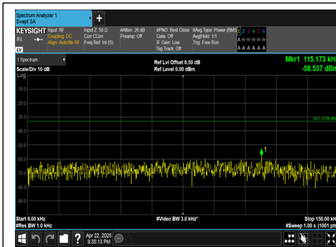
Band5-3MHz-16QAM-20635-1RB#14-0.009~0.15-PASS
