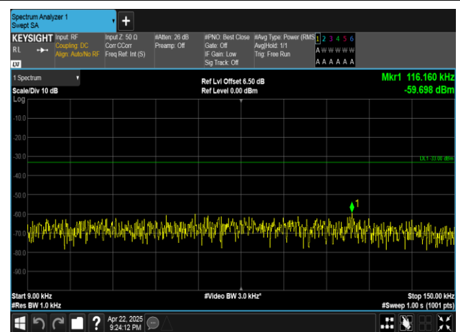
Band5-3MHz-16QAM-20415-15RB#0-0.009~0.15-PASS
