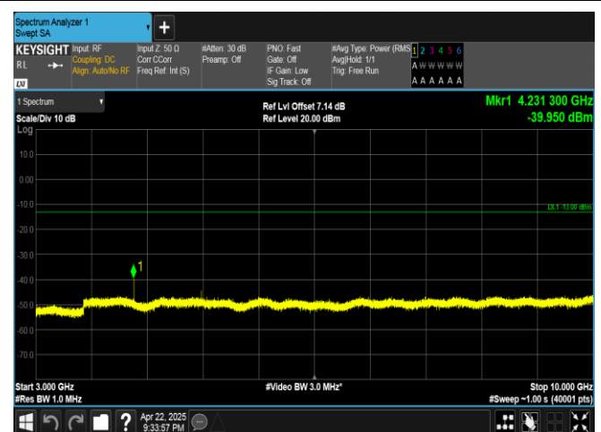
Band5-3MHz-16QAM-20635-1RB#0-3000~10000-PASS
