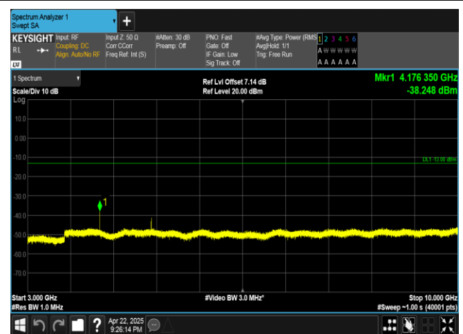
Band5-3MHz-QPSK-20525-1RB#0-3000~10000-PASS
