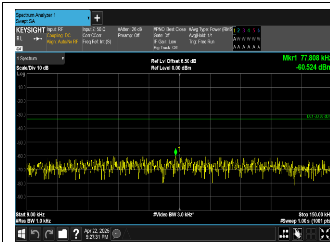
Band5-3MHz-QPSK-20525-1RB#14-0.009~0.15-PASS
