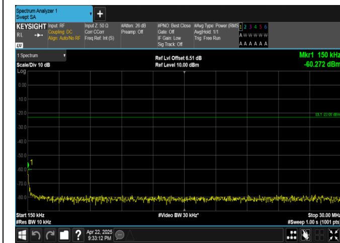
Band5-3MHz-16QAM-20635-1RB#0-0.15~30-PASS
