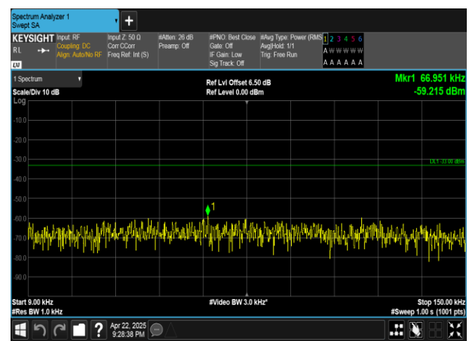
Band5-3MHz-16QAM-20525-1RB#14-0.009~0.15-PASS
