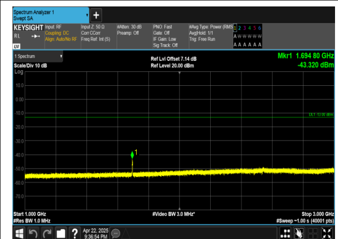
Band5-3MHz-QPSK-20635-15RB#0-1000~3000-PASS
