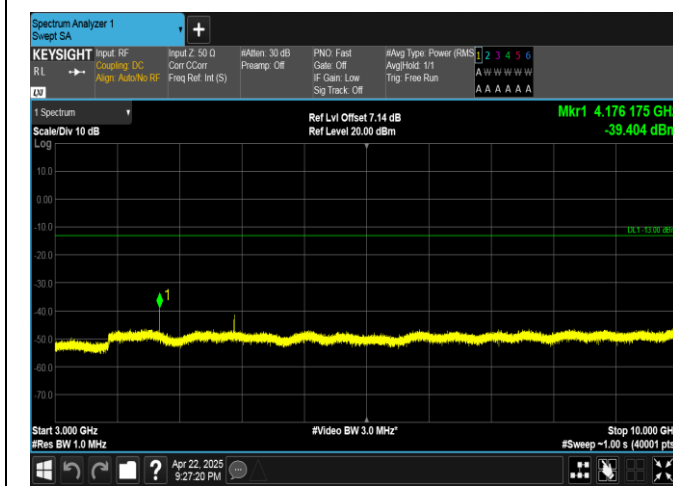
Band5-3MHz-16QAM-20525-1RB#0-3000~10000-PASS
