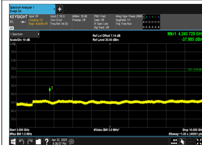
Band5-3MHz-16QAM-20635-1RB#14-3000~10000-PASS
