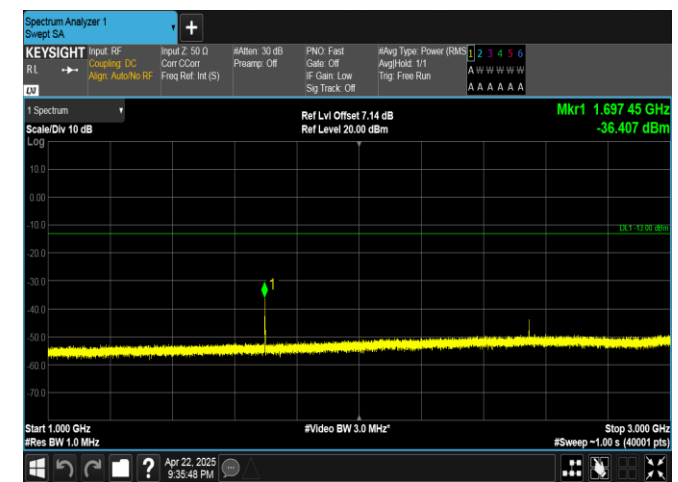
Band5-3MHz-16QAM-20635-1RB#14-1000~3000-PASS
