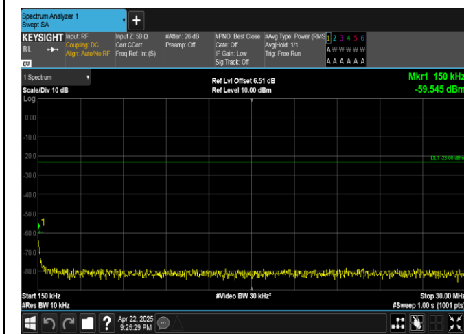
Band5-3MHz-QPSK-20525-1RB#0-0.15~30-PASS
