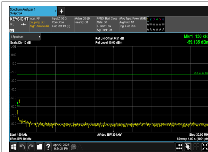
Band5-3MHz-16QAM-20415-15RB#0-0.15~30-PASS
