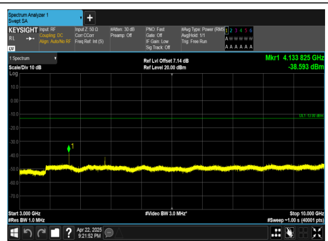
Band5-3MHz-QPSK-20415-1RB#14-3000~10000-PASS
