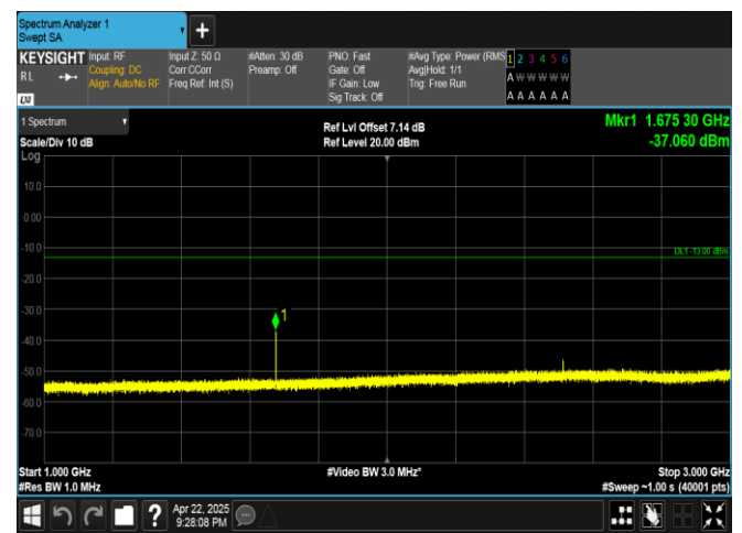
Band5-3MHz-QPSK-20525-1RB#14-1000~3000-PASS
