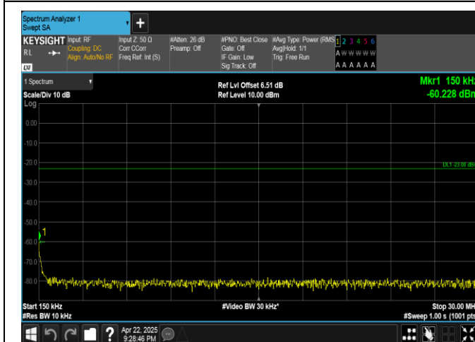
Band5-3MHz-16QAM-20525-1RB#14-0.15~30-PASS
