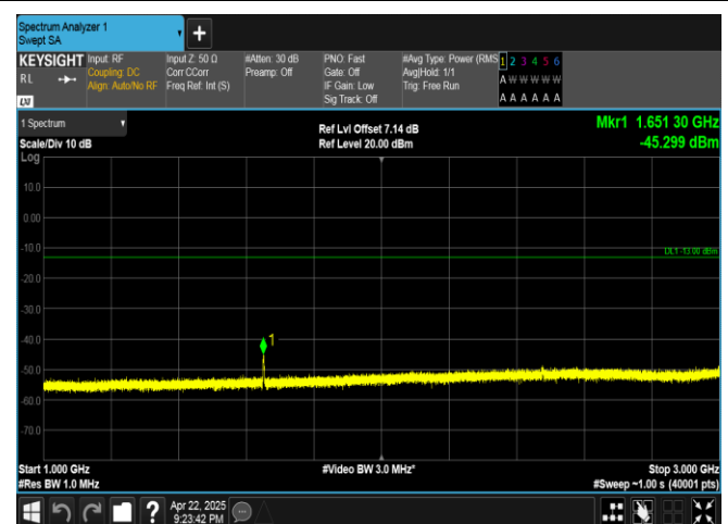
Band5-3MHz-QPSK-20415-15RB#0-1000~3000-PASS
