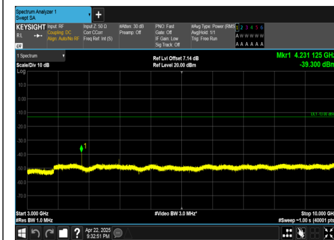
Band5-3MHz-QPSK-20635-1RB#0-3000~10000-PASS
