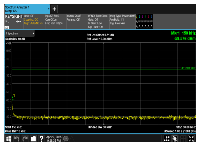
Band5-3MHz-16QAM-20525-1RB#0-0.15~30-PASS
