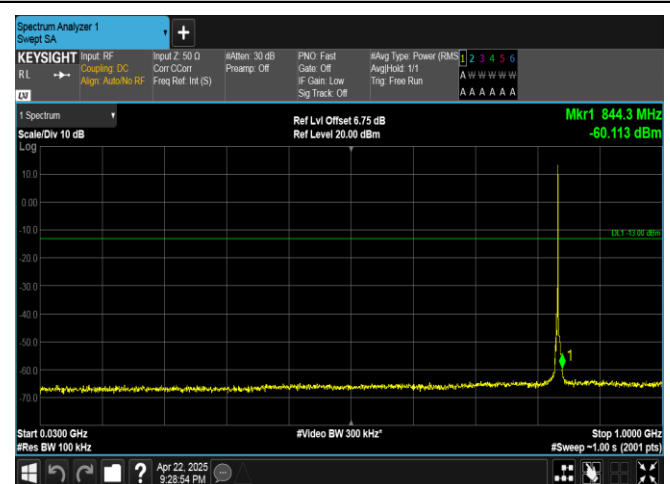
Band5-3MHz-16QAM-20525-1RB#14-30~1000-PASS
