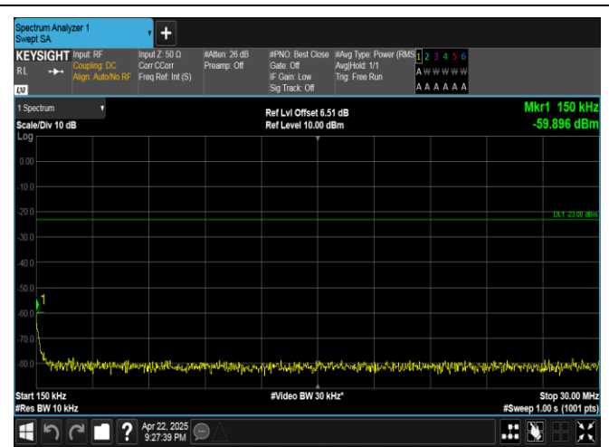
Band5-3MHz-QPSK-20525-1RB#14-0.15~30-PASS
