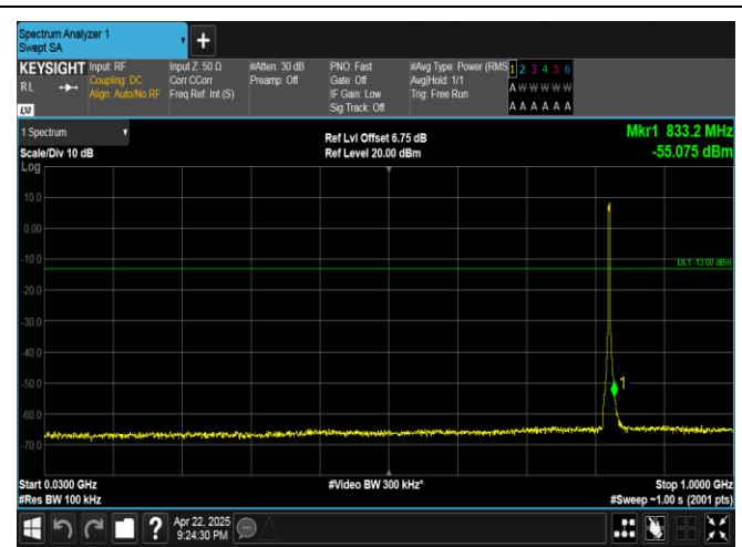
Band5-3MHz-16QAM-20415-15RB#0-30~1000-PASS
