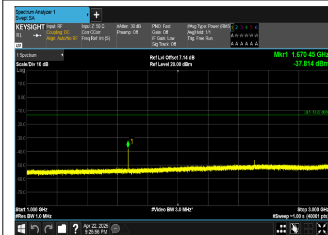
Band5-3MHz-QPSK-20525-1RB#0-1000~3000-PASS
