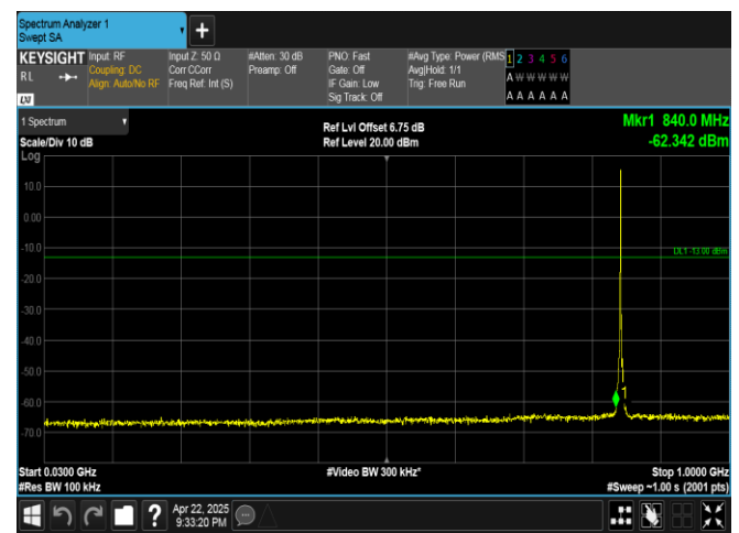
Band5-3MHz-16QAM-20635-1RB#0-30~1000-PASS
