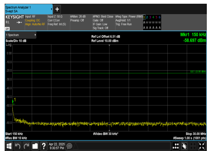
Band5-3MHz-16QAM-20525-15RB#0-0.15~30-PASS
