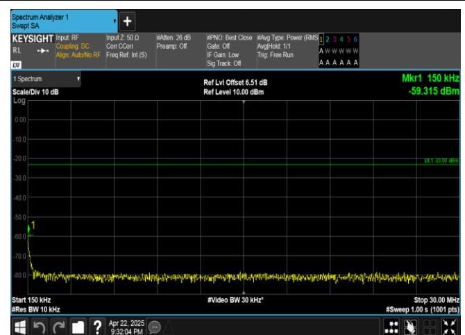
Band5-3MHz-QPSK-20635-1RB#0-0.15~30-PASS
