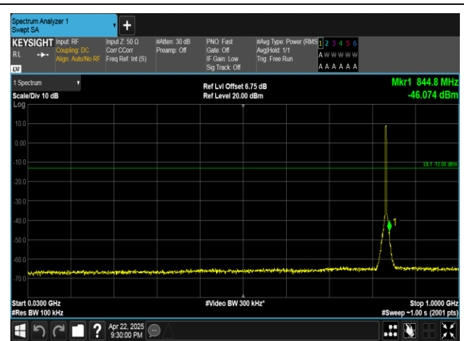
Band5-3MHz-QPSK-20525-15RB#0-30~1000-PASS
