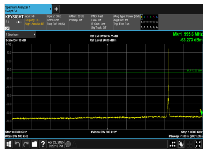
Band5-3MHz-16QAM-20415-1RB#0-30~1000-PASS
