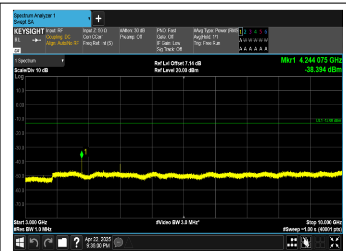
Band5-3MHz-QPSK-20635-1RB#14-3000~10000-PASS
