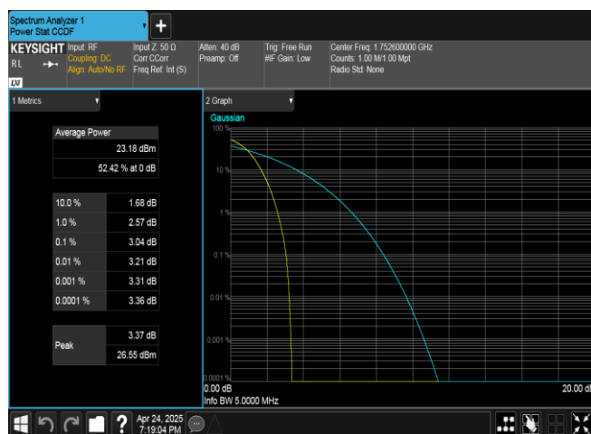
Band4-1513-1-PASS
