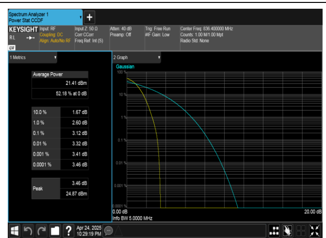
Band5-4182-PASS
