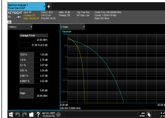
Band5-4233-PASS
