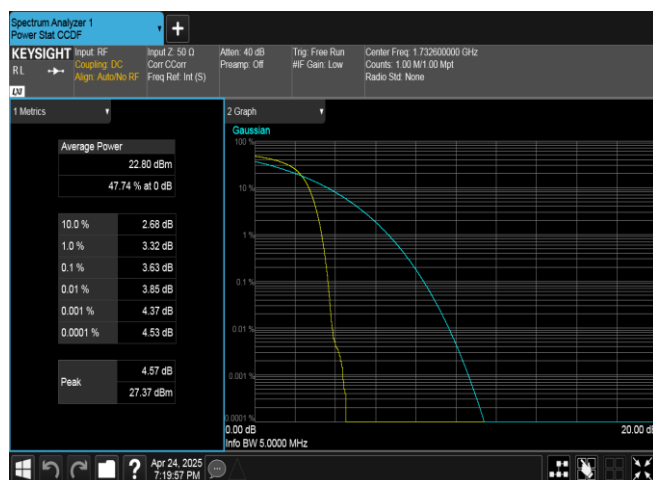
Band4-1413-2-PASS
