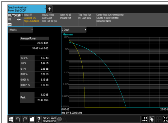
Band5-4132-PASS
